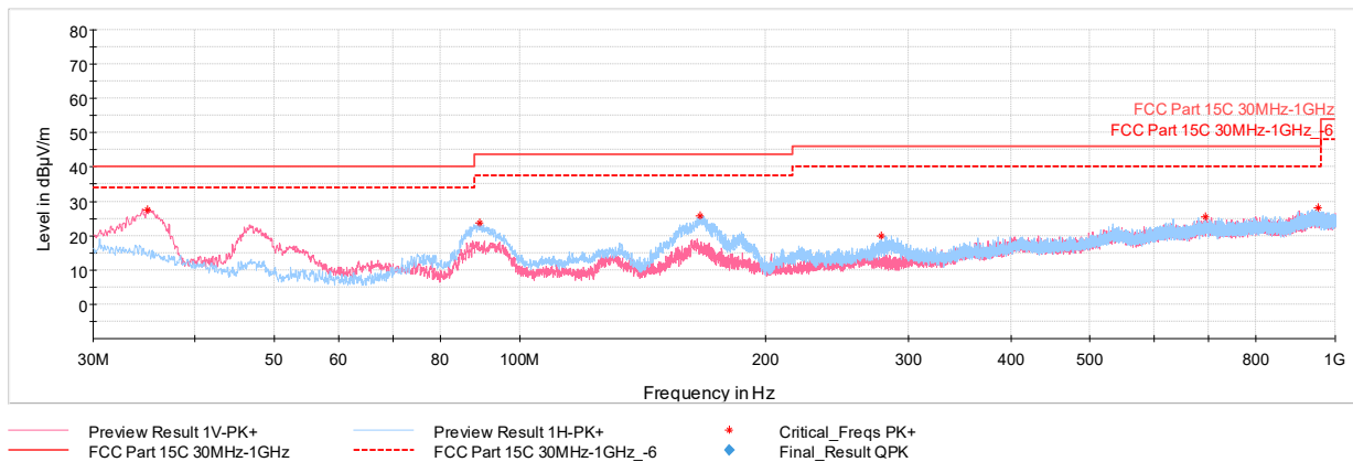
Plot 7-918. Radiated Spurious Plot below 1GHz CDD/SDM (RU242 - Ch. 36), with AC/DC Adapter
