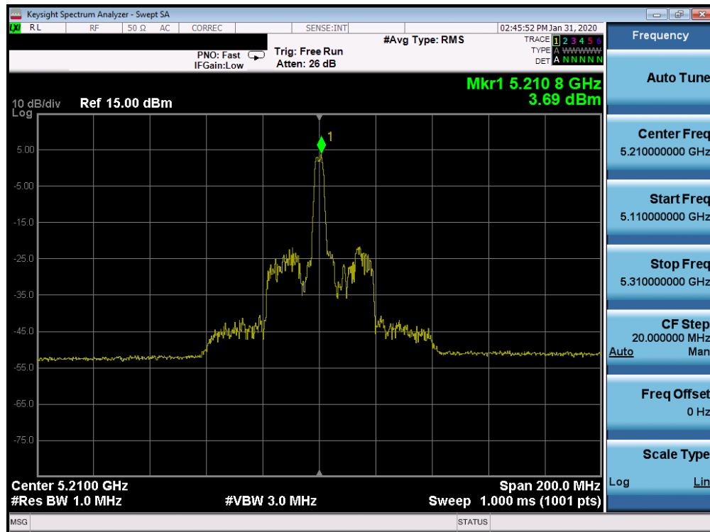
Plot 7-438. Power Spectral Density Plot ISSED SISO CORE 1 (80MHz BW 802.11ax Index 18 – RU26 (UNII Band 1) – Ch. 42)
