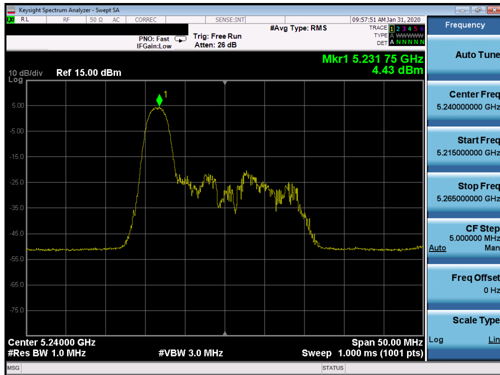
Plot 7-423. Power Spectral Density Plot ISD SISO CORE 1 (20MHz BW 802.11ax Index 0 – RU26 (UNII Band 1) – Ch. 48)
