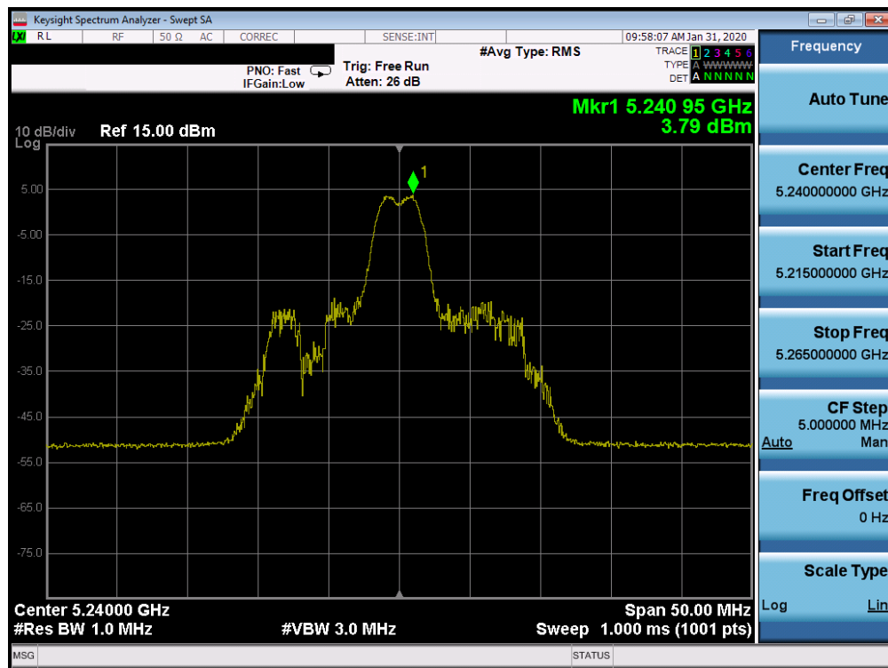
Plot 7-424. Power Spectral Density Plot ISD SISO CORE 1 (20MHz BW 802.11ax Index 4 – RU26 (UNII Band 1) – Ch. 48)
