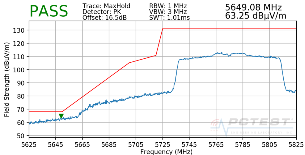
Plot 7-254. Radiated Lower Band Edge Plot SISO CORE1 (Peak – UNII Band 3)
