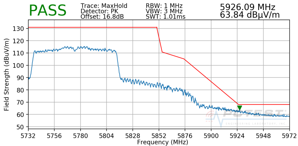
Plot 7-280. Radiated Upper Band Edge Plot CDD (Peak – UNII Band 3)
