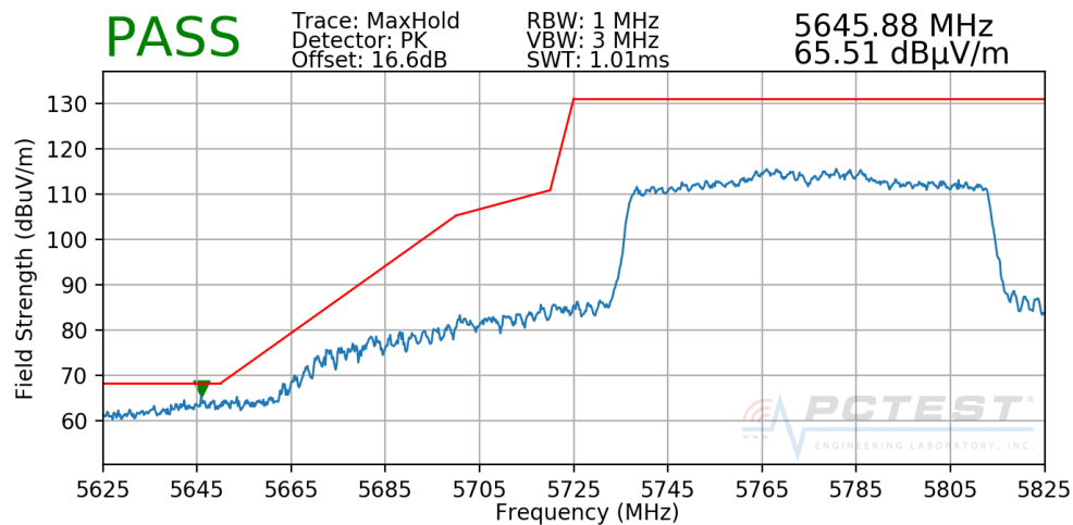
Plot 7-279. Radiated Lower Band Edge Plot CDD (Peak - UNII Band 3)
