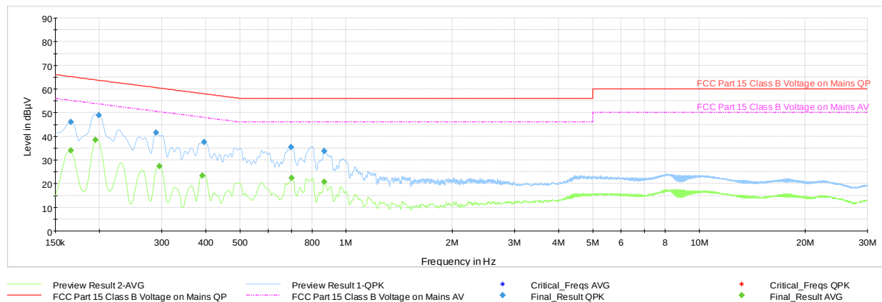
Plot 7-284. Line Conducted Plot with 802.11n UNII Band 1 – Ch.36 (N), with AC/DC Adapter)
