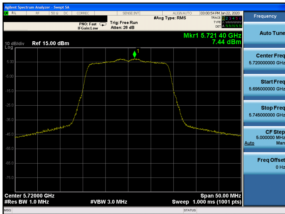
Plot 7-99. Power Spectral Density Plot SISO CORE1 (20MHz BW 802.11n (UNII Band 2C) – Ch. 144)
