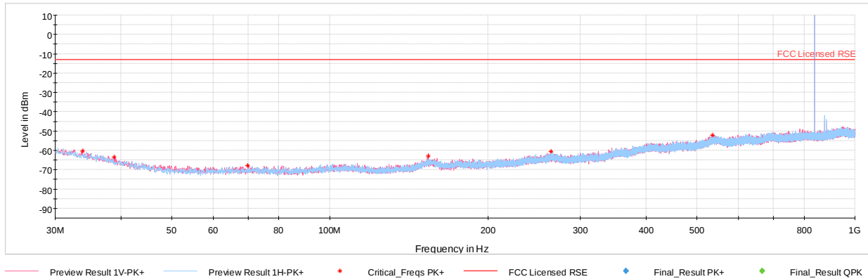
Plot 7-76. Radiated Spurious Plot Below 1GHz (Cellular GPRS Mode) with AC/DC Adapter
