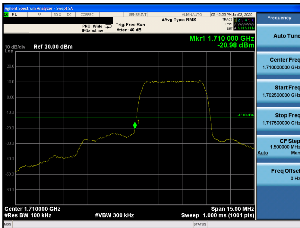
Plot 7-61. Band Edge Plot (AWS WCDMA Mode - Low Channel)
