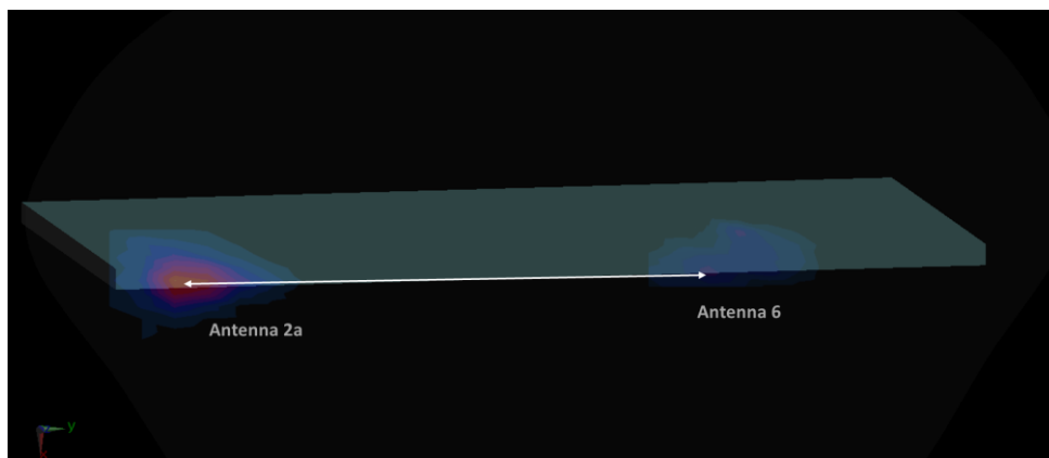
Figure 11-35 Left Edge Spatial Separation for Antenna 2A and Antenna 6
