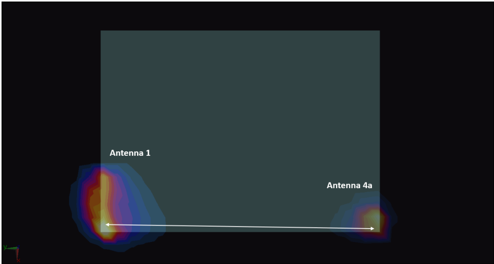
Figure 11-1 Back Side Spatial Separation for Antenna 4A and Antenna 1
