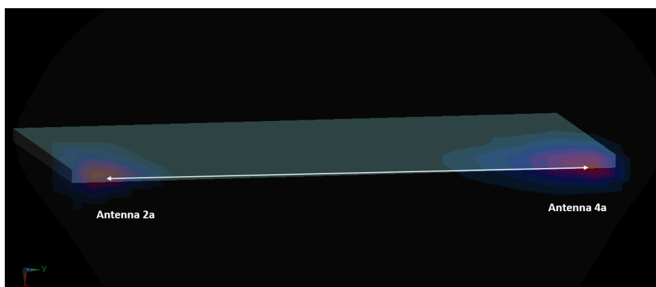
Figure 11-33 Left Edge Spatial Separation for Antenna 2A and Antenna 4A
