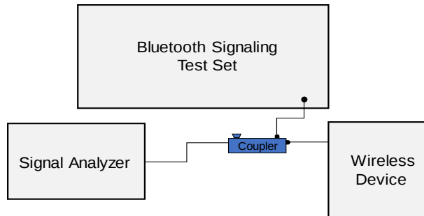
Figure 8-11 Power Measurement Setup
