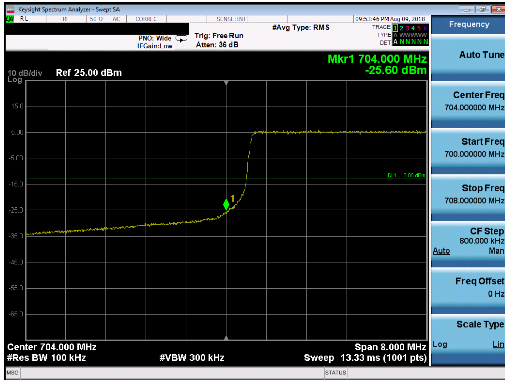
Plot 7-196. Lower Band Edge Plot (Band 17 – 10.0MHz QPSK – RB Size 50)
