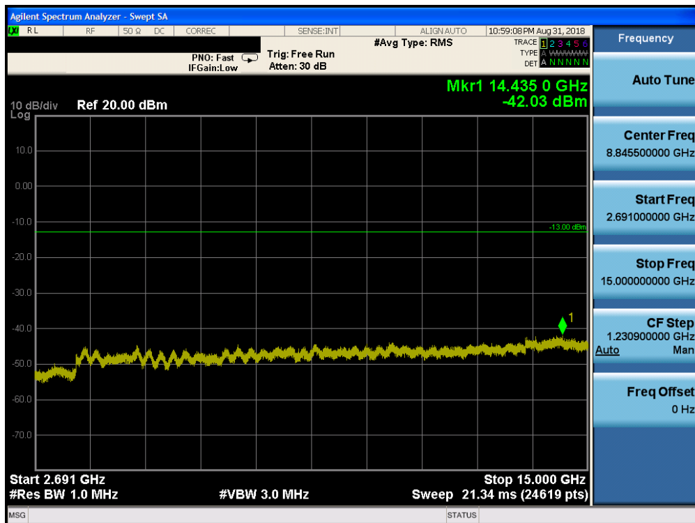
Plot 7-176. Conducted Spurious Plot (Band 41 – 20.0MHz QPSK – RB Size 1, RB Offset 0 – High Channel)
