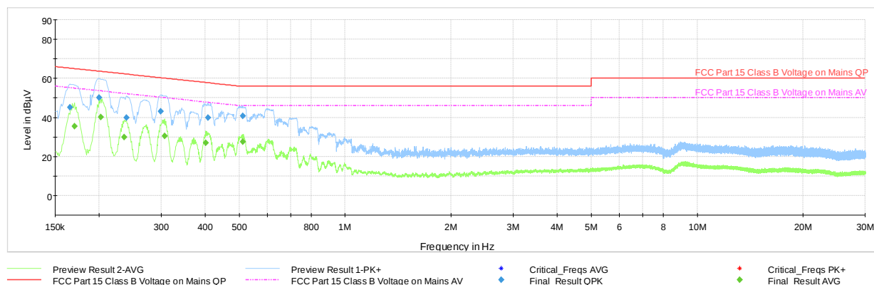
Plot 7-168. Line Conducted Plot with 802.11n CDD Primary (L1, with AC/DC Adapter)
