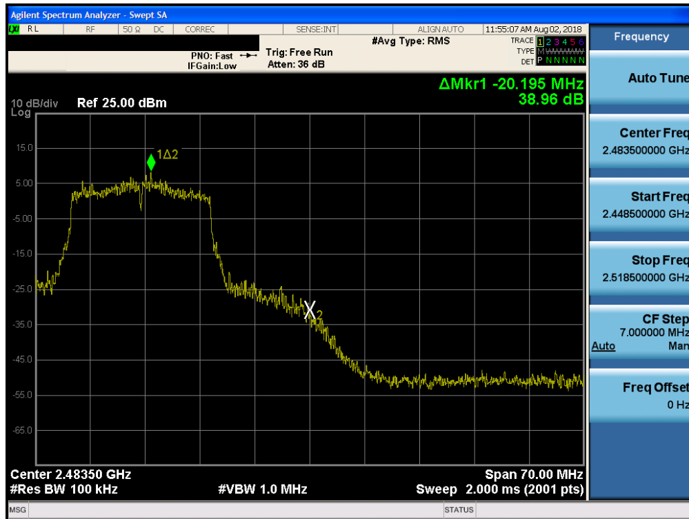
Plot 7-90. Band Edge Plot SISO CORE1 PRIMARY (802.11n (2.4GHz) – Ch. 11)
