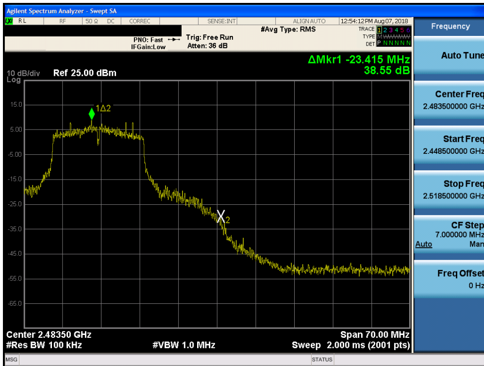
Plot 7-94. Band Edge Plot SISO CORE1 DIVERSITY (802.11g - Ch. 11)
