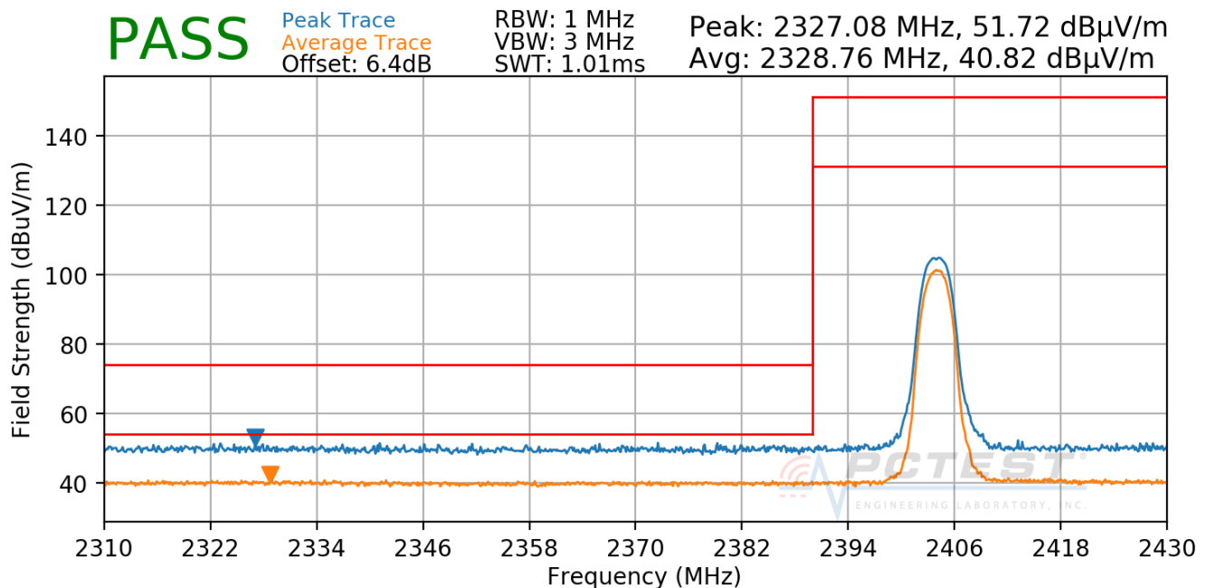
Plot 7-105. Radiated Restricted Lower Band Edge Measurement ANT0 (Average & Peak)
