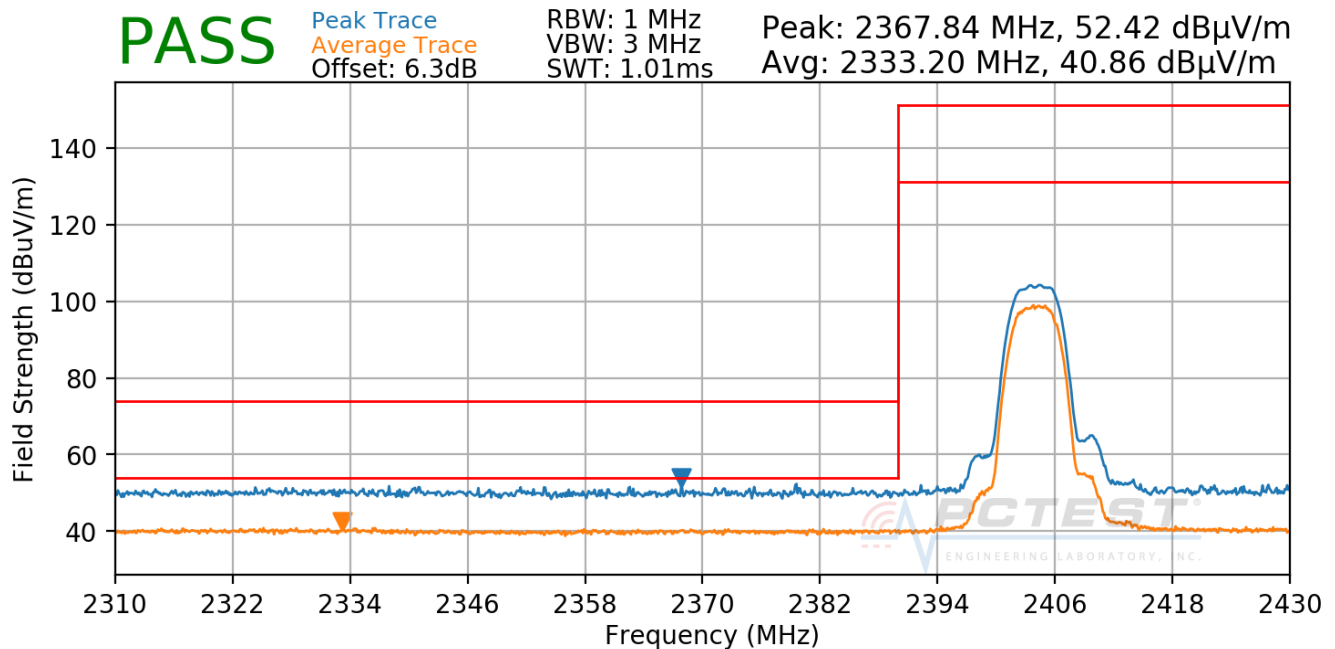
Plot 7-106. Radiated Restricted Lower Band Edge Measurement ANT0 (Average & Peak)
