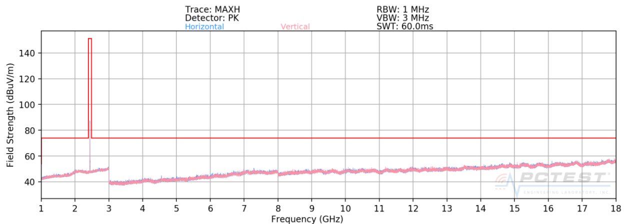
Plot 7-101. Radiated Spurious Plot Above 1GHz ANT2 (4Mbps, HDR4 ePA – Ch. 38, Ant. Pol. H & V)
