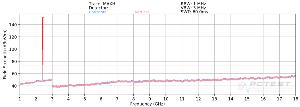
Plot 7-94. Radiated Spurious Plot Above 1GHz ANT1 (8Mbps, HDR8 ePA – Ch. 1, Ant. Pol. H & V)
