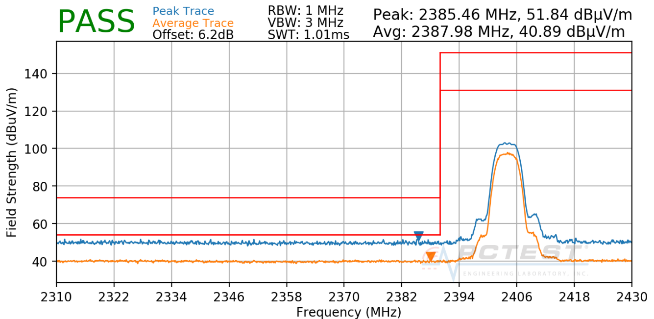
Plot 7-110. Radiated Restricted Lower Band Edge Measurement ANT1 (Average & Peak)
