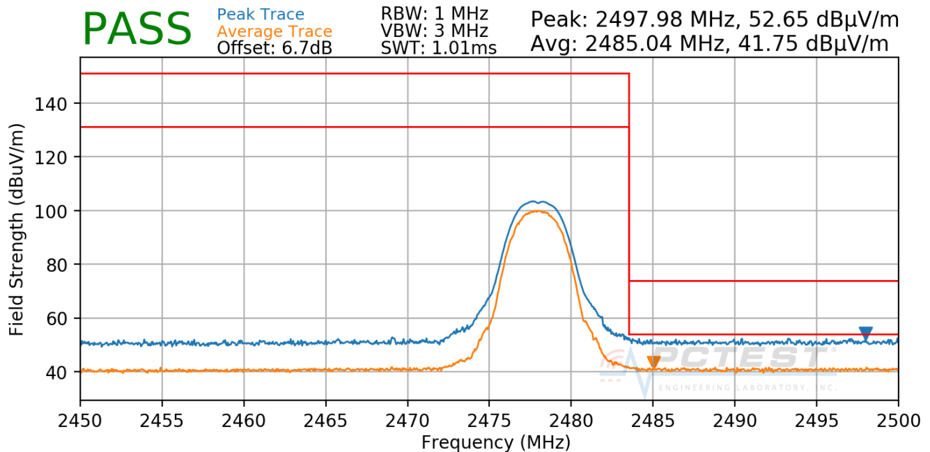
Plot 7-111. Radiated Restricted Upper Band Edge Measurement ANT1 (Average & Peak)
