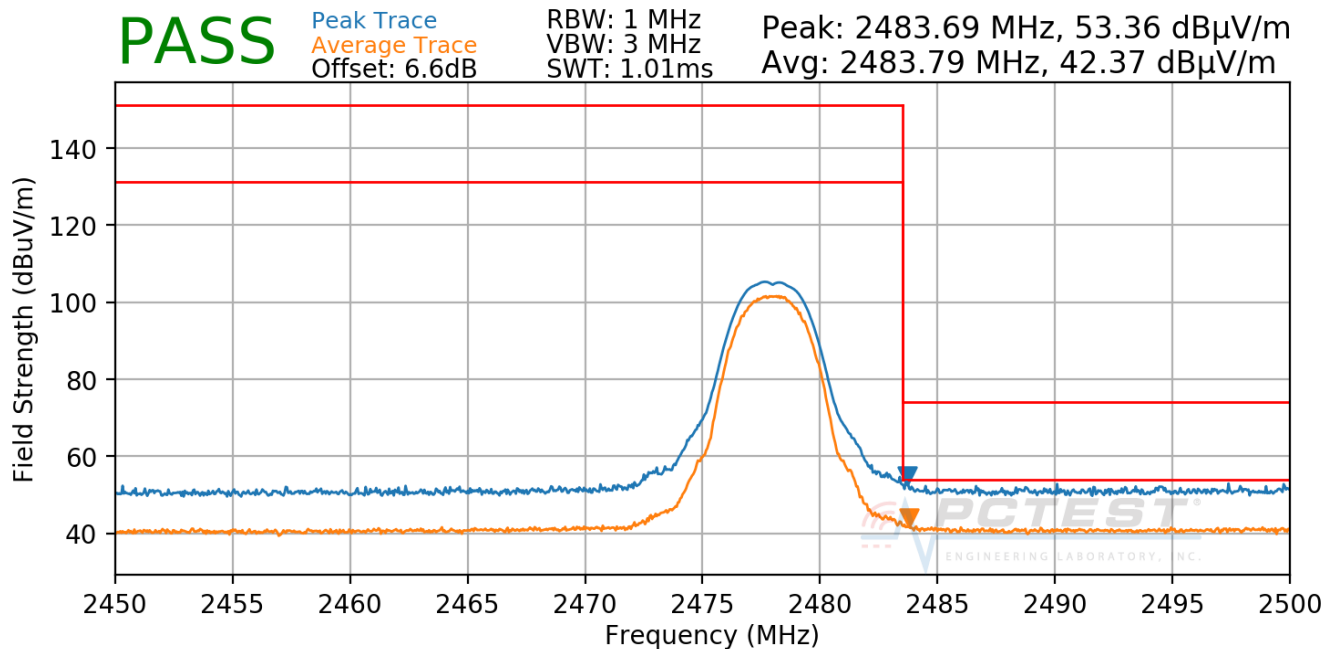
Plot 7-107. Radiated Restricted Upper Band Edge Measurement ANT0 (Average & Peak)
