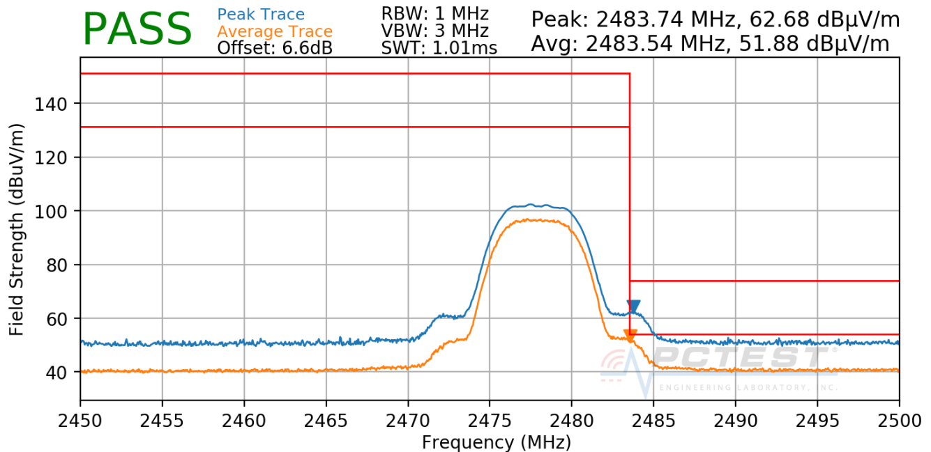
Plot 7-112. Radiated Restricted Upper Band Edge Measurement ANT1 (Average & Peak)
