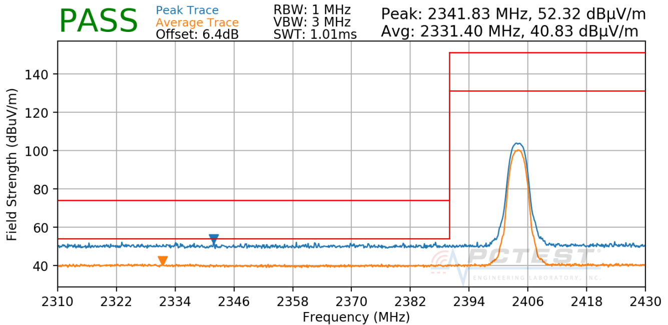
Plot 7-109. Radiated Restricted Lower Band Edge Measurement ANT1 (Average & Peak)
