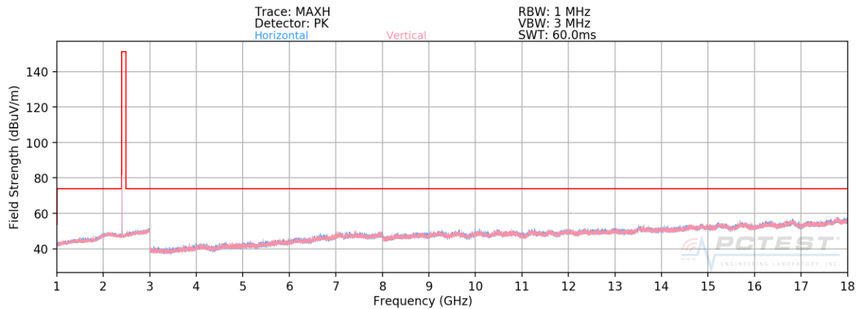
Plot 7-100. Radiated Spurious Plot Above 1GHz ANT2 (4Mbps, HDR4 ePA – Ch. 1, Ant. Pol. H & V)
