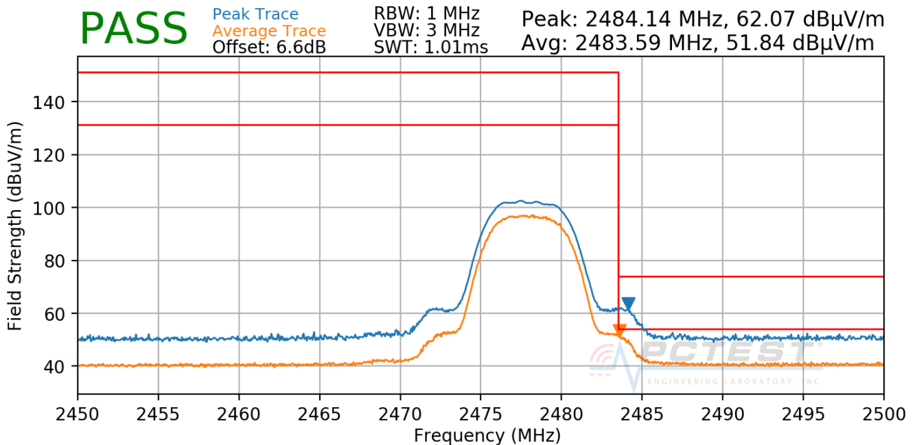
Plot 7-108. Radiated Restricted Upper Band Edge Measurement ANT0 (Average & Peak)
