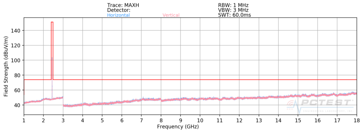
Plot 7-95. Radiated Spurious Plot Above 1GHz ANT1 (8Mbps, HDR8 ePA – Ch. 38, Ant. Pol. H & V)
