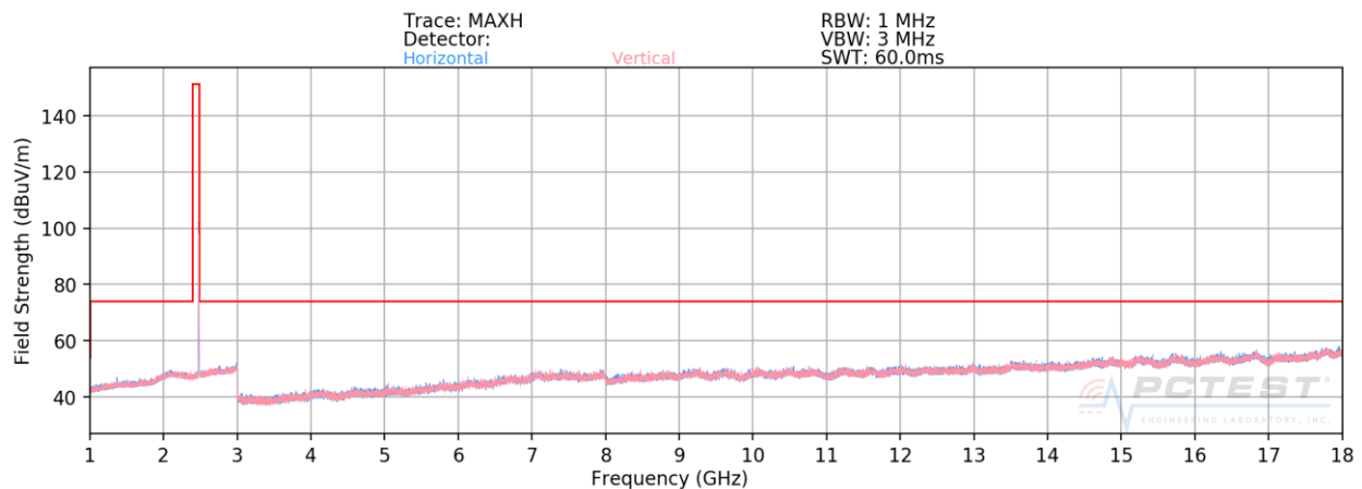
Plot 7-96. Radiated Spurious Plot Above 1GHz ANT1 (8Mbps, HDR8 ePA – Ch. 75, Ant. Pol. H & V)
