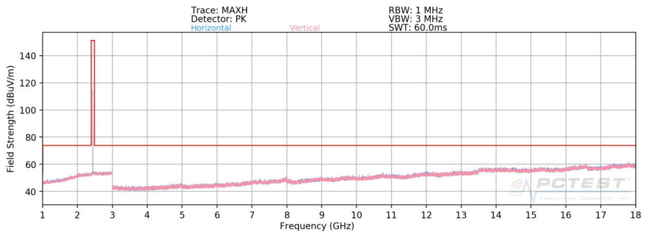
Plot 7-92. Radiated Spurious Plot Above 1GHz ANT1 (4Mbps, HDR4 ePA – Ch. 38, Ant. Pol. H & V)
