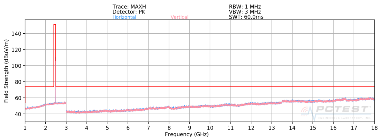
Plot 7-93. Radiated Spurious Plot Above 1GHz ANT1 (4Mbps, HDR4 ePA – Ch. 75, Ant. Pol. H & V)
