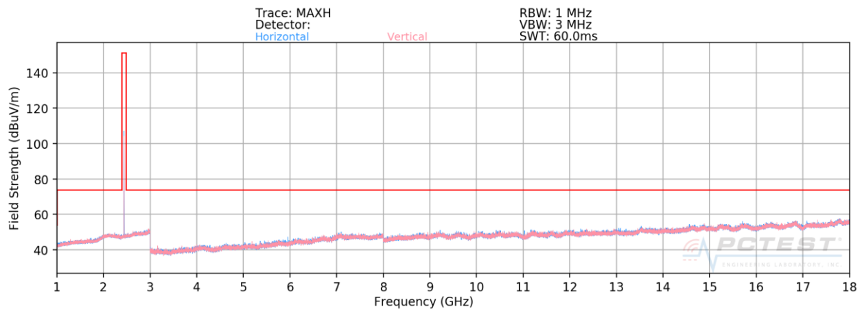
Plot 7-86. Radiated Spurious Plot Above 1GHz ANT0 (4Mbps, HDR4 ePA – Ch. 38, Ant. Pol. H & V)
