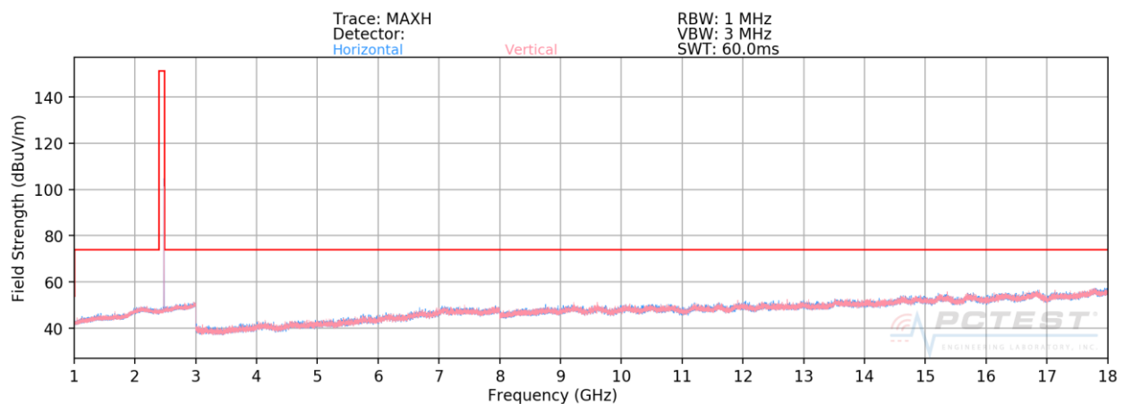
Plot 7-87. Radiated Spurious Plot Above 1GHz ANT0 (4Mbps, HDR4 ePA – Ch. 75, Ant. Pol. H & V)
