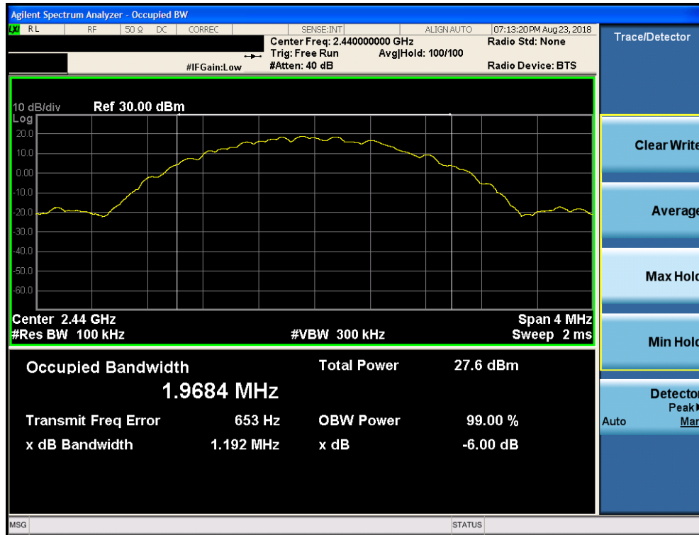
Plot 7-5. 6dB Bandwidth Plot ANT0 (Bluetooth (LE), 2Mbps, ePA – Ch. 19)
