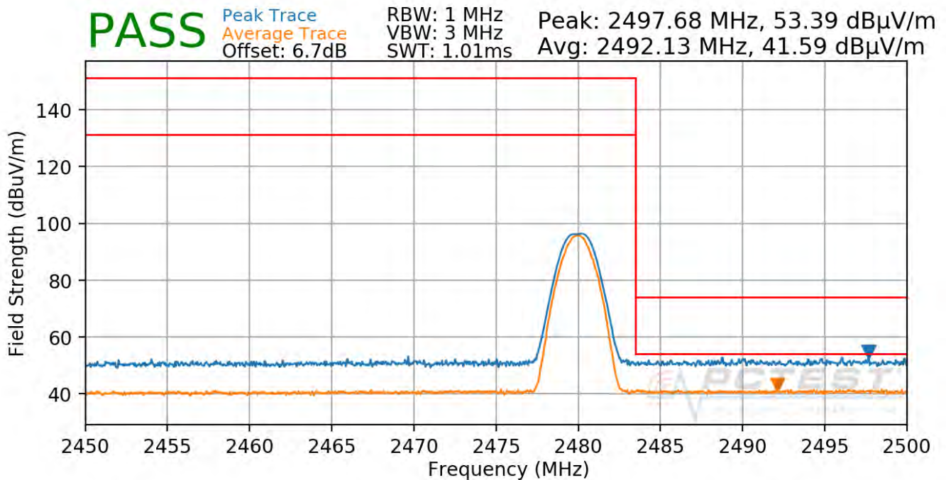
Plot 7-101. Radiated Restricted Upper Band Edge Measurement ANT2 (Average & Peak)
