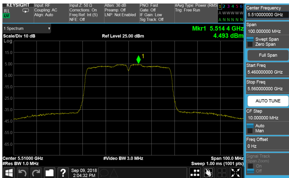
Plot 7-136. Power Spectral Density Plot CDD ANT2 (40MHz BW 802.11n (UNII Band 2C) – Ch. 102)
