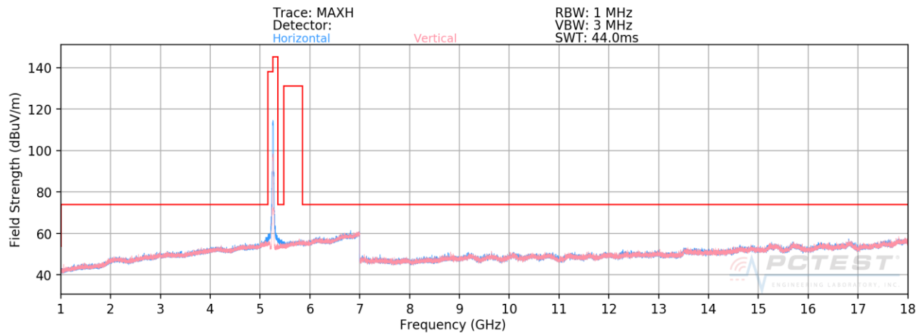
Plot 7-160. Radiated Spurious Plot above 1GHz SISO CORE0 (802.11n – U2A Ch. 52)
