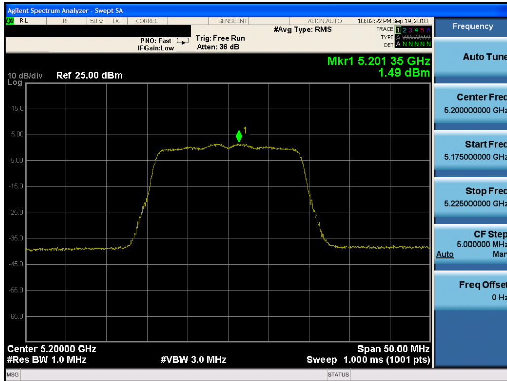
Plot 7-107. Power Spectral Density Plot CDD ANT1 (20MHz BW 802.11n (UNII Band 1) – Ch. 40)
