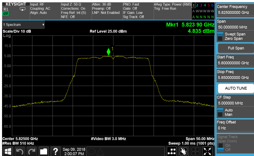
Plot 7-150. Power Spectral Density Plot CDD ANT2 (20MHz BW 802.11n (UNII Band 3) – Ch. 165)
