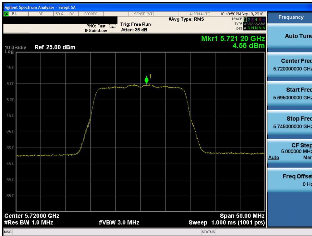
Plot 7-134. Power Spectral Density Plot CDD ANT2 (20MHz BW 802.11n (UNII Band 2C) – Ch. 144)
