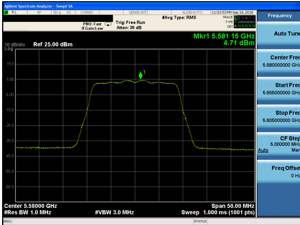
Plot 7-131. Power Spectral Density Plot CDD ANT1 (20MHz BW 802.11n (UNII Band 2C) – Ch. 116)
