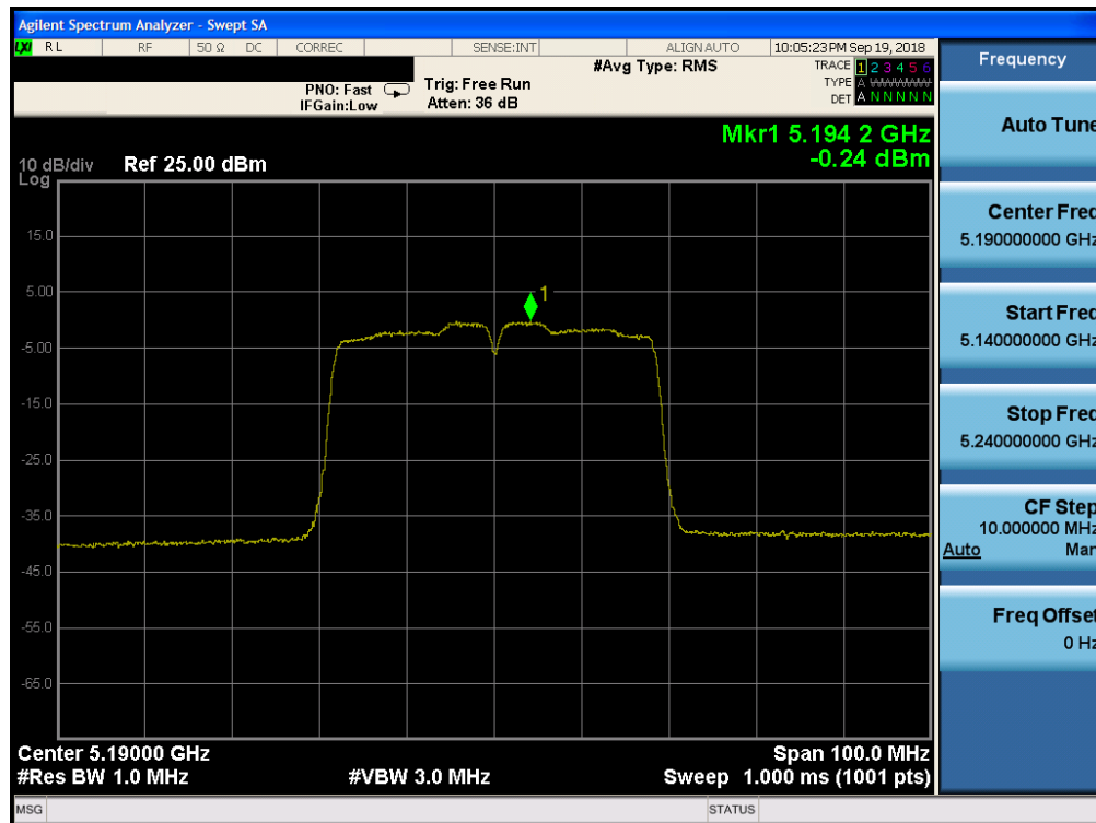
Plot 7-111. Power Spectral Density Plot CDD ANT1 (40MHz BW 802.11n (UNII Band 1) – Ch. 38)
