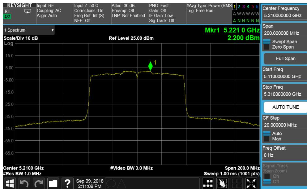
Plot 7-116. Power Spectral Density Plot CDD ANT2 (80MHz BW 802.11ac (UNII Band 1) – Ch. 42)
