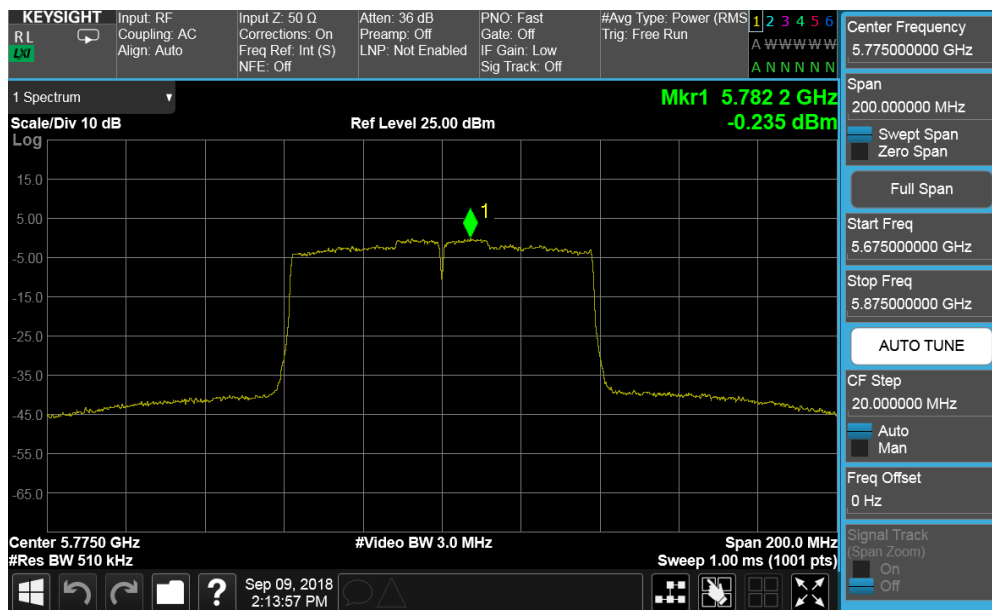
Plot 7-156. Power Spectral Density Plot CDD ANT2 (80MHz BW 802.11ac (UNII Band 3) – Ch. 155)
