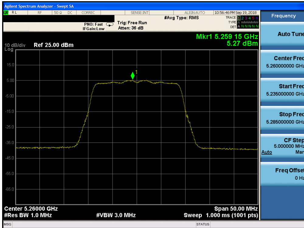
Plot 7-117. Power Spectral Density Plot CDD ANT1 (20MHz BW 802.11n (UNII Band 2A) – Ch. 52)
