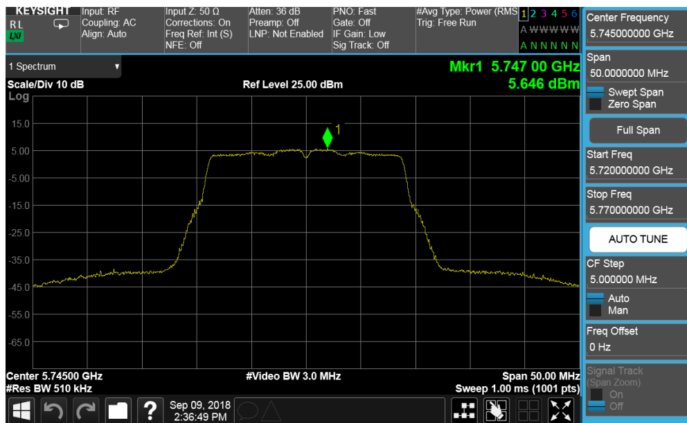
Plot 7-145. Power Spectral Density Plot CDD ANT1 (20MHz BW 802.11n (UNII Band 3) – Ch. 149)
