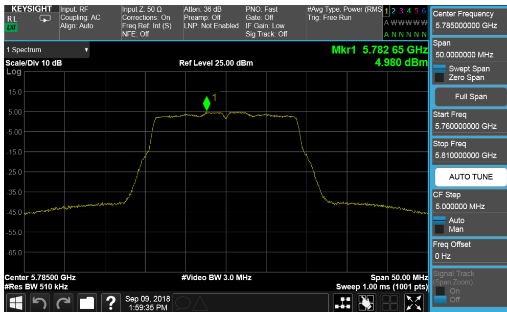
Plot 7-148. Power Spectral Density Plot CDD ANT2 (20MHz BW 802.11n (UNII Band 3) – Ch. 157)
