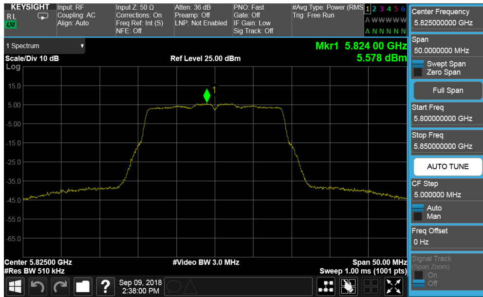
Plot 7-149. Power Spectral Density Plot CDD ANT1 (20MHz BW 802.11n (UNII Band 3) – Ch. 165)
