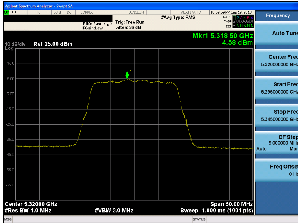
Plot 7-121. Power Spectral Density Plot CDD ANT1 (20MHz BW 802.11n (UNII Band 2A) – Ch. 64)
