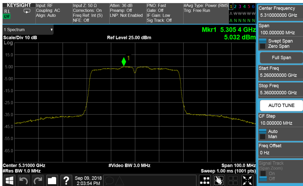
Plot 7-126. Power Spectral Density Plot CDD ANT2 (40MHz BW 802.11n (UNII Band 2A) – Ch. 62)
