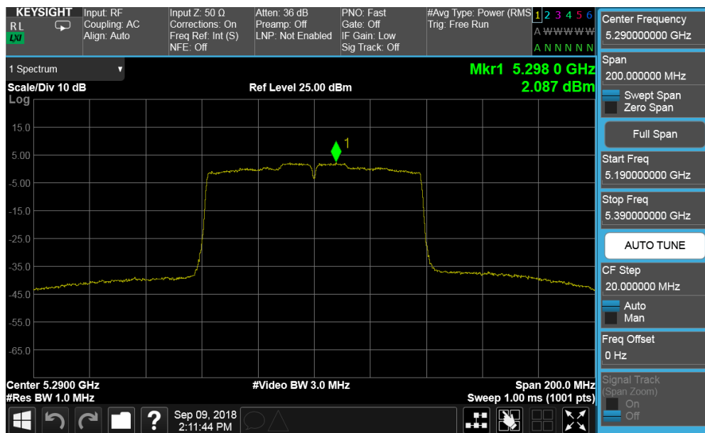
Plot 7-128. Power Spectral Density Plot CDD ANT2 (80MHz BW 802.11ac (UNII Band 2A) – Ch. 58)
