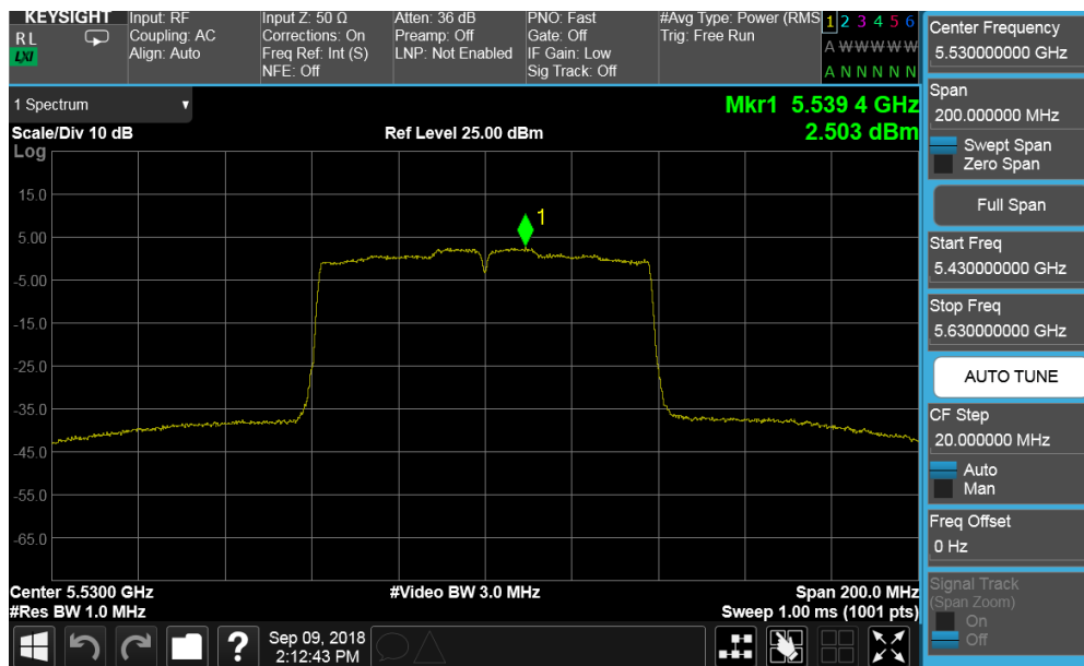
Plot 7-142. Power Spectral Density Plot CDD ANT2 (80MHz BW 802.11ac (UNII Band 2C) – Ch. 106)
