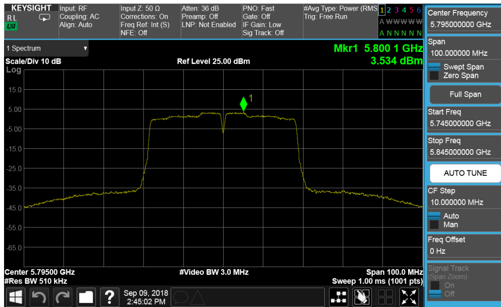
Plot 7-153. Power Spectral Density Plot CDD ANT1 (40MHz BW 802.11n (UNII Band 3) – Ch. 159)
