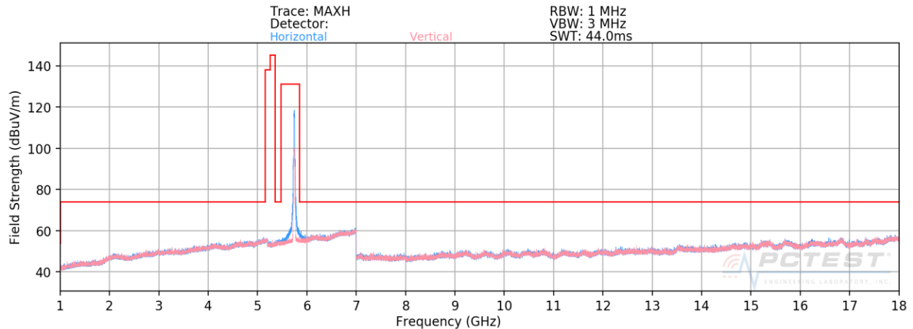
Plot 7-166. Radiated Spurious Plot above 1GHz SISO CORE0 (802.11n - U3 Ch. 149)
