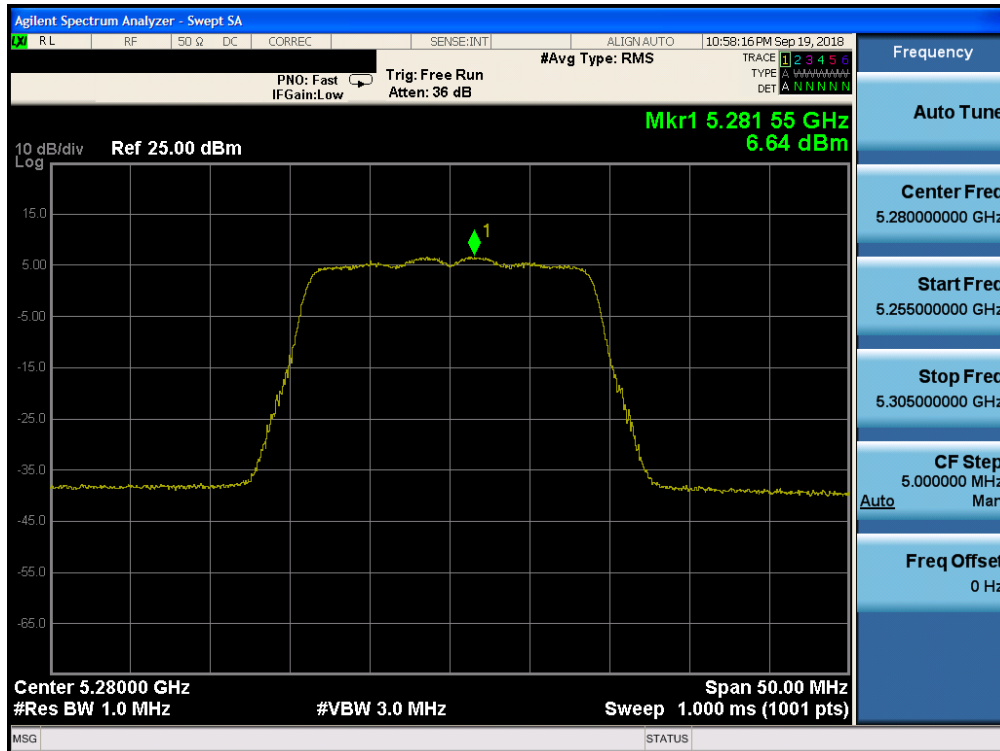
Plot 7-119. Power Spectral Density Plot CDD ANT1 (20MHz BW 802.11n (UNII Band 2A) – Ch. 56)
