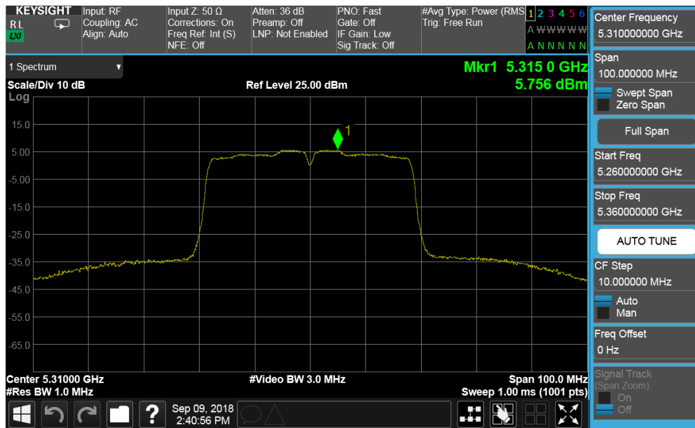
Plot 7-125. Power Spectral Density Plot CDD ANT1 (40MHz BW 802.11n (UNII Band 2A) – Ch. 62)
