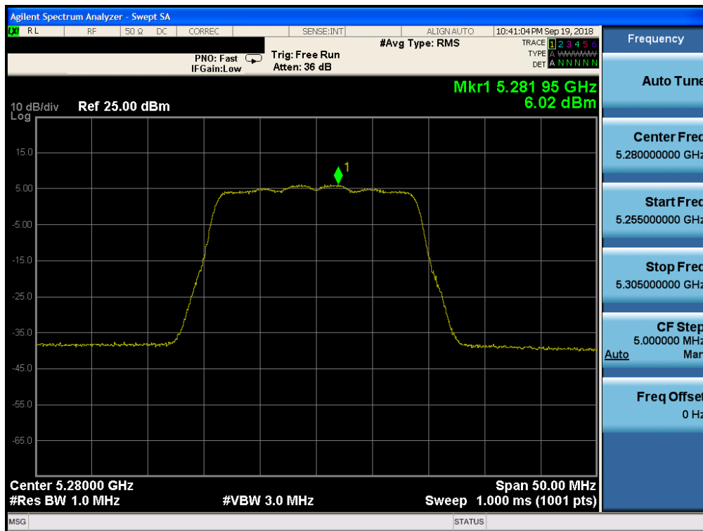
Plot 7-120. Power Spectral Density Plot CDD ANT2 (20MHz BW 802.11n (UNII Band 2A) – Ch. 56)
