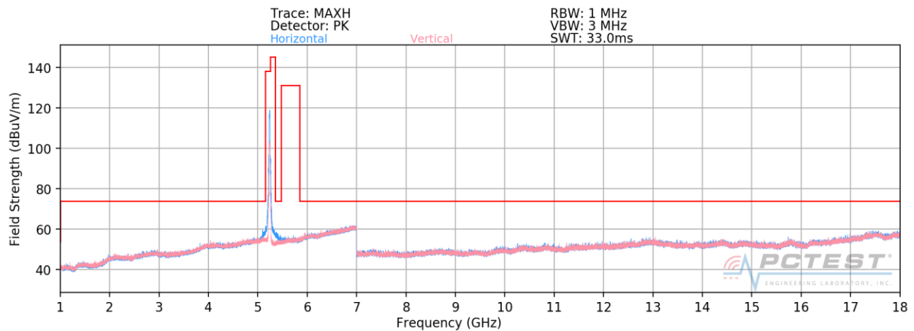
Plot 7-183. Radiated Spurious Plot above 1GHz CDD (802.11n – U1 Ch. 48)
