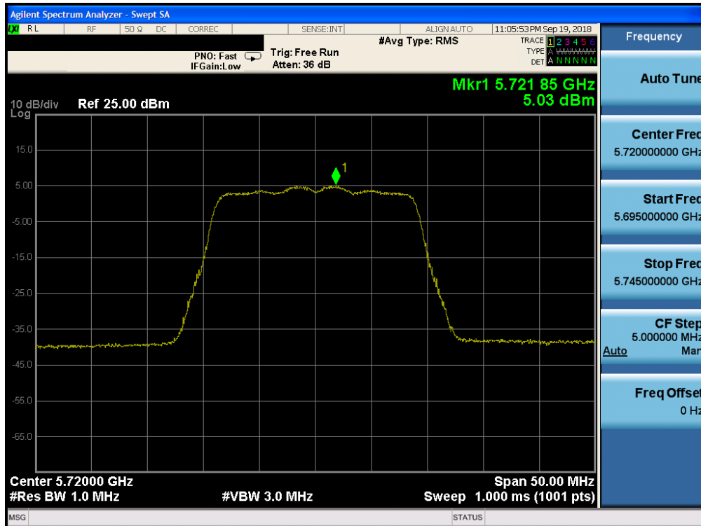
Plot 7-133. Power Spectral Density Plot CDD ANT1 (20MHz BW 802.11n (UNII Band 2C) – Ch. 144)
