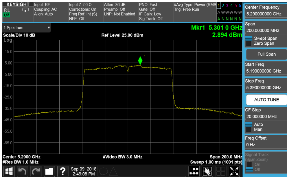
Plot 7-127. Power Spectral Density Plot CDD ANT1 (80MHz BW 802.11ac (UNII Band 2A) – Ch. 58)
