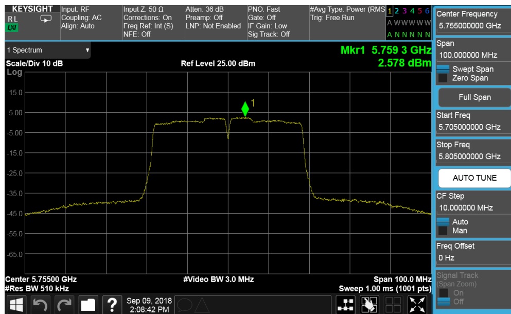
Plot 7-152. Power Spectral Density Plot CDD ANT2 (40MHz BW 802.11n (UNII Band 3) – Ch. 151)
