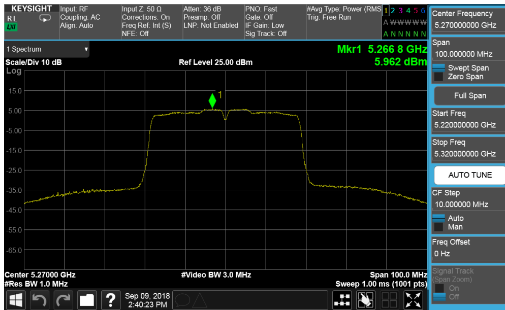
Plot 7-123. Power Spectral Density Plot CDD ANT1 (40MHz BW 802.11n (UNII Band 2A) – Ch. 54)
