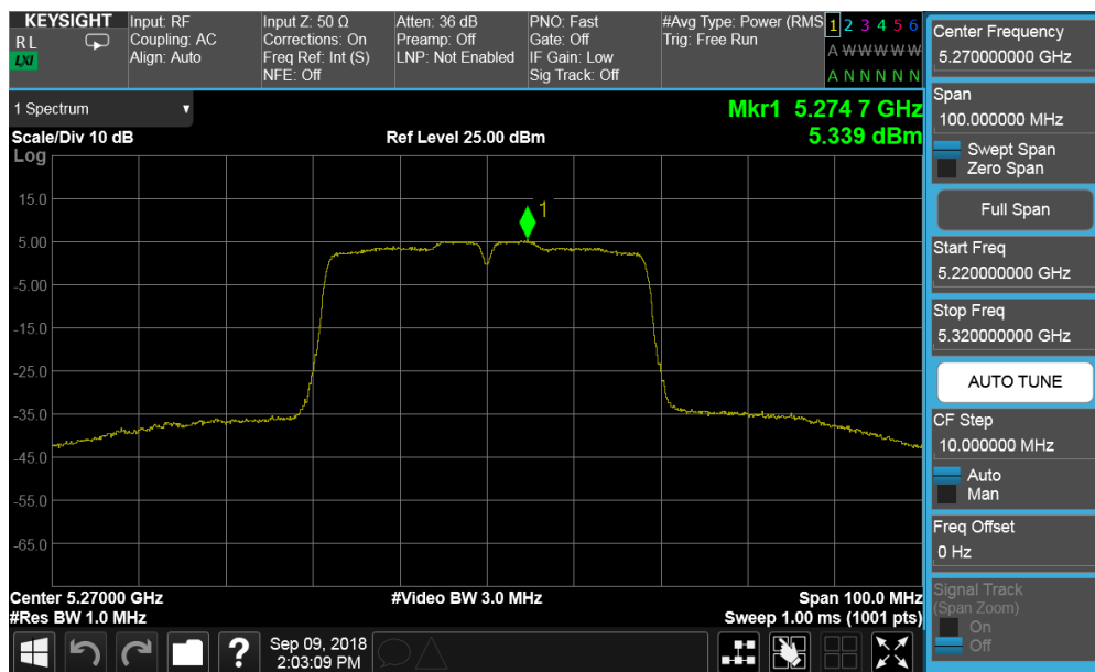
Plot 7-124. Power Spectral Density Plot CDD ANT2 (40MHz BW 802.11n (UNII Band 2A) – Ch. 54)
