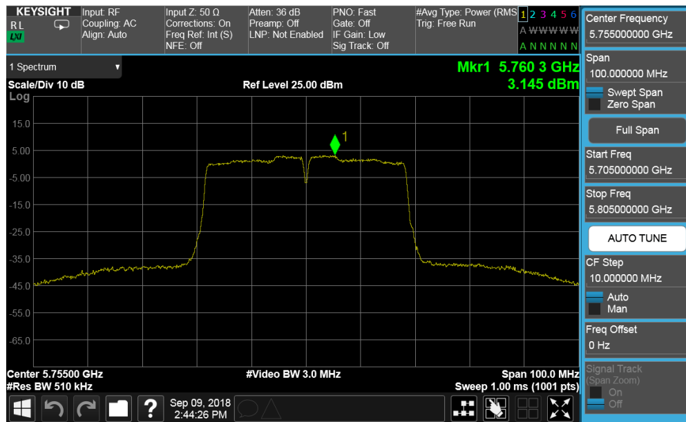
Plot 7-151. Power Spectral Density Plot CDD ANT1 (40MHz BW 802.11n (UNII Band 3) – Ch. 151)
