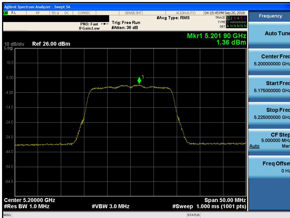
Plot 7-108. Power Spectral Density Plot CDD ANT2 (20MHz BW 802.11n (UNII Band 1) – Ch. 40)
