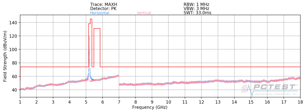
Plot 7-182. Radiated Spurious Plot above 1GHz CDD (802.11n – U1 Ch. 40)
