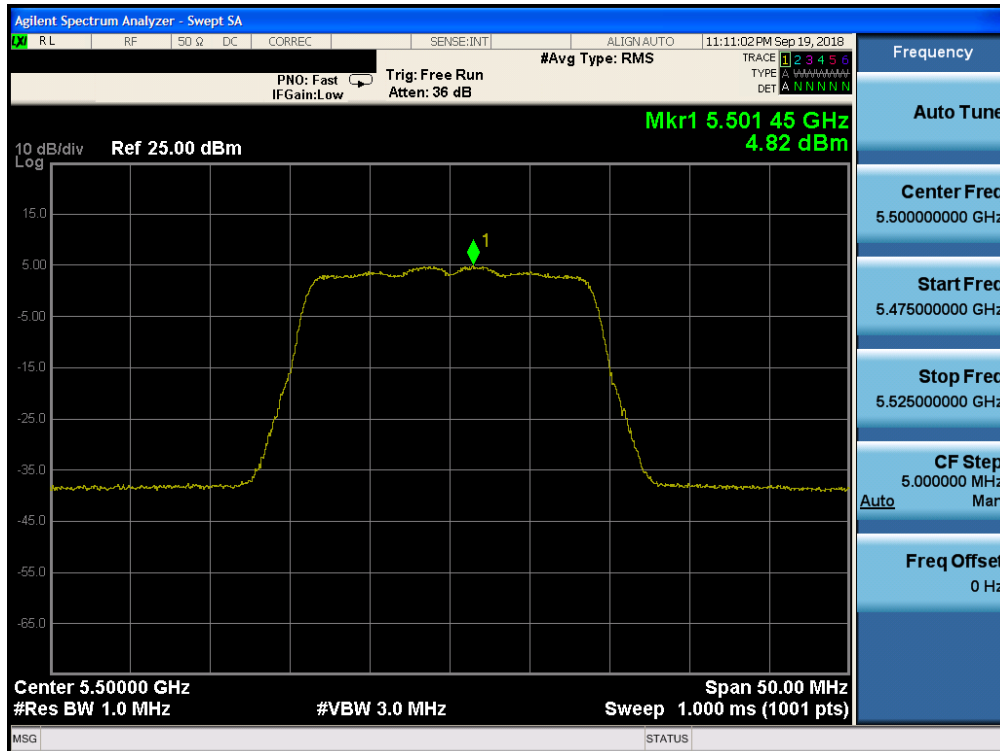
Plot 7-129. Power Spectral Density Plot CDD ANT1 (20MHz BW 802.11n (UNII Band 2C) – Ch. 100)
