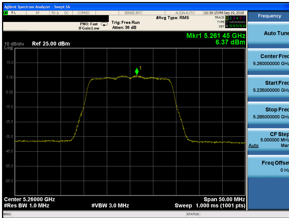
Plot 7-118. Power Spectral Density Plot CDD ANT2 (20MHz BW 802.11n (UNII Band 2A) – Ch. 52)
