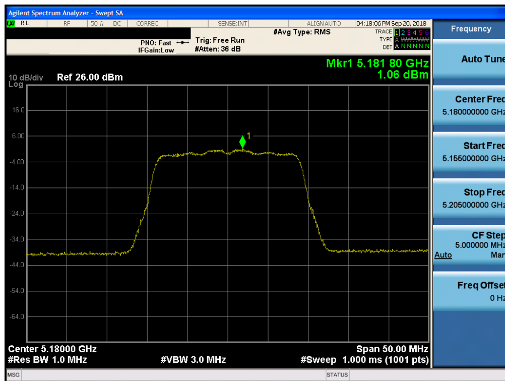
Plot 7-106. Power Spectral Density Plot CDD ANT2 (20MHz BW 802.11n (UNII Band 1) – Ch. 36)
