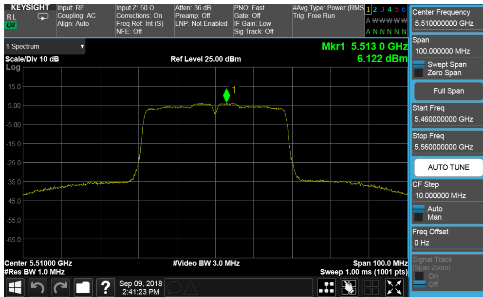
Plot 7-135. Power Spectral Density Plot CDD ANT1 (40MHz BW 802.11n (UNII Band 2C) – Ch. 102)
