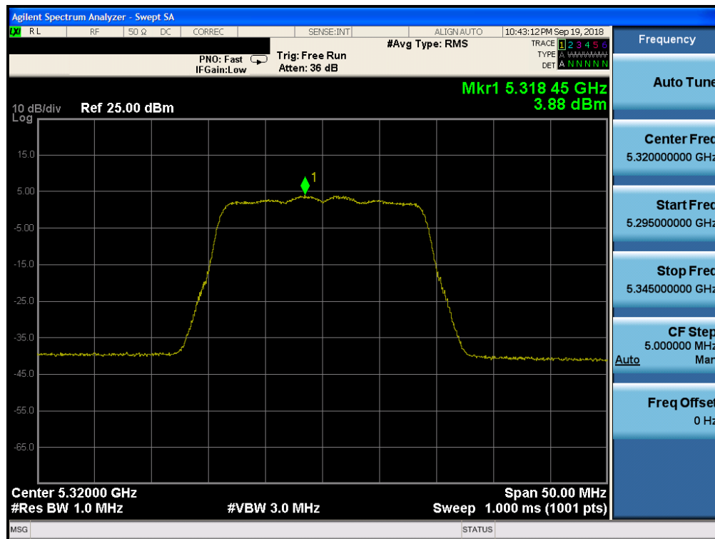
Plot 7-122. Power Spectral Density Plot CDD ANT2 (20MHz BW 802.11n (UNII Band 2A) – Ch. 64)
