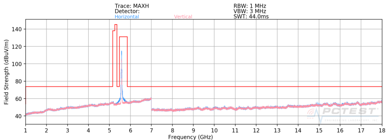
Plot 7-176. Radiated Spurious Plot above 1GHz SISO CORE1 (802.11n – U2C Ch. 120)
