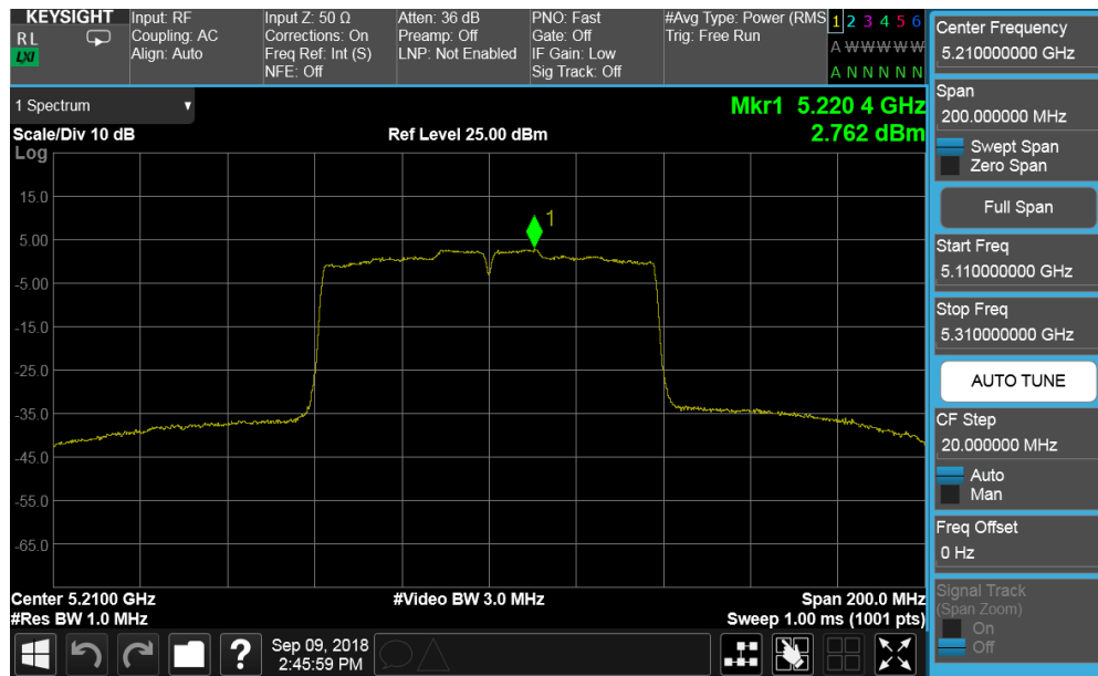
Plot 7-115. Power Spectral Density Plot CDD ANT1 (80MHz BW 802.11ac (UNII Band 1) – Ch. 42)
