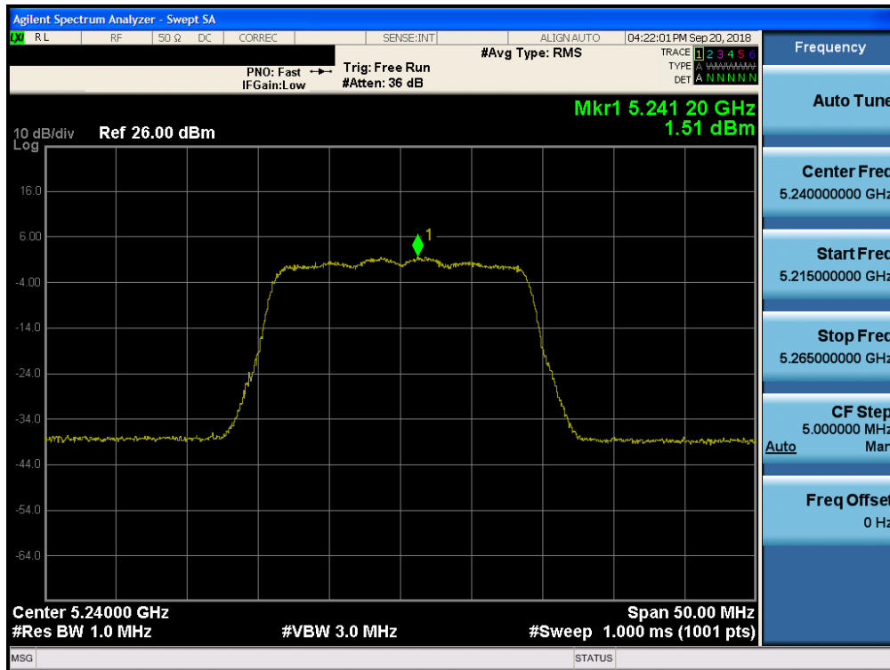
Plot 7-110. Power Spectral Density Plot CDD ANT2 (20MHz BW 802.11n (UNII Band 1) – Ch. 48)
