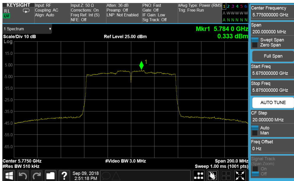
Plot 7-155. Power Spectral Density Plot CDD ANT1 (80MHz BW 802.11ac (UNII Band 3) – Ch. 155)
