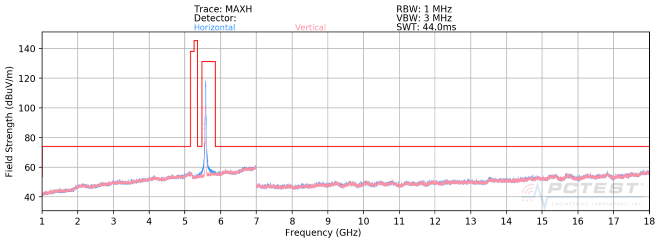
Plot 7-164. Radiated Spurious Plot above 1GHz SISO CORE0 (802.11n – U2C Ch. 120)
