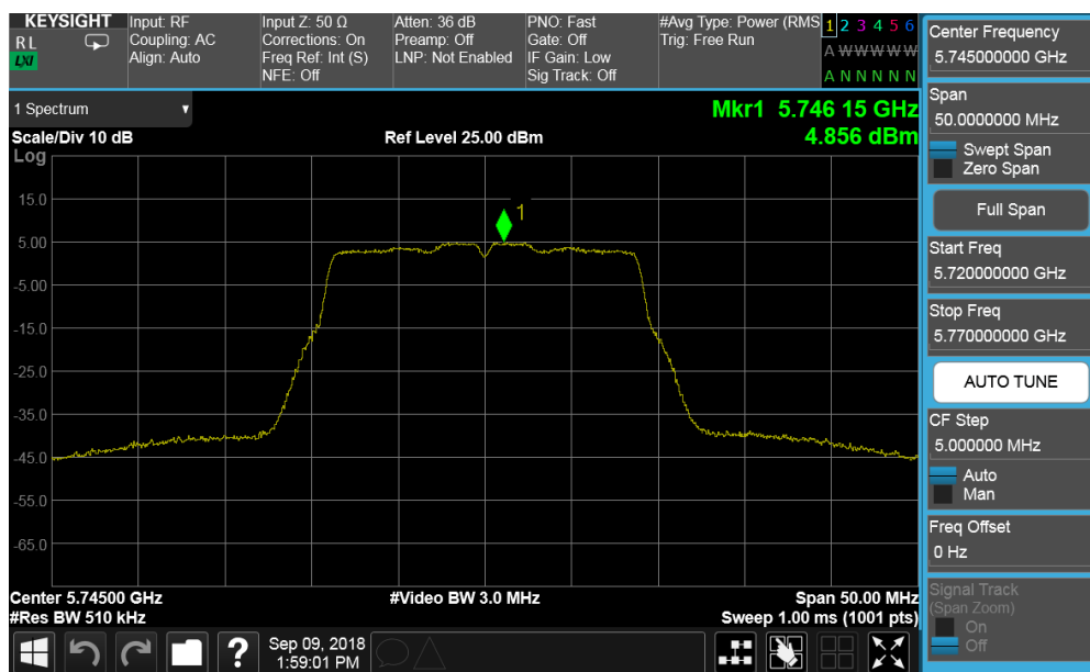
Plot 7-146. Power Spectral Density Plot CDD ANT2 (20MHz BW 802.11n (UNII Band 3) – Ch. 149)
