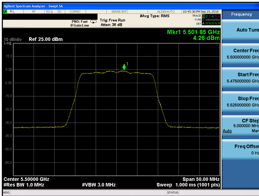
Plot 7-130. Power Spectral Density Plot CDD ANT2 (20MHz BW 802.11n (UNII Band 2C) – Ch. 100)
