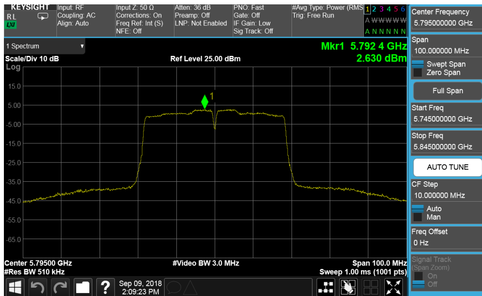
Plot 7-154. Power Spectral Density Plot CDD ANT2 (40MHz BW 802.11n (UNII Band 3) – Ch. 159)
