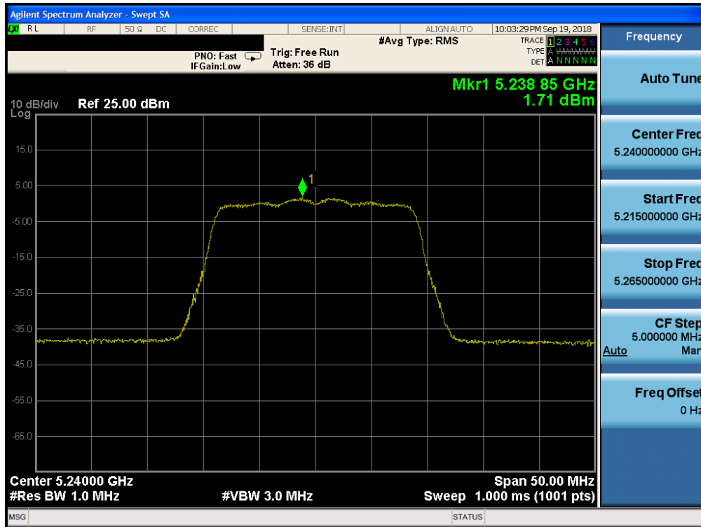
Plot 7-109. Power Spectral Density Plot CDD ANT1 (20MHz BW 802.11n (UNII Band 1) – Ch. 48)
