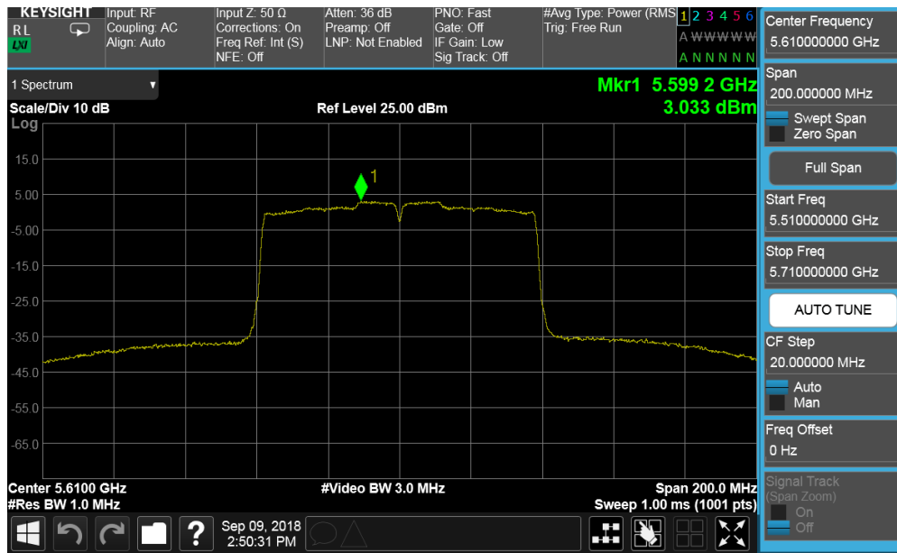
Plot 7-143. Power Spectral Density Plot CDD ANT1 (80MHz BW 802.11ac (UNII Band 2C) – Ch. 122)
