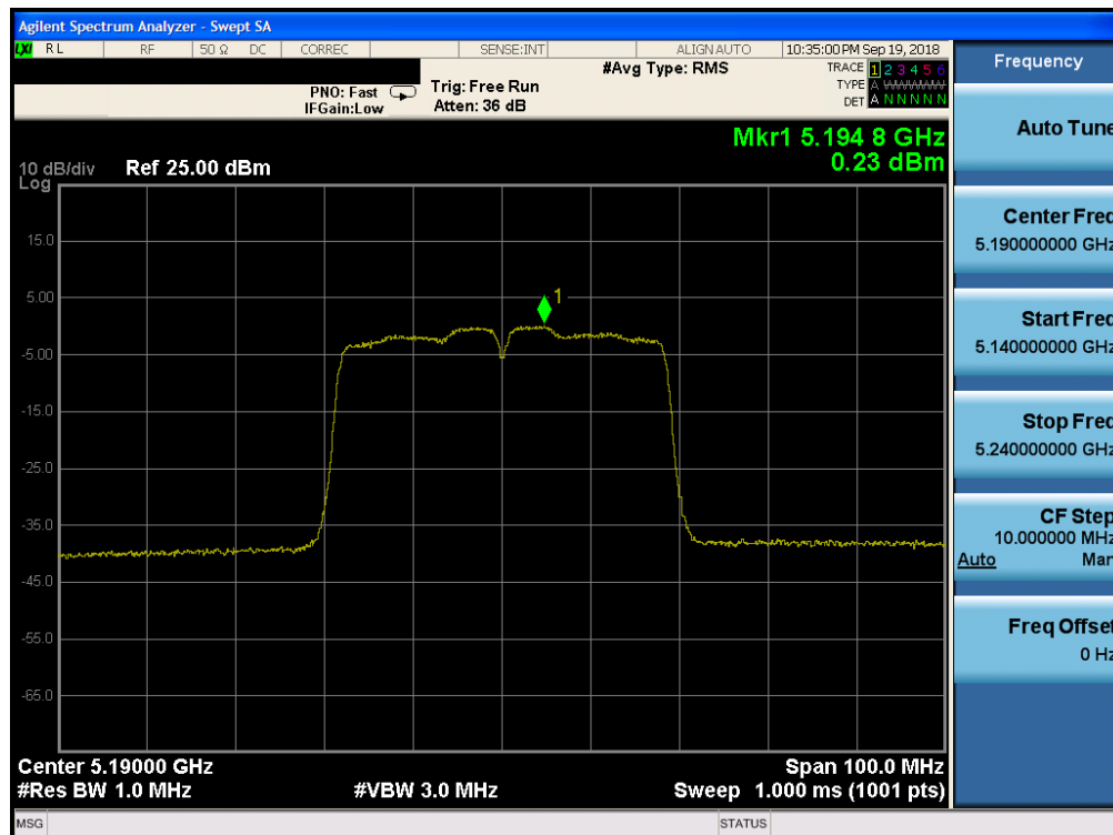
Plot 7-112. Power Spectral Density Plot CDD ANT2 (40MHz BW 802.11n (UNII Band 1) – Ch. 38)
