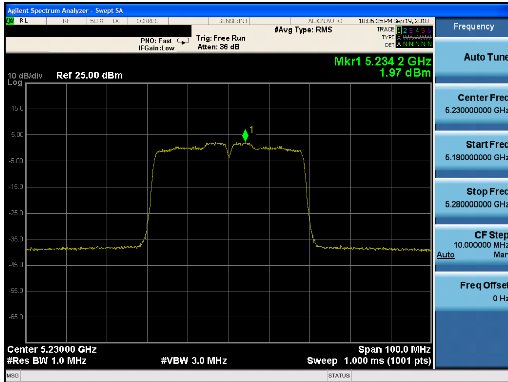
Plot 7-113. Power Spectral Density Plot CDD ANT1 (40MHz BW 802.11n (UNII Band 1) – Ch. 46)
