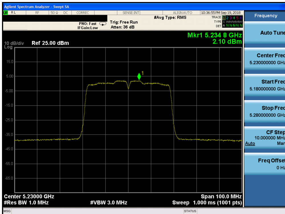
Plot 7-114. Power Spectral Density Plot CDD ANT2 (40MHz BW 802.11n (UNII Band 1) – Ch. 46)
