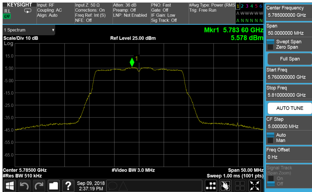
Plot 7-147. Power Spectral Density Plot CDD ANT1 (20MHz BW 802.11n (UNII Band 3) – Ch. 157)
