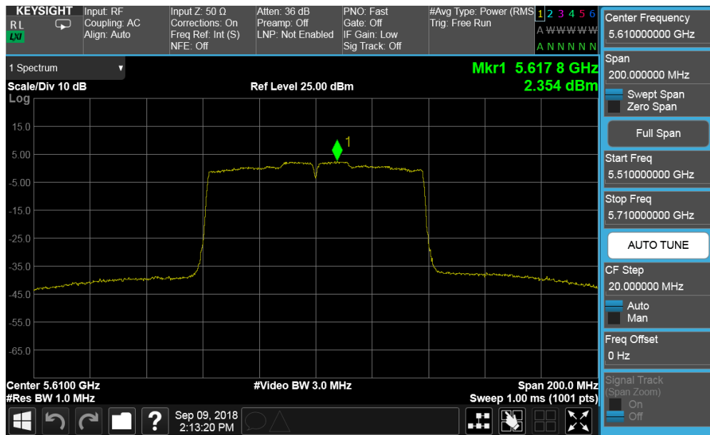
Plot 7-144. Power Spectral Density Plot CDD ANT2 (80MHz BW 802.11ac (UNII Band 2C) – Ch. 122)
