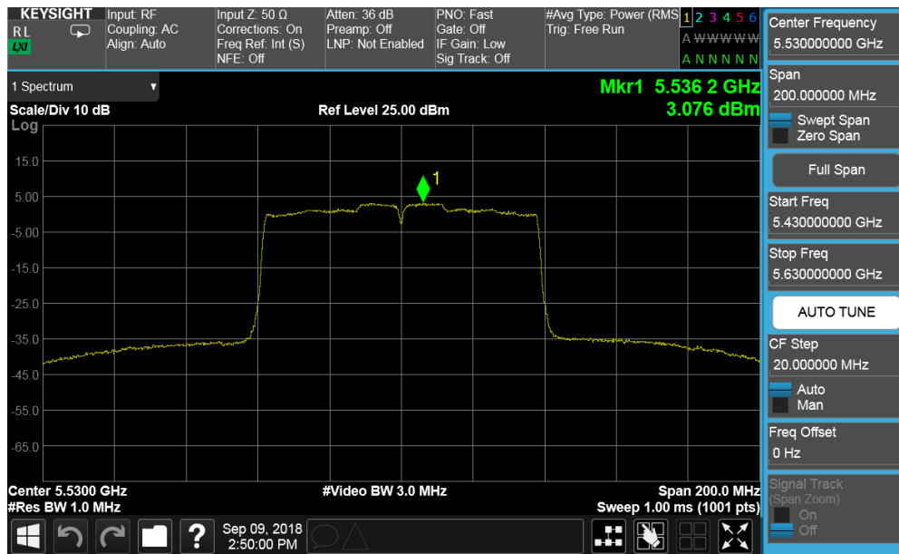
Plot 7-141. Power Spectral Density Plot CDD ANT1 (80MHz BW 802.11ac (UNII Band 2C) – Ch. 106)
