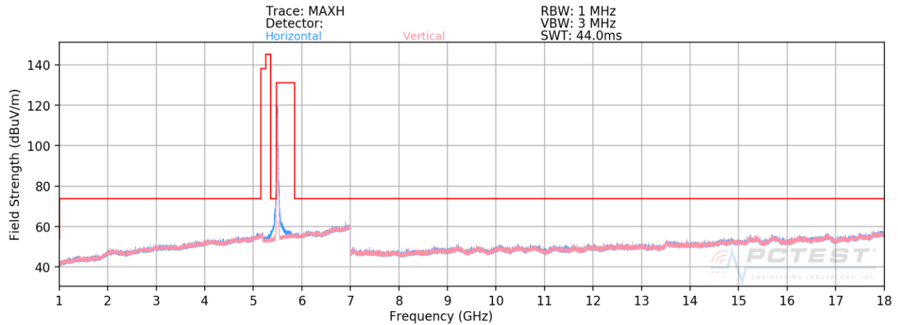
Plot 7-163. Radiated Spurious Plot above 1GHz SISO CORE0 (802.11n – U2C Ch. 100)
