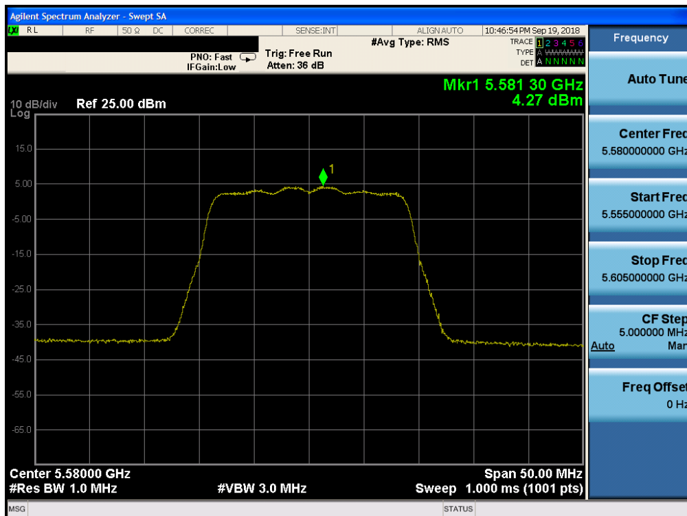
Plot 7-132. Power Spectral Density Plot CDD ANT2 (20MHz BW 802.11n (UNII Band 2C) – Ch. 116)
