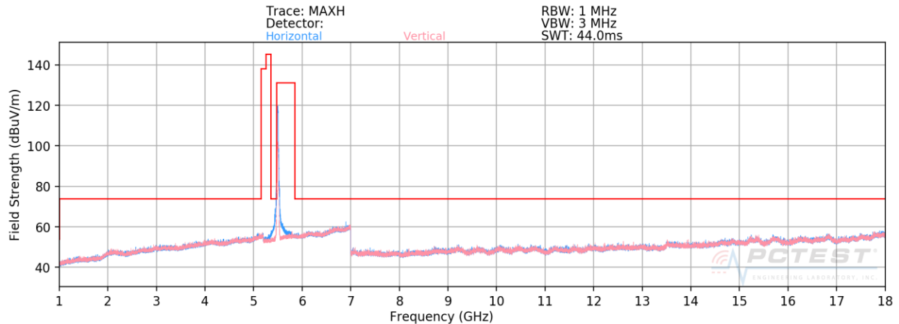
Plot 7-175. Radiated Spurious Plot above 1GHz SISO CORE1 (802.11n – U2C Ch. 100)
