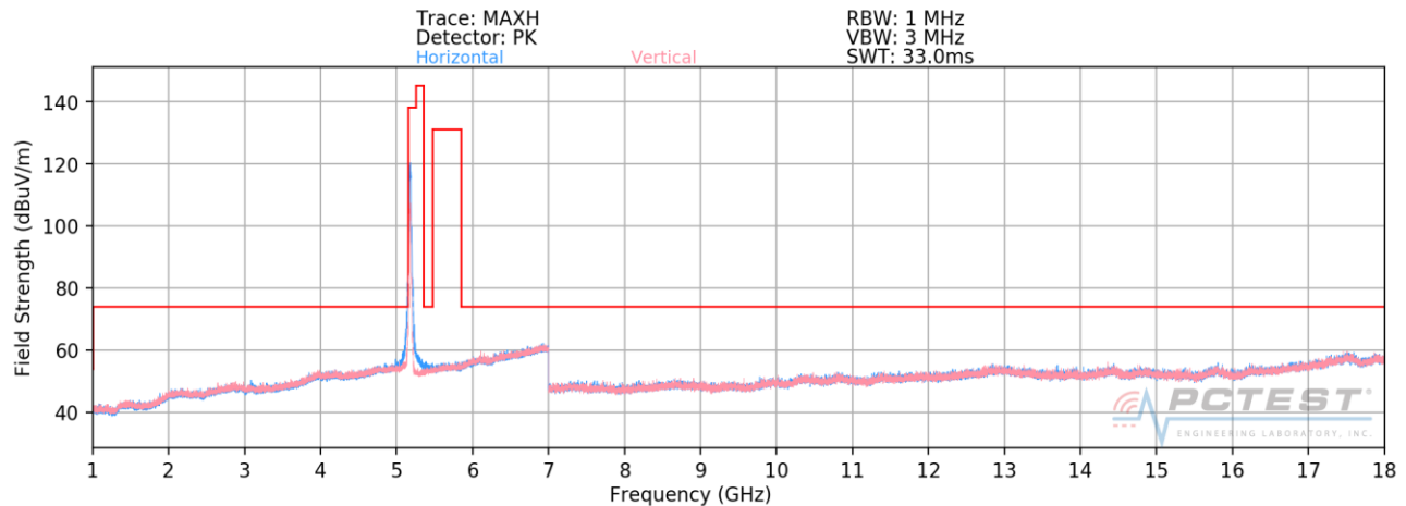
Plot 7-181. Radiated Spurious Plot above 1GHz CDD (802.11n – U1 Ch. 36)
