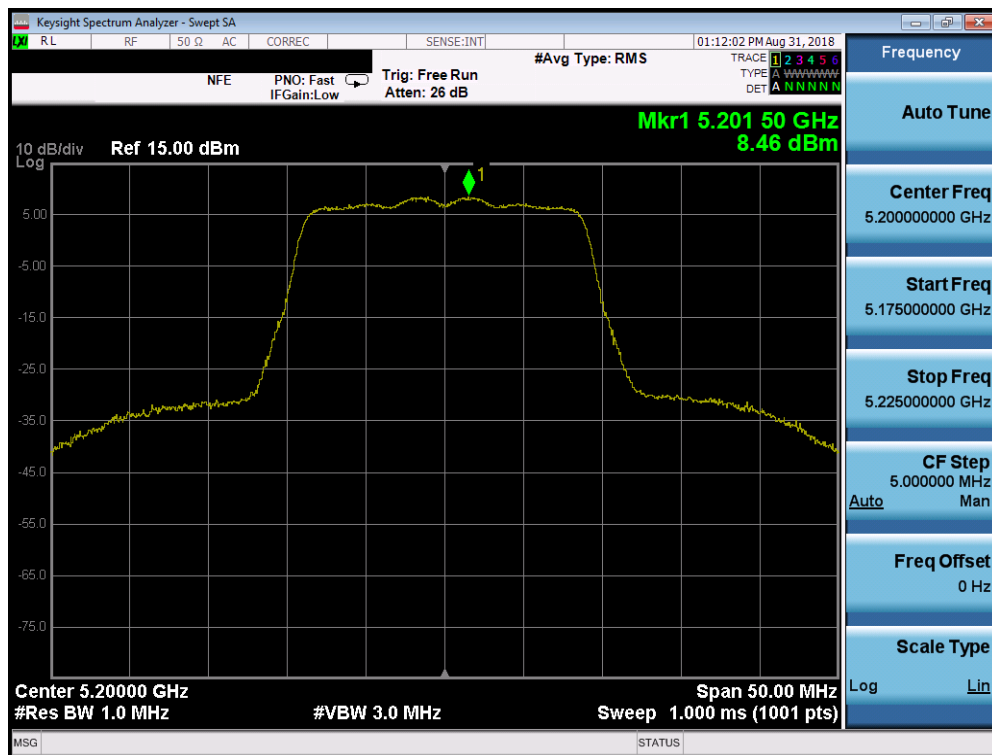
Plot 7-54. Power Spectral Density Plot SISO CORE0 (20MHz BW 802.11n (UNII Band 1) – Ch. 40)
