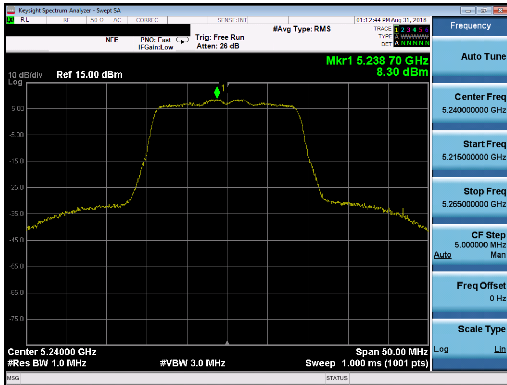
Plot 7-55. Power Spectral Density Plot SISO CORE0 (20MHz BW 802.11n (UNII Band 1) – Ch. 48)
