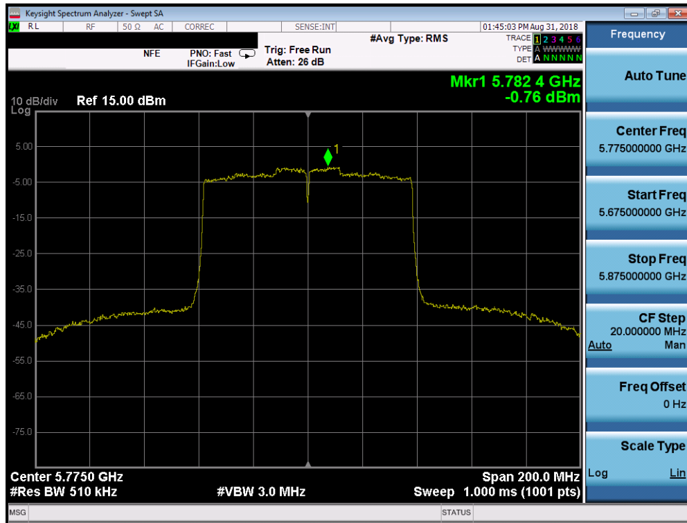
Plot 7-104. Power Spectral Density Plot SISO CORE1 (80MHz BW 802.11ac (UNII Band 3) – Ch. 155)
