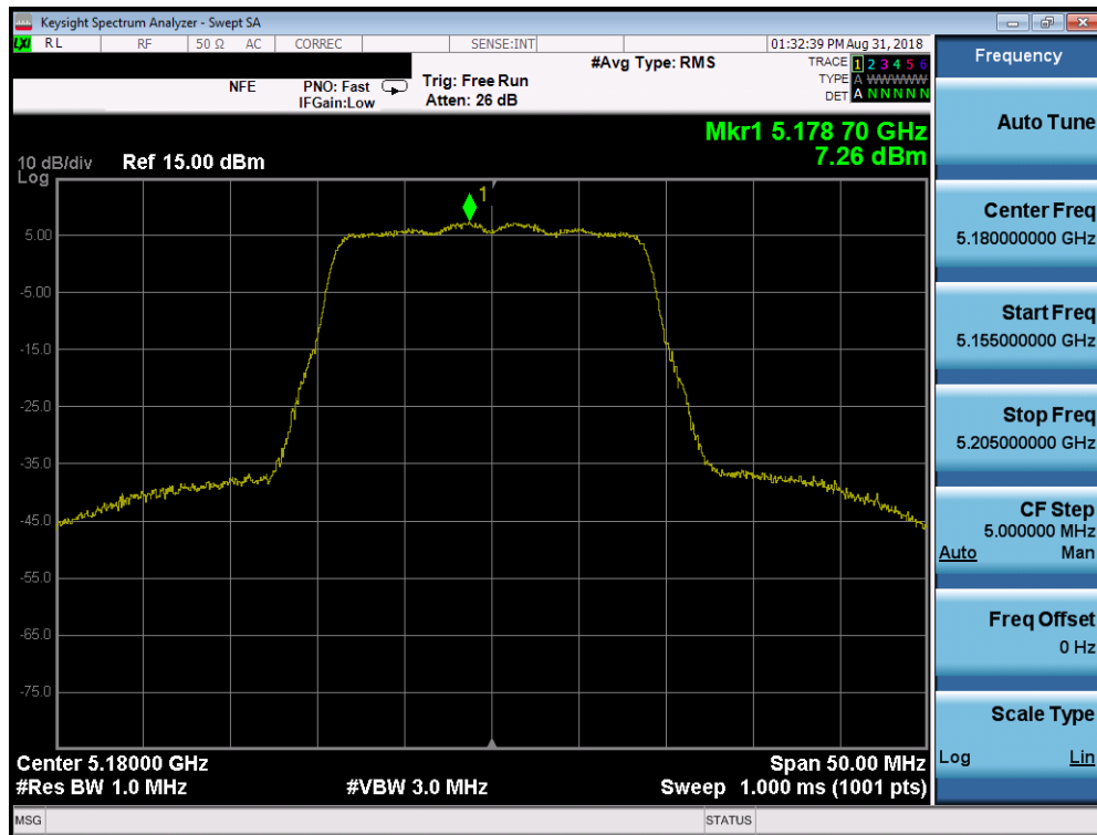
Plot 7-79. Power Spectral Density Plot SISO CORE1 (20MHz BW 802.11n (UNII Band 1) – Ch. 36)
