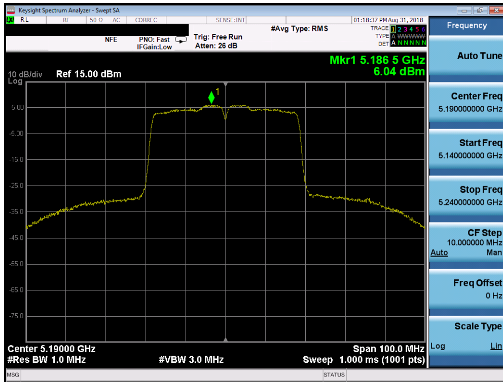
Plot 7-56. Power Spectral Density Plot SISO CORE0 (40MHz BW 802.11n (UNII Band 1) – Ch. 38)
