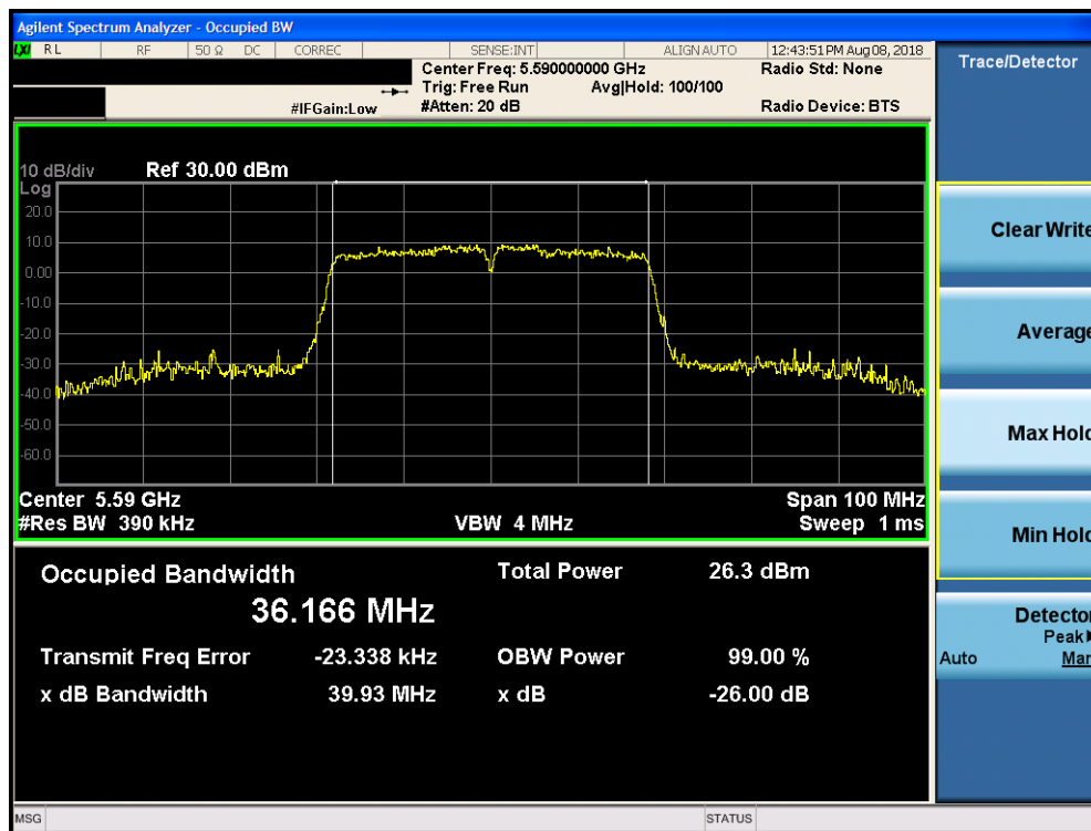
Plot 7-37. 26dB Bandwidth Plot SISO CORE1 (40MHz BW 802.11n (UNII Band 2C) – Ch. 118)
