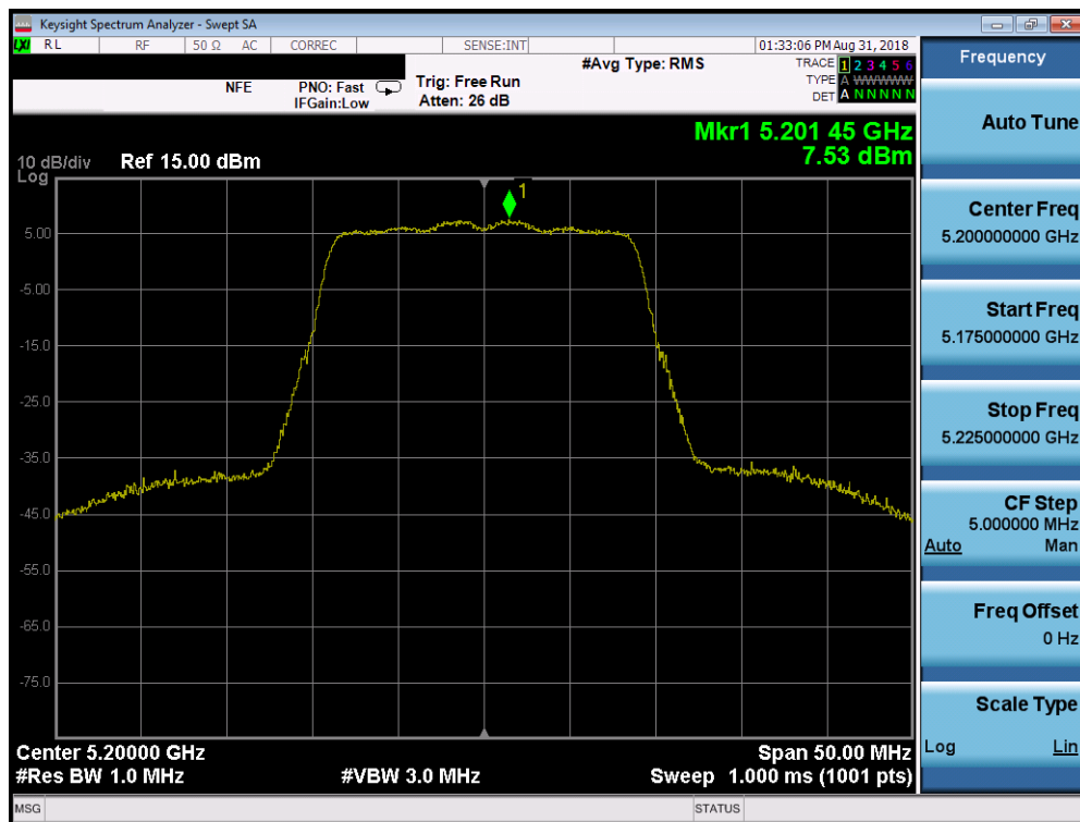
Plot 7-80. Power Spectral Density Plot SISO CORE1 (20MHz BW 802.11n (UNII Band 1) – Ch. 40)
