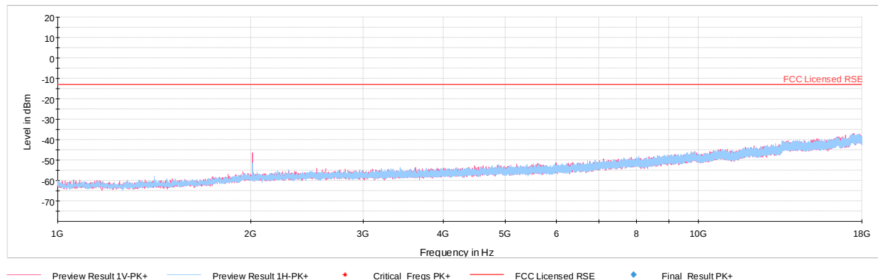
Plot 7-444. Radiated Spurious Plot above 1GHz (Band 71)
