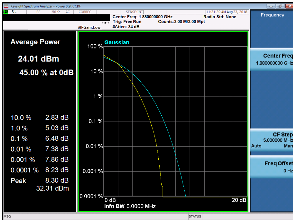
Plot 7-391. PAR Plot (Band 2 – 5.0MHz 16-QAM – RB Size 25)
