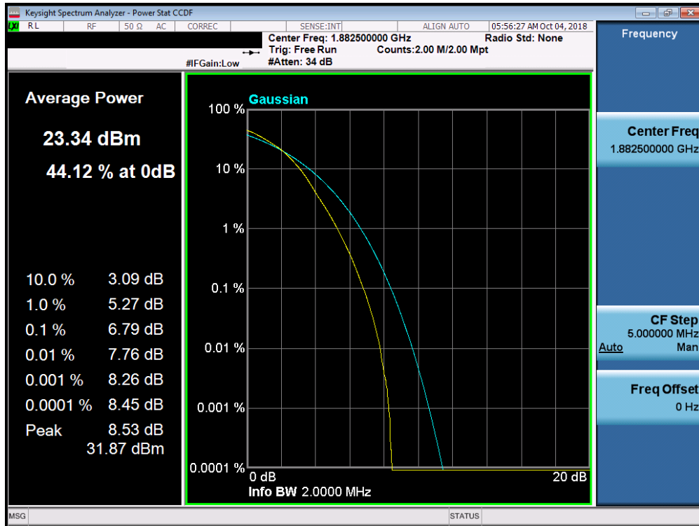
Plot 7-404. PAR Plot (Band 25 – 1.4MHz 64-QAM – RB Size 6)
