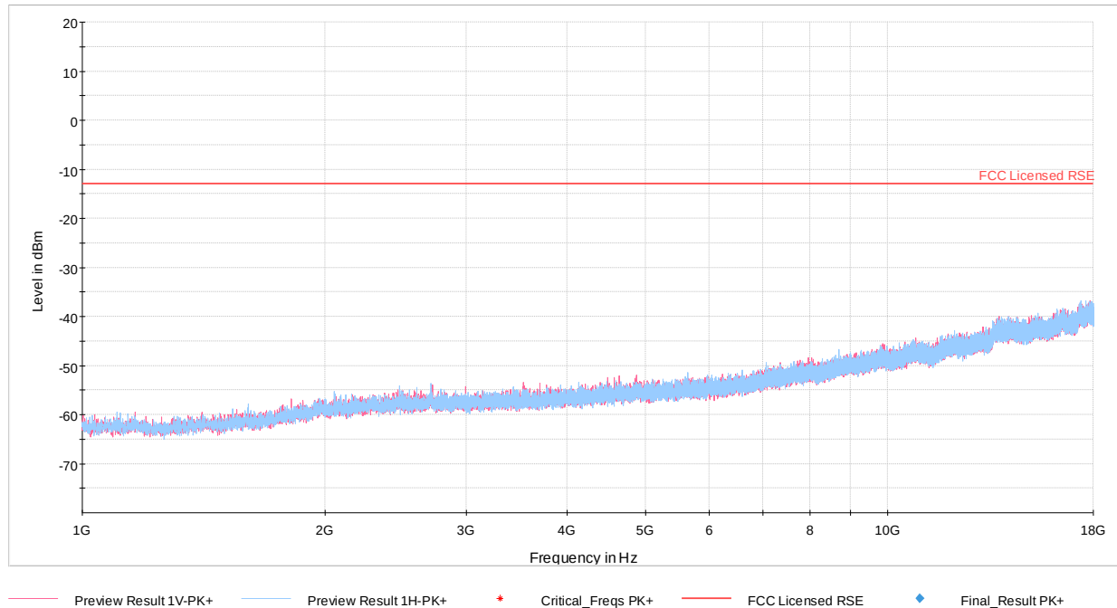
Plot 7-51. Radiated Spurious Plot above 1GHz (Band 26)
