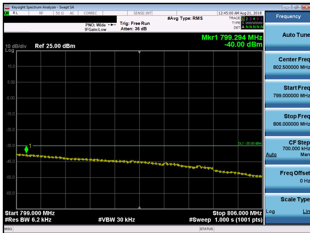
Plot 7-48. Upper Emission Mask Plot (LTE Band 14, 10MHz QPSK – RB Size 50)
