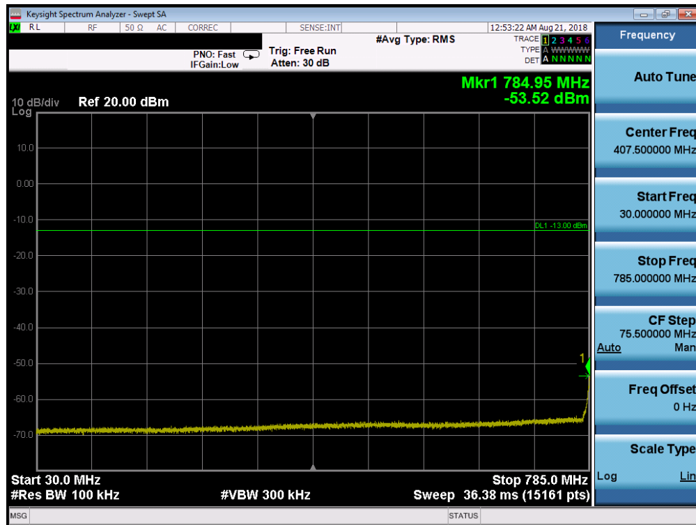
Plot 7-31. Conducted Spurious Plot (LTE Band 14, 5 MHz QPSK – RB Size 1, RB Offset 0 – High Channel)
