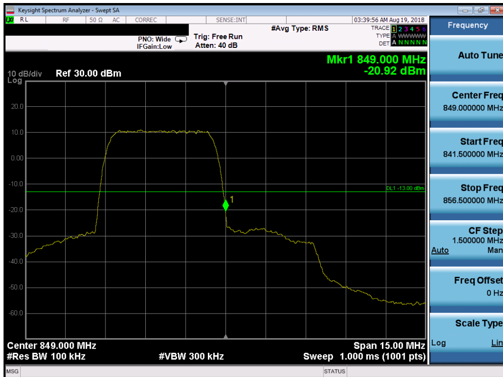
Plot 7-58. Band Edge Plot (Cellular WCDMA Mode - High Channel)
