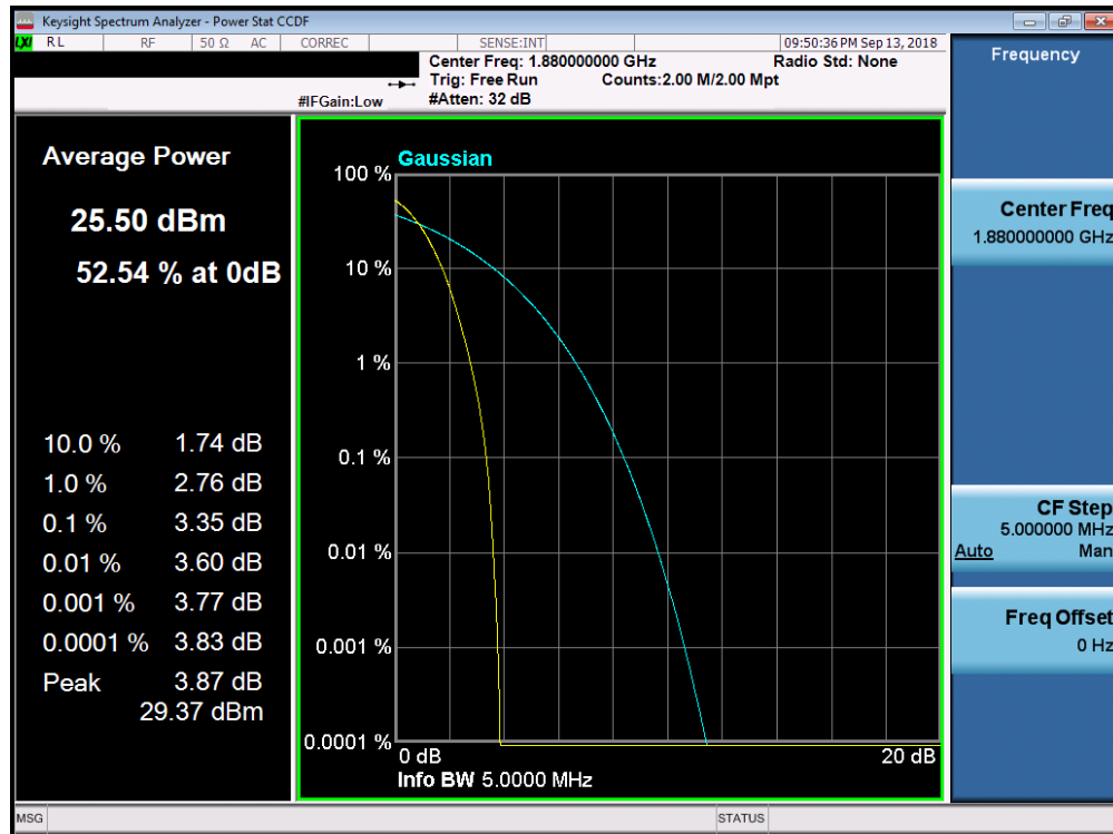
Plot 7-73. Peak-Average Ratio Plot (PCS WCDMA Mode)
