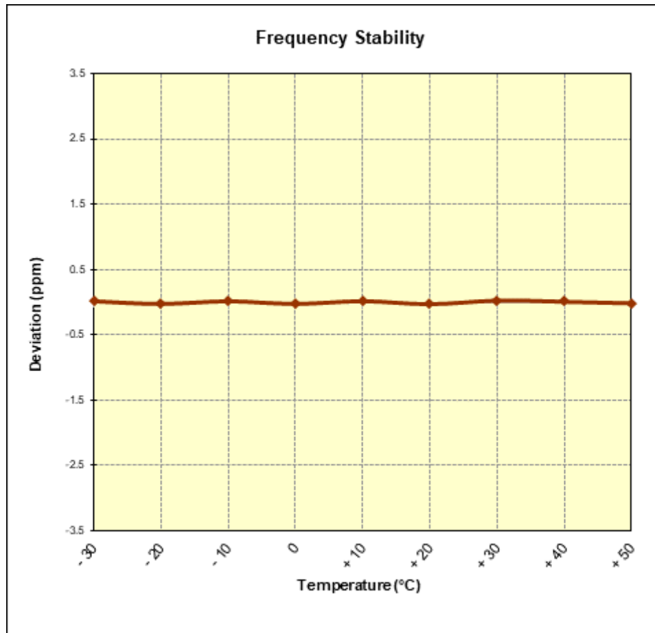
Figure 7-9. Frequency Stability Graph (AWS WCDMA Mode – Ch. 1413)
