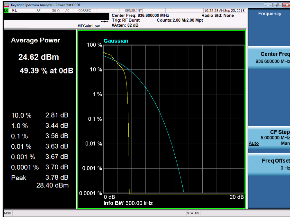
Plot 7-68. Peak-Average Ratio Plot (EDGE850 Mode)
