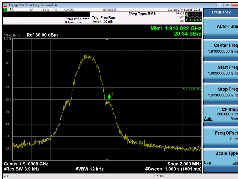
Plot 7-56. Band Edge Plot (PCS GSM Mode - High Channel)
