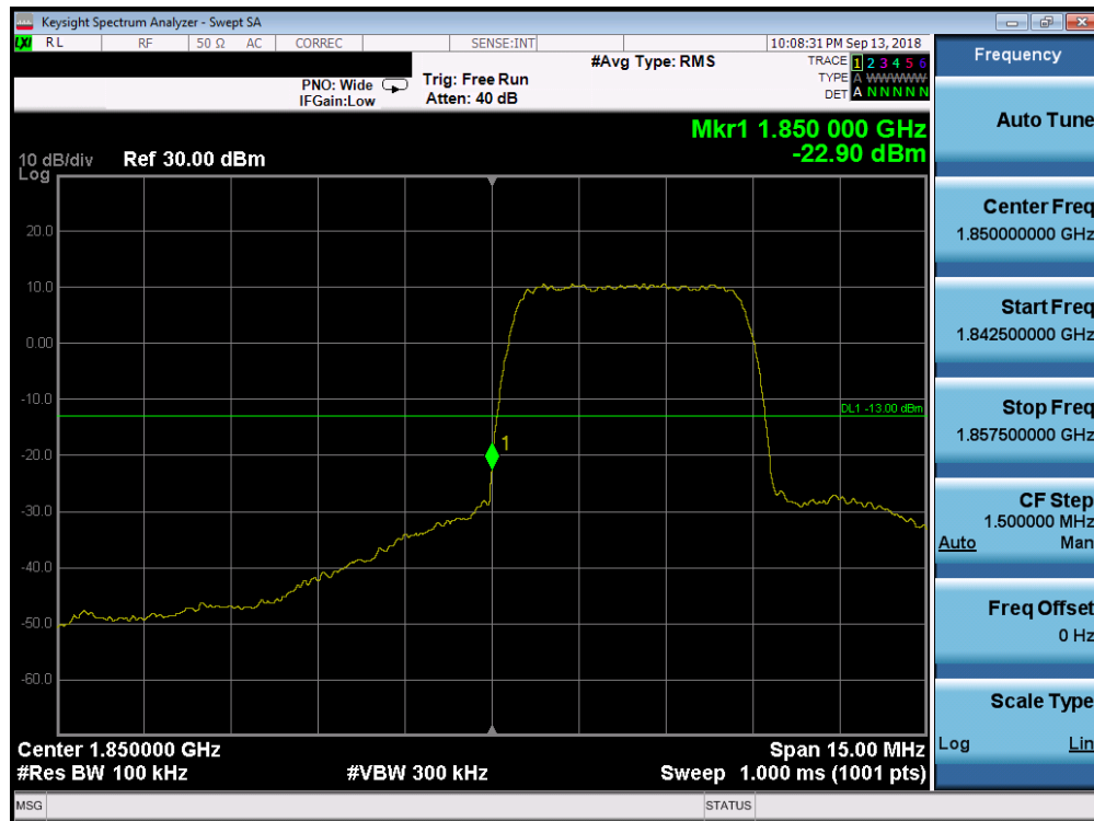
Plot 7-63. Band Edge Plot (PCS WCDMA Mode - Low Channel)
