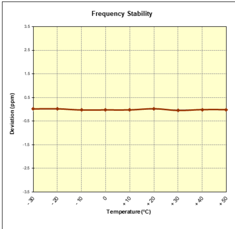
Figure 7-10. Frequency Stability Graph (PCS GPRS Mode – Ch. 661)
