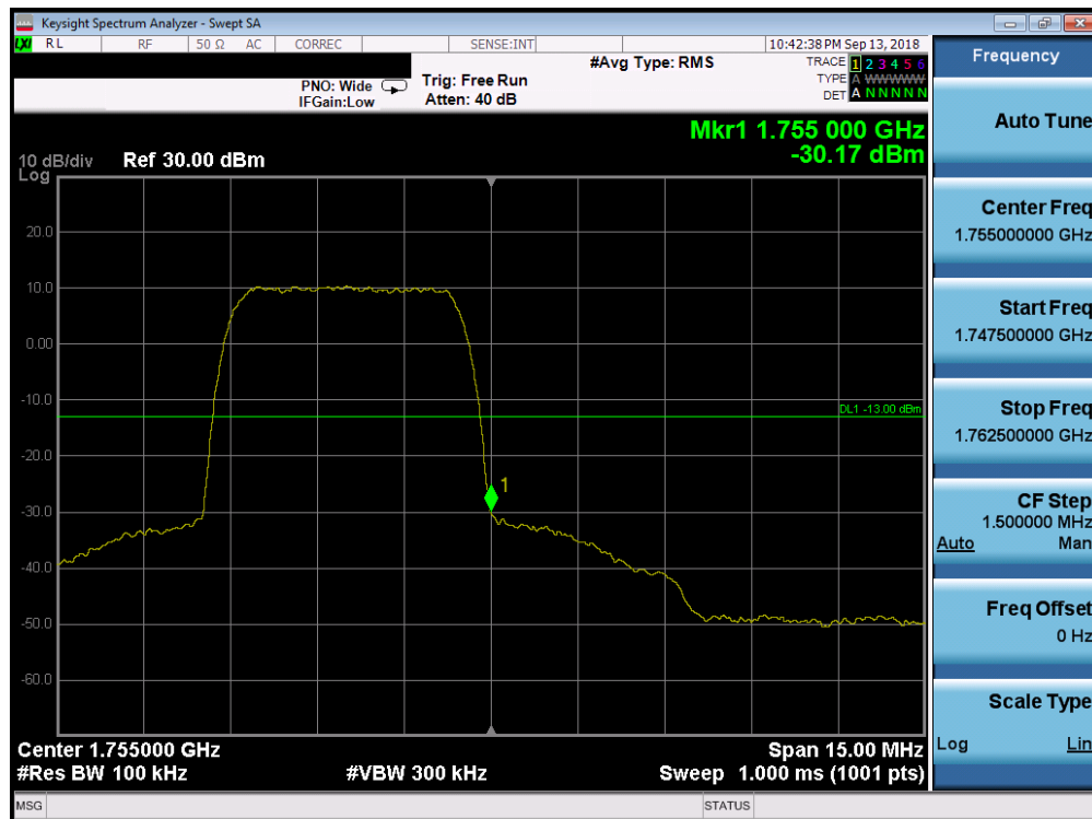
Plot 7-61. Band Edge Plot (AWS WCDMA Mode - High Channel)
