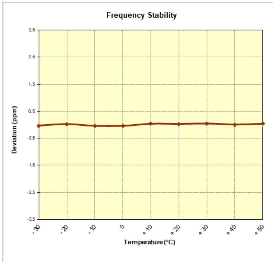
Figure 7-7. Frequency Stability Graph (Cellular GPRS Mode – Ch. 190)
