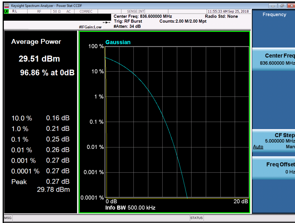
Plot 7-67. Peak-Average Ratio Plot (Cellular GPRS Mode)
