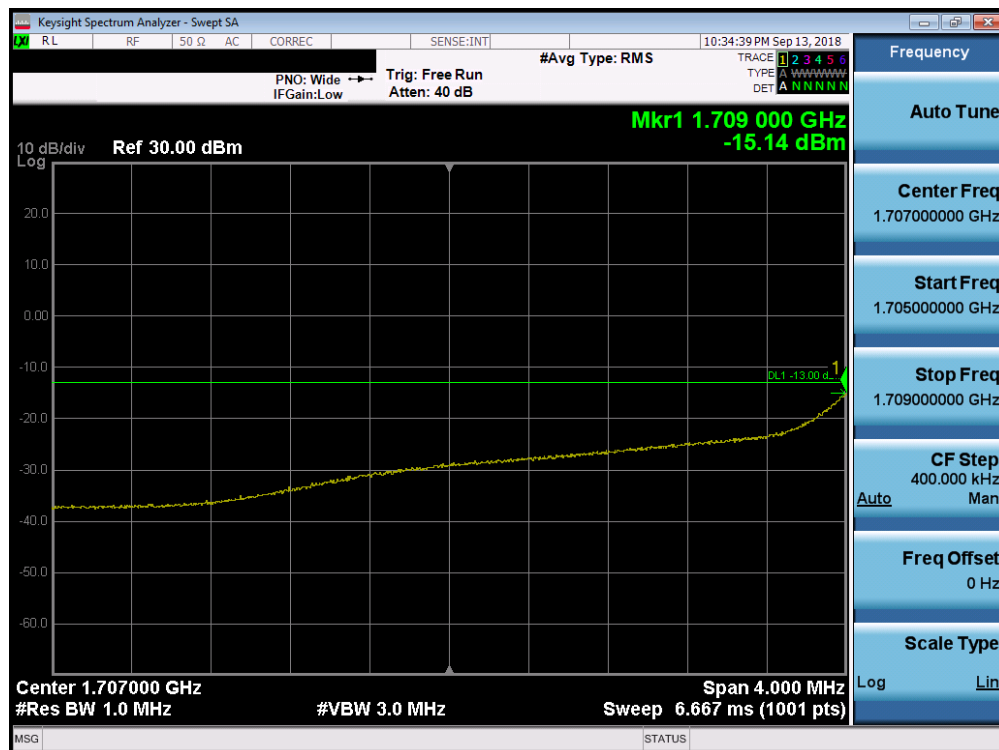
Plot 7-60. 4MHz Span Plot (AWS WCDMA Mode - Low Channel)
