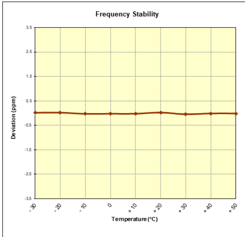
Figure 7-11. Frequency Stability Graph (PCS WCDMA Mode – Ch. 9400)
