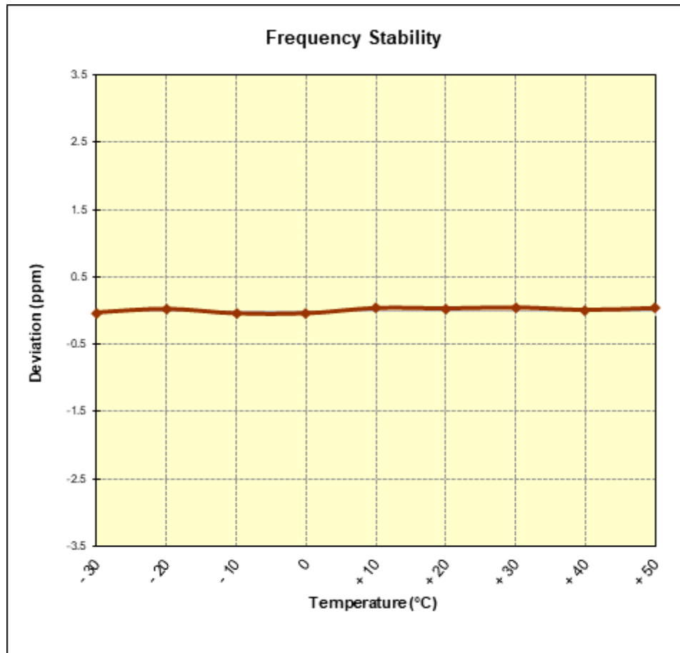
Figure 7-8. Frequency Stability Graph (Cellular WCDMA Mode – Ch. 4183)
