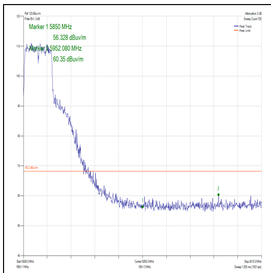
Figure 420 – Channel 142 - Authorised Band Edge
