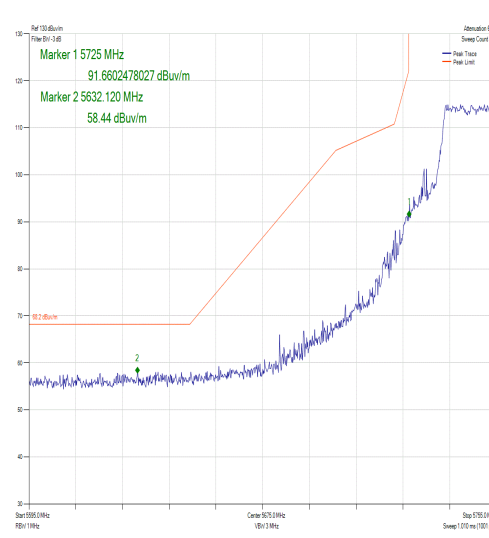
Figure 451 – Channel 149 - Authorised Band Edge
