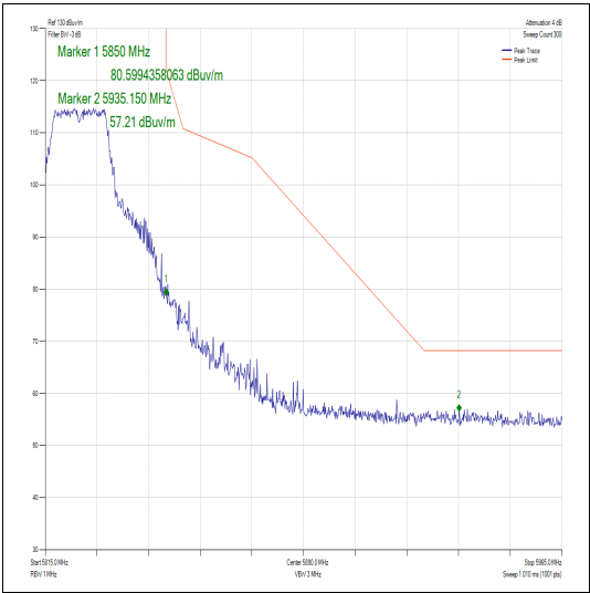
Figure 452 – Channel 165 - Authorised Band Edge
