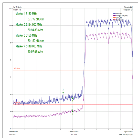
Figure 539 – Channel 42 – Restricted Band Edge
