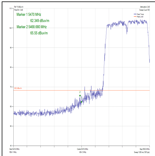
Figure 418 – Channel 102 - Authorised Band Edge
