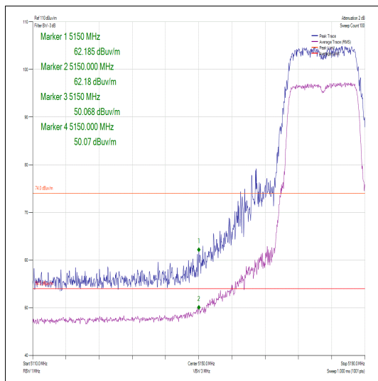
Figure 542 – Channel 36 – Restricted Band Edge
