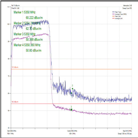
Figure 525 – Channel 62 - Restricted Band Edge
