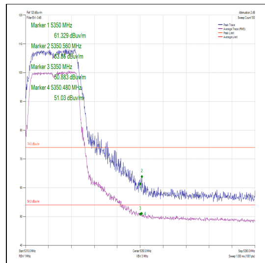
Figure 543 – Channel 64 - Restricted Band Edge
