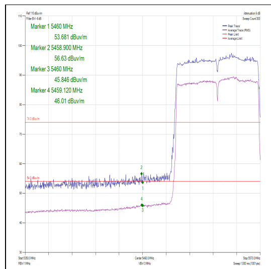
Figure 541 – Channel 106 – Restricted Band Edge
