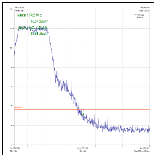
Figure 449 – Channel 140 - Authorised Band Edge
