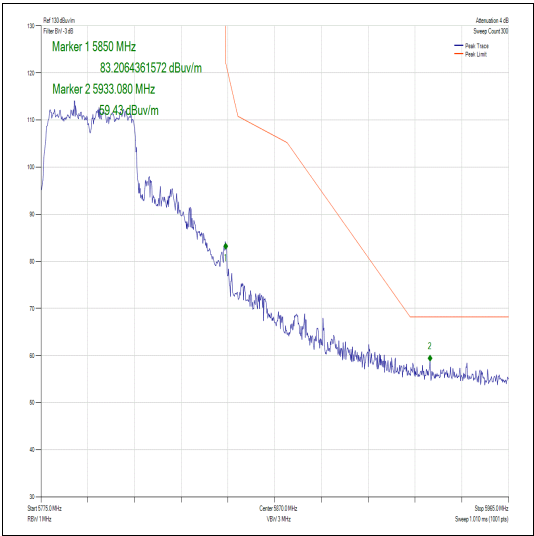
Figure 432 – Channel 159 - Authorised Band Edge
