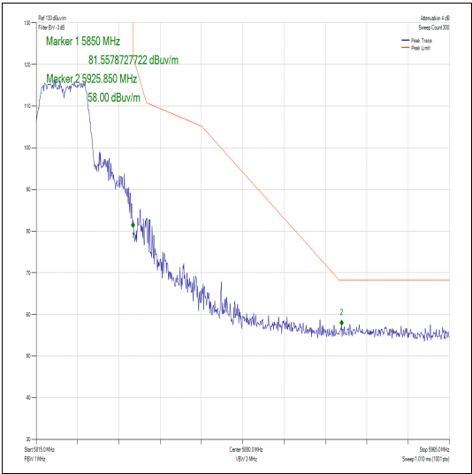
Figure 412 – Channel 165 - Authorised Band Edge
