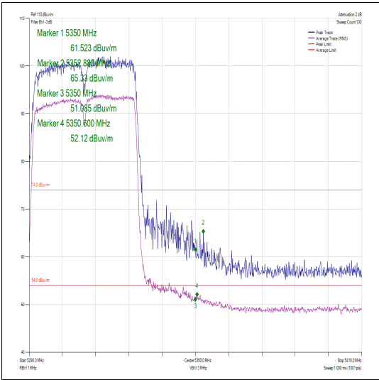
Figure 549 – Channel 62 - Restricted Band Edge
