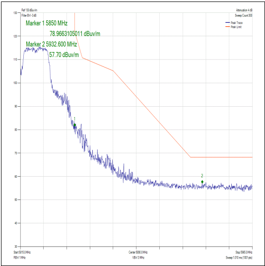
Figure 402 – Channel 165 - Authorized Band Edge
