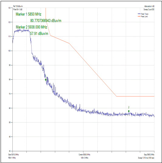
Figure 407 – Channel 165 - Authorised Band Edge
