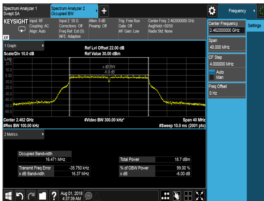
Figure 27 - 2462 MHz – 6 dB Bandwidth and 99% Occupied Bandwidth
