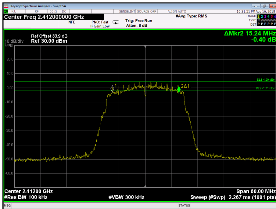
Figure 16 - 2412 MHz – 6 dB Bandwidth
