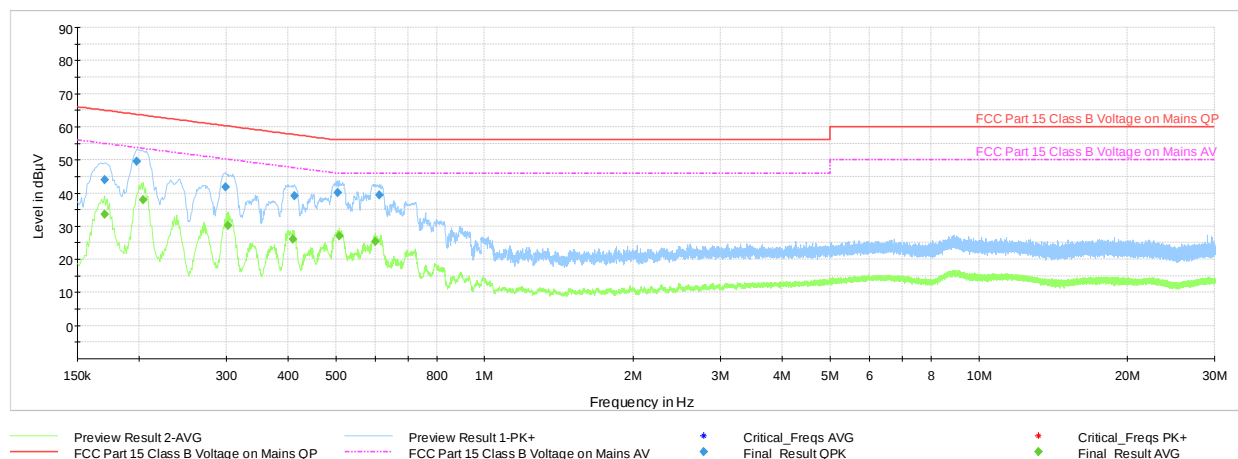
Plot 7-118. Line Conducted Plot with Bluetooth HDR (L1, with AC/DC Adapter)
