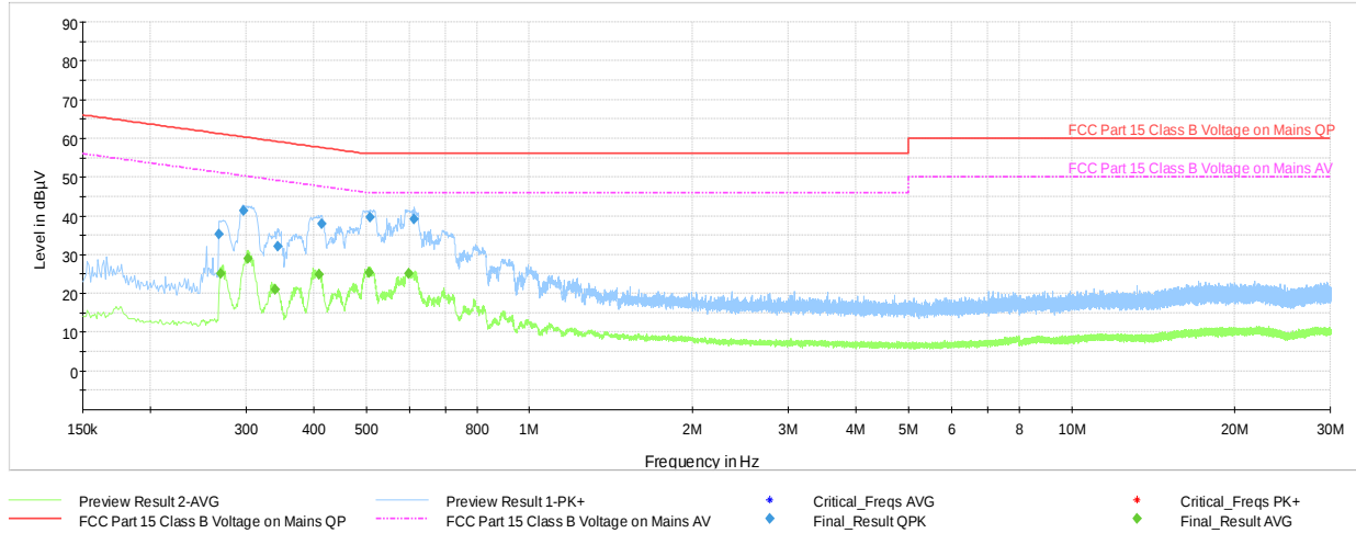
Plot 7-119. Line Conducted Plot with Bluetooth HDR (N, with AC/DC Adapter)
