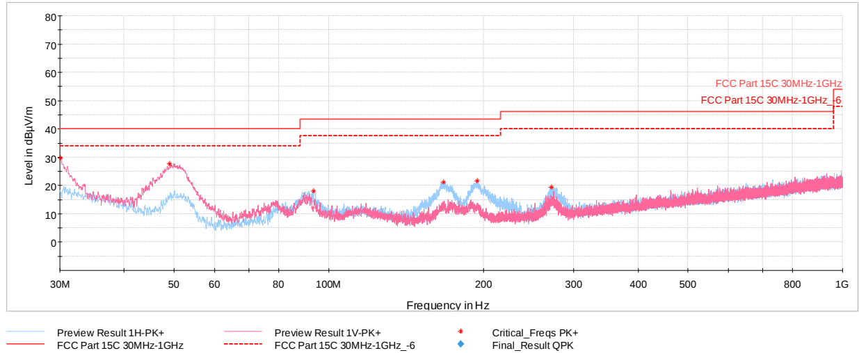
Plot 7-117. Radiated Spurious Plot below 1GHz (4Mbps, HDR4 ePA, Pol. H & V, with AC/DC Adapter)
