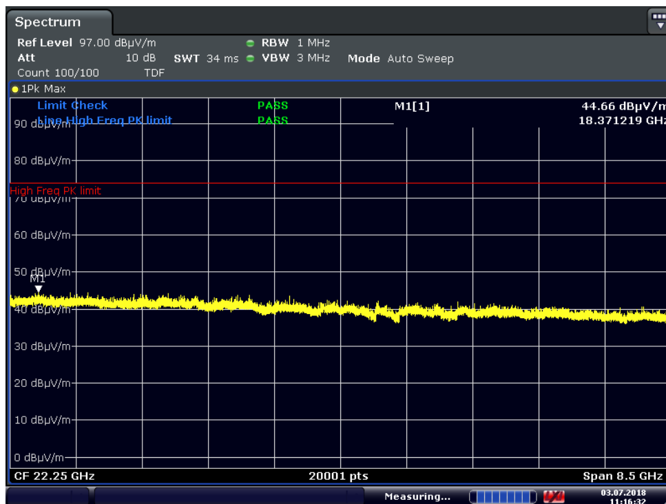
Plot 7-104. Radiated Spurious Plot Above 18GHz ANT0 (8Mbps, HDR8 ePA, Ant. Pol. V)
