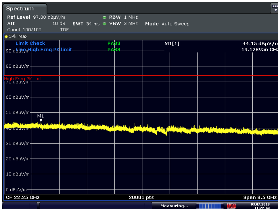
Plot 7-103. Radiated Spurious Plot Above 18GHz ANT0 (8Mbps, HDR8 ePA, Ant. Pol. H)
