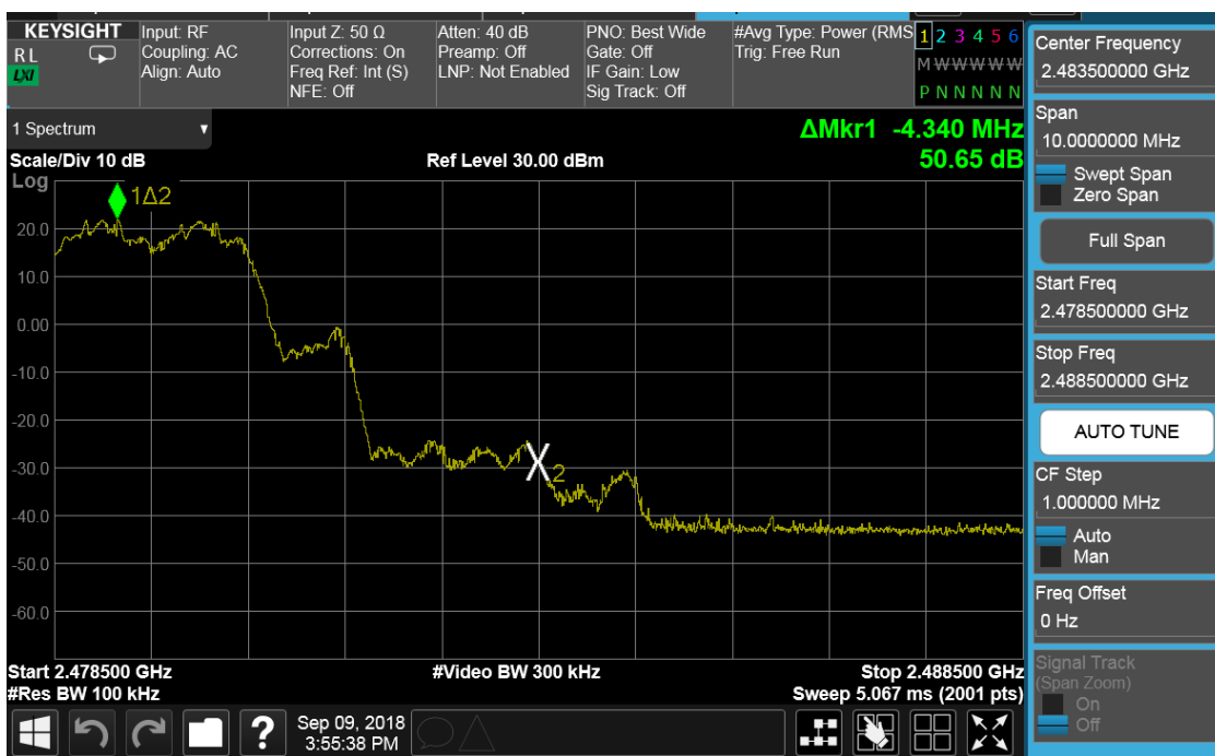
Plot 7-26. Band Edge Plot ANT 0 (Bluetooth with Hopping Enabled, 8DPSK, ePA)
