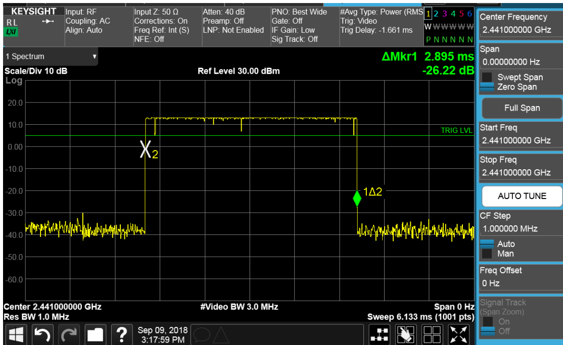
Plot 7-49. Time of Occupancy Plot ANT0(Bluetooth, GFSK, ePA)
