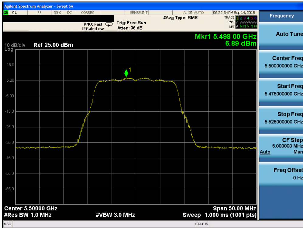
Plot 7-129. Power Spectral Density Plot CDD CORE 0 (20MHz BW 802.11n (UNII Band 2C) – Ch. 100)
