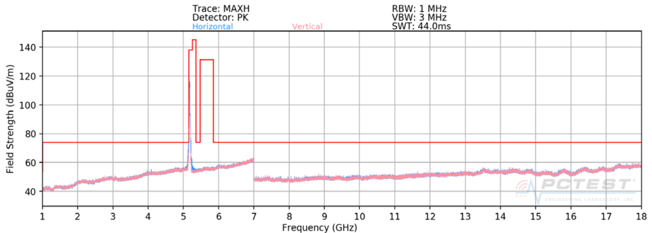
Plot 7-170. Radiated Spurious Plot above 1GHz SISO CORE 1 (802.11n – U1 Ch. 36)
