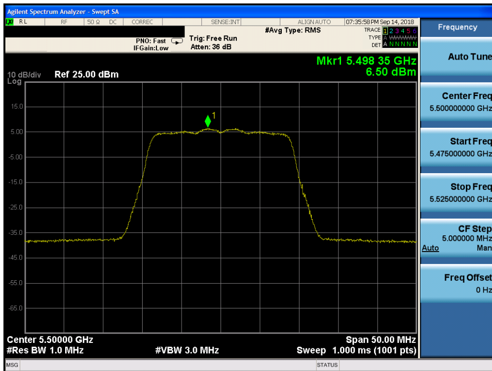
Plot 7-130. Power Spectral Density Plot CDD CORE 1 (20MHz BW 802.11n (UNII Band 2C) – Ch. 100)
