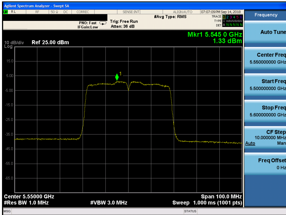
Plot 7-137. Power Spectral Density Plot CDD CORE 0 (40MHz BW 802.11n (UNII Band 2C) – Ch. 110)
