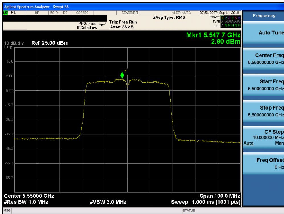
Plot 7-138. Power Spectral Density Plot CDD CORE 1 (40MHz BW 802.11n (UNII Band 2C) – Ch. 110)
