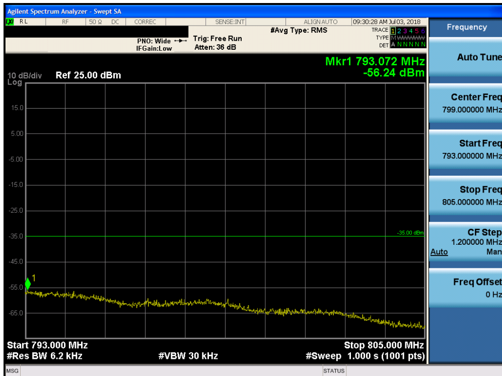
Plot 7-175. Upper Emission Mask Edge Plot (Band 13 - 5.0MHz QPSK - Full RB Configuration)
