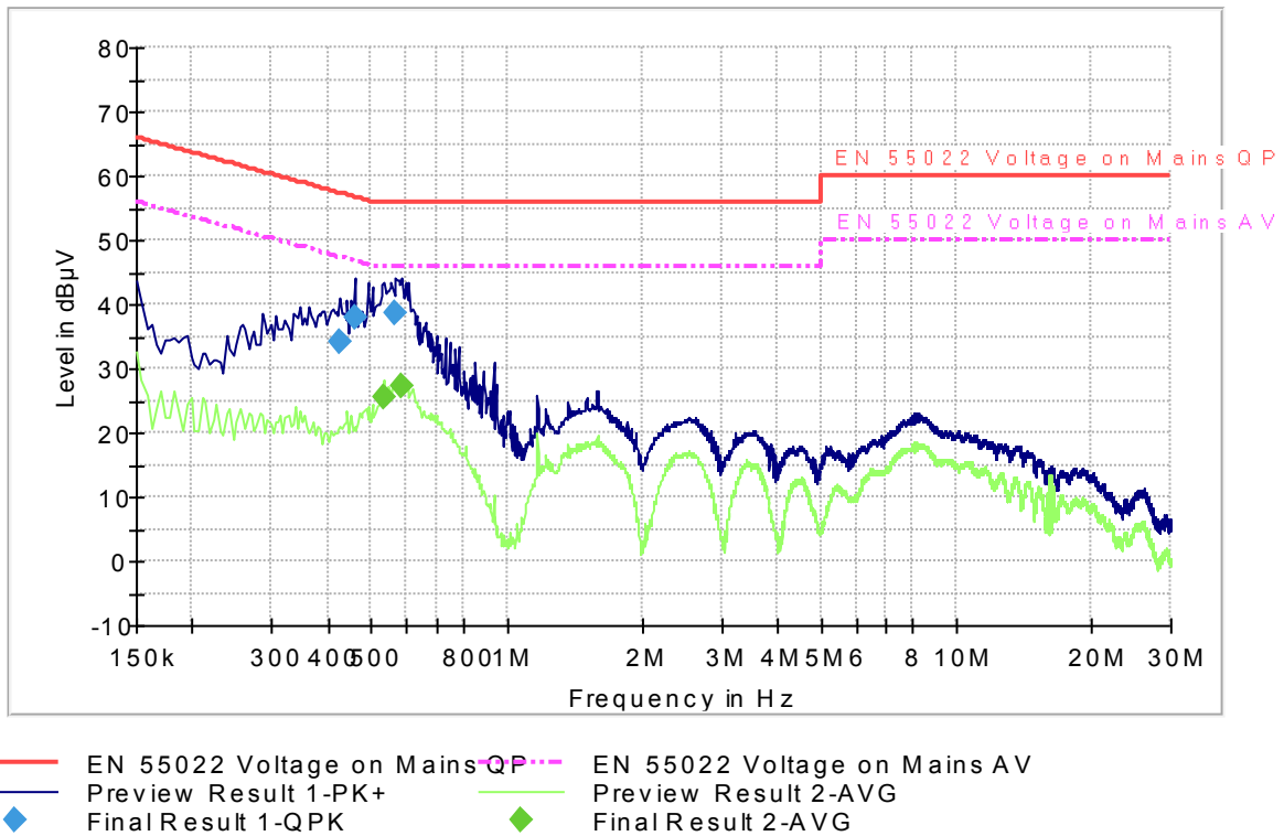
CISPR 22 Mains Conducted FCC_LISN
