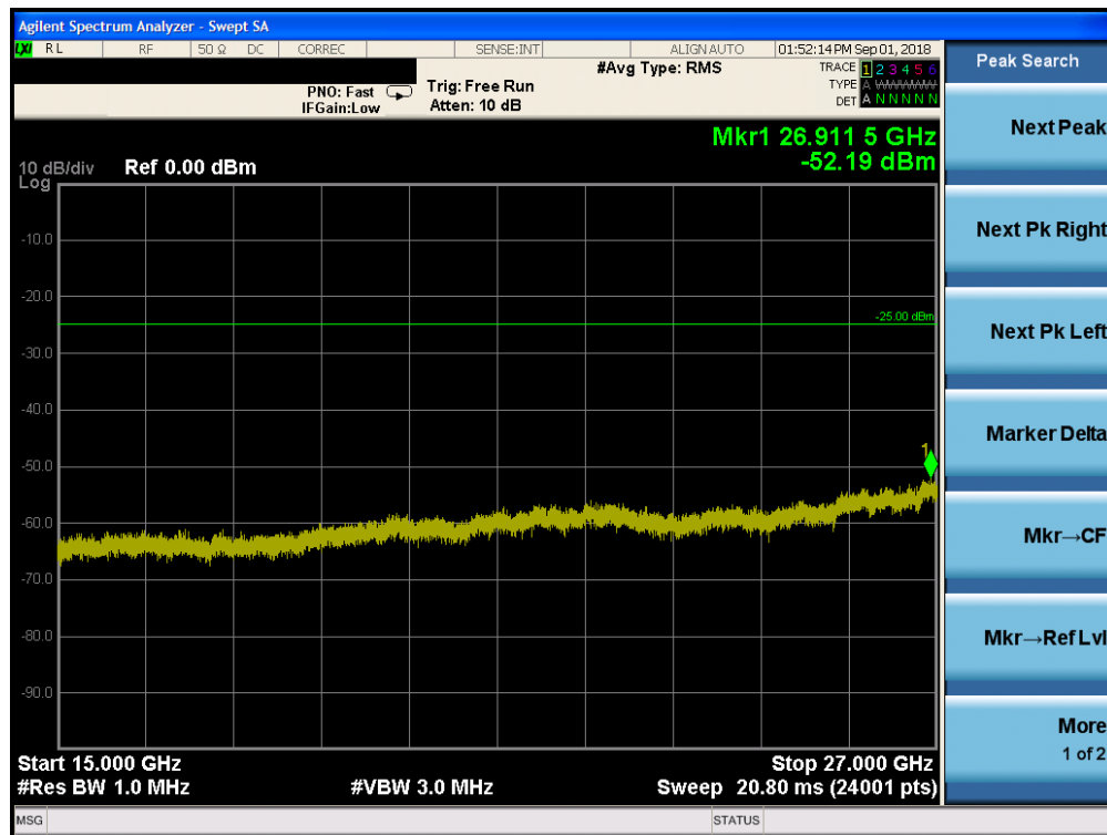
Plot 7-394. Conducted Spurious Plot (Band 7 – 20.0MHz QPSK – PCC 100/0 SCC 100/0 – Mid Channel)
