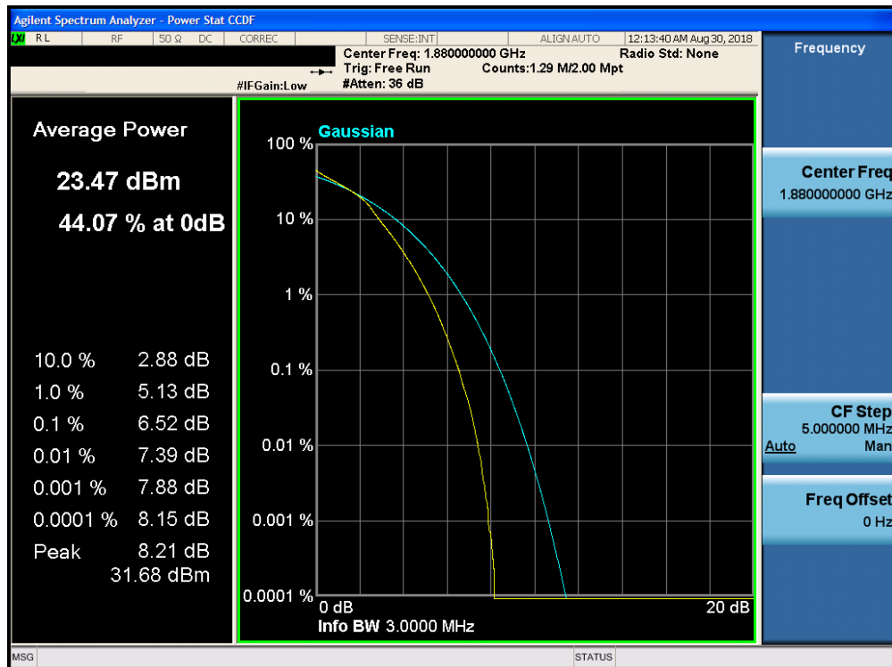
Plot 7-355. PAR Plot (Band 2 – 3.0MHz 16-QAM – RB Size 15)
