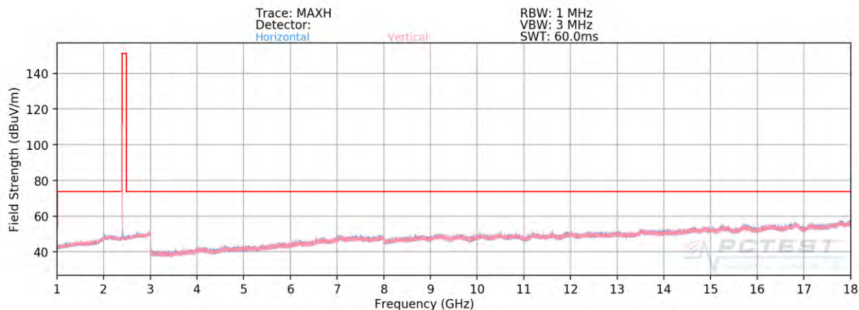
Plot 7-82. Radiated Spurious Plot Above 1GHz ANT1 (1Mbps, ePA – Ch. 0, Ant. Pol. H & V)
