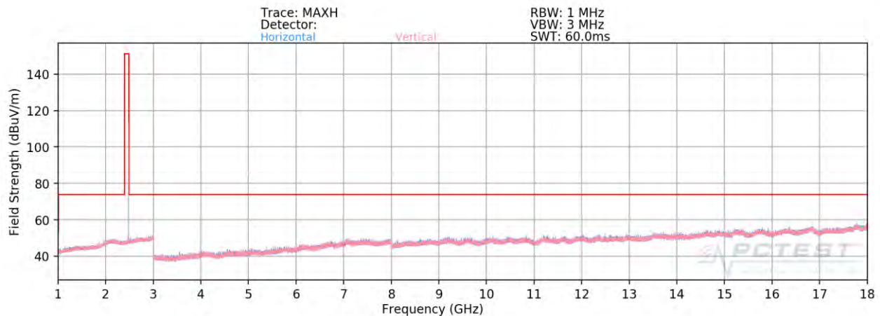
Plot 7-81. Radiated Spurious Plot Above 1GHz ANT0 (1Mbps, ePA – Ch. 39, Ant. Pol. H & V)
