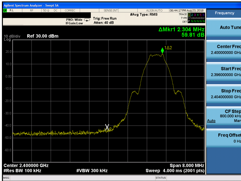
Plot 7-55. Band Edge Plot ANT0 (Bluetooth (LE), 2Mbps – Ch. 0)
