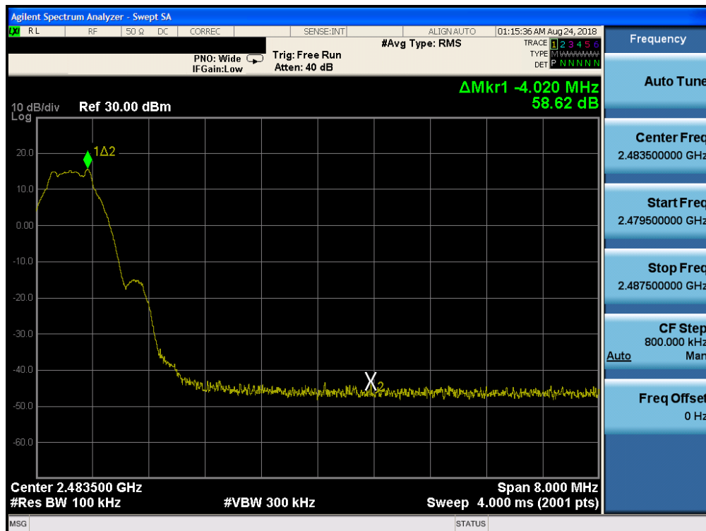
Plot 7-60. Band Edge Plot ANT2 (Bluetooth (LE), 2Mbps – Ch. 39)
