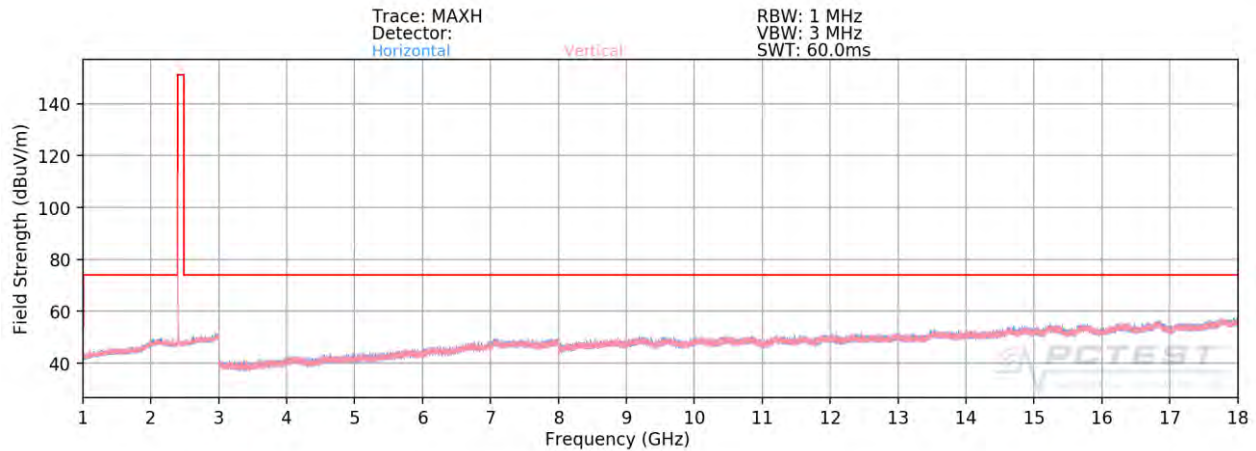
Plot 7-79. Radiated Spurious Plot Above 1GHz ANT0 (1Mbps, ePA – Ch. 0, Ant. Pol. H & V)
