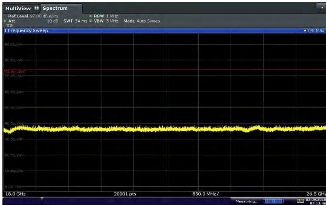
Plot 7-88. Radiated Spurious Plot Above 18GHz ANT0 (1Mbps, ePA, Ant. Pol. H)
