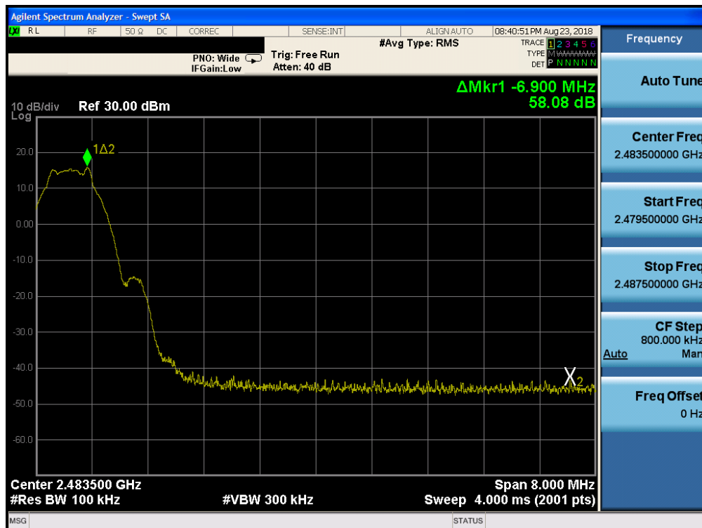
Plot 7-58. Band Edge Plot ANT1 (Bluetooth (LE), 2Mbps - Ch. 39)
