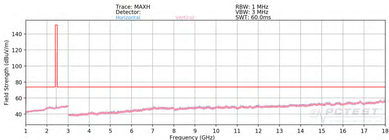
Plot 7-83. Radiated Spurious Plot Above 1GHz ANT1 (1Mbps, ePA – Ch. 19, Ant. Pol. H & V)
