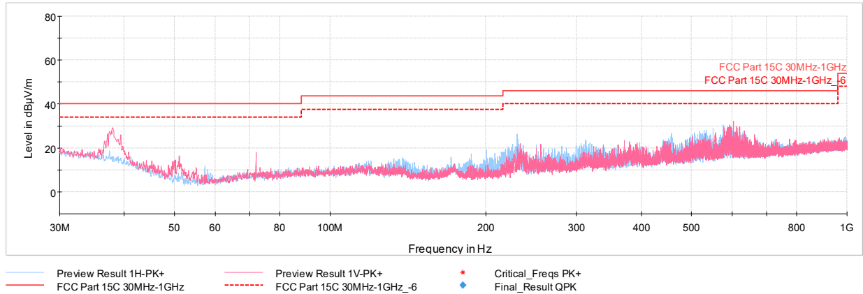
Plot 7-102. Radiated Spurious Plot below 1GHz (1Mbps, ePA, Pol. H & V, with Laptop)
