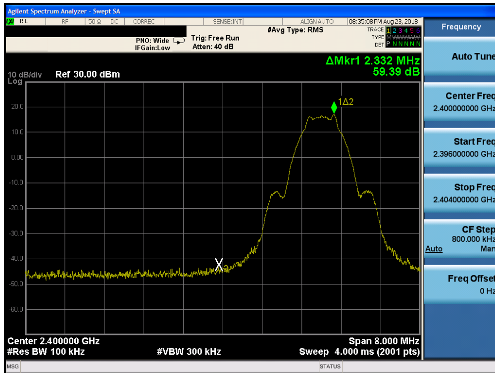
Plot 7-57. Band Edge Plot ANT1 (Bluetooth (LE), 2Mbps - Ch. 0)
