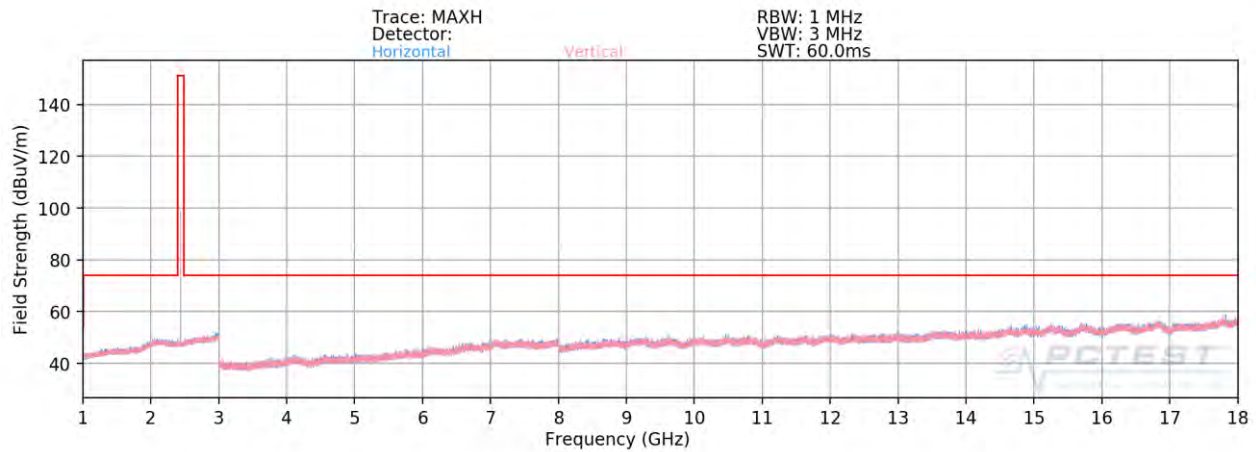
Plot 7-86. Radiated Spurious Plot Above 1GHz ANT2 (1Mbps, ePA – Ch. 19, Ant. Pol. H & V)
