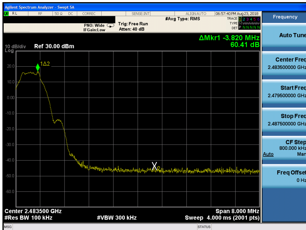
Plot 7-56. Band Edge Plot ANT0 (Bluetooth (LE), 2Mbps – Ch. 39)
