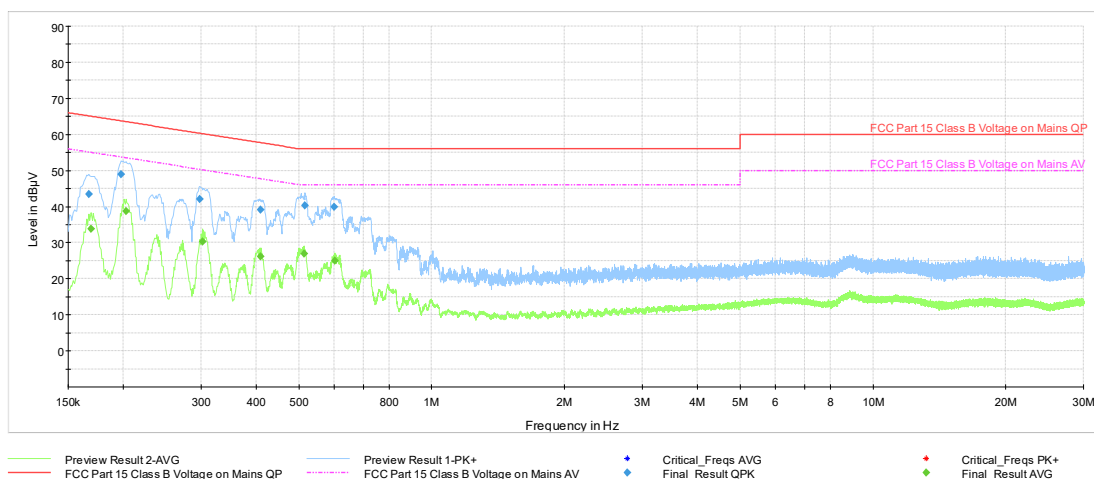
Plot 7-103. Line Conducted Plot with Bluetooth LE (L1, with AC/DC Adapter)
