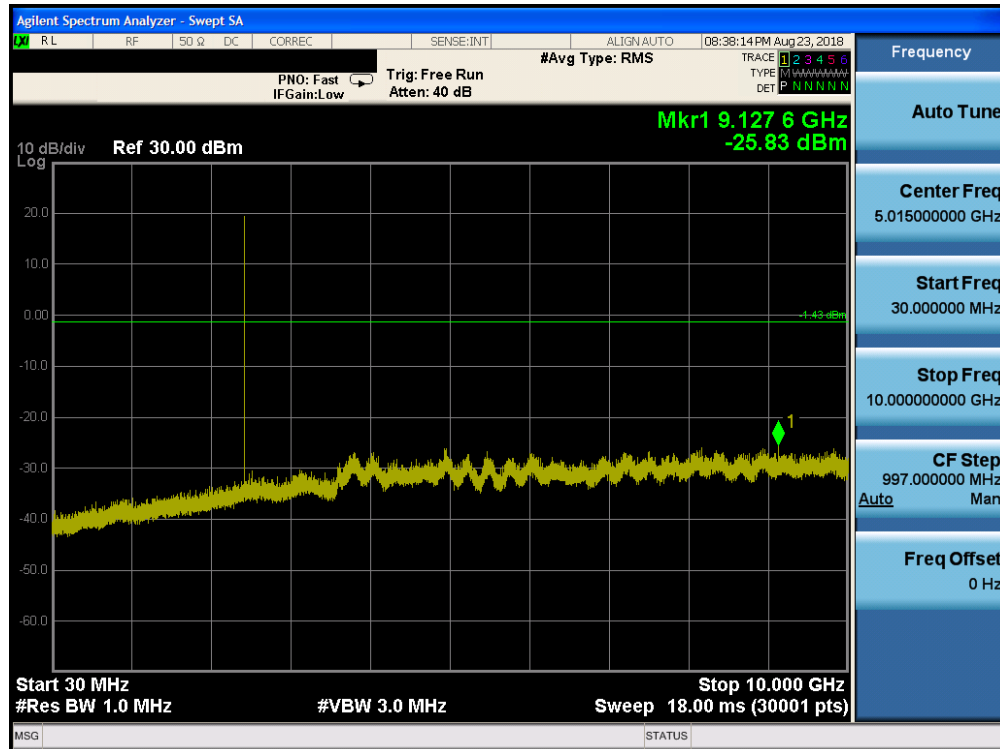
Plot 7-69. Conducted Spurious Plot ANT1 (Bluetooth (LE), 1Mbps, ePA - Ch. 19)
