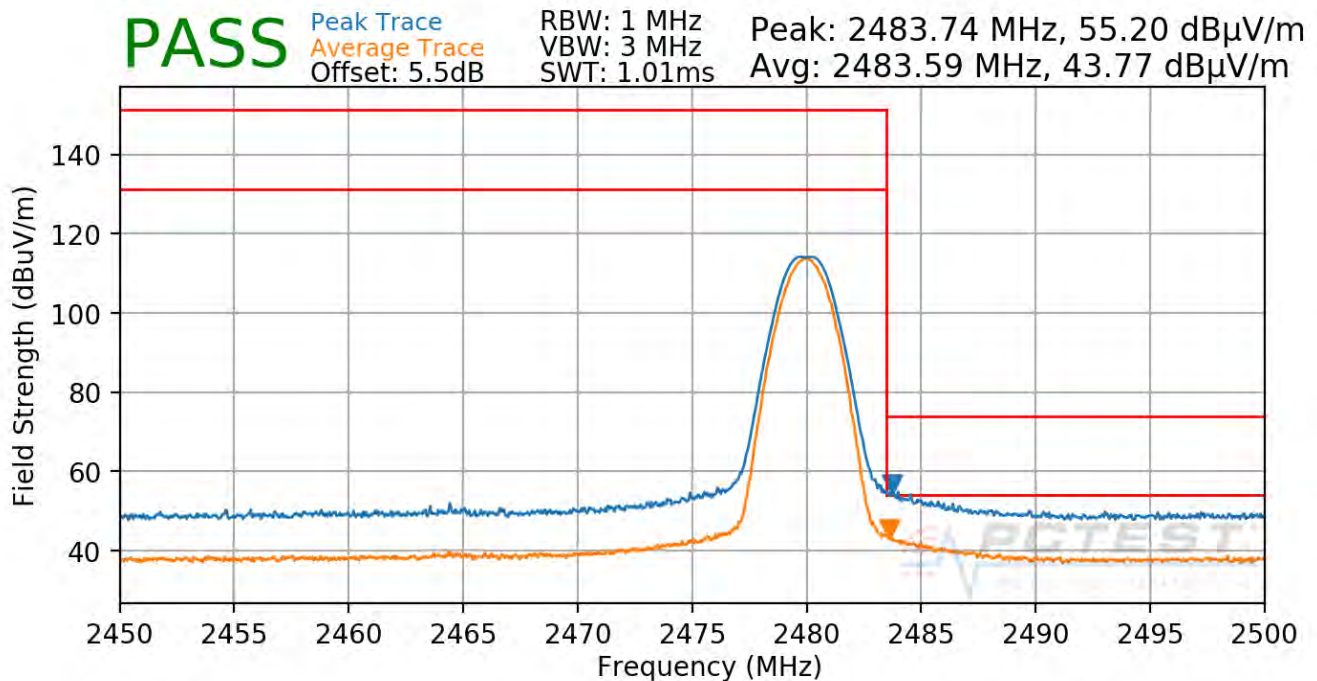
Plot 7-97. Radiated Restricted Upper Band Edge Measurement ANT1 (Average & Peak)
