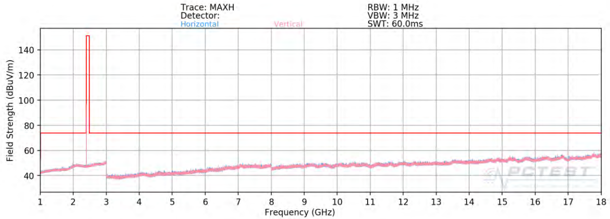
Plot 7-85. Radiated Spurious Plot Above 1GHz ANT2 (1Mbps, ePA – Ch. 0, Ant. Pol. H & V)
