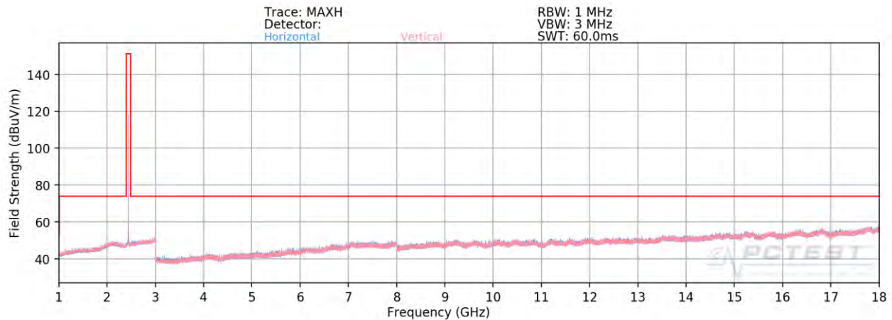
Plot 7-80. Radiated Spurious Plot Above 1GHz ANT0 (1Mbps, ePA – Ch. 19, Ant. Pol. H & V)
