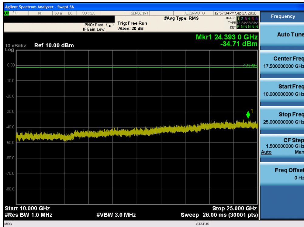
Plot 7-70. Conducted Spurious Plot ANT1 (Bluetooth (LE), 1Mbps, ePA - Ch. 19)
