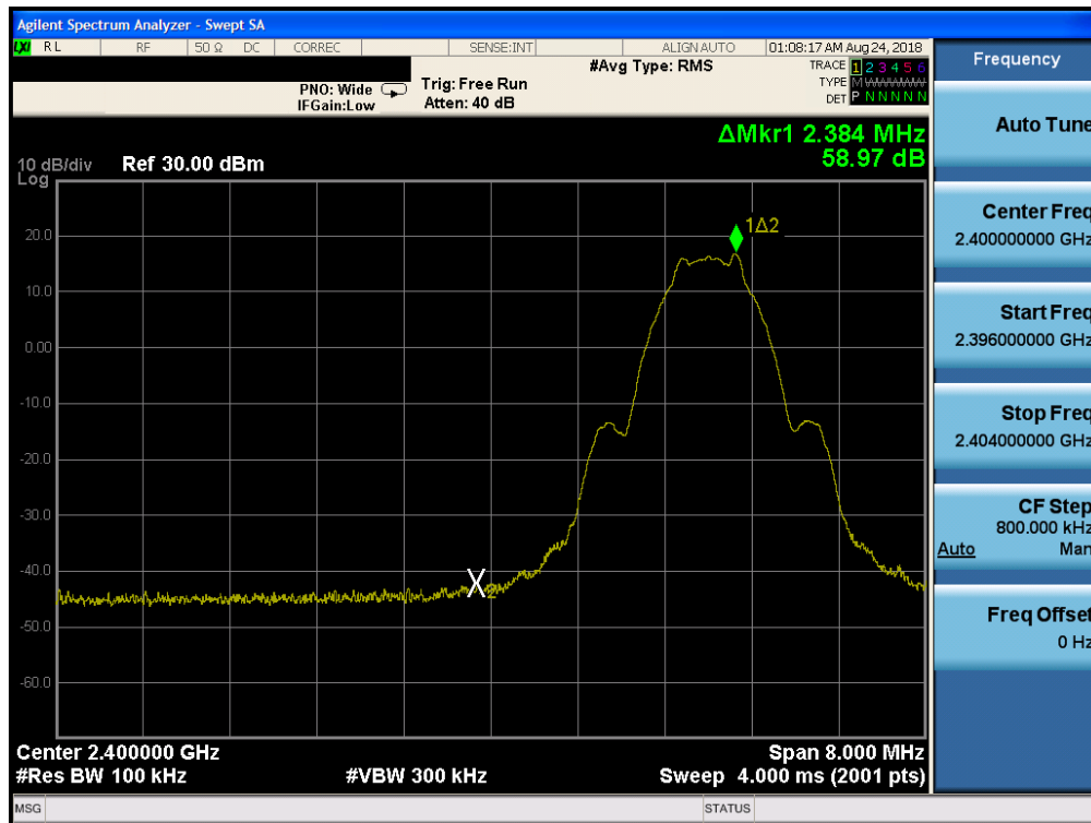
Plot 7-59. Band Edge Plot ANT2 (Bluetooth (LE), 2Mbps – Ch. 0)
