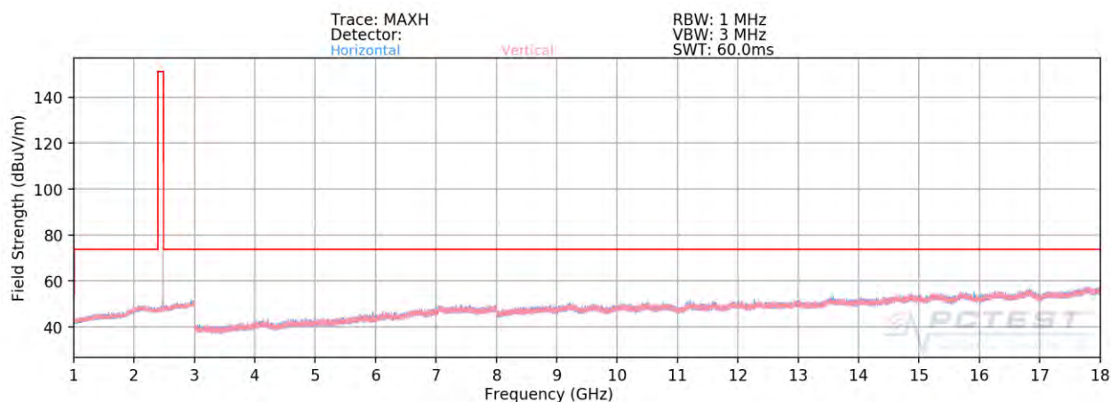
Plot 7-84. Radiated Spurious Plot Above 1GHz ANT1 (1Mbps, ePA – Ch. 39, Ant. Pol. H & V)
