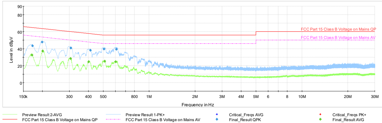
Plot 7-104. Line Conducted Plot with Bluetooth LE (N, with AC/DC Adapter)
