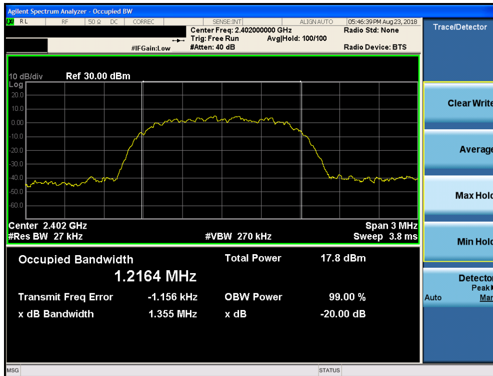
Plot 7-4. 20dB Bandwidth Plot ANT 0 (Bluetooth, 8DPSK, ePA – Ch. 0)
