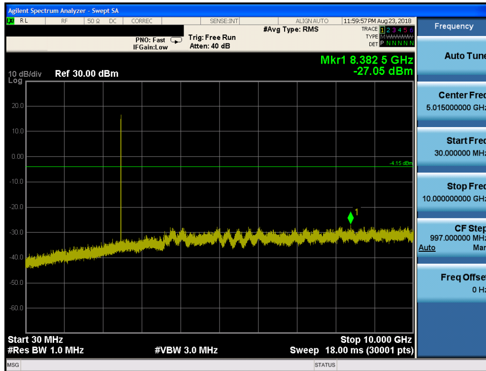
Plot 7-83. Conducted Spurious Plot ANT 2 (Bluetooth, GFSK, ePA – Ch. 78)
