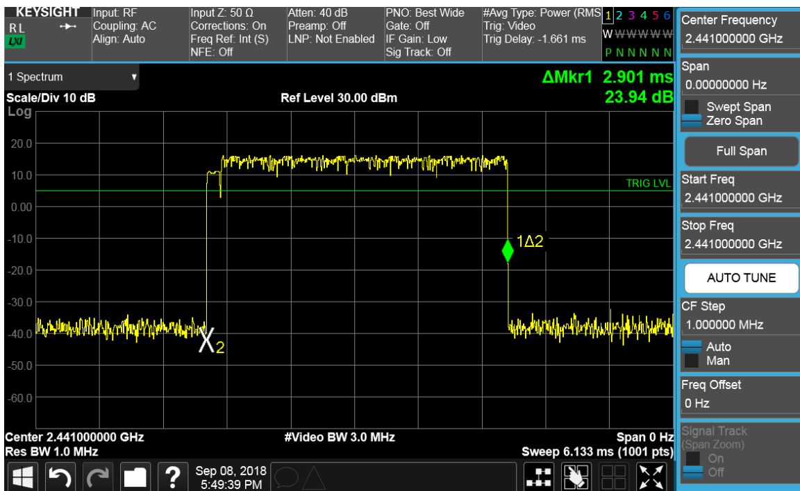
Plot 7-54. Time of Occupancy Plot ANT2(Bluetooth, 8DPSK, ePA)
