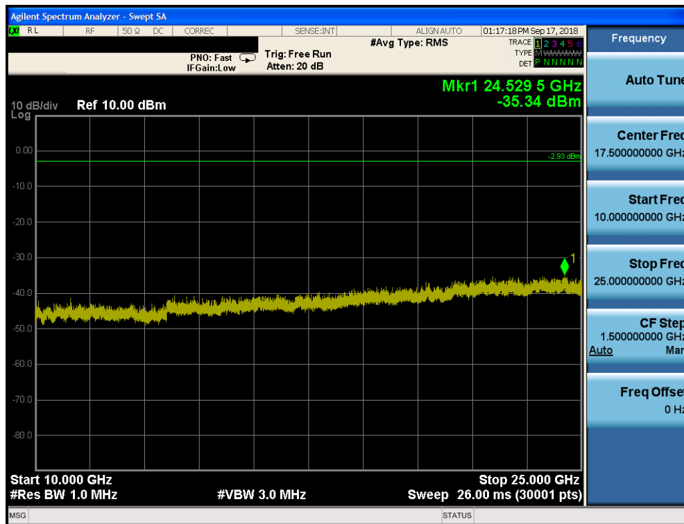
Plot 7-74. Conducted Spurious Plot ANT 1 (Bluetooth, GFSK, ePA – Ch. 0)
