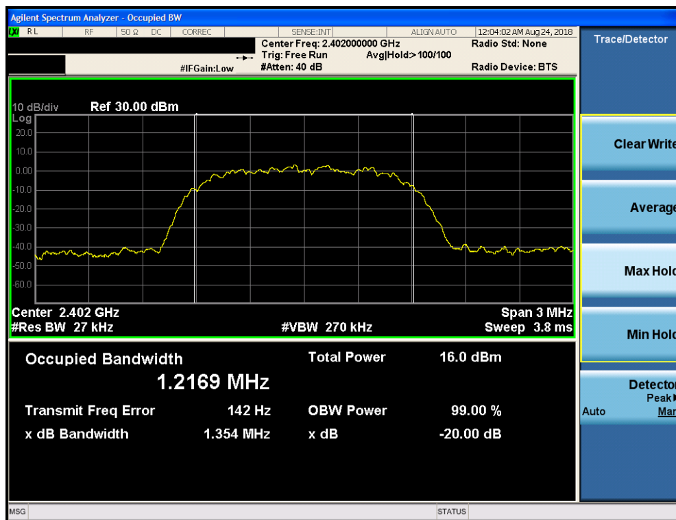
Plot 7-16. 20dB Bandwidth Plot ANT 2 (Bluetooth, 8DPSK, ePA – Ch. 0)
