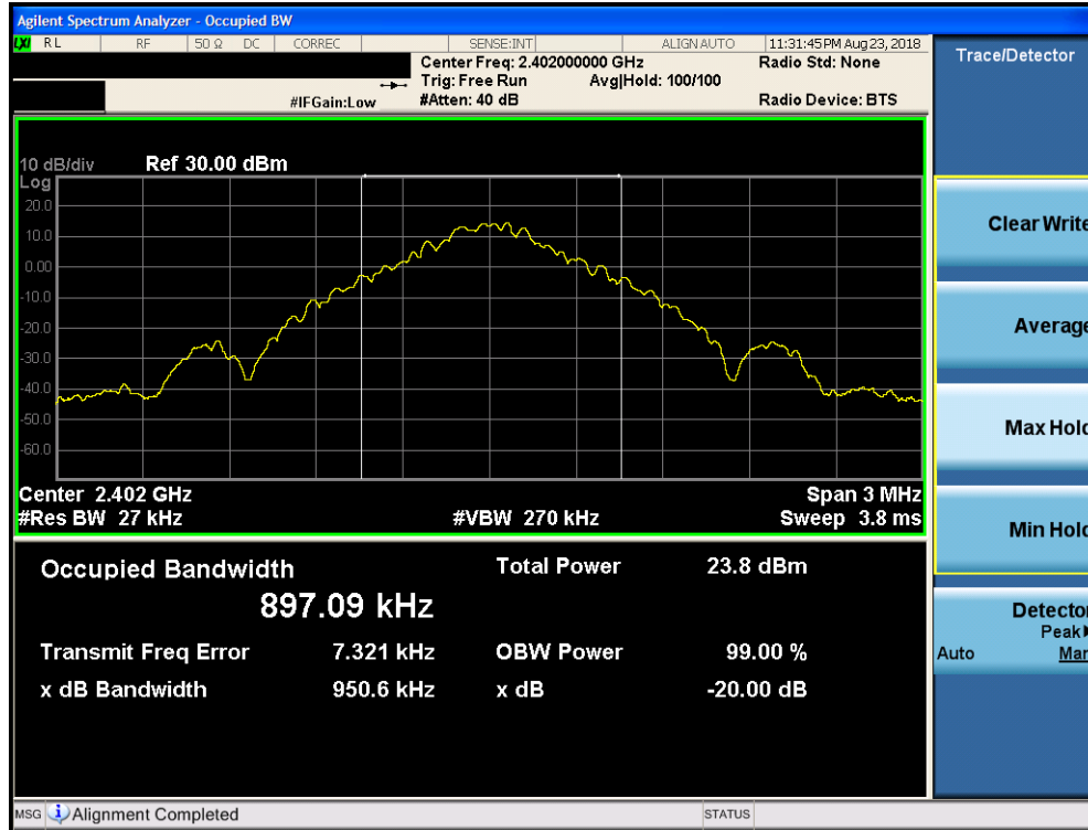
Plot 7-13. 20dB Bandwidth Plot ANT 2 (Bluetooth, GFSK, ePA – Ch. 0)
