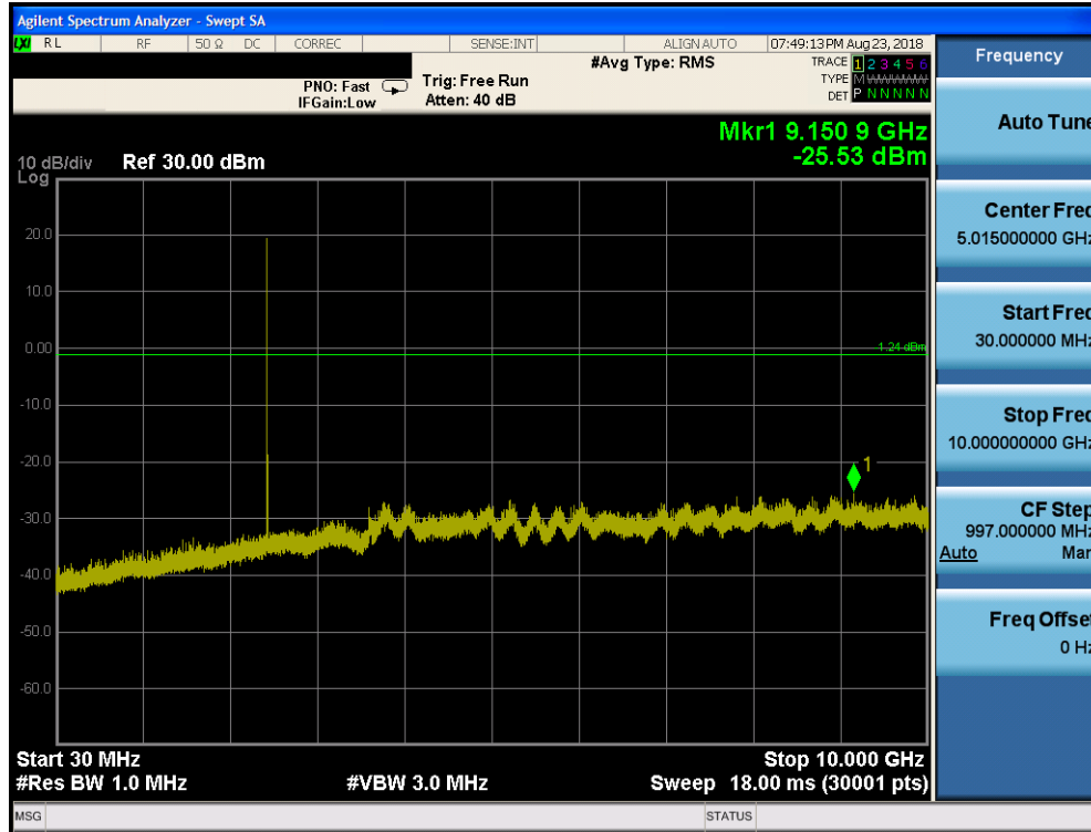
Plot 7-75. Conducted Spurious Plot ANT 1 (Bluetooth, GFSK, ePA – Ch. 39)
