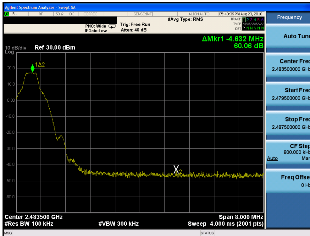
Plot 7-20. Band Edge Plot ANT 0 (Bluetooth with Hopping Disabled, GFSK, ePA – Ch. 78)
