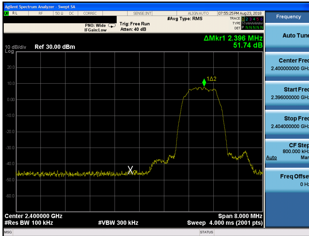
Plot 7-31. Band Edge Plot ANT 1 (Bluetooth with Hopping Disabled, 8DPSK, ePA – Ch. 0)
