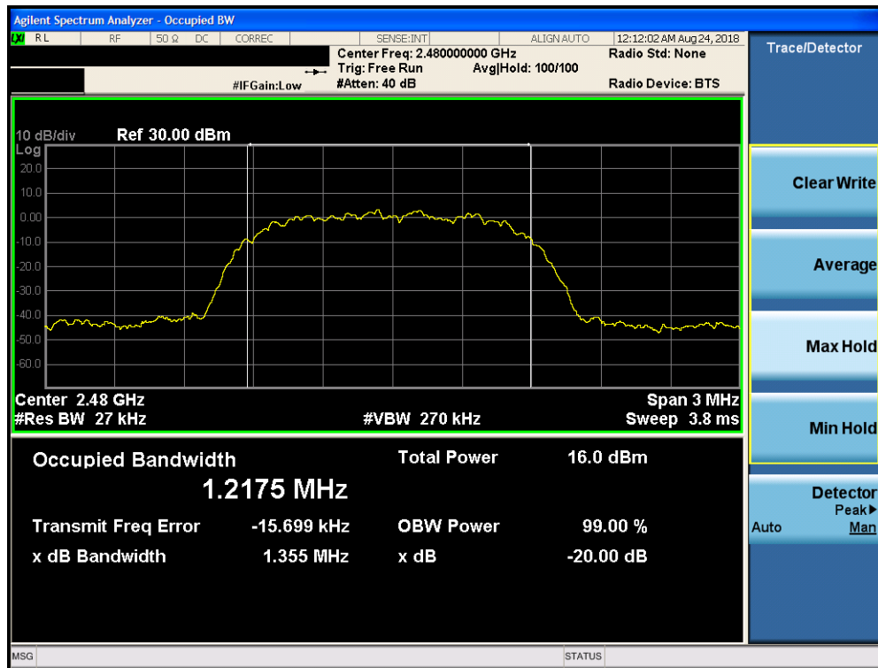
Plot 7-18. 20dB Bandwidth Plot ANT 2 (Bluetooth, 8DPSK, ePA – Ch. 78)
