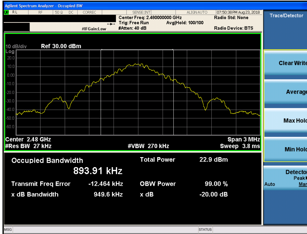
Plot 7-9. 20dB Bandwidth Plot ANT 1 (Bluetooth, GFSK, ePA – Ch. 78)
