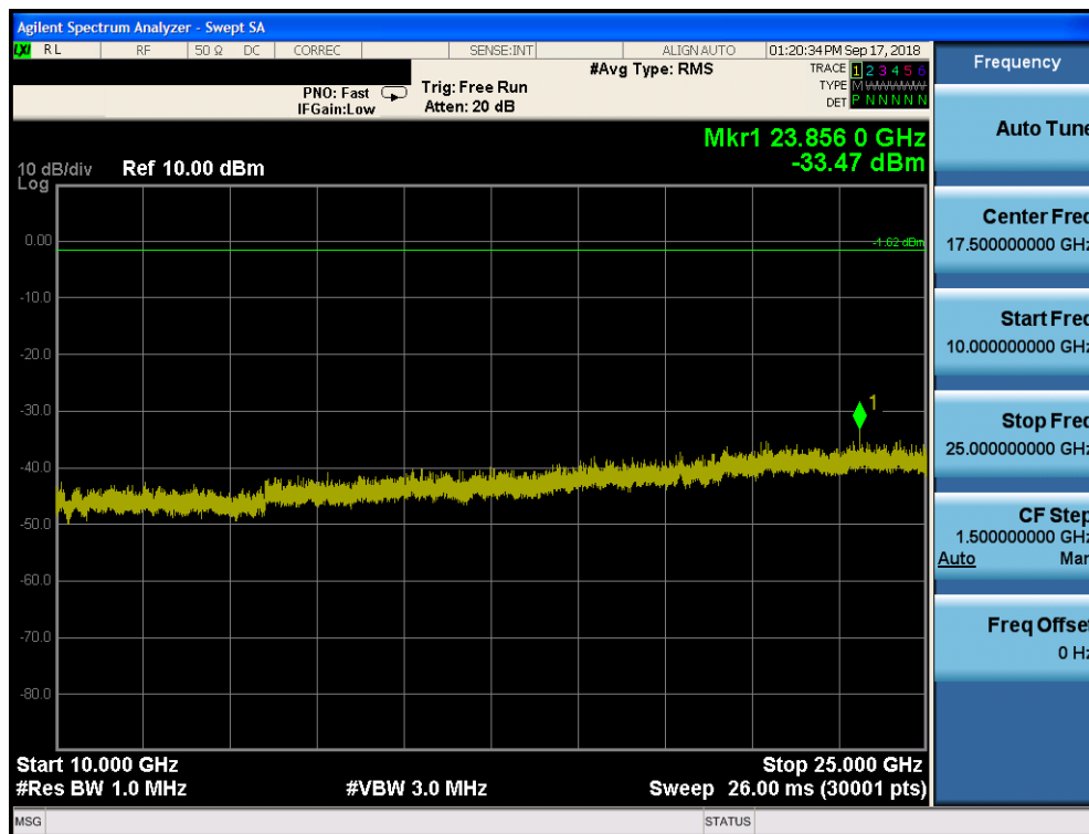
Plot 7-82. Conducted Spurious Plot ANT 2 (Bluetooth, GFSK, ePA Ch. 39)
