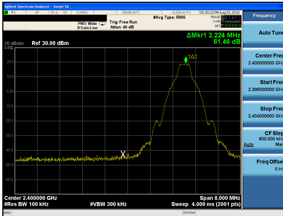
Plot 7-19. Band Edge Plot ANT 0 (Bluetooth with Hopping Disabled, GFSK, ePA – Ch. 0)
