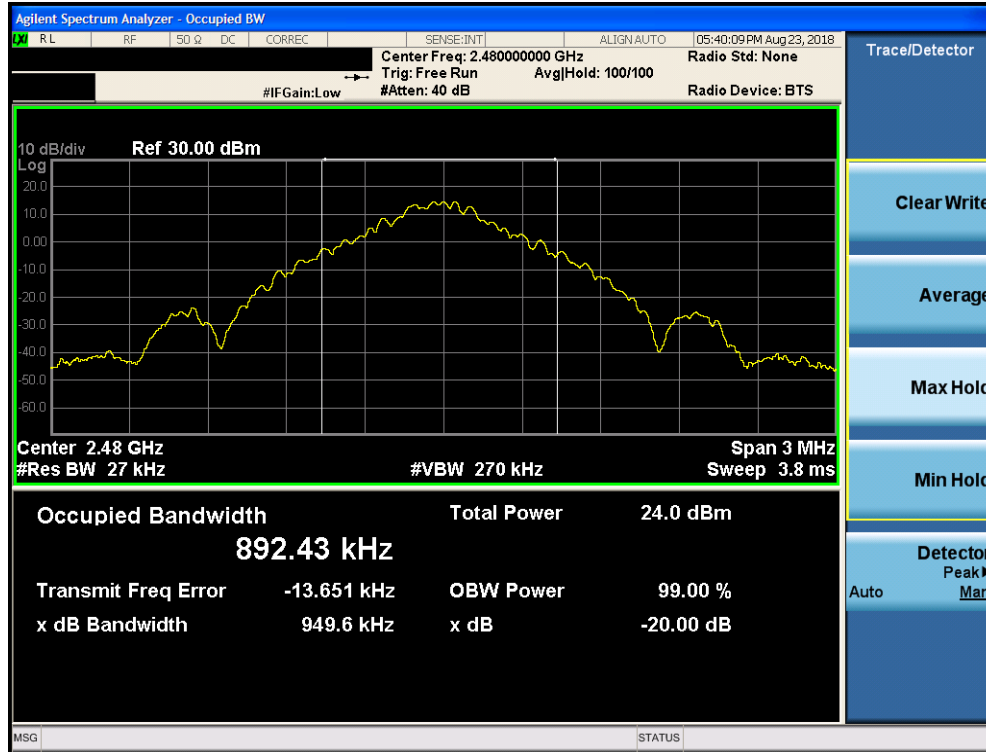
Plot 7-3. 20dB Bandwidth Plot ANT 0 (Bluetooth, GFSK, ePA – Ch. 78)
