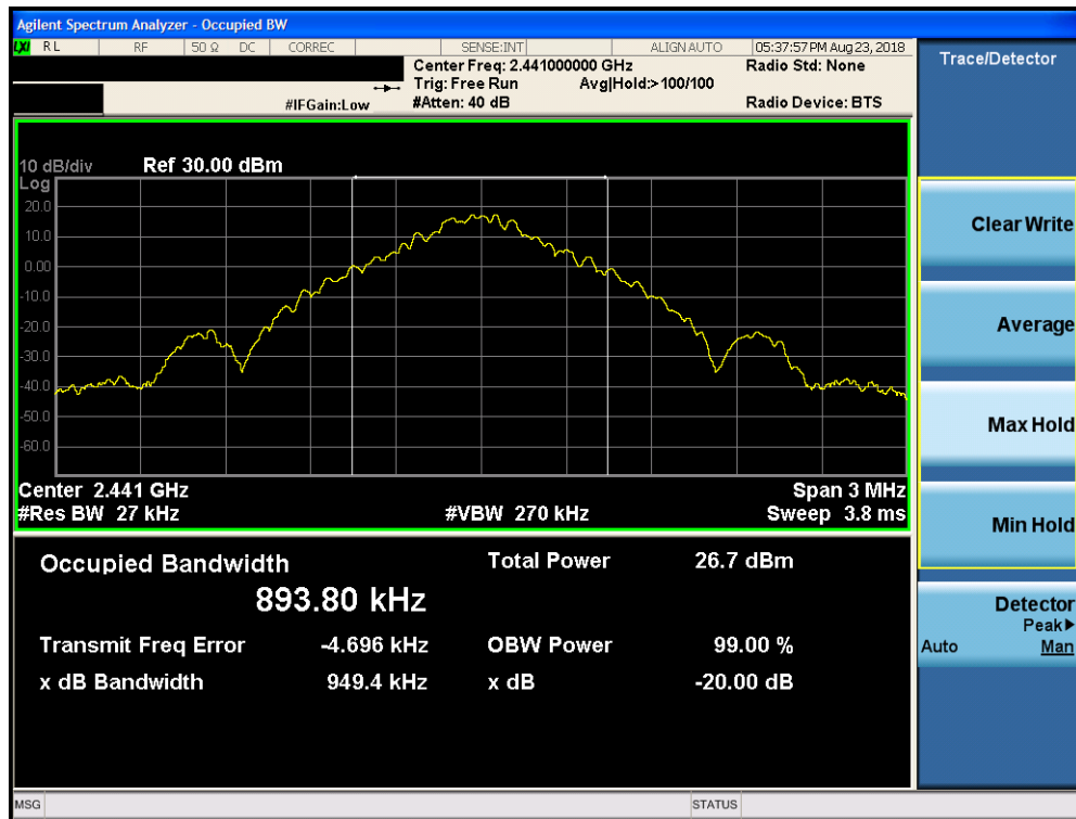
Plot 7-2. 20dB Bandwidth Plot ANT 0 (Bluetooth, GFSK, ePA – Ch. 39)
