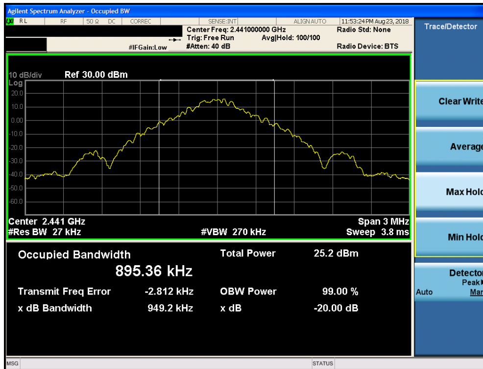
Plot 7-14. 20dB Bandwidth Plot ANT 2 (Bluetooth, GFSK, ePA – Ch. 39)
