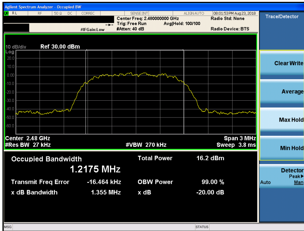
Plot 7-12. 20dB Bandwidth Plot ANT 1 (Bluetooth, 8DPSK, ePA – Ch. 78)
