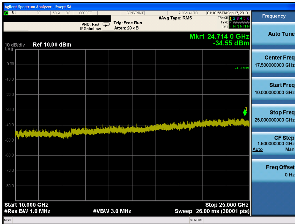
Plot 7-78. Conducted Spurious Plot ANT 1 (Bluetooth, GFSK, ePA – Ch. 78)
