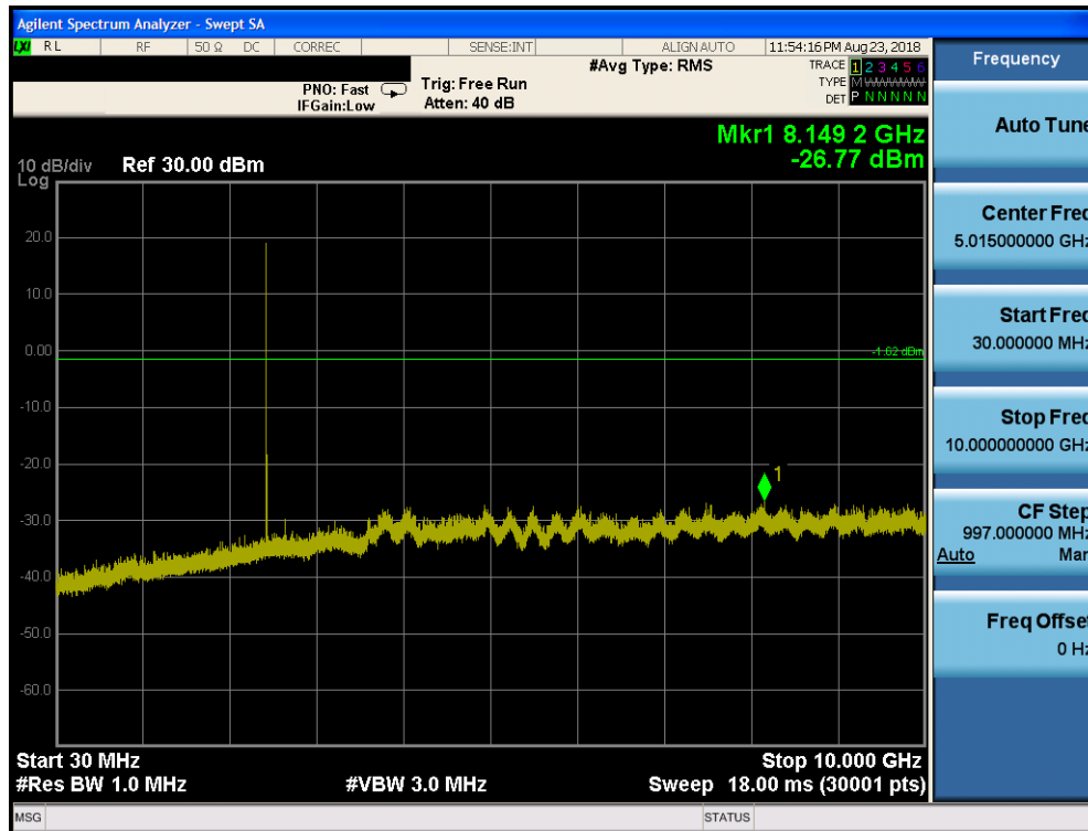
Plot 7-81. Conducted Spurious Plot ANT 2 (Bluetooth, GFSK, ePA – Ch. 39)
