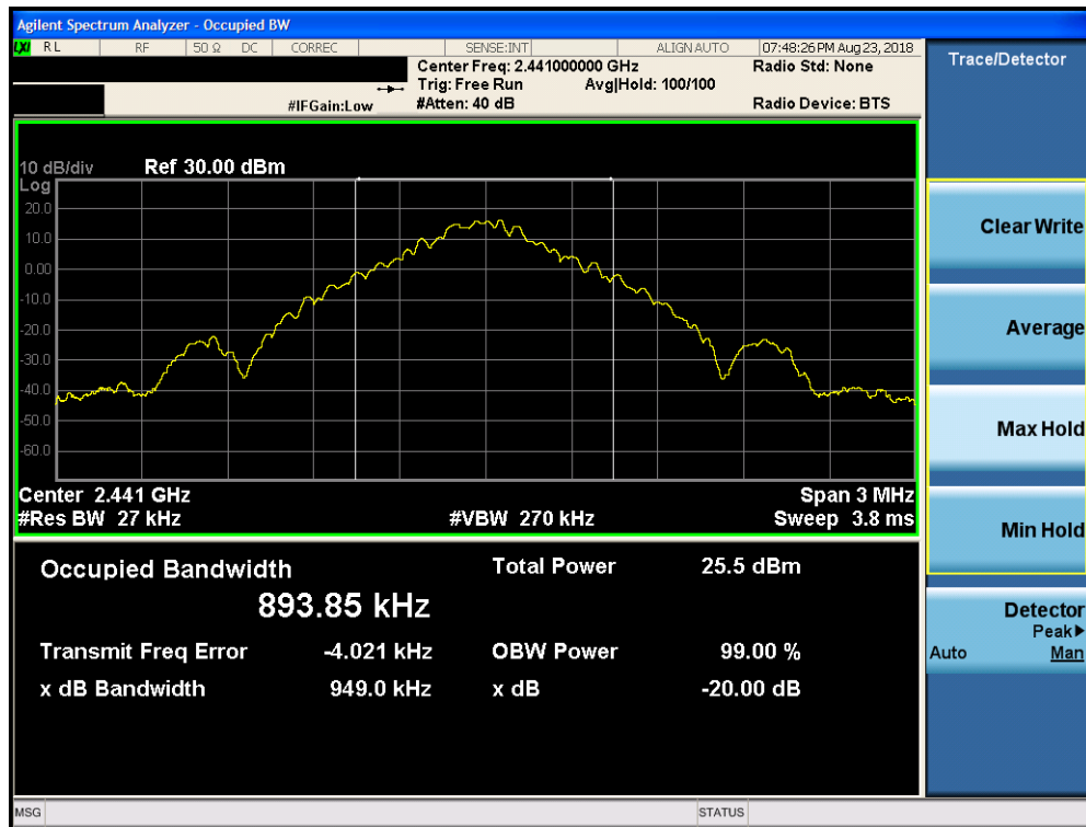
Plot 7-8. 20dB Bandwidth Plot ANT 1 (Bluetooth, GFSK, ePA – Ch. 39)
