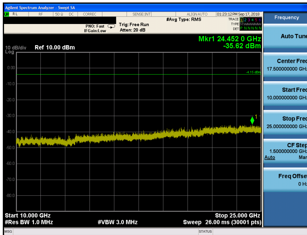
Plot 7-84. Conducted Spurious Plot ANT 2 (Bluetooth, GFSK, ePA – Ch. 78)
