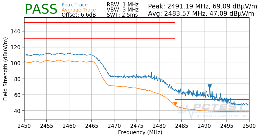
Plot 7-173. Radiated Restricted Upper Band Edge Measurement CDD Primary
