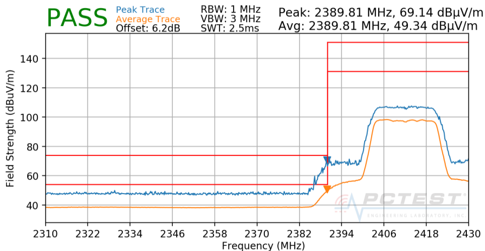
Plot 7-177. Radiated Restricted Lower Band Edge Measurement CDD Diversity
