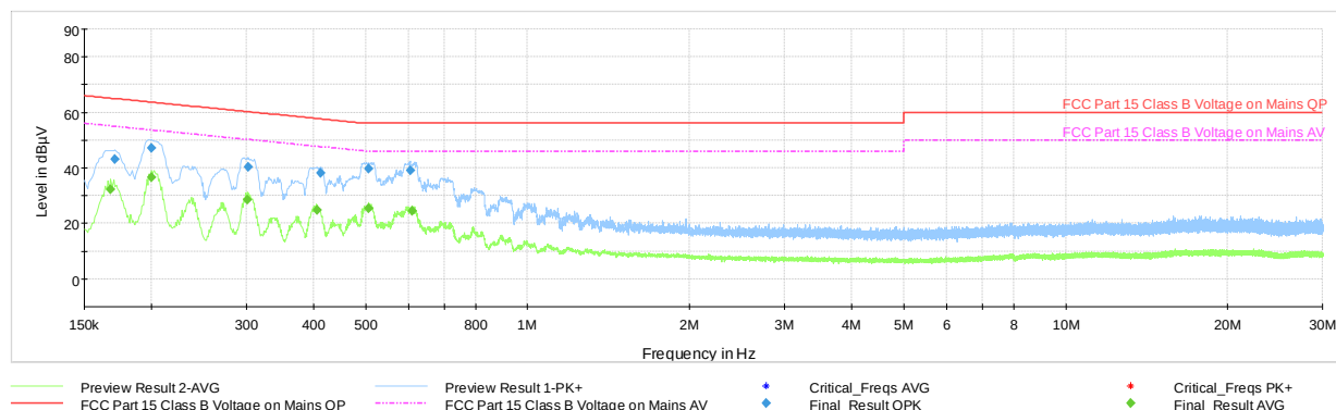
Plot 7-185. Line Conducted Plot with 802.11n CDD Primary (N, with AC/DC Adapter)
