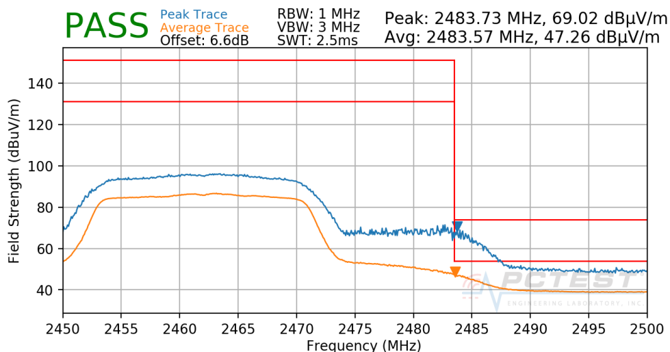
Plot 7-168. Radiated Restricted Upper Band Edge Measurement SISO CORE1 DIVERSITY
