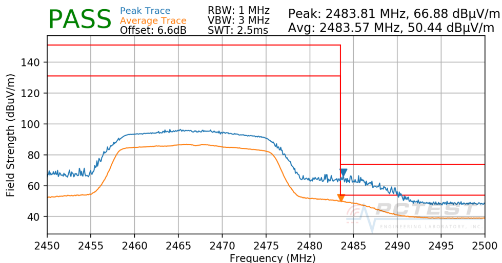
Plot 7-169. Radiated Restricted Upper Band Edge Measurement SISO CORE1 DIVERSITY
