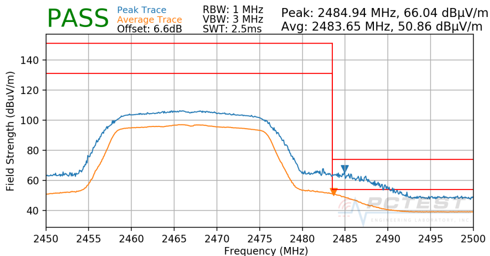
Plot 7-181. Radiated Restricted Upper Band Edge Measurement CDD Diversity
