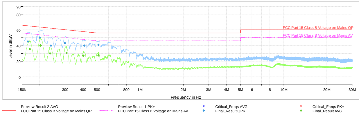
Plot 7-184. Line Conducted Plot with 802.11n CDD Primary (L1, with AC/DC Adapter)
