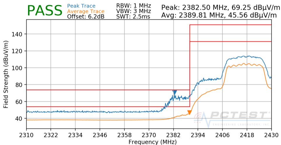
Plot 7-172. Radiated Restricted Lower Band Edge Measurement CDD Primary
