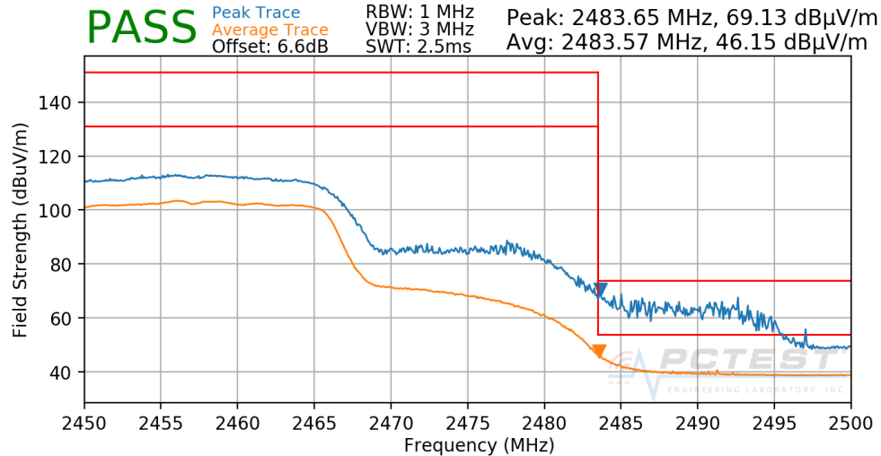
Plot 7-179. Radiated Restricted Upper Band Edge Measurement CDD Diversity
