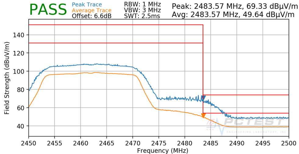
Plot 7-180. Radiated Restricted Upper Band Edge Measurement CDD Diversity
