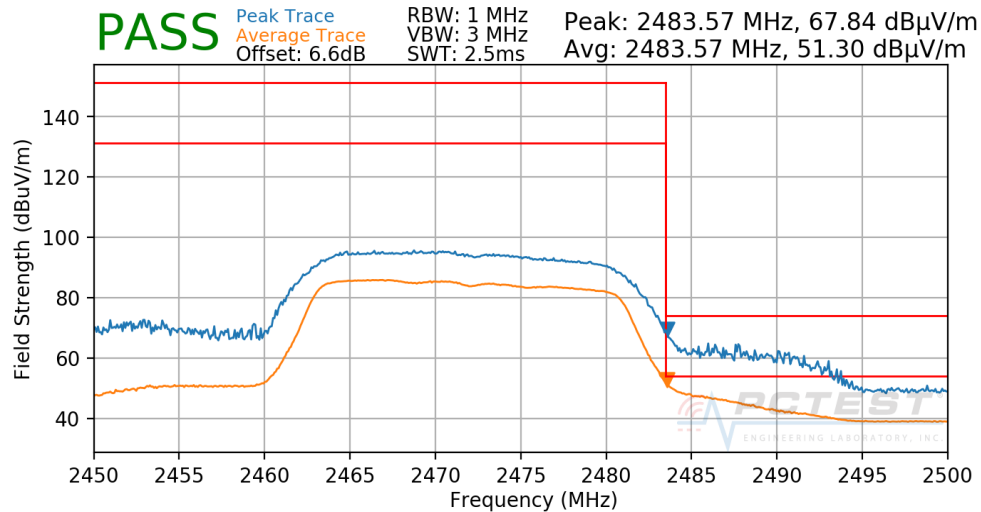
Plot 7-170. Radiated Restricted Upper Band Edge Measurement SISO CORE1 DIVERSITY
