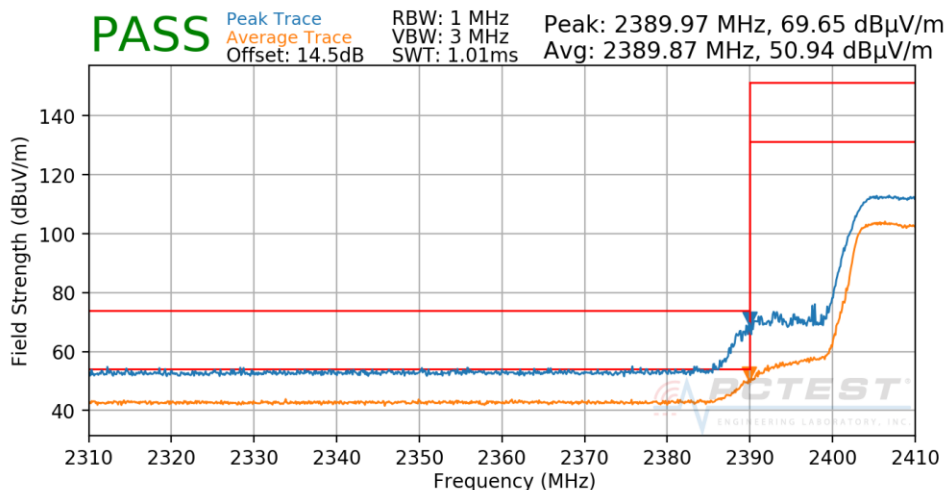
Plot 7-171. Radiated Restricted Lower Band Edge Measurement CDD Primary
