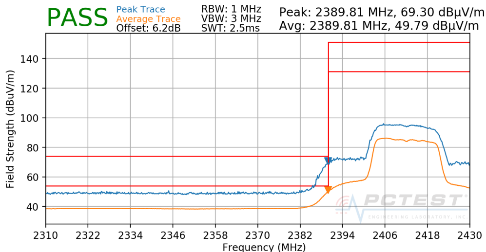
Plot 7-166. Radiated Restricted Lower Band Edge Measurement SISO CORE1 DIVERSITY
