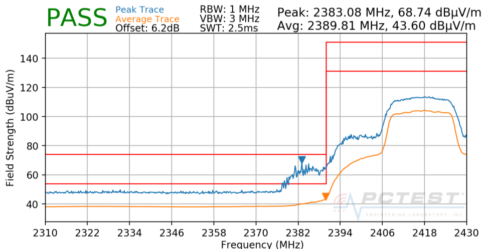
Plot 7-178. Radiated Restricted Lower Band Edge Measurement CDD Diversity
