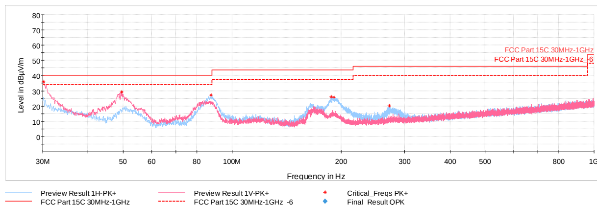
Plot 7-183. Radiated Spurious Plot below 1GHz CDD Primary
