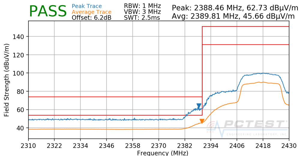
Plot 7-167. Radiated Restricted Lower Band Edge Measurement SISO CORE1 DIVERSITY
