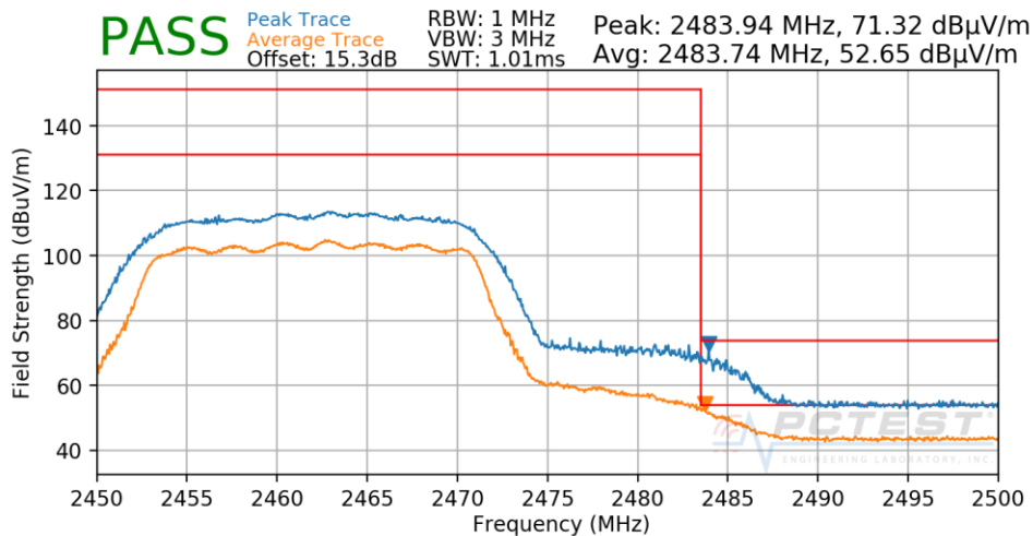
Plot 7-174. Radiated Restricted Upper Band Edge Measurement CDD Primary
