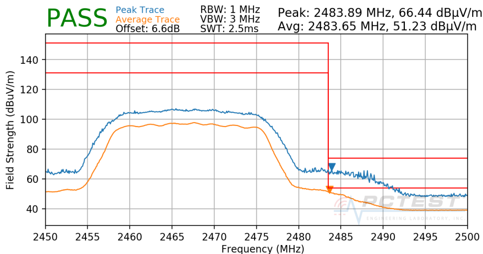
Plot 7-175. Radiated Restricted Upper Band Edge Measurement CDD Primary
