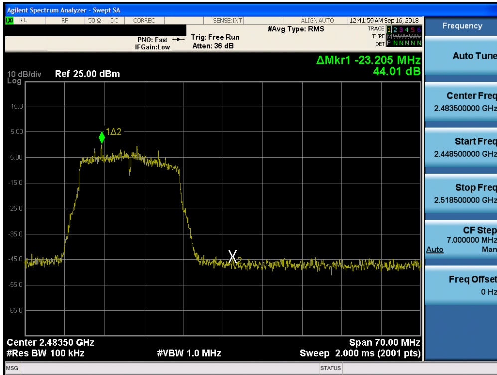
Plot 7-89. Band Edge Plot SISO CORE0 (802.11n – Ch. 12)
