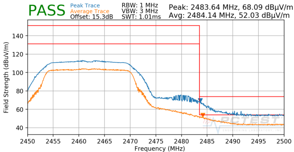
Plot 7-161. Radiated Restricted Upper Band Edge Measurement SISO CORE1 PRIMARY
