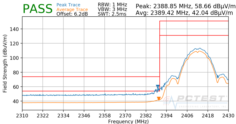
Plot 7-150. Radiated Restricted Lower Band Edge Measurement SISO CORE0
