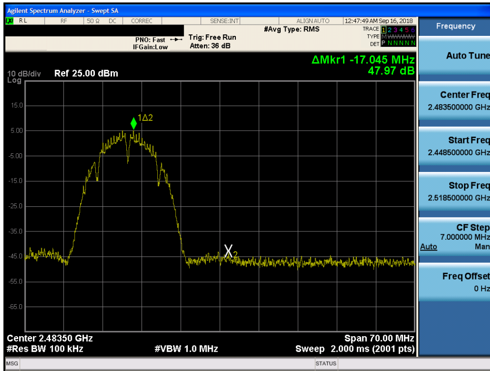
Plot 7-93. Band Edge Plot SISO CORE1 PRIMARY (802.11b – Ch. 12)
