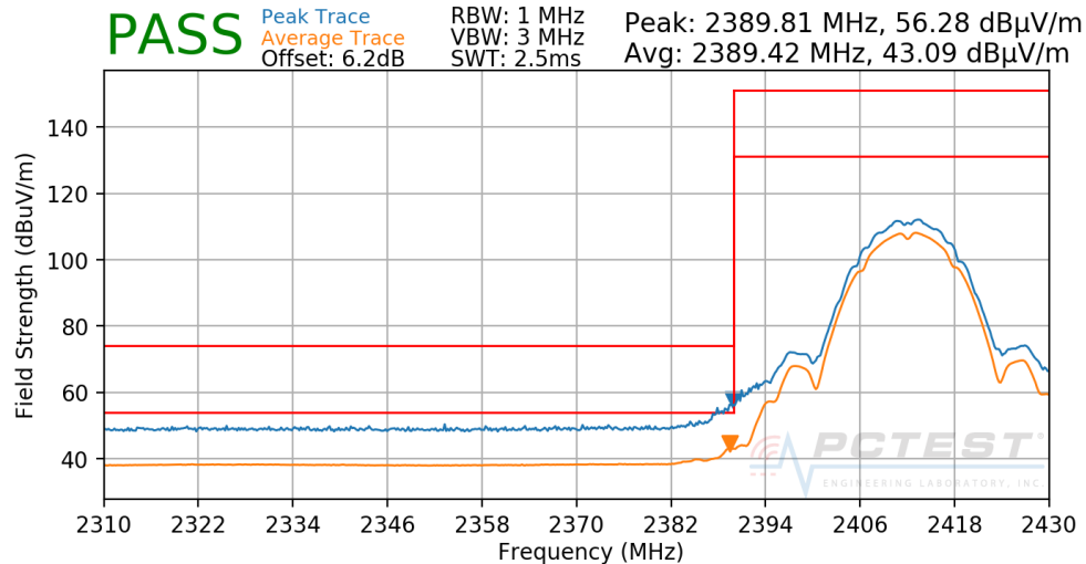
Plot 7-157. Radiated Restricted Lower Band Edge Measurement SISO CORE1 PRIMARY
