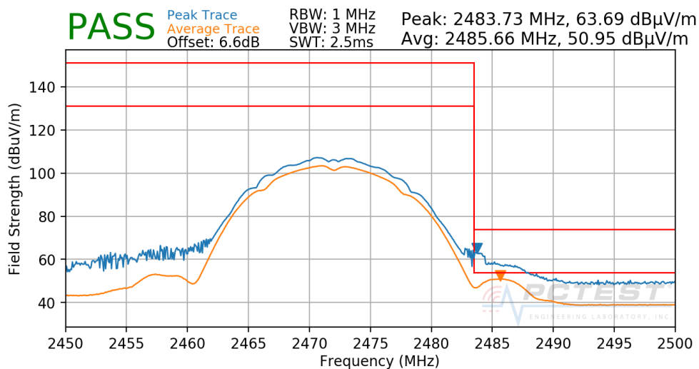
Plot 7-152. Radiated Restricted Upper Band Edge Measurement SISO CORE0
