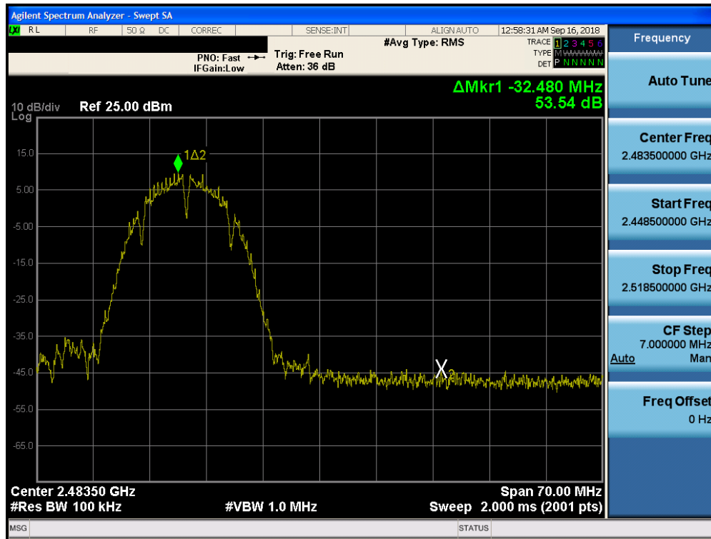
Plot 7-105. Band Edge Plot SISO CORE1 DIVERSITY (802.11b – Ch. 12)
