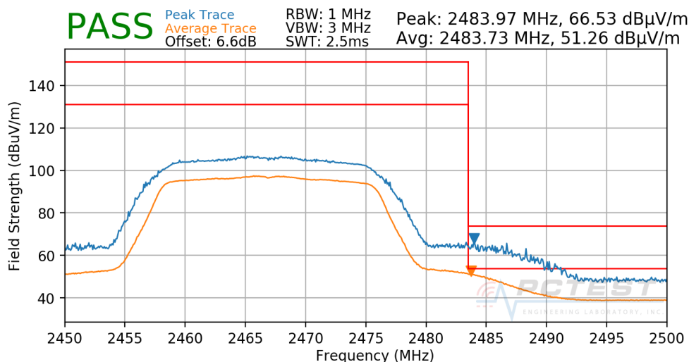
Plot 7-155. Radiated Restricted Upper Band Edge Measurement SISO CORE0
