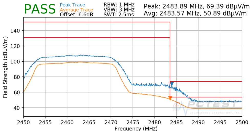
Plot 7-154. Radiated Restricted Upper Band Edge Measurement SISO CORE0
