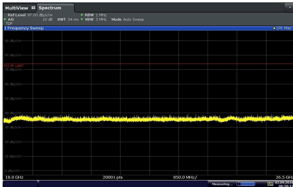
Plot 7-149. Radiated Spurious Plot above 18GHz CDD Primary (802.11n, Pol. V)
