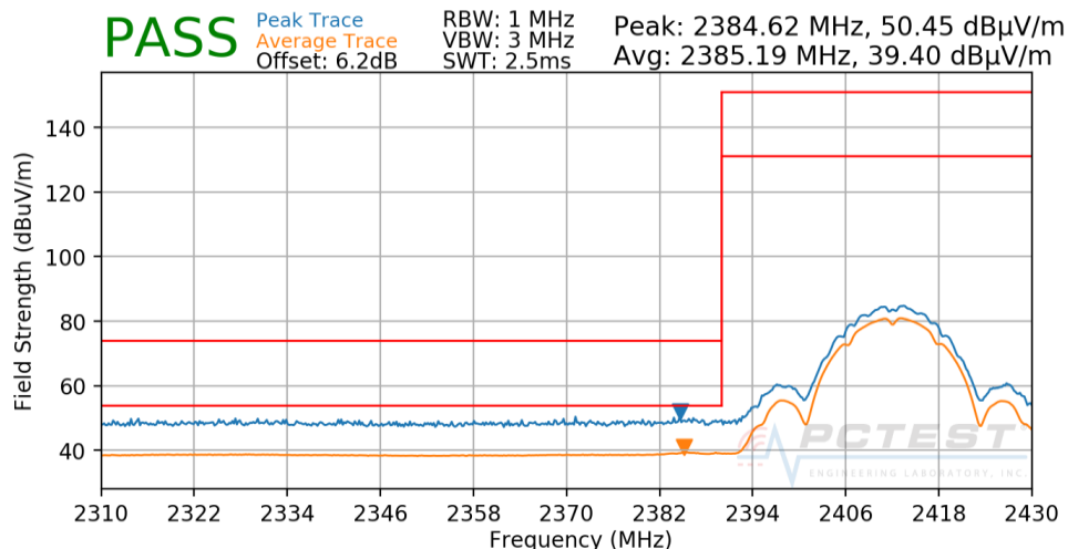
Plot 7-164. Radiated Restricted Lower Band Edge Measurement SISO CORE1 DIVERSITY
