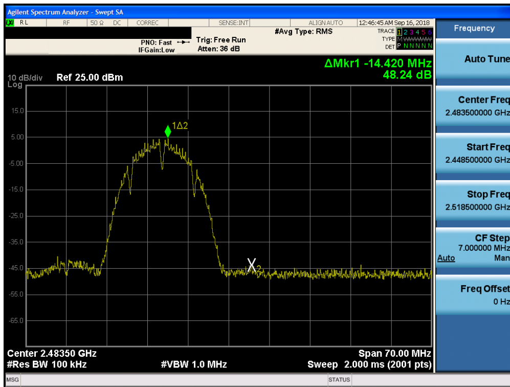
Plot 7-94. Band Edge Plot SISO CORE1 PRIMARY (802.11b – Ch. 13)
