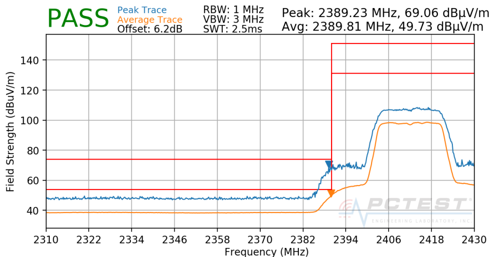
Plot 7-153. Radiated Restricted Lower Band Edge Measurement SISO CORE0
