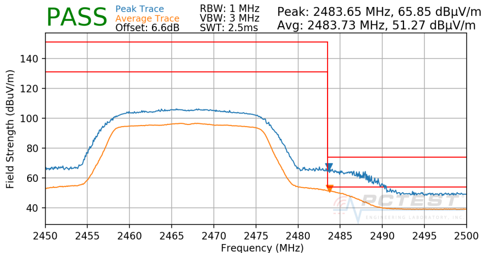
Plot 7-162. Radiated Restricted Upper Band Edge Measurement SISO CORE1 PRIMARY
