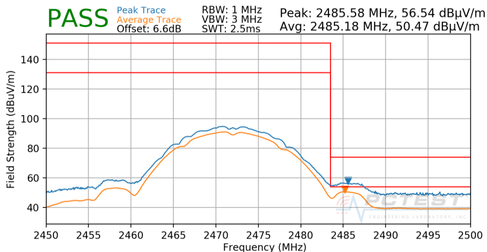
Plot 7-165. Radiated Restricted Upper Band Edge Measurement SISO CORE1 DIVERSITY
