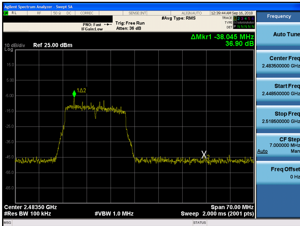
Plot 7-90. Band Edge Plot SISO CORE0 (802.11n – Ch. 13)
