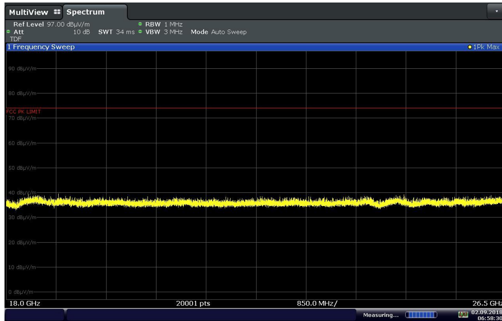
Plot 7-148. Radiated Spurious Plot above 18GHz CDD Primary (802.11n, Pol. H)
