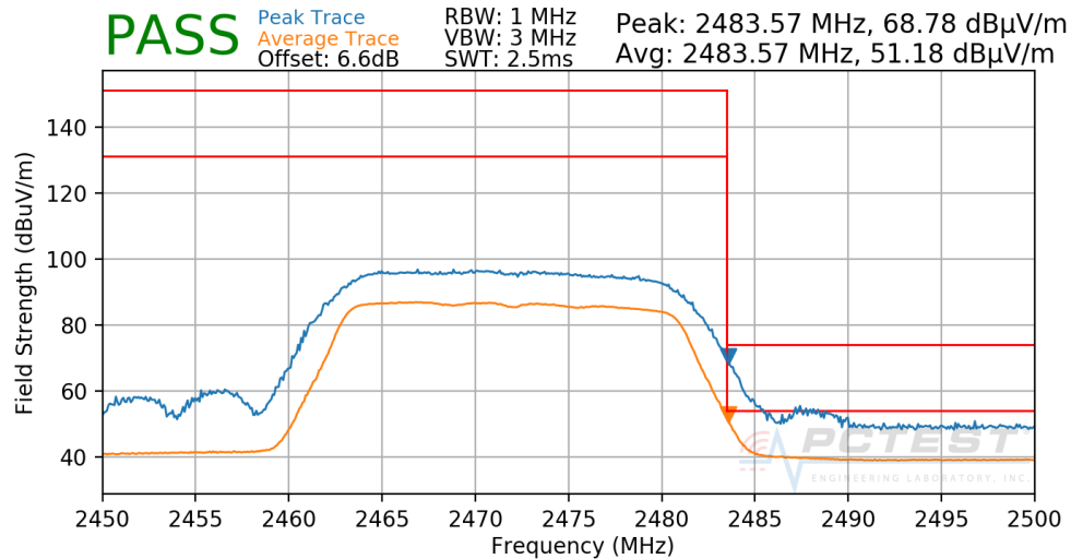
Plot 7-163. Radiated Restricted Upper Band Edge Measurement SISO CORE1 PRIMARY
