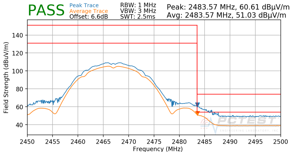
Plot 7-151. Radiated Restricted Upper Band Edge Measurement SISO CORE0
