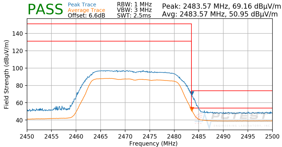
Plot 7-156. Radiated Restricted Upper Band Edge Measurement SISO CORE0
