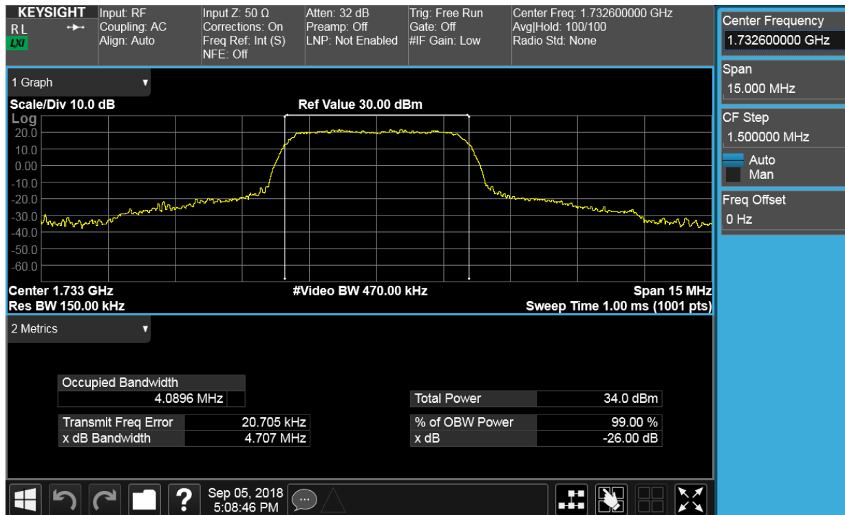
Plot 7-6. Occupied Bandwidth Plot (AWS WCDMA Mode)
