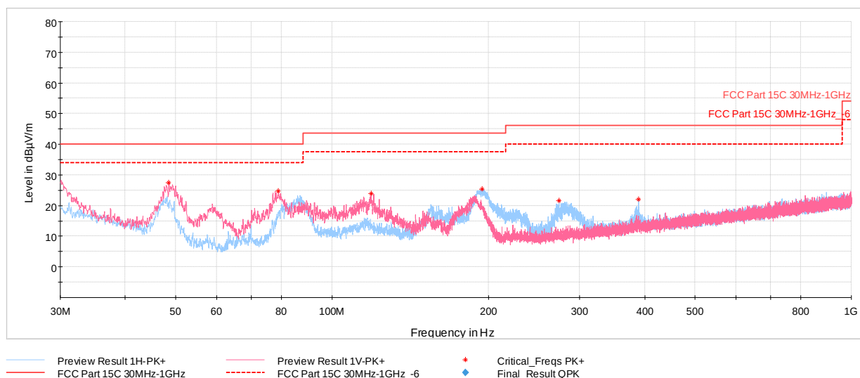
Plot 7-4. Radiated Spurious Plot above 30MHz (Pol. H & V)
