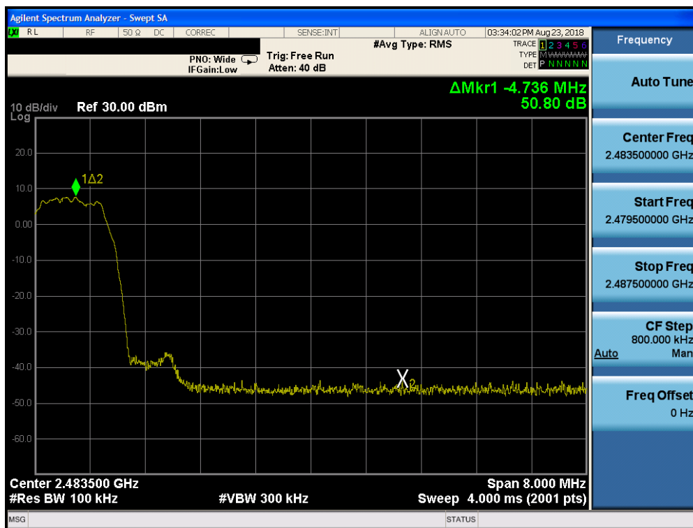
Plot 7-32. Band Edge Plot ANT1 (Bluetooth with Hopping Disabled, 8DPSK, ePA – Ch. 78)
