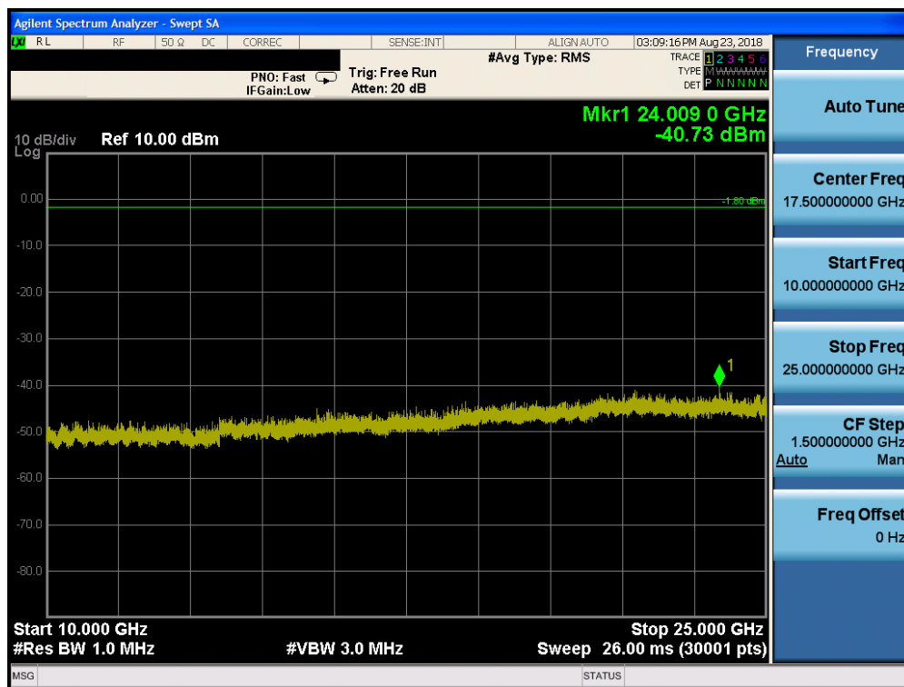
Plot 7-76. Conducted Spurious Plot ANT1 (Bluetooth, GFSK, ePA Ch. 39)
