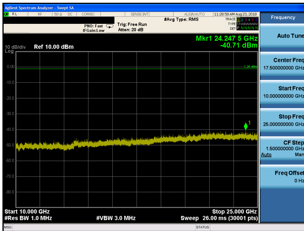
Plot 7-72. Conducted Spurious Plot ANT0 (Bluetooth, GFSK, ePA – Ch. 78)
