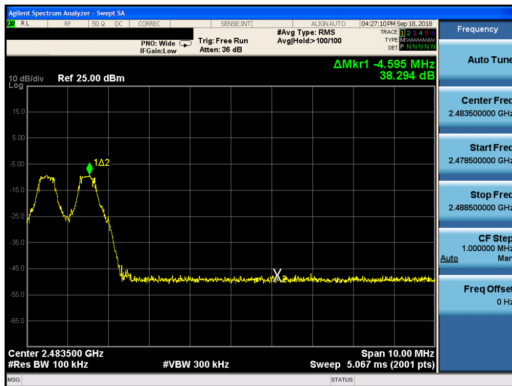
Plot 7-38. Band Edge Plot ANT2 (Bluetooth with Hopping Enabled, GFSK, ePA – Ch. 78)
