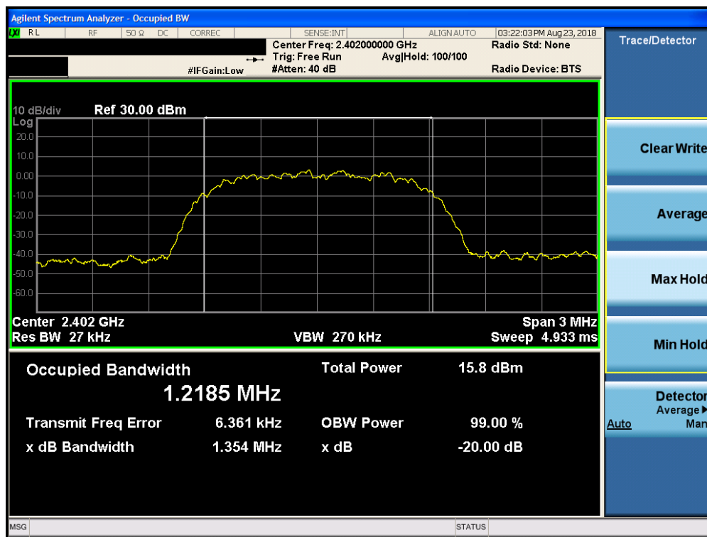
Plot 7-10. 20dB Bandwidth Plot ANT1 (Bluetooth, 8DPSK, ePA – Ch. 0)
