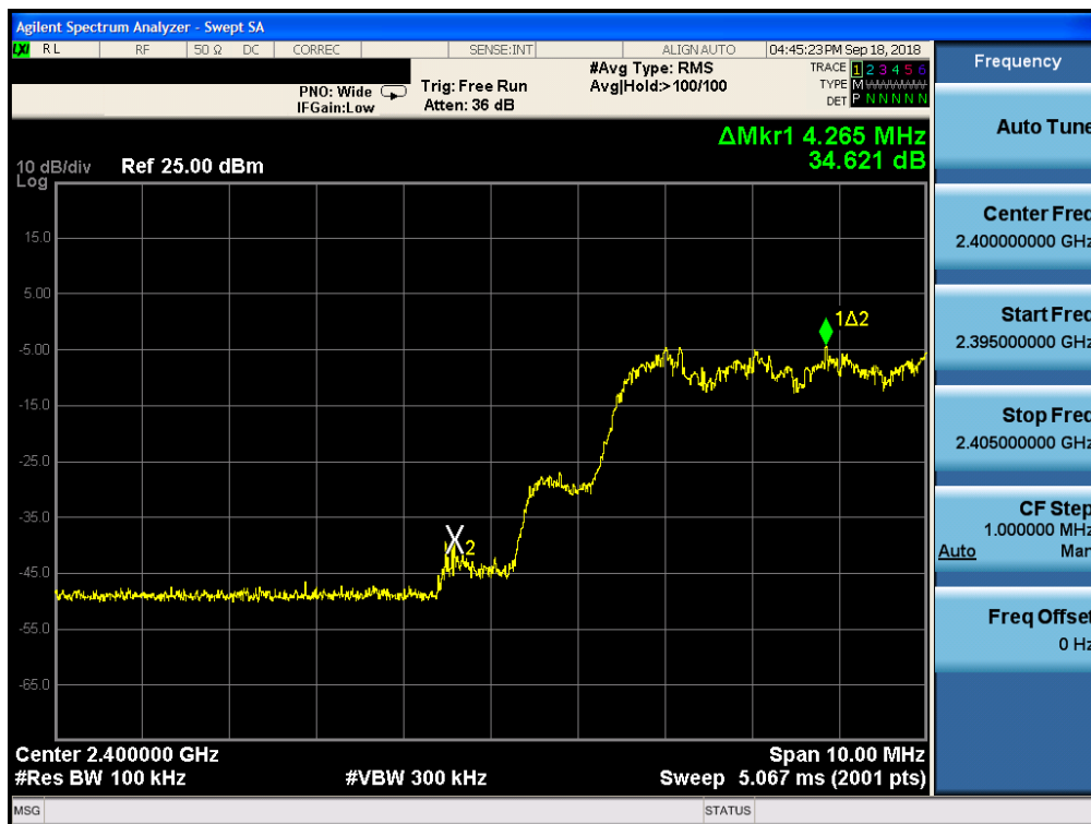
Plot 7-41. Band Edge Plot ANT2 (Bluetooth with Hopping Enabled, 8DPSK, ePA – Ch. 0)
