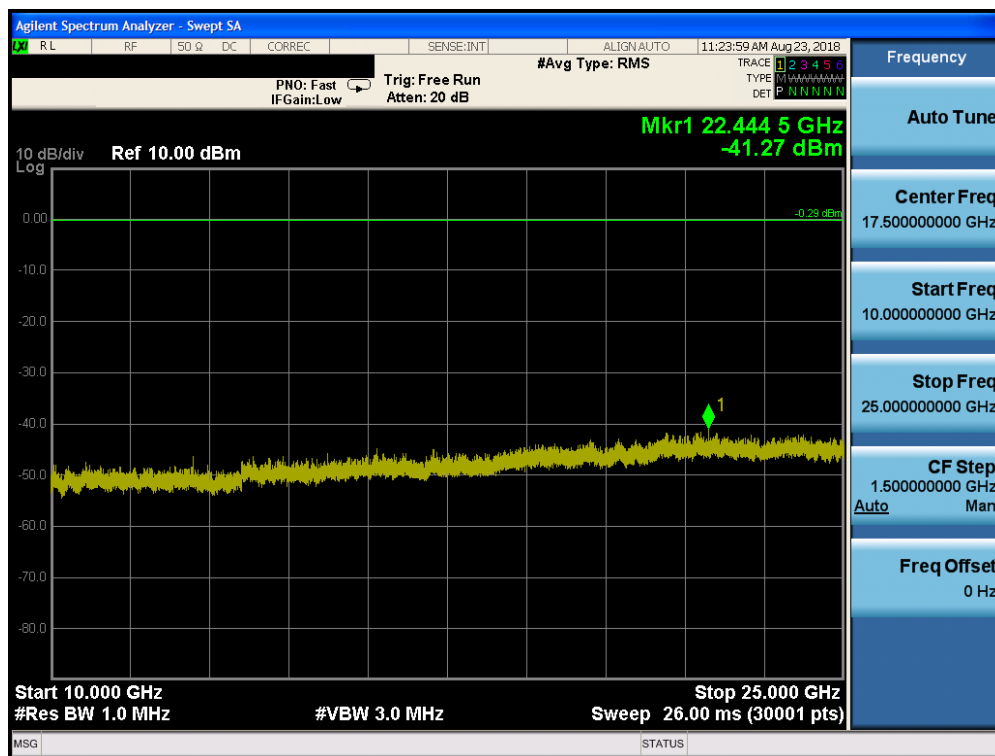
Plot 7-70. Conducted Spurious Plot ANT0 (Bluetooth, GFSK, ePA Ch. 39)
