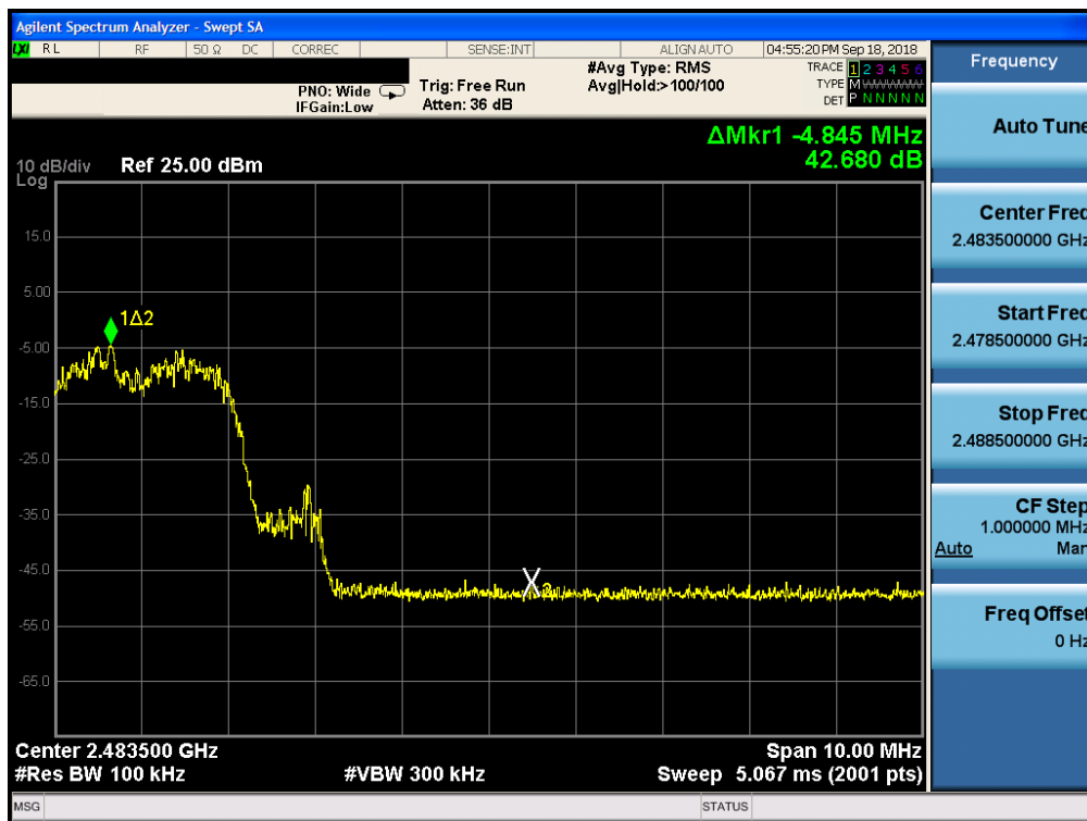
Plot 7-42. Band Edge Plot ANT2 (Bluetooth with Hopping Enabled, 8DPSK, ePA – Ch. 78)
