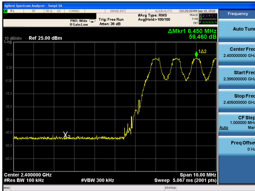
Plot 7-29. Band Edge Plot ANT1 (Bluetooth with Hopping Enabled, GFSK, ePA – Ch. 0)
