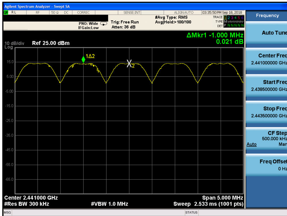
Plot 7-45. Channel Spacing Plot ANT1 (Bluetooth, GFSK, ePA)
