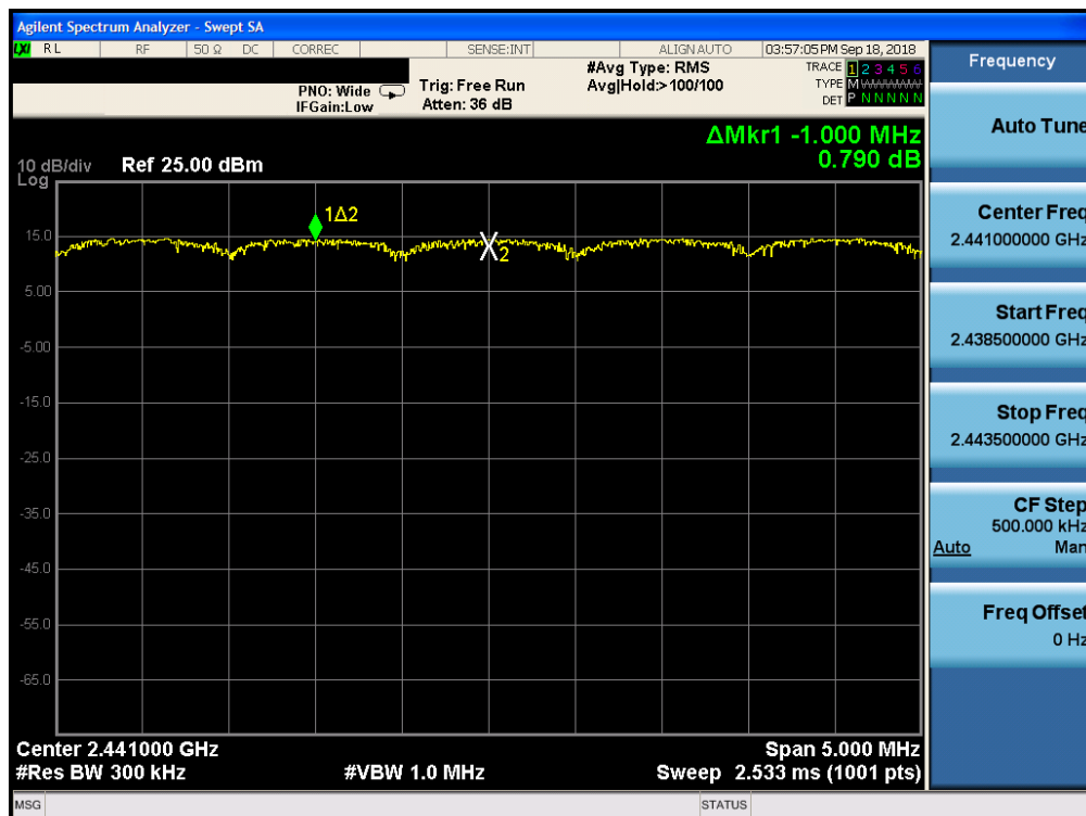
Plot 7-46. Channel Spacing Plot ANT1 (Bluetooth, 8DPSK, ePA)
