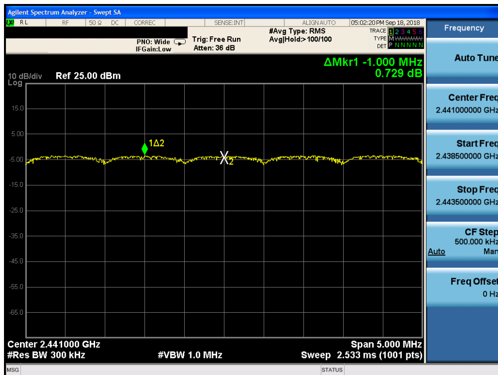
Plot 7-48. Channel Spacing Plot ANT2 (Bluetooth, 8DPSK, ePA)
