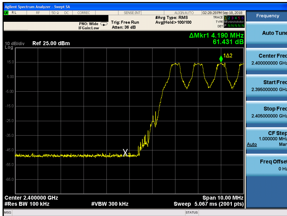
Plot 7-21. Band Edge Plot ANT0 (Bluetooth with Hopping Enabled, GFSK, ePA – Ch. 0)
