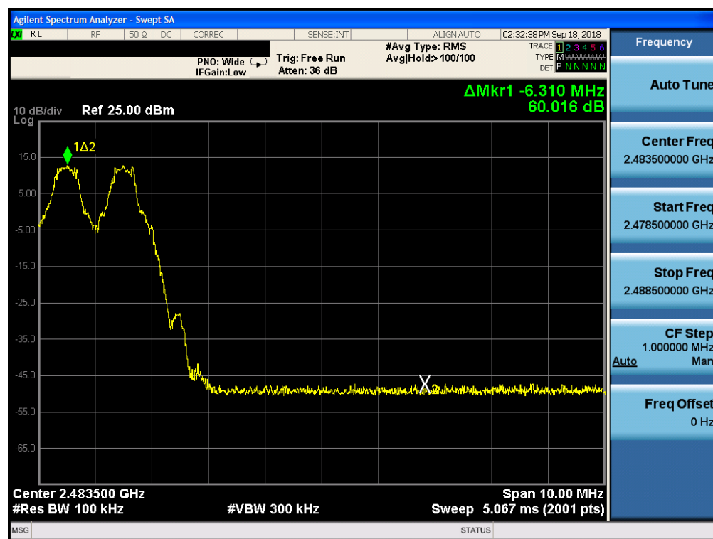
Plot 7-22. Band Edge Plot ANT0 (Bluetooth with Hopping Enabled, GFSK, ePA – Ch. 78)
