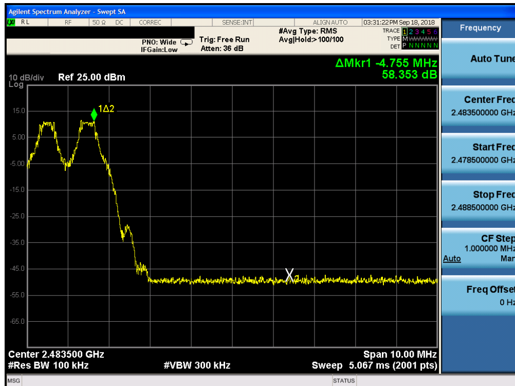
Plot 7-30. Band Edge Plot ANT1 (Bluetooth with Hopping Enabled, GFSK, ePA – Ch. 78)
