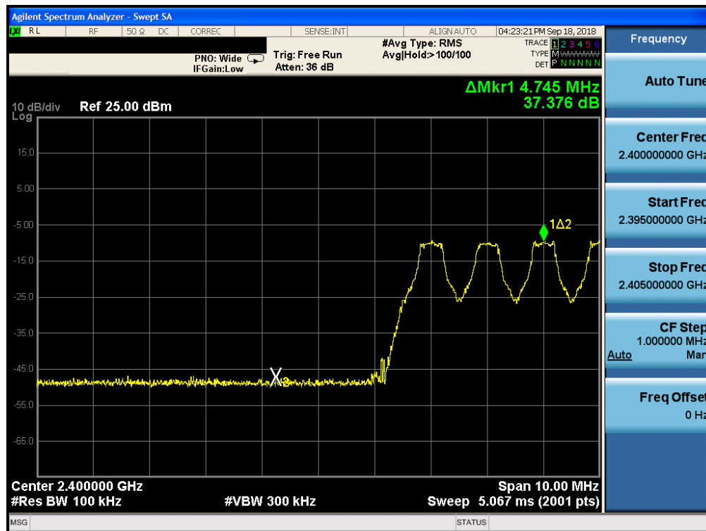
Plot 7-37. Band Edge Plot ANT2 (Bluetooth with Hopping Enabled, GFSK, ePA – Ch. 0)
