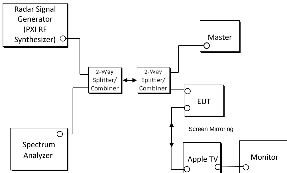
Figure 5-2. Mode-2 Test Setup (Mode 2)
