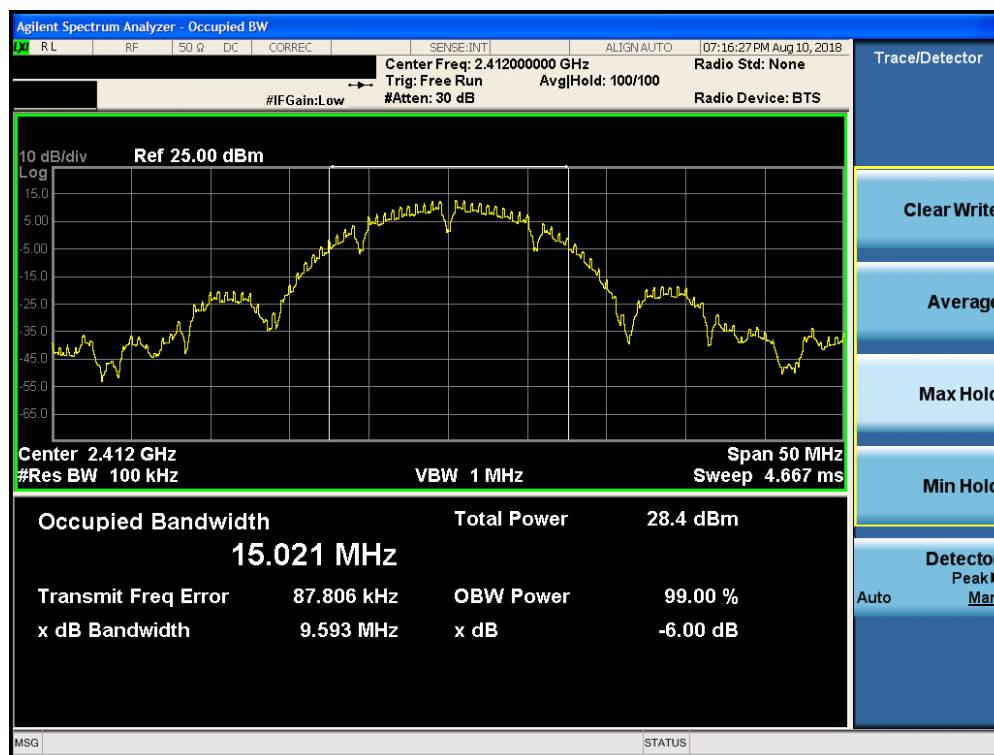
Plot 7-19. 6dB Bandwidth Plot SISO CORE1 DIVERSITY (802.11b - Ch. 1)
