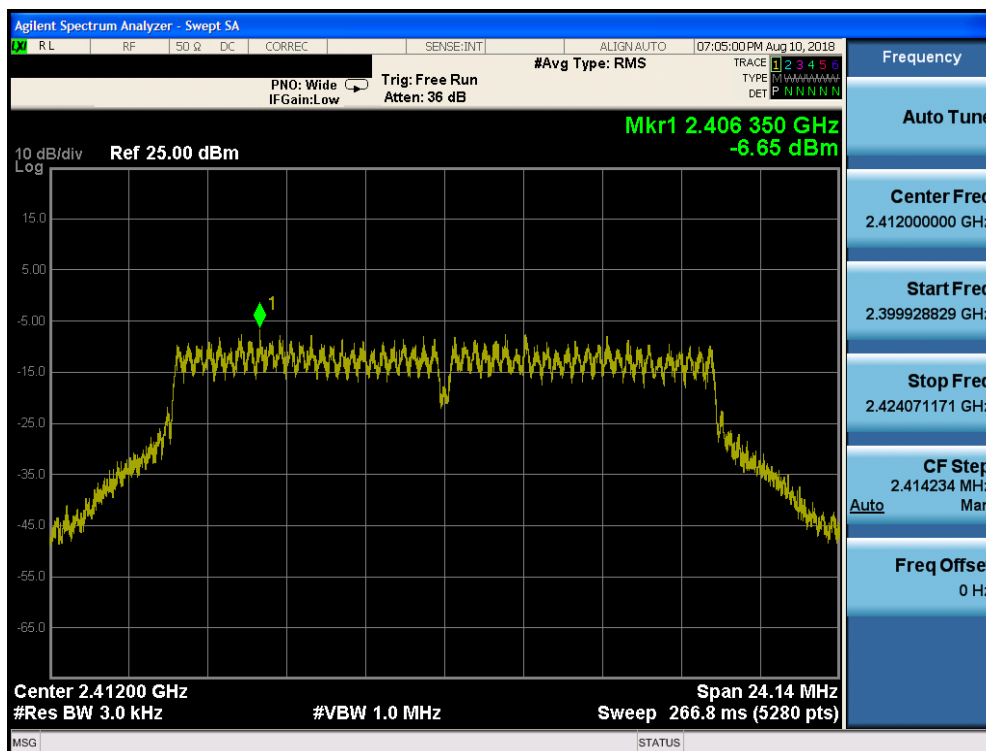
Plot 7-40. Power Spectral Density Plot SISO CORE1 PRIMARY (802.11g – Ch. 1)
