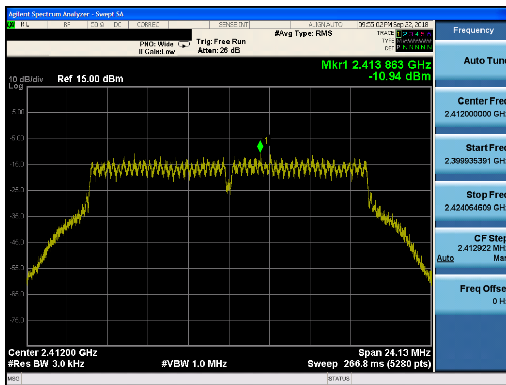
Plot 7-55. Power Spectral Density Plot CDD Core 0 (802.11g – Ch. 1)
