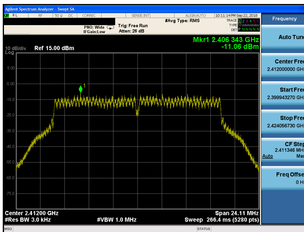
Plot 7-67. Power Spectral Density Plot CDD Core 0 (802.11g - Ch. 1)
