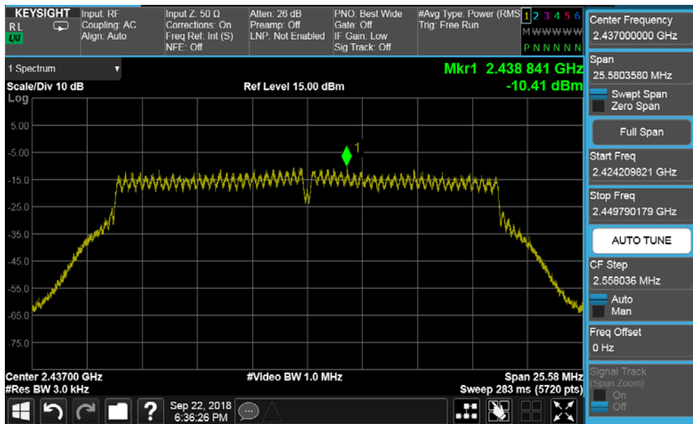
Plot 7-63. Power Spectral Density Plot CDD Core 0 (802.11n – Ch. 6)
