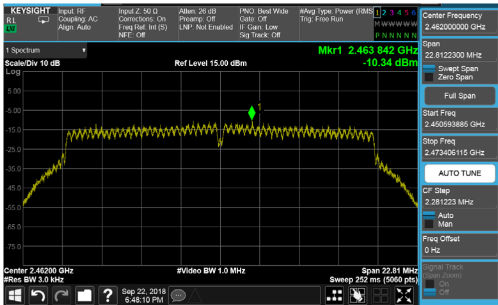
Plot 7-65. Power Spectral Density Plot CDD Core 0 (802.11n – Ch. 11)
