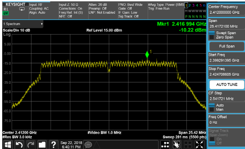
Plot 7-61. Power Spectral Density Plot CDD Core 0 (802.11n – Ch. 1)
