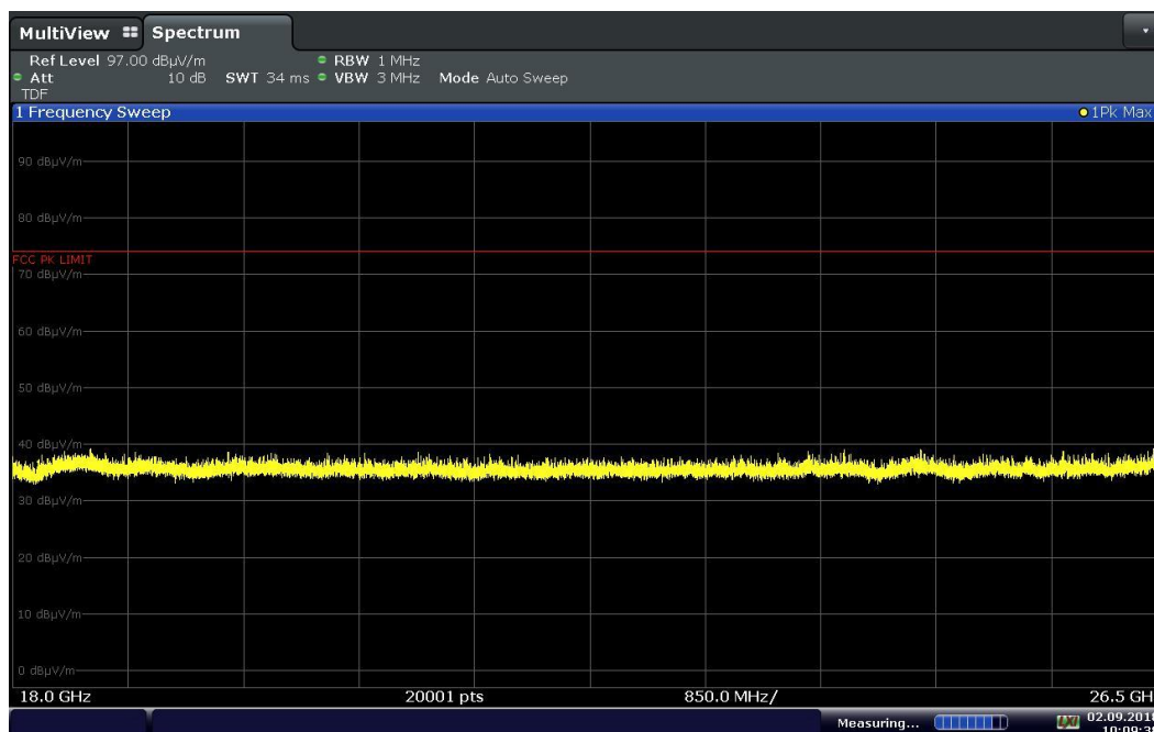
Plot 7-104. Radiated Spurious Plot above 18GHz ANT0 (8Mbps, HDR8 ePA – Ch. 38, Ant. Pol. V)
