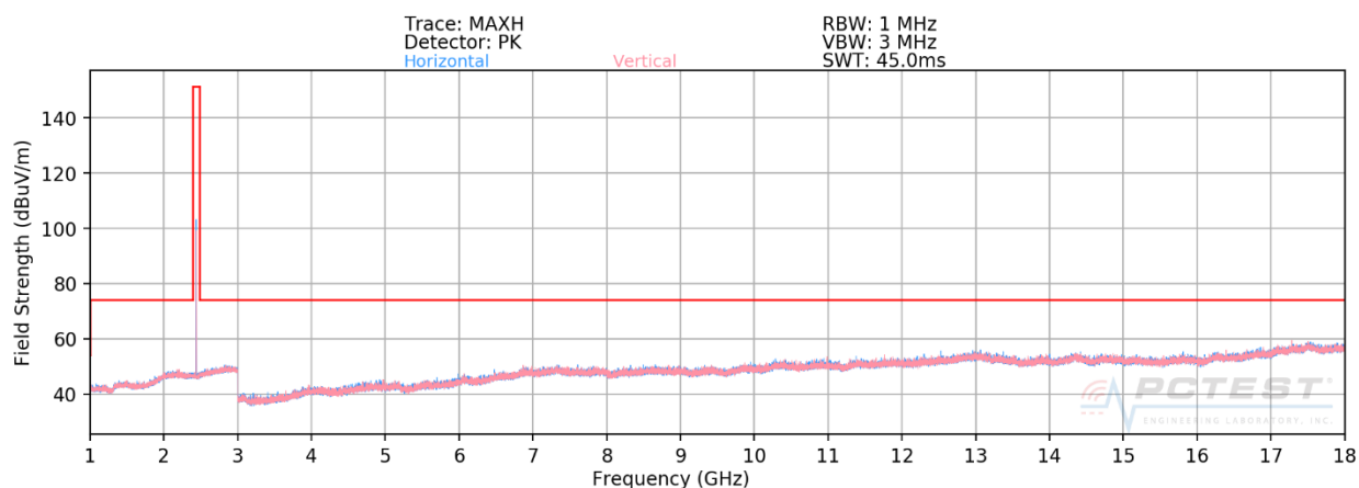
Plot 7-86. Radiated Spurious Plot ANT0 (4Mbps, HDR4, ePA – Ch. 38, Ant. Pol. H & V)
