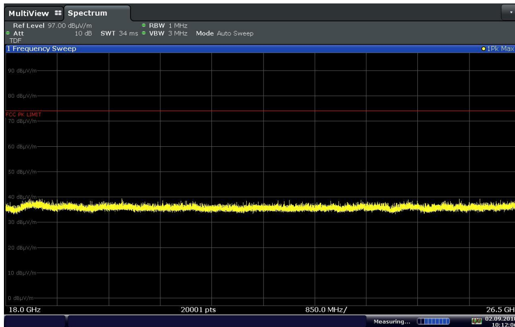
Plot 7-103. Radiated Spurious Plot above 18GHz ANT0 (8Mbps, HDR8 ePA – Ch. 38, Ant. Pol. H)
