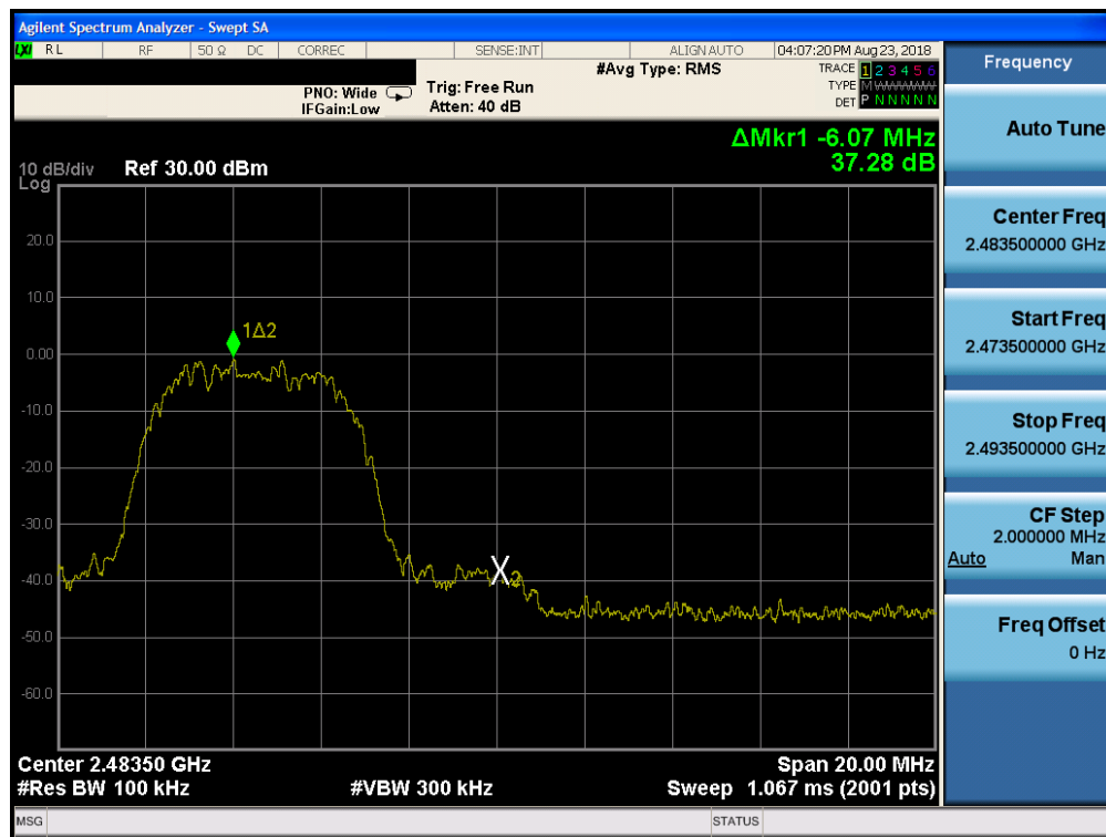
Plot 7-62. Band Edge Plot ANT1 (Bluetooth (HDR8, ePA), 8Mbps – Ch. 75)
