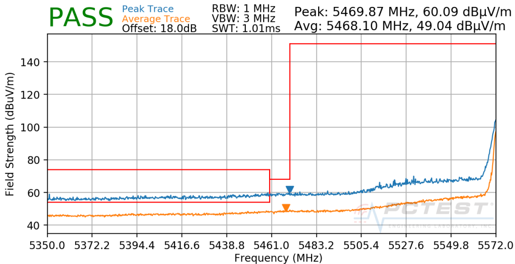
Plot 7-262. Radiated Lower Band Edge Plot SISO CORE1 (UNII Band 2C)
