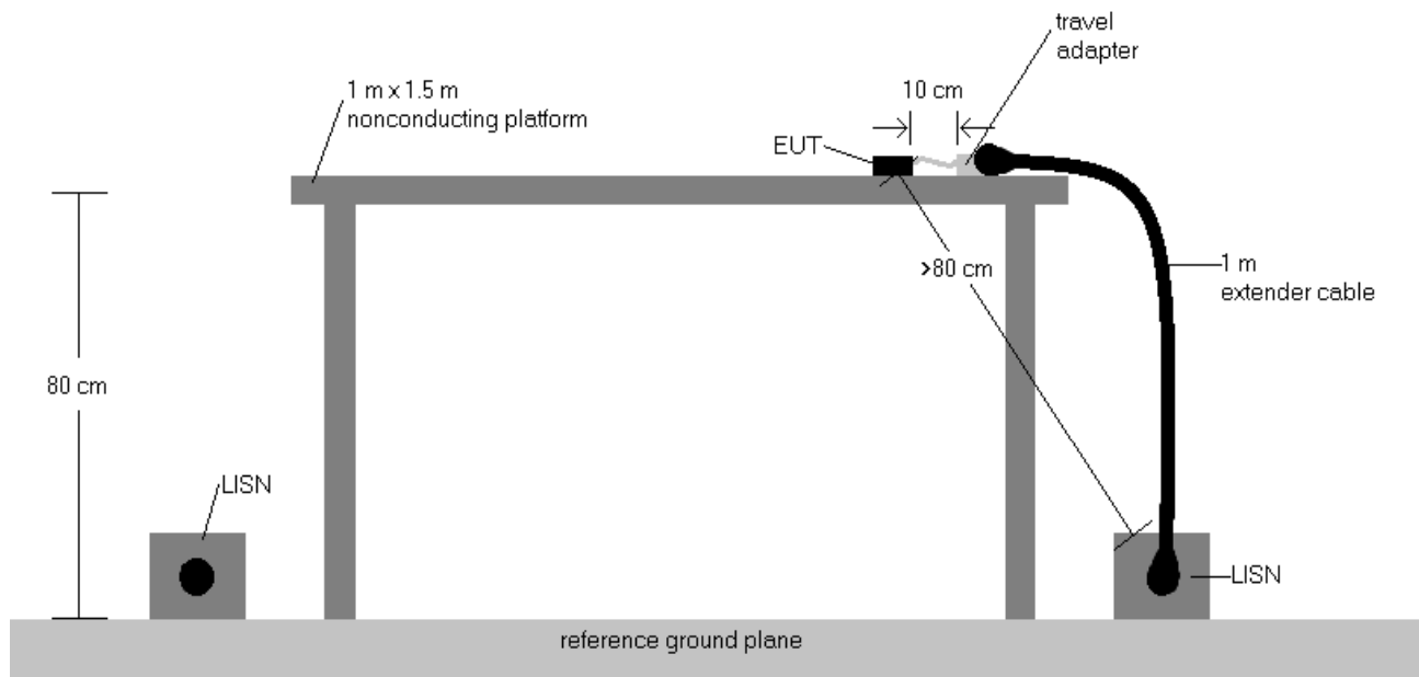
Figure 7-8. Test Instrument & Measurement Setup
