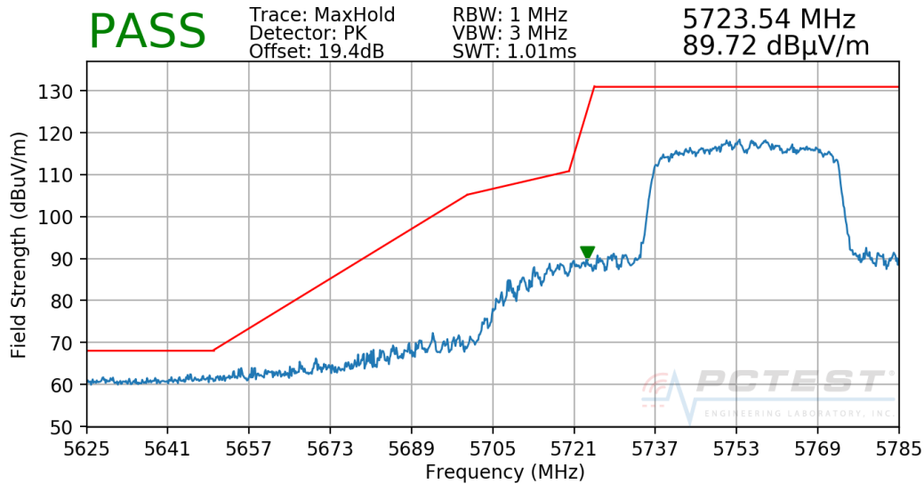
Plot 7-283. Radiated Lower Band Edge Plot CDD (Peak - UNII Band 3)
