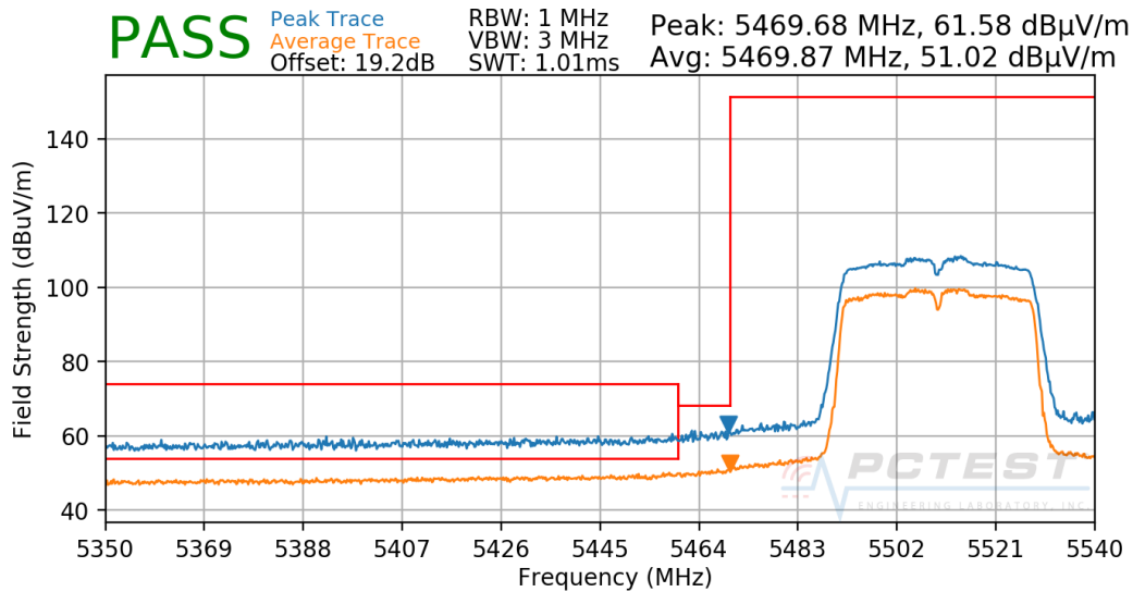
Plot 7-253. Radiated Lower Band Edge Plot SISO CORE1 (UNII Band 2C)
