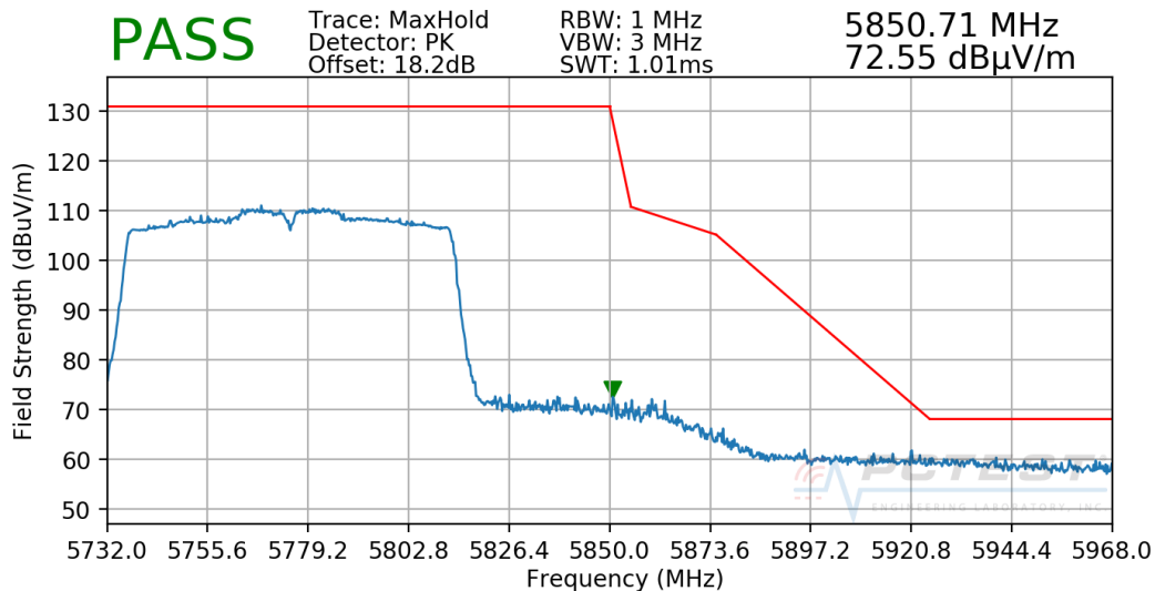
Plot 7-264. Radiated Upper Band Edge Plot SISO CORE1 (Peak – UNII Band 3)
