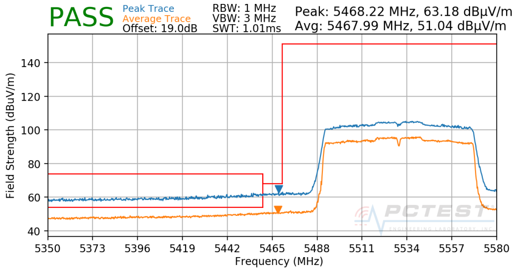
Plot 7-261. Radiated Lower Band Edge Plot SISO CORE1 (UNII Band 2C)
