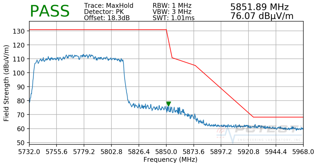
Plot 7-290. Radiated Upper Band Edge Plot CDD (Peak - UNII Band 3)
