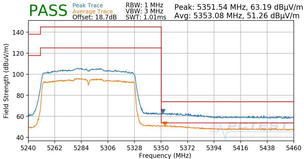
Plot 7-260. Radiated Upper Band Edge Plot SISO CORE1 (UNII Band 2A)
