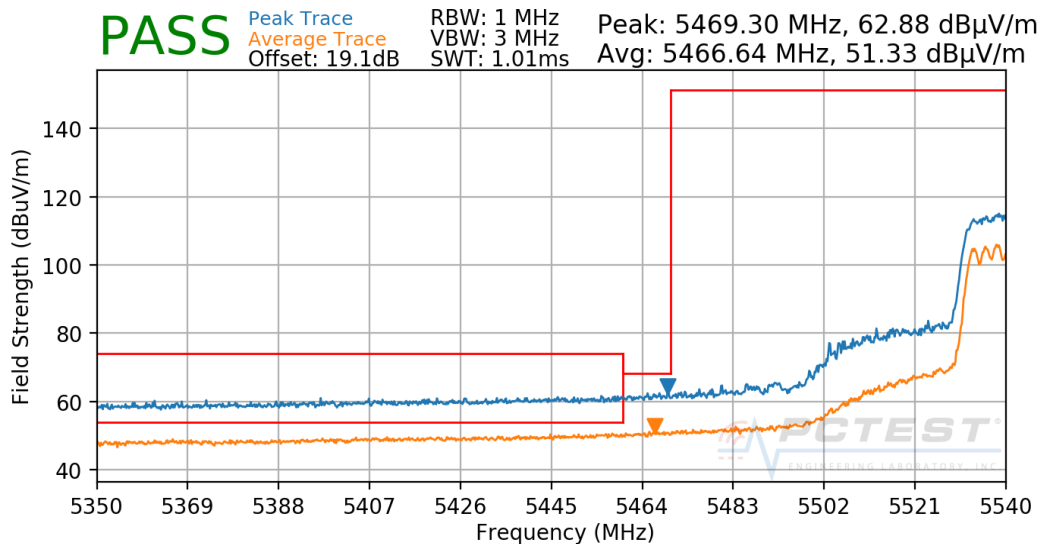
Plot 7-280. Radiated Lower Band Edge Plot CDD (Peak - UNII Band 2C)
