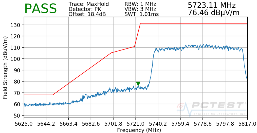
Plot 7-289. Radiated Lower Band Edge Plot CDD (Peak - UNII Band 3)
