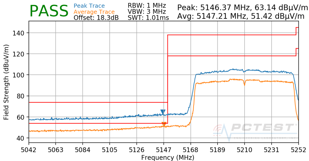
Plot 7-259. Radiated Lower Band Edge Plot SISO CORE1 (UNII Band 1)
