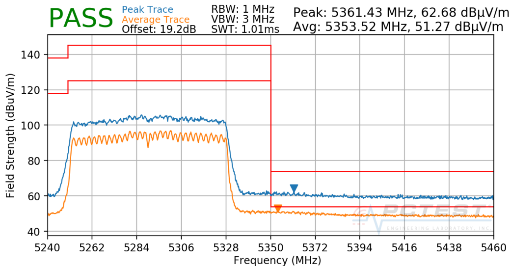
Plot 7-286. Radiated Upper Band Edge Plot CDD (UNII Band 2A)
