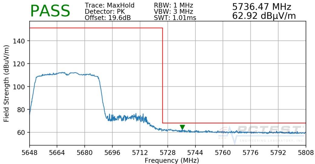
Plot 7-256. Radiated Upper Band Edge Plot SISO CORE1 (Peak - UNII Band 2C)
