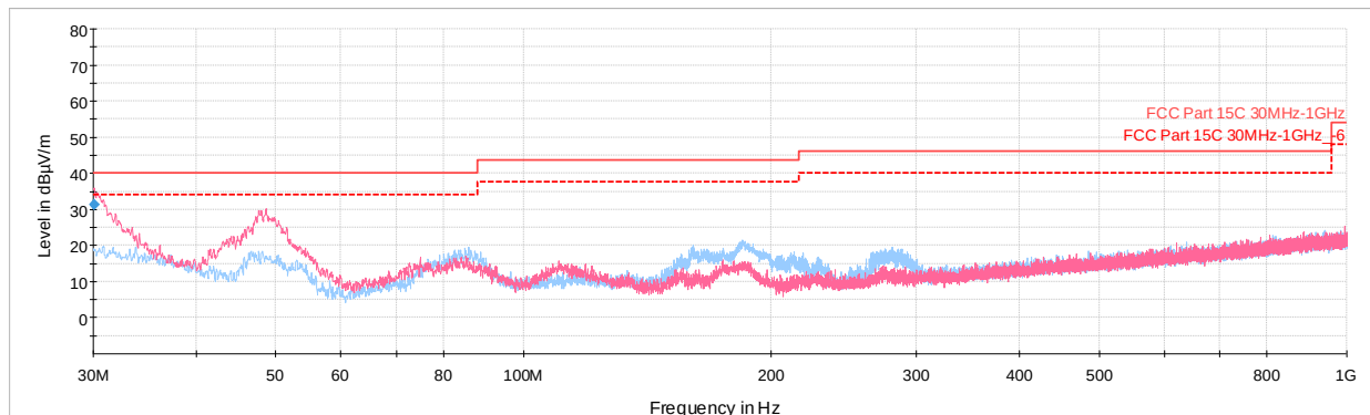
Plot 7-291. Radiated Spurious Plot below 1GHz CDD (802.11n – U3 Ch. 157 w/ AC/DC charger)
