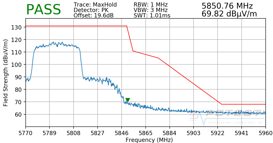
Plot 7-284. Radiated Upper Band Edge Plot CDD (Peak - UNII Band 3)
