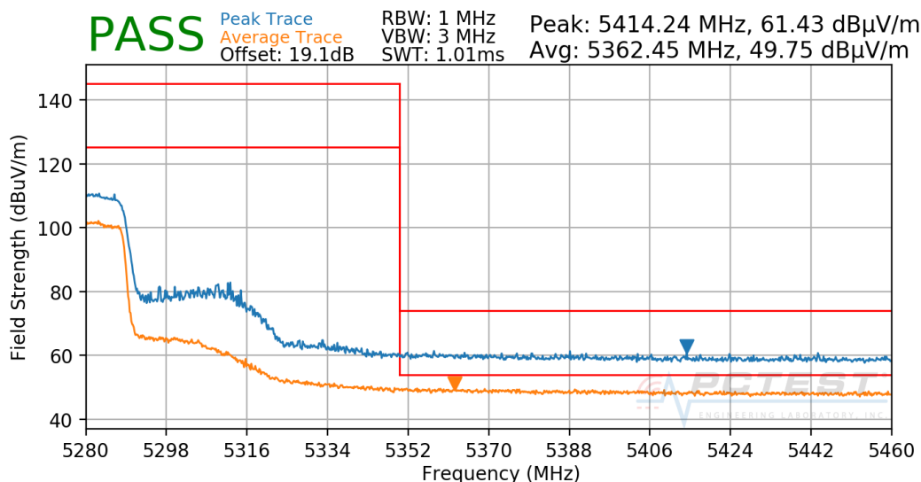
Plot 7-251. Radiated Upper Band Edge Plot SISO CORE1 (UNII Band 2A)
