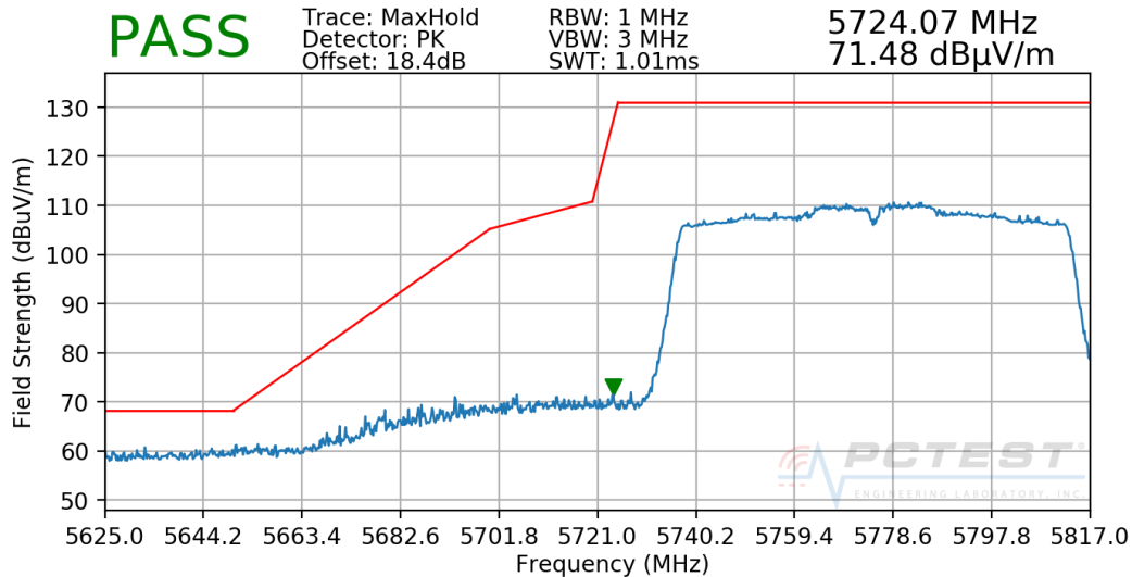
Plot 7-263. Radiated Lower Band Edge Plot SISO CORE1 (Peak – UNII Band 3)
