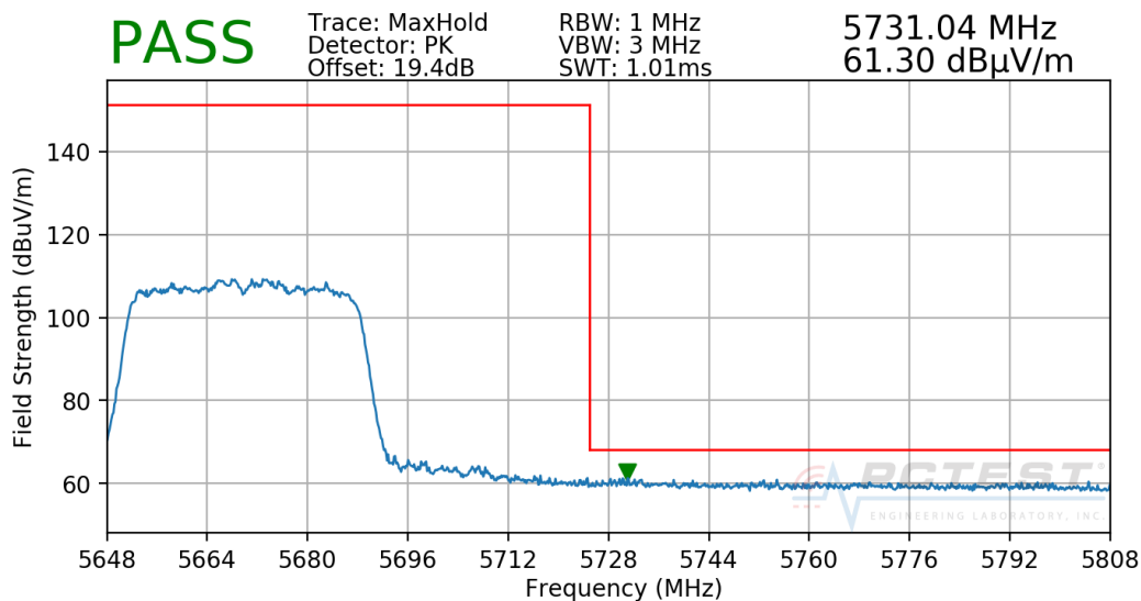
Plot 7-282. Radiated Upper Band Edge Plot CDD (Peak - UNII Band 2C)
