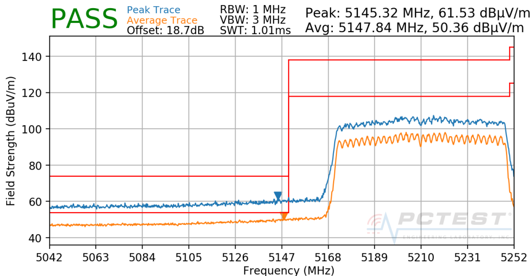
Plot 7-285. Radiated Lower Band Edge Plot CDD (UNII Band 1)
