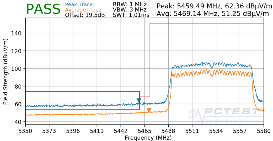
Plot 7-287. Radiated Lower Band Edge Plot CDD (UNII Band 2C)
