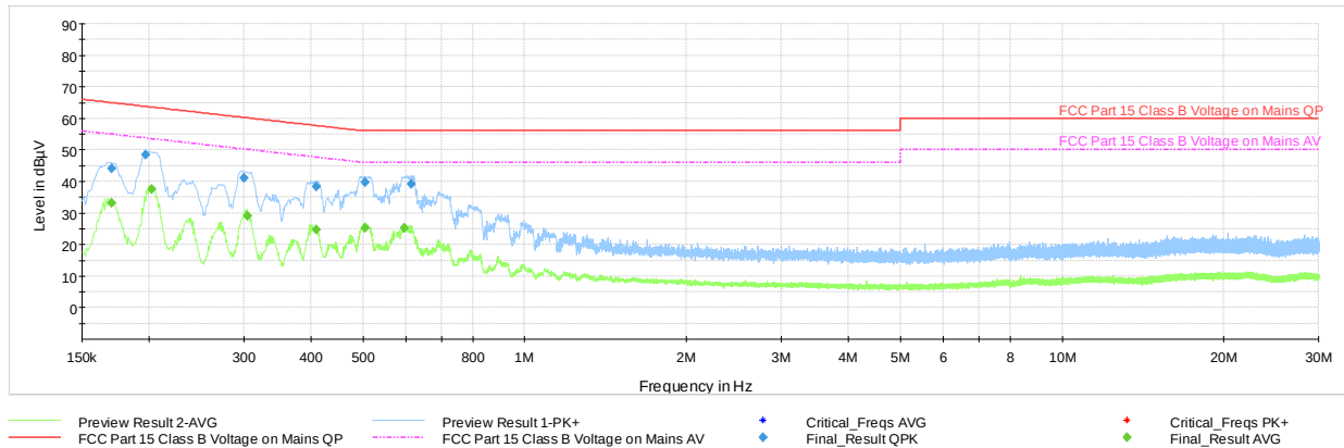
Plot 7-294. Line Conducted Plot with 802.11n UNII Band 1 (N) w/ AC/DC charger
