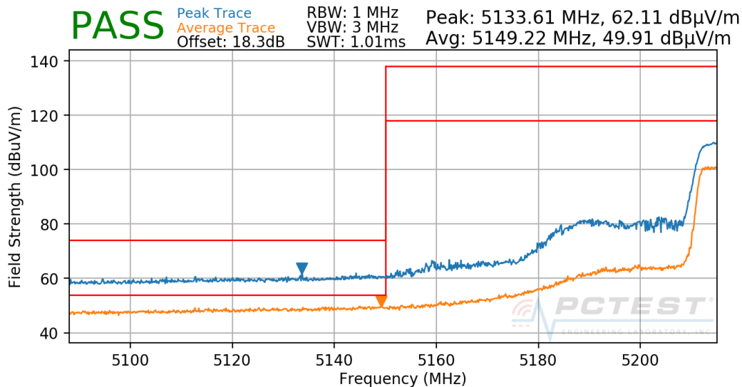
Plot 7-250. Radiated Lower Band Edge Plot SISO CORE1 (UNII Band 1)
