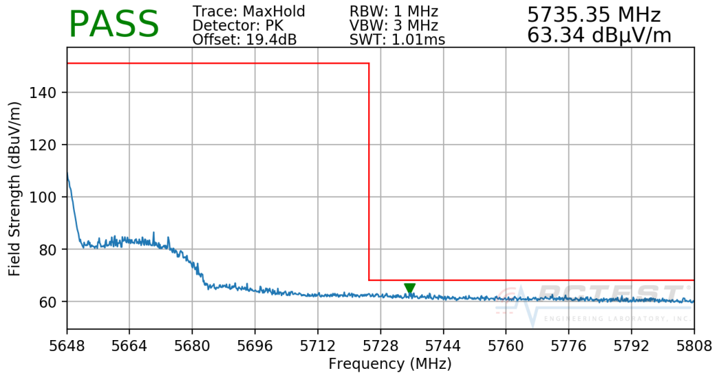
Plot 7-255. Radiated Upper Band Edge Plot SISO CORE1 (Peak - UNII Band 2C)
