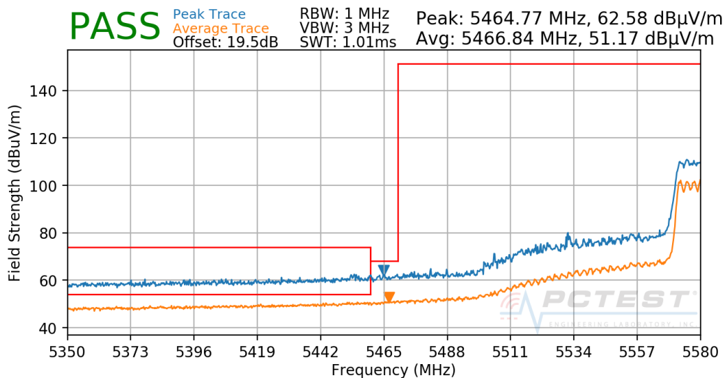
Plot 7-288. Radiated Lower Band Edge Plot CDD (UNII Band 2C)
