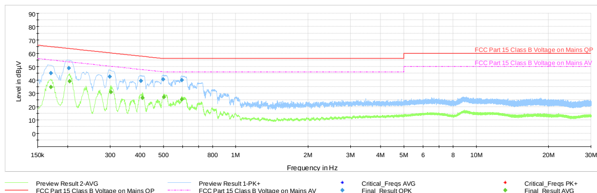
Plot 7-292. Line Conducted Plot with 802.11n UNII Band 1 (L1) w/ AC/DC charger
