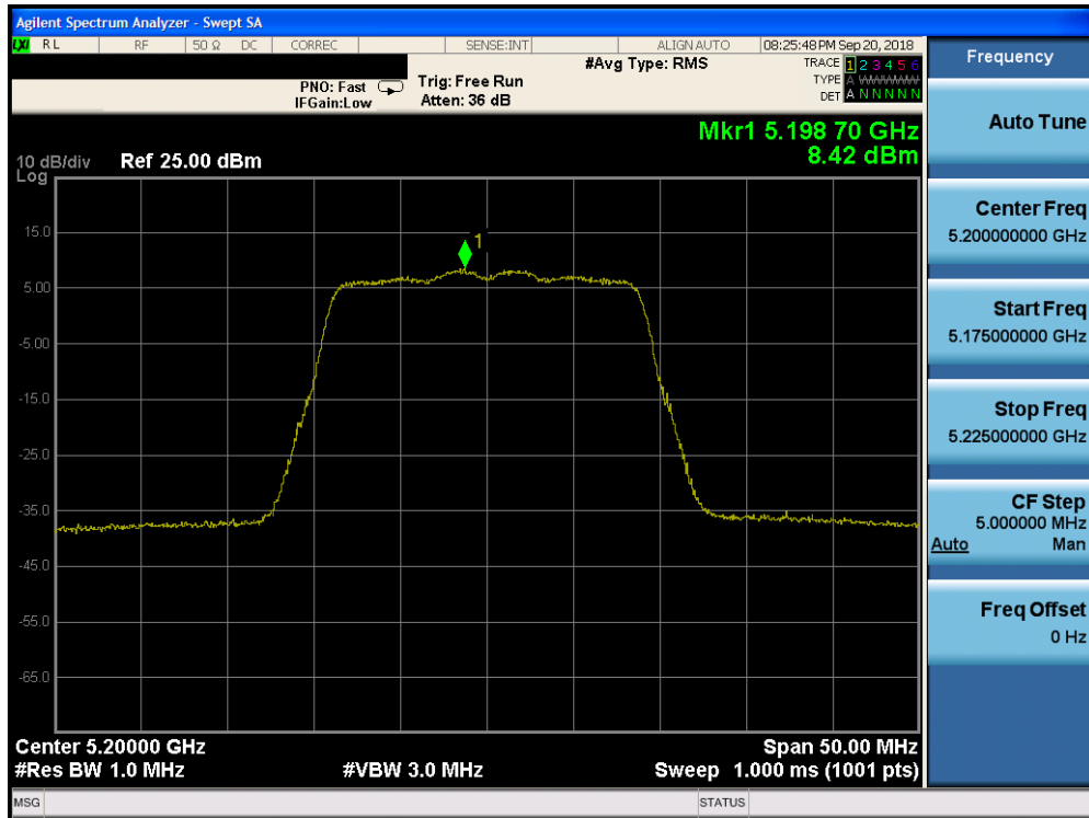
Plot 7-120. Power Spectral Density Plot CDD CORE 0 (20MHz BW 802.11n (UNII Band 1) – Ch. 40)
