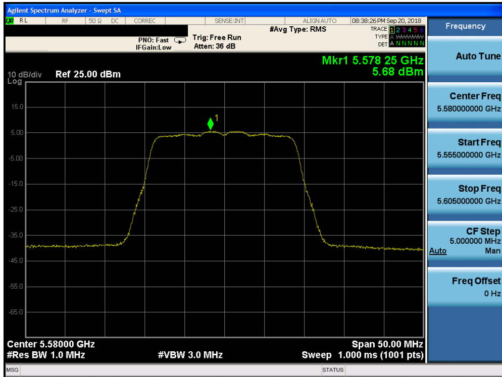
Plot 7-144. Power Spectral Density Plot CDD CORE 0 (20MHz BW 802.11n (UNII Band 2C) – Ch. 116)
