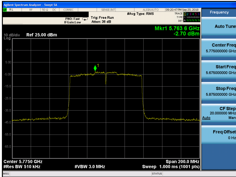
Plot 7-168. Power Spectral Density Plot CDD CORE 0 (80MHz BW 802.11ac (UNII Band 3) – Ch. 155)
