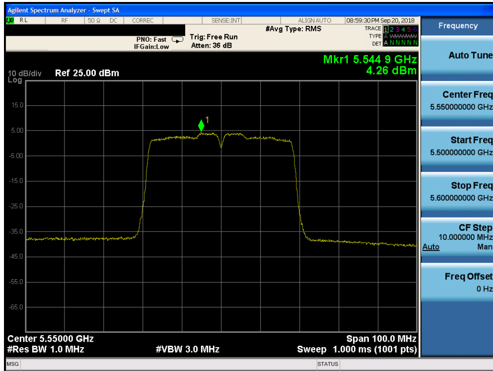
Plot 7-150. Power Spectral Density Plot CDD CORE 0 (40MHz BW 802.11n (UNII Band 2C) – Ch. 110)
