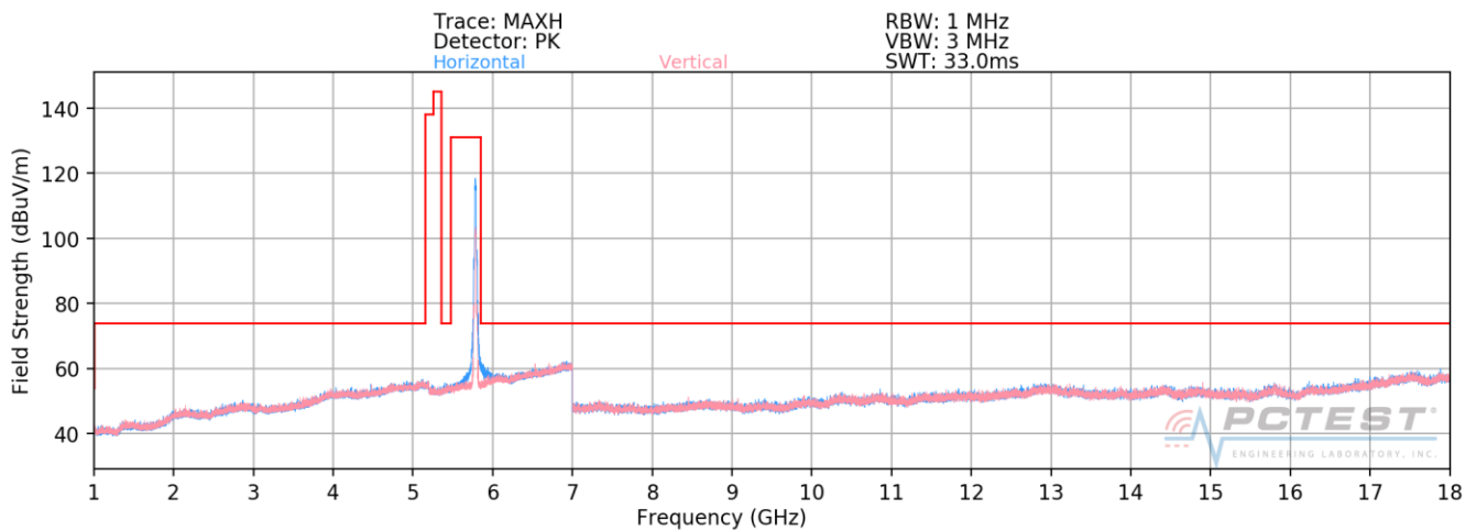
Plot 7-180. Radiated Spurious Plot above 1GHz SISO CORE0 (802.11n – U3 Ch. 157)
