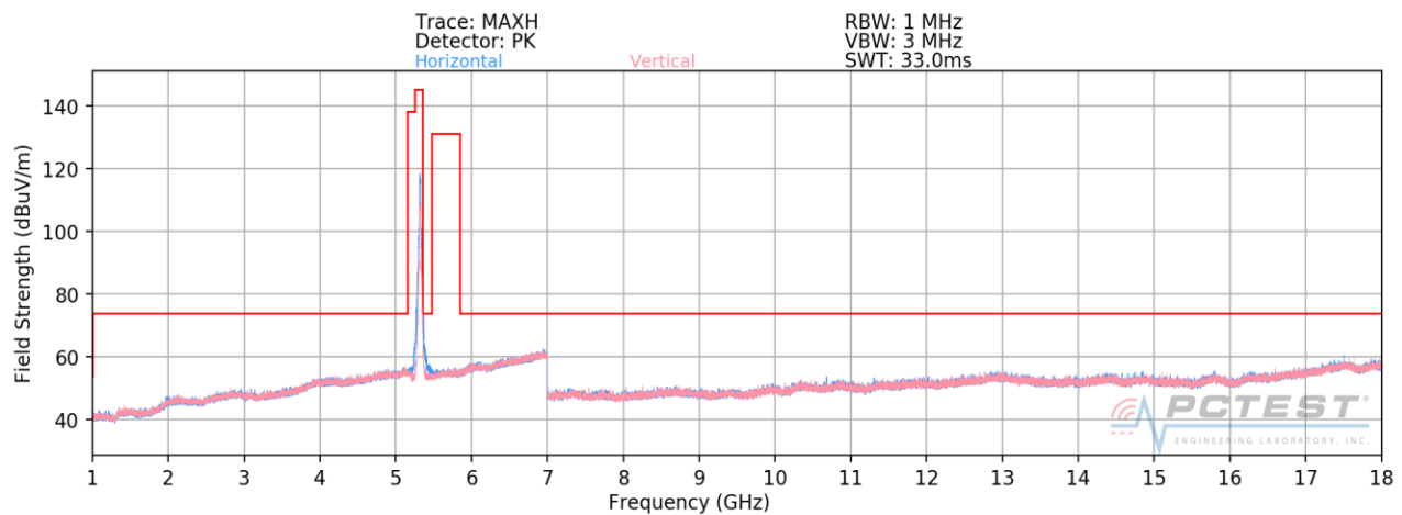
Plot 7-175. Radiated Spurious Plot above 1GHz SISO CORE0 (802.11n – U2A Ch. 64)
