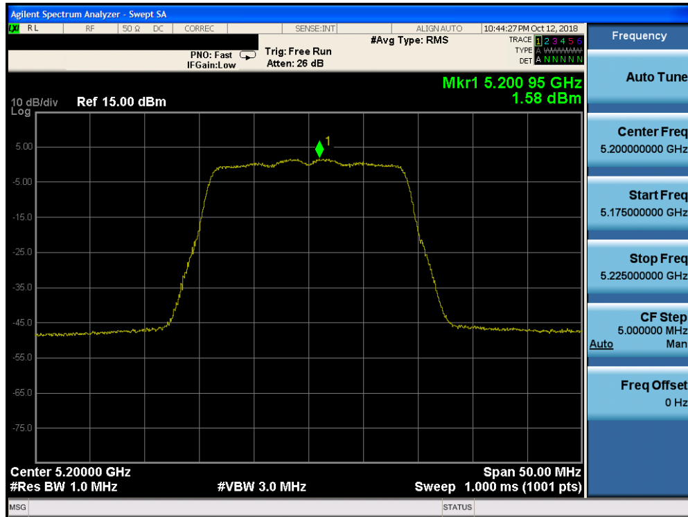
Plot 7-110. Power Spectral Density Plot CDD CORE 0 (20MHz BW 802.11n (UNII Band 1) – Ch. 40) - ISED
