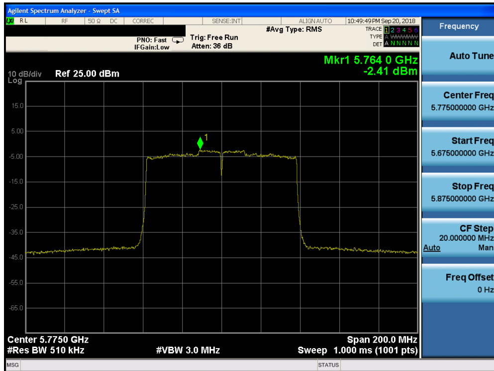
Plot 7-169. Power Spectral Density Plot CDD CORE 1 (80MHz BW 802.11ac (UNII Band 3) – Ch. 155)
