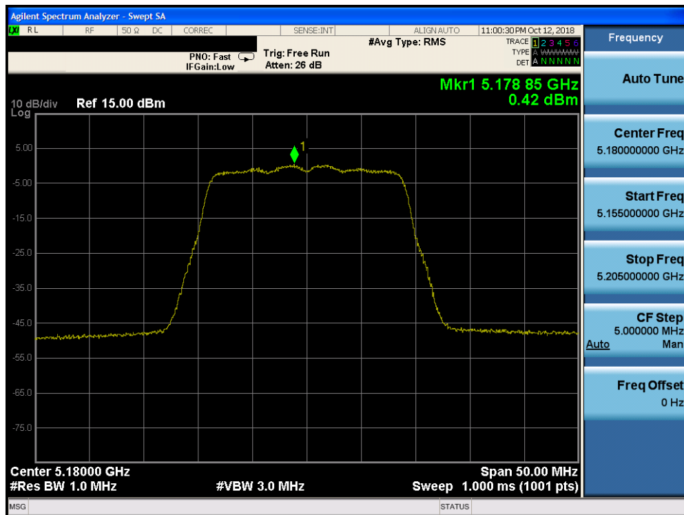
Plot 7-109. Power Spectral Density Plot CDD CORE 1 (20MHz BW 802.11n (UNII Band 1) – Ch. 36) - ISED
