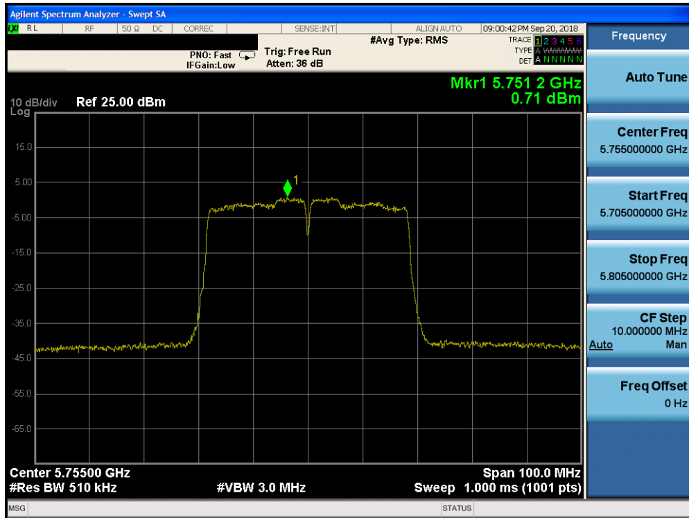
Plot 7-164. Power Spectral Density Plot CDD CORE 0 (40MHz BW 802.11n (UNII Band 3) – Ch. 151)
