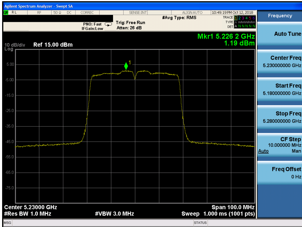
Plot 7-116. Power Spectral Density Plot CDD CORE 0 (40MHz BW 802.11n (UNII Band 1) – Ch. 46) - ISED
