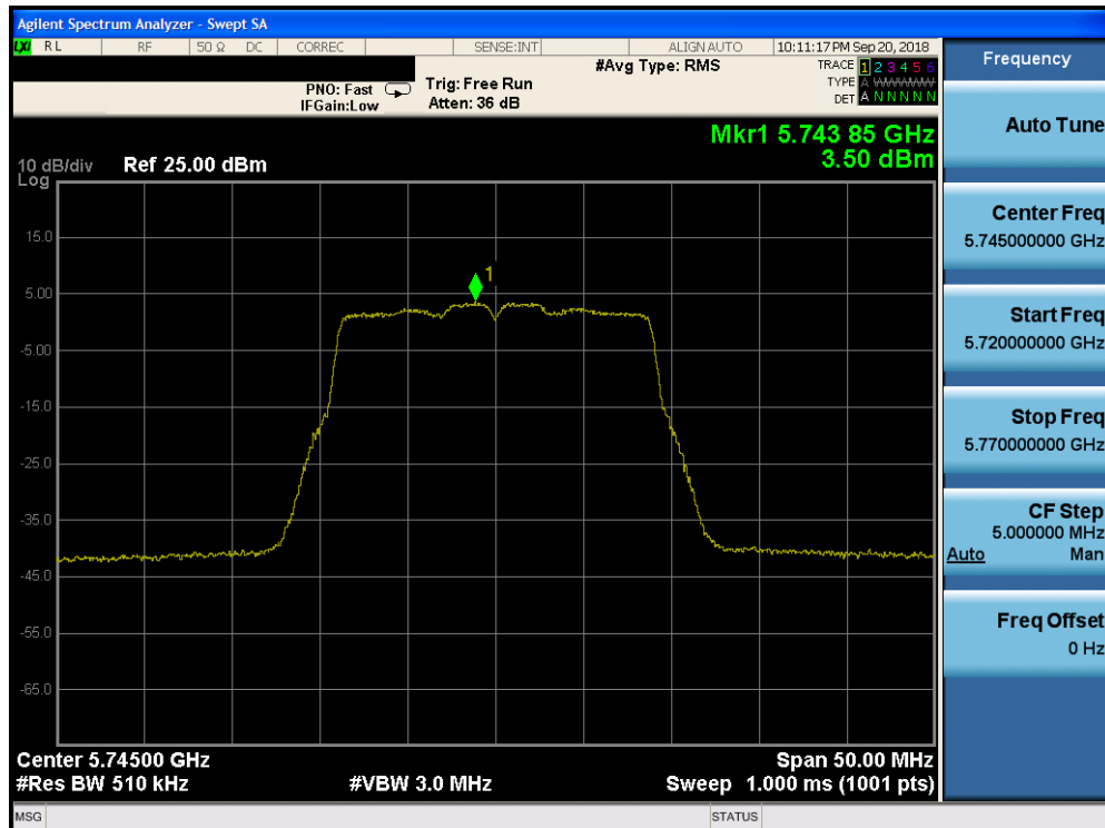
Plot 7-159. Power Spectral Density Plot CDD CORE 1 (20MHz BW 802.11n (UNII Band 3) – Ch. 149)
