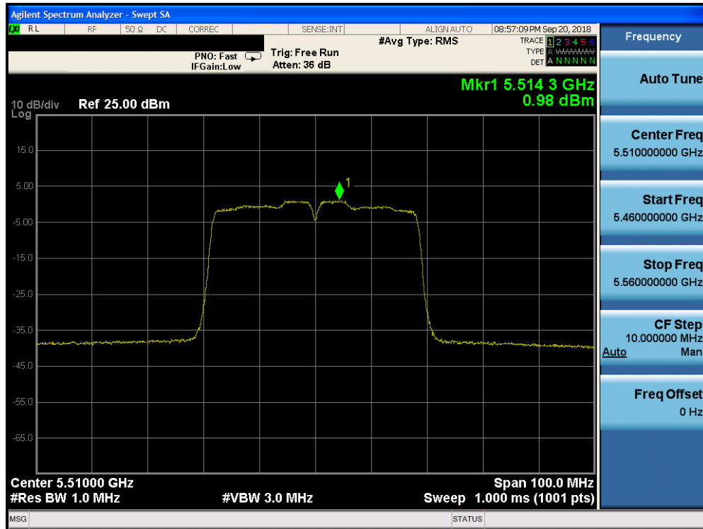
Plot 7-148. Power Spectral Density Plot CDD CORE 0 (40MHz BW 802.11n (UNII Band 2C) – Ch. 102)
