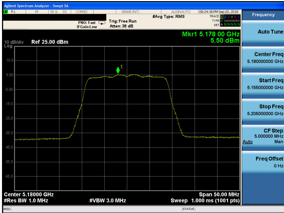
Plot 7-118. Power Spectral Density Plot CDD CORE 0 (20MHz BW 802.11n (UNII Band 1) – Ch. 36)
