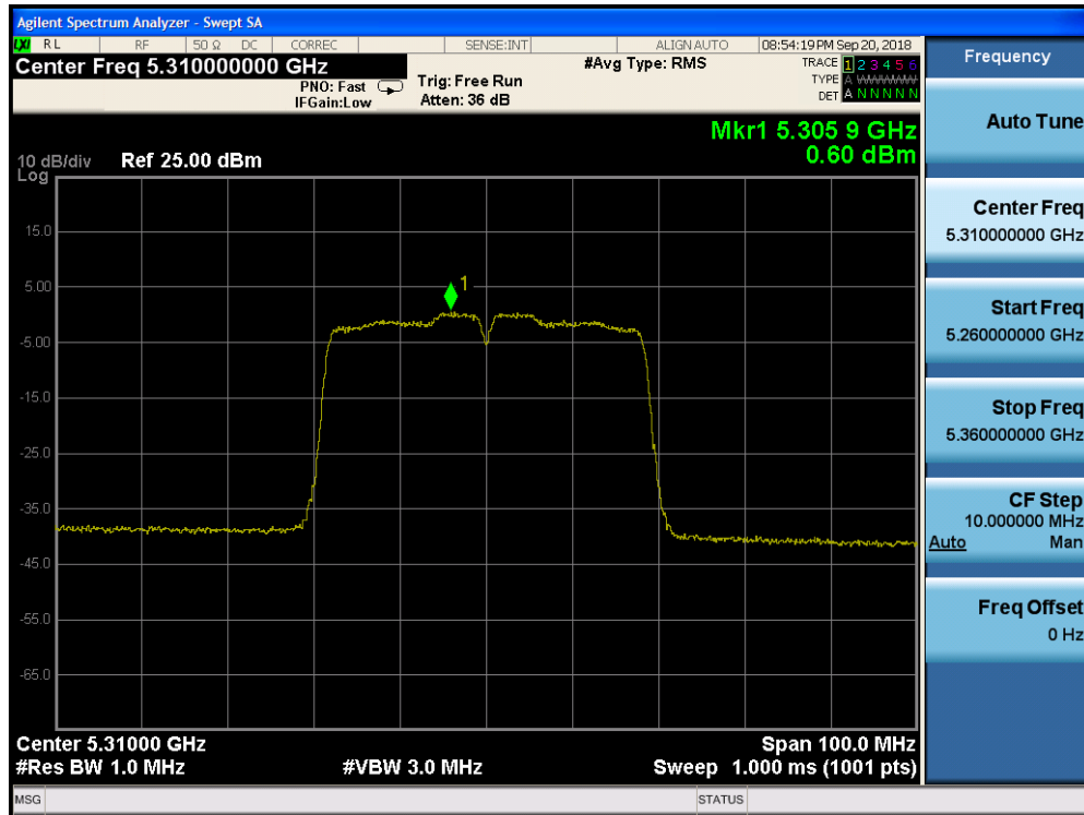
Plot 7-138. Power Spectral Density Plot CDD CORE 0 (40MHz BW 802.11n (UNII Band 2A) – Ch. 62)
