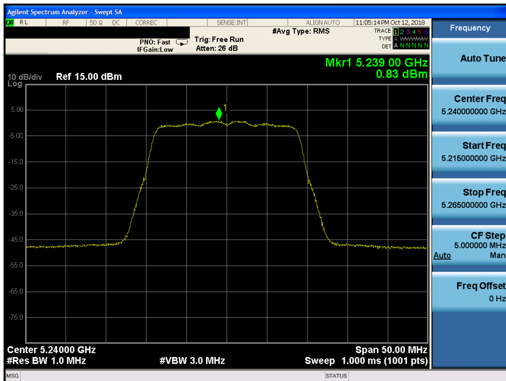
Plot 7-113. Power Spectral Density Plot CDD CORE 1 (20MHz BW 802.11n (UNII Band 1) – Ch. 48) - ISED
