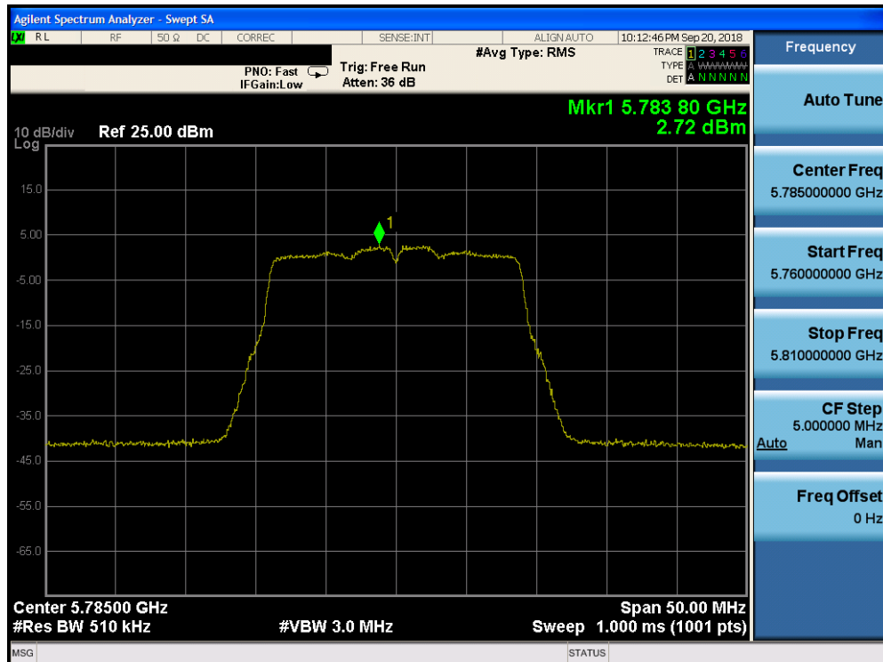
Plot 7-161. Power Spectral Density Plot CDD CORE 1 (20MHz BW 802.11n (UNII Band 3) – Ch. 157)
