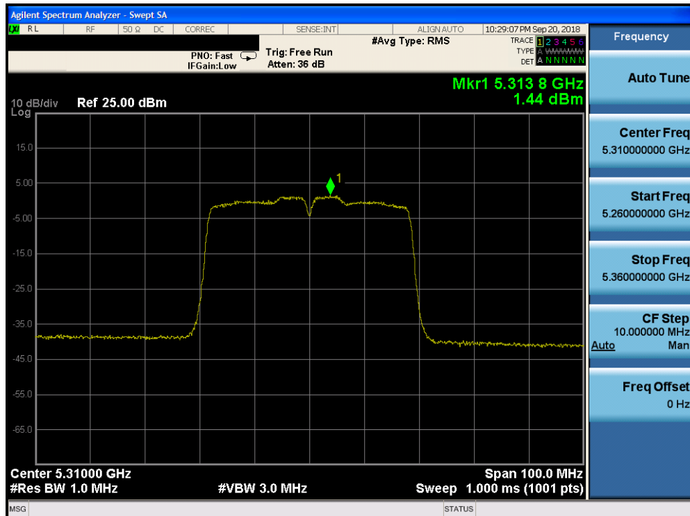
Plot 7-139. Power Spectral Density Plot CDD CORE 1 (40MHz BW 802.11n (UNII Band 2A) – Ch. 62)
