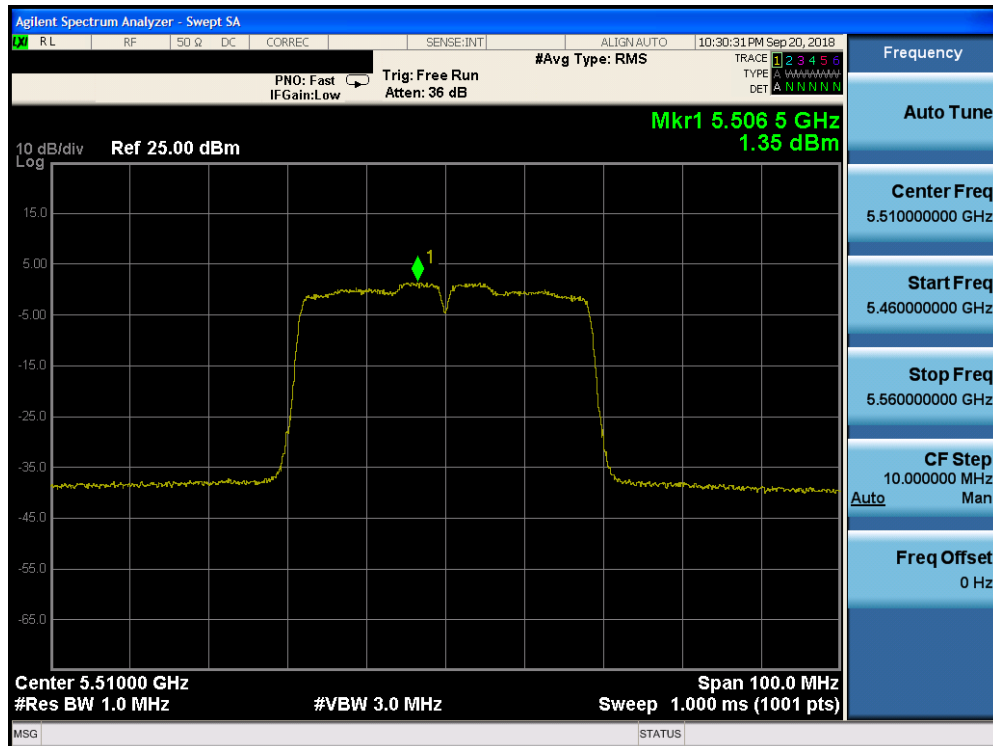
Plot 7-149. Power Spectral Density Plot CDD CORE 1 (40MHz BW 802.11n (UNII Band 2C) – Ch. 102)
