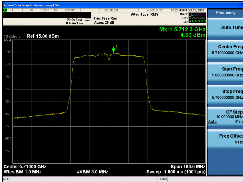
Plot 7-153. Power Spectral Density Plot CDD CORE 1 (40MHz BW 802.11n (UNII Band 2C) – Ch. 142)
