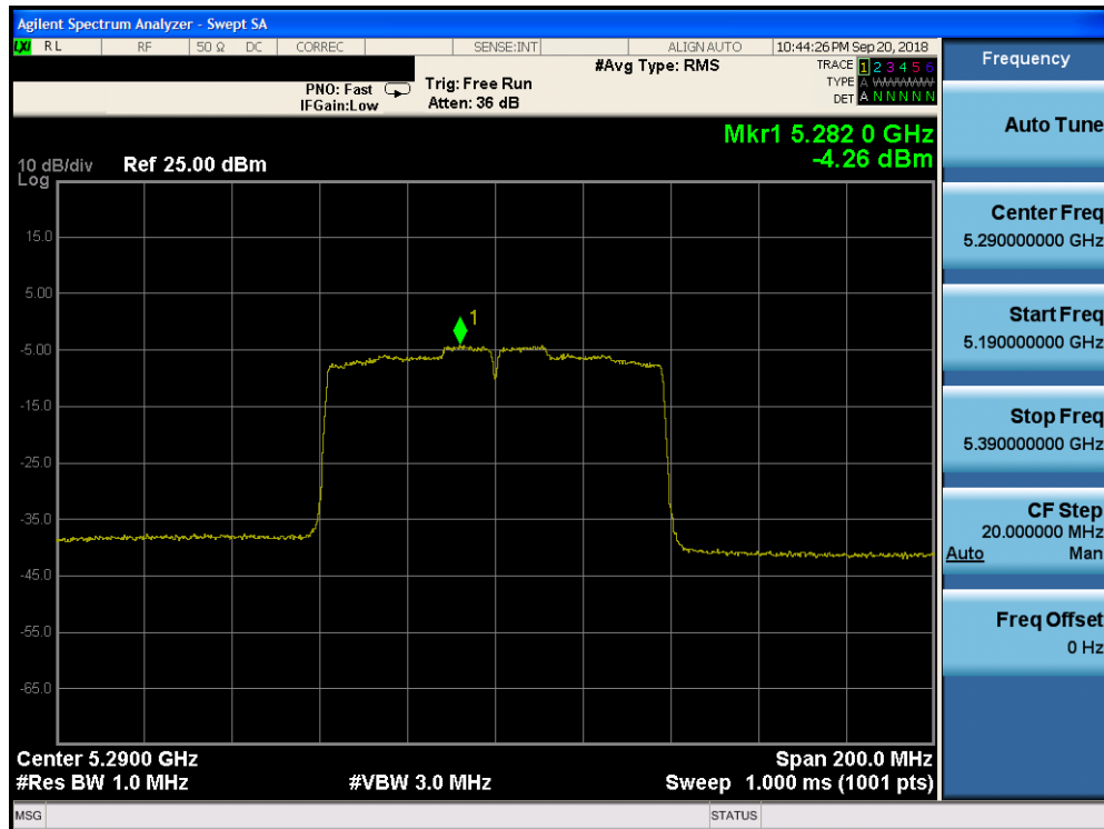
Plot 7-141. Power Spectral Density Plot CDD CORE 1 (80MHz BW 802.11ac (UNII Band 2A) – Ch. 58)
