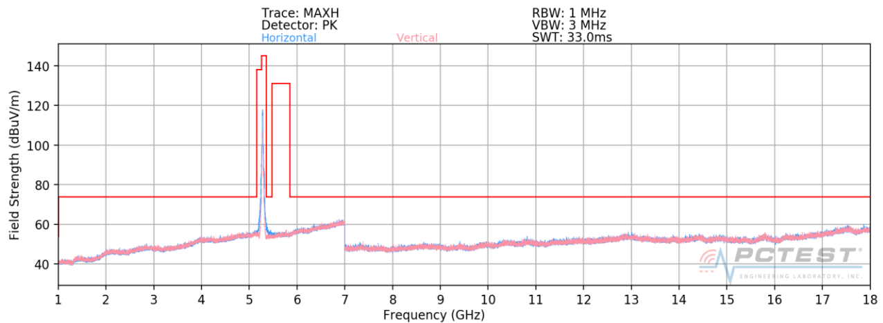
Plot 7-174. Radiated Spurious Plot above 1GHz SISO CORE0 (802.11n – U2A Ch. 56)
