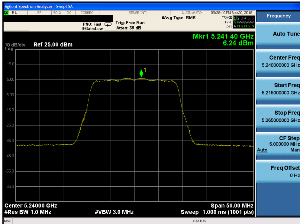
Plot 7-123. Power Spectral Density Plot CDD CORE 1 (20MHz BW 802.11n (UNII Band 1) – Ch. 48)
