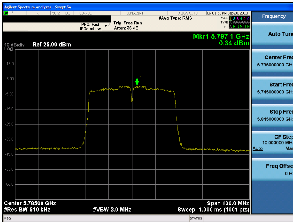
Plot 7-166. Power Spectral Density Plot CDD CORE 0 (40MHz BW 802.11n (UNII Band 3) – Ch. 159)
