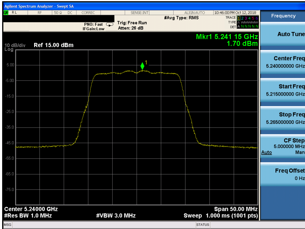
Plot 7-112. Power Spectral Density Plot CDD CORE 0 (20MHz BW 802.11n (UNII Band 1) – Ch. 48) - ISED
