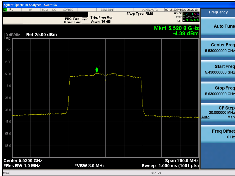
Plot 7-154. Power Spectral Density Plot CDD CORE 0 (80MHz BW 802.11ac (UNII Band 2C) – Ch. 106)
