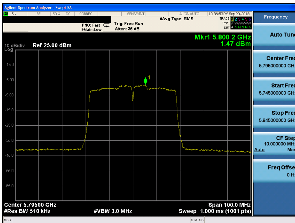
Plot 7-167. Power Spectral Density Plot CDD CORE 1 (40MHz BW 802.11n (UNII Band 3) – Ch. 159)
