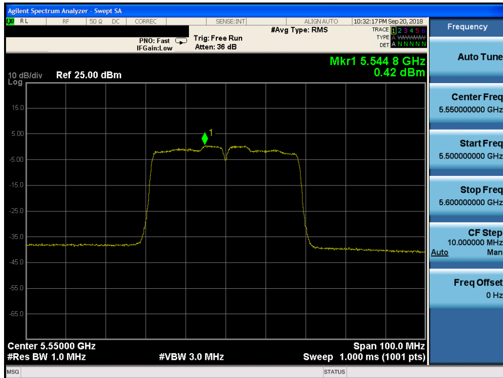
Plot 7-151. Power Spectral Density Plot CDD CORE 1 (40MHz BW 802.11n (UNII Band 2C) – Ch. 110)
