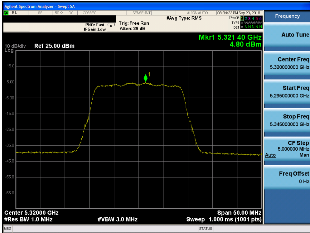
Plot 7-134. Power Spectral Density Plot CDD CORE 0 (20MHz BW 802.11n (UNII Band 2A) – Ch. 64)
