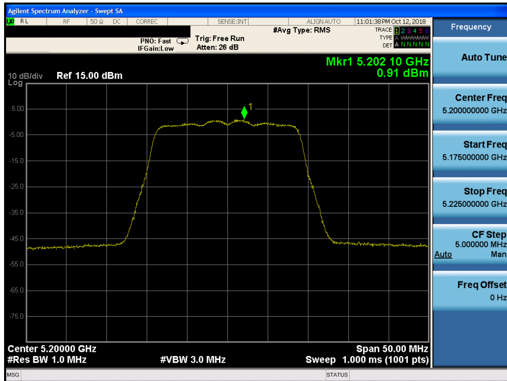
Plot 7-111. Power Spectral Density Plot CDD CORE 1 (20MHz BW 802.11n (UNII Band 1) – Ch. 40) - ISED
