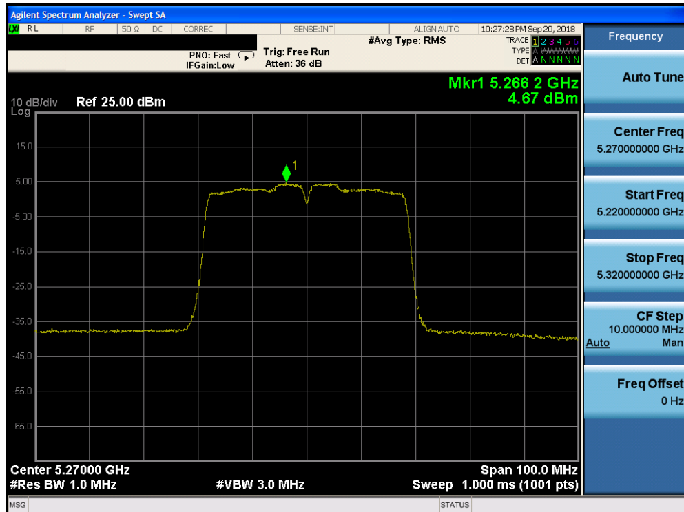
Plot 7-137. Power Spectral Density Plot CDD CORE 1 (40MHz BW 802.11n (UNII Band 2A) – Ch. 54)
