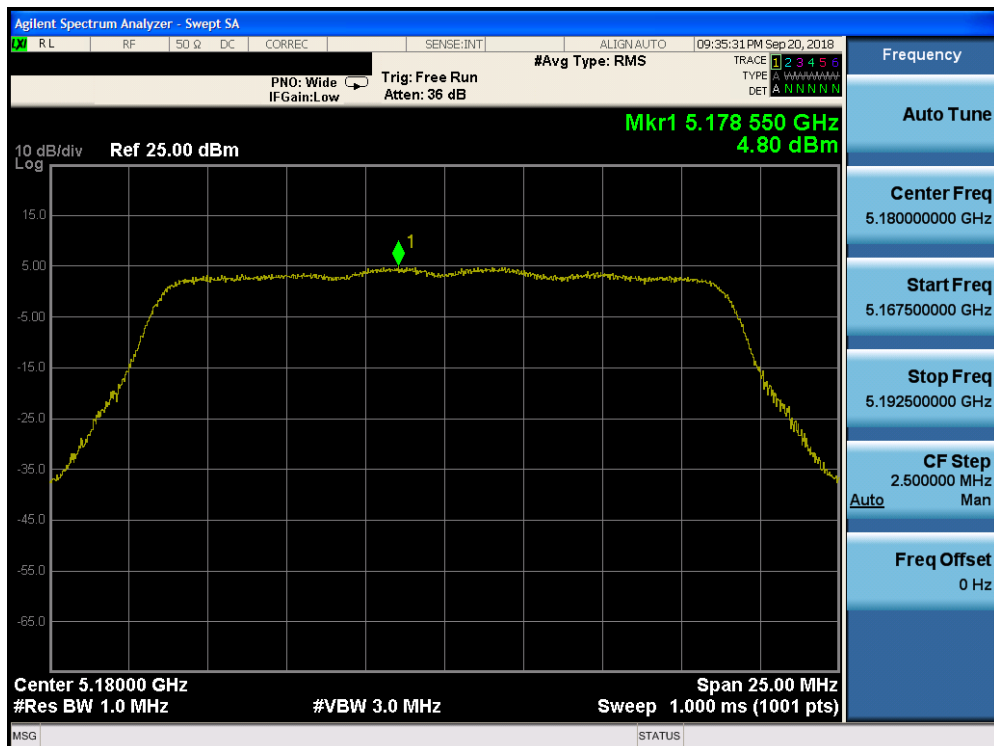
Plot 7-119. Power Spectral Density Plot CDD CORE 1 (20MHz BW 802.11n (UNII Band 1) – Ch. 36)
