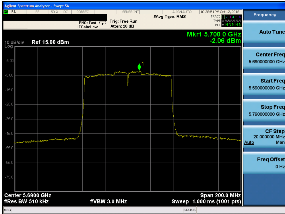
Plot 7-156. Power Spectral Density Plot CDD CORE 0 (80MHz BW 802.11ac (UNII Band 2C) – Ch. 138)
