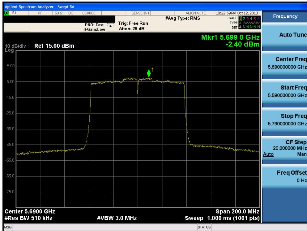
Plot 7-157. Power Spectral Density Plot CDD CORE 1 (80MHz BW 802.11ac (UNII Band 2C) – Ch. 138)
