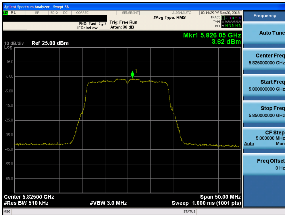
Plot 7-163. Power Spectral Density Plot CDD CORE 1 (20MHz BW 802.11n (UNII Band 3) – Ch. 165)
