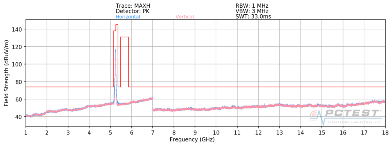
Plot 7-172. Radiated Spurious Plot above 1GHz SISO CORE0 (802.11n – U1 Ch. 48)
