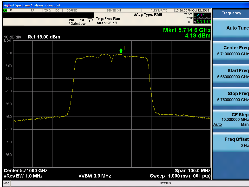
Plot 7-152. Power Spectral Density Plot CDD CORE 0 (40MHz BW 802.11n (UNII Band 2C) – Ch. 142)
