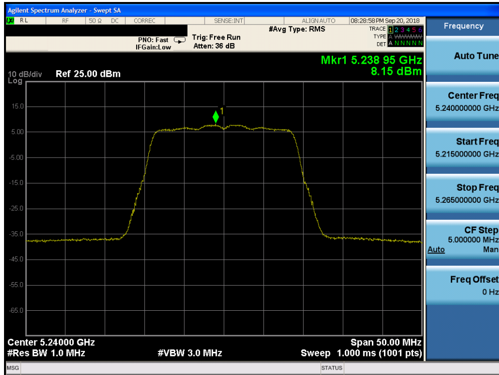
Plot 7-122. Power Spectral Density Plot CDD CORE 0 (20MHz BW 802.11n (UNII Band 1) – Ch. 48)
