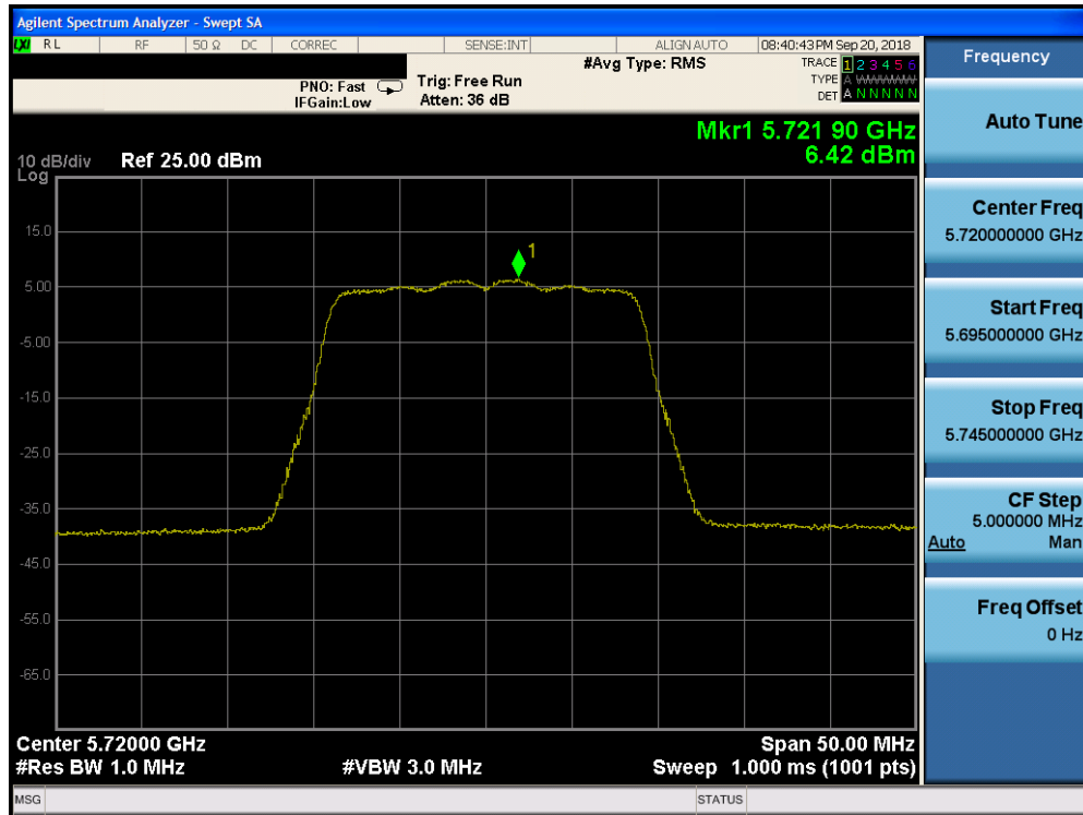
Plot 7-146. Power Spectral Density Plot CDD CORE 0 (20MHz BW 802.11n (UNII Band 2C) – Ch. 144)
