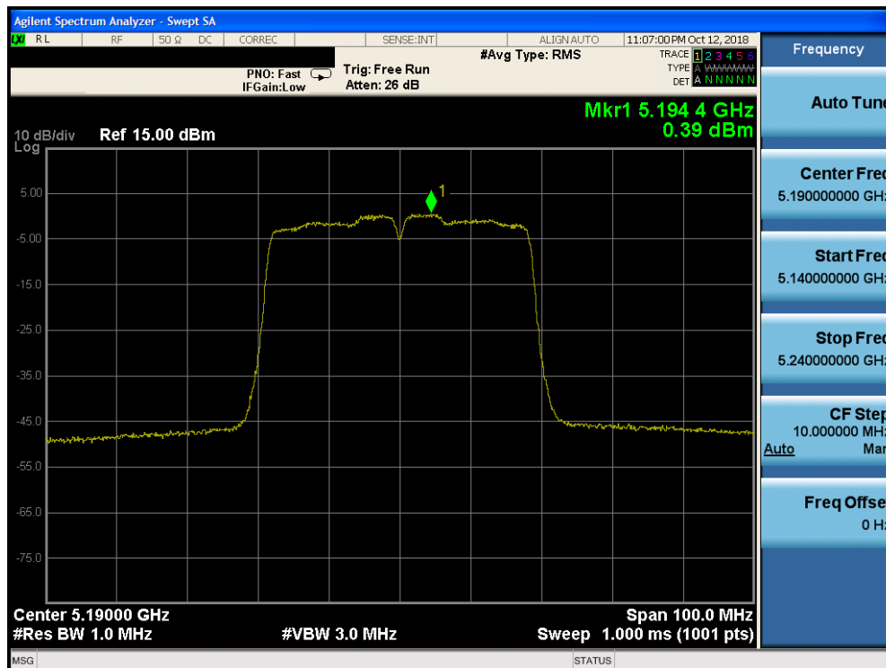
Plot 7-115. Power Spectral Density Plot CDD CORE 1 (40MHz BW 802.11n (UNII Band 1) – Ch. 38) - ISED
