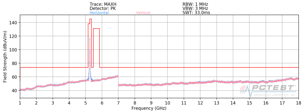
Plot 7-173. Radiated Spurious Plot above 1GHz SISO CORE0 (802.11n – U2A Ch. 52)
