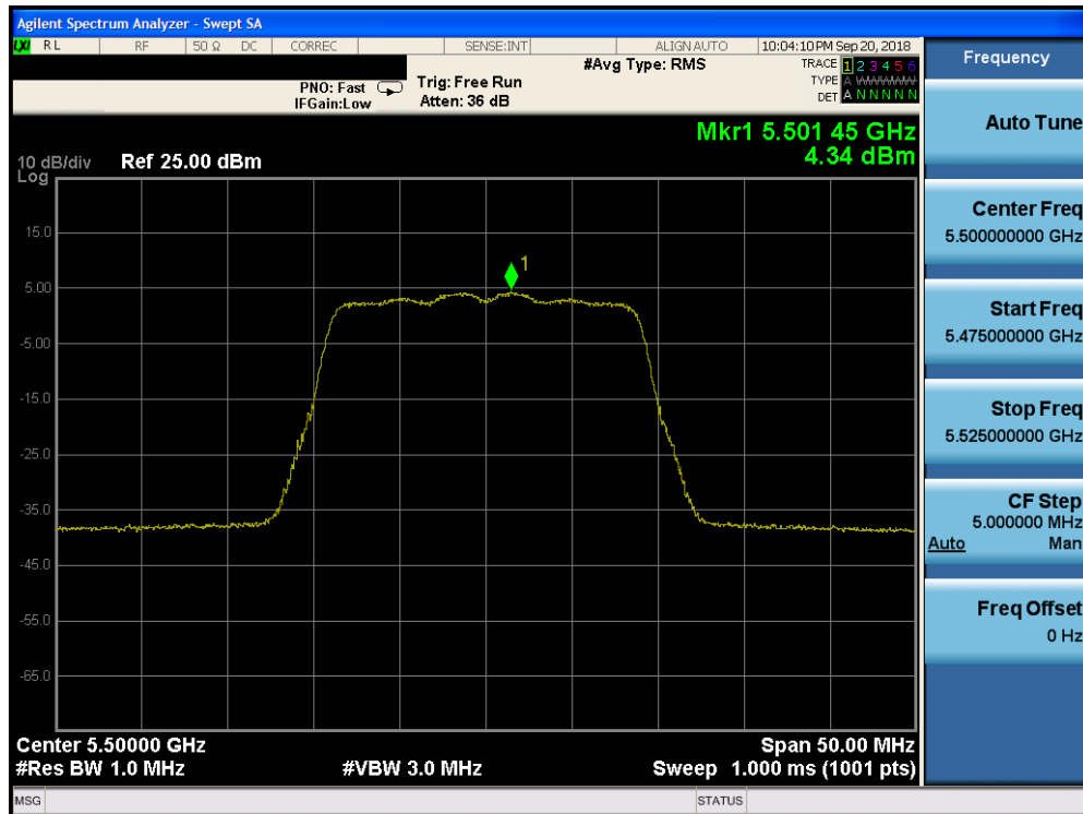
Plot 7-143. Power Spectral Density Plot CDD CORE 1 (20MHz BW 802.11n (UNII Band 2C) – Ch. 100)
