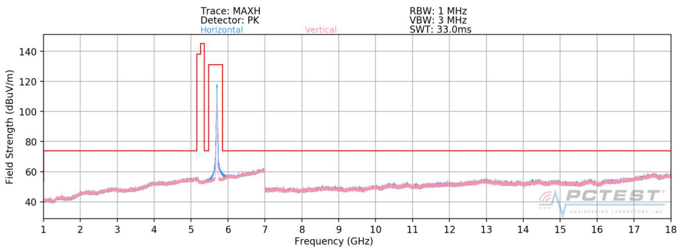
Plot 7-178. Radiated Spurious Plot above 1GHz SISO CORE0 (802.11n – U2C Ch. 140)
