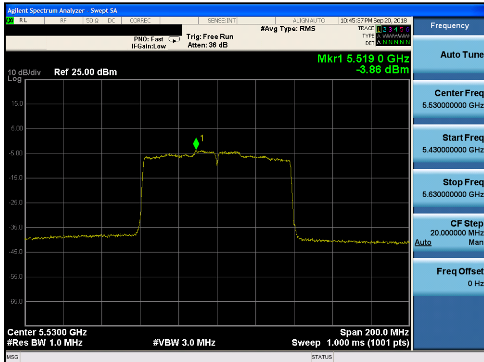
Plot 7-155. Power Spectral Density Plot CDD CORE 1 (80MHz BW 802.11ac (UNII Band 2C) – Ch. 106)
