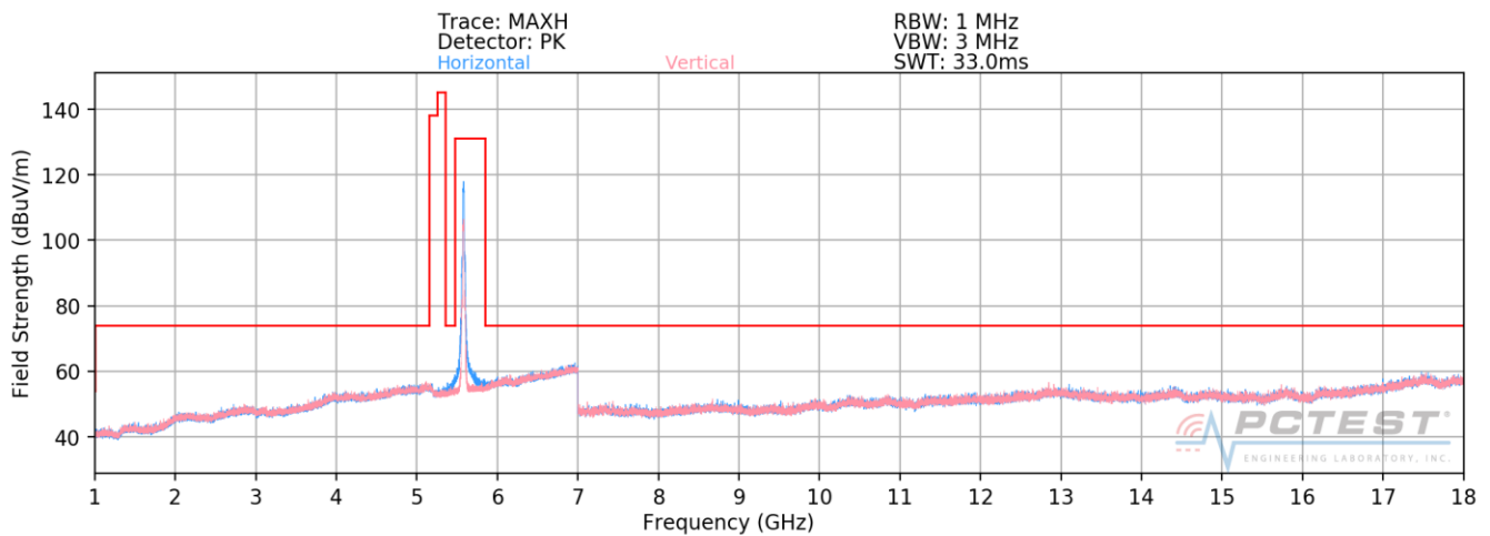
Plot 7-177. Radiated Spurious Plot above 1GHz SISO CORE0 (802.11n – U2C Ch. 116)
