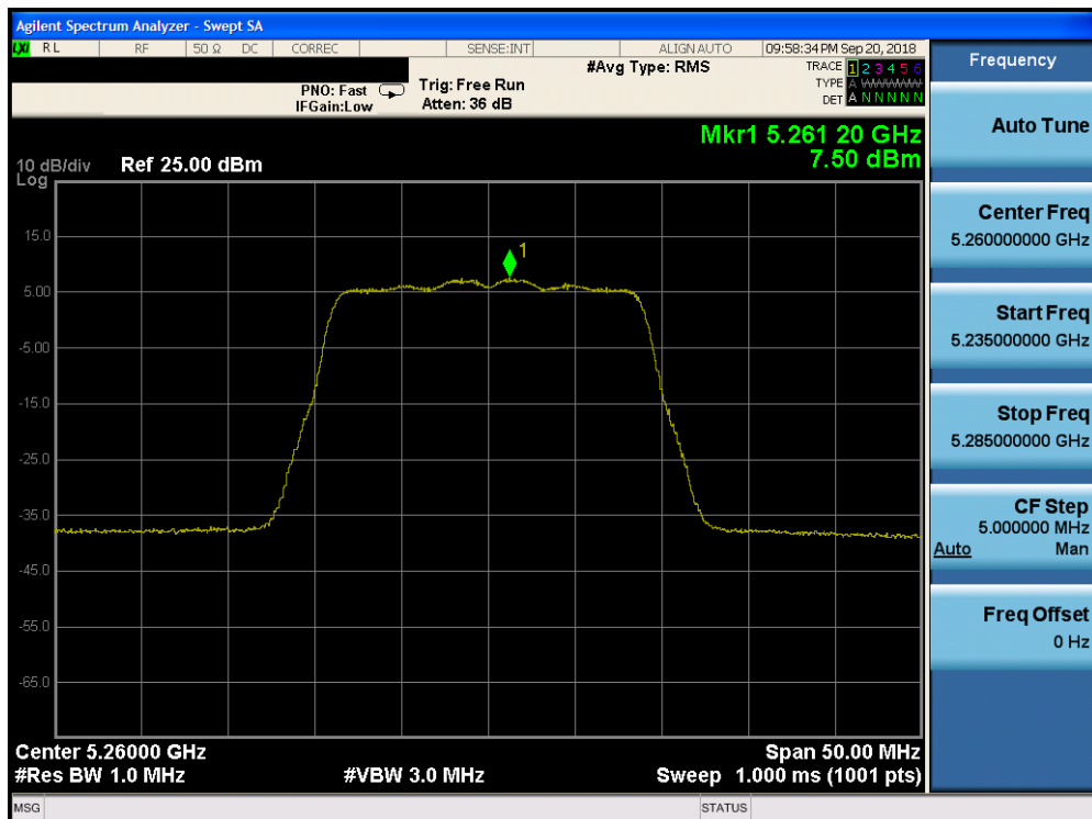
Plot 7-131. Power Spectral Density Plot CDD CORE 1 (20MHz BW 802.11n (UNII Band 2A) – Ch. 52)
