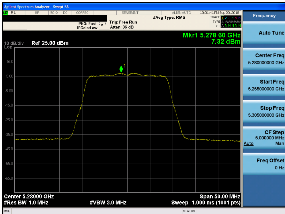
Plot 7-133. Power Spectral Density Plot CDD CORE 1 (20MHz BW 802.11n (UNII Band 2A) – Ch. 56)
