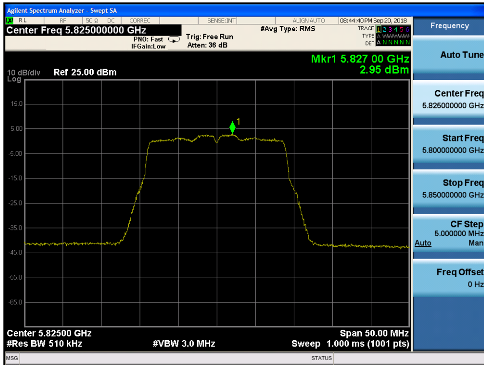
Plot 7-162. Power Spectral Density Plot CDD CORE 0 (20MHz BW 802.11n (UNII Band 3) – Ch. 165)
