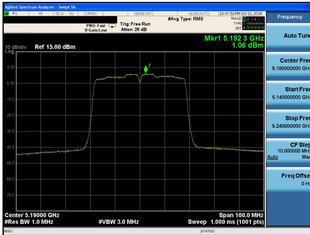
Plot 7-114. Power Spectral Density Plot CDD CORE 0 (40MHz BW 802.11n (UNII Band 1) – Ch. 38) - ISED
