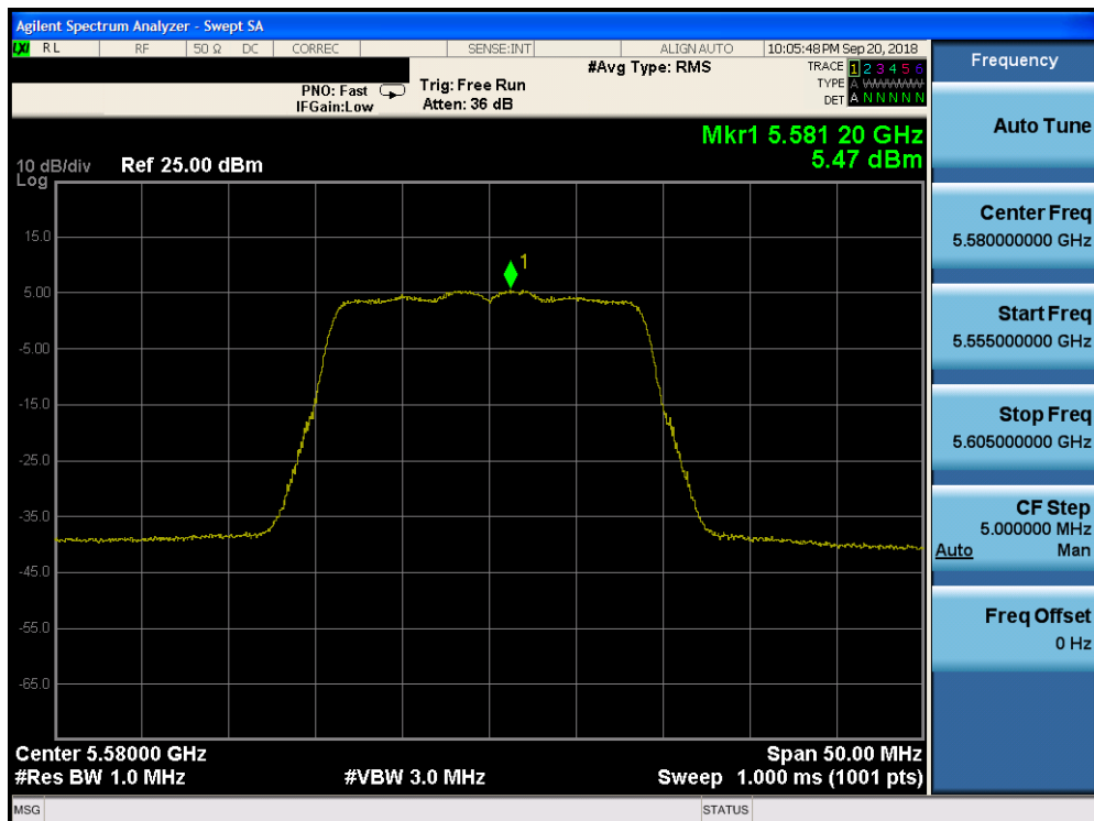
Plot 7-145. Power Spectral Density Plot CDD CORE 1 (20MHz BW 802.11n (UNII Band 2C) – Ch. 116)
