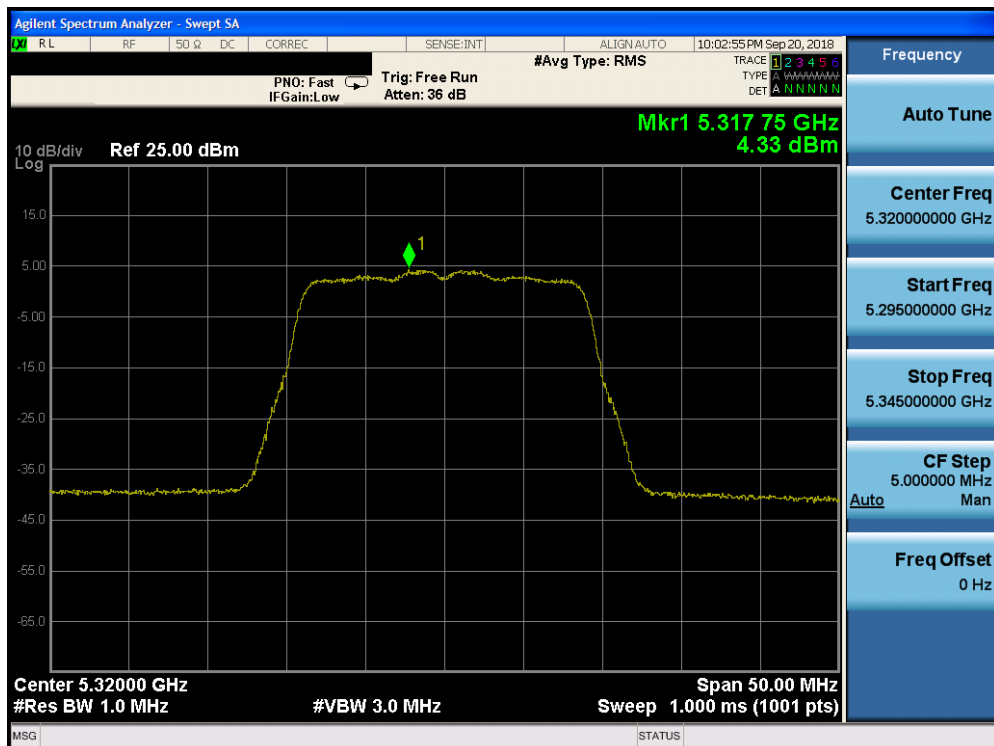
Plot 7-135. Power Spectral Density Plot CDD CORE 1 (20MHz BW 802.11n (UNII Band 2A) – Ch. 64)
