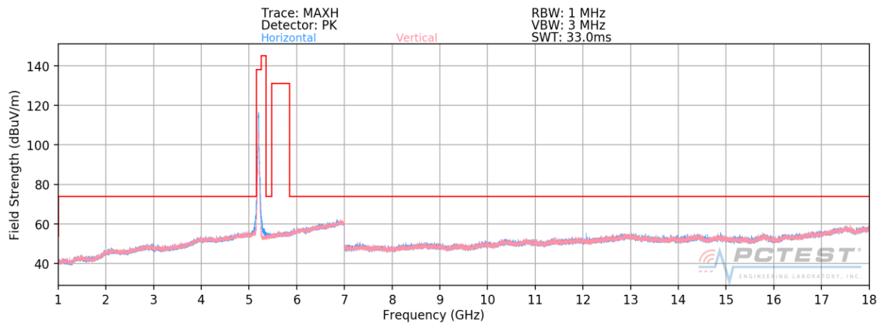
Plot 7-171. Radiated Spurious Plot above 1GHz SISO CORE0 (802.11n – U1 Ch. 40)
