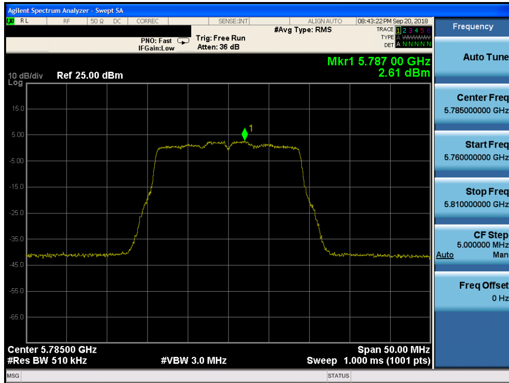
Plot 7-160. Power Spectral Density Plot CDD CORE 0 (20MHz BW 802.11n (UNII Band 3) – Ch. 157)
