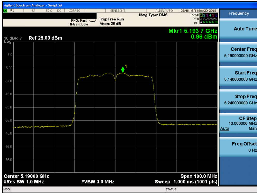
Plot 7-124. Power Spectral Density Plot CDD CORE 0 (40MHz BW 802.11n (UNII Band 1) – Ch. 38)
