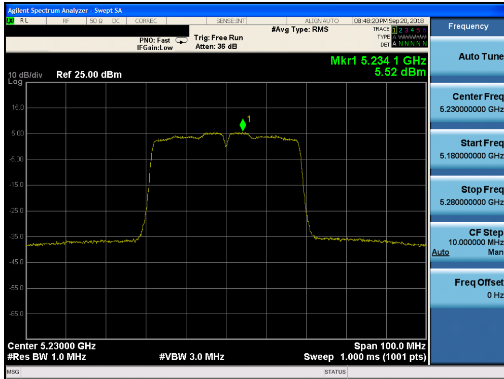
Plot 7-126. Power Spectral Density Plot CDD CORE 0 (40MHz BW 802.11n (UNII Band 1) – Ch. 46)
