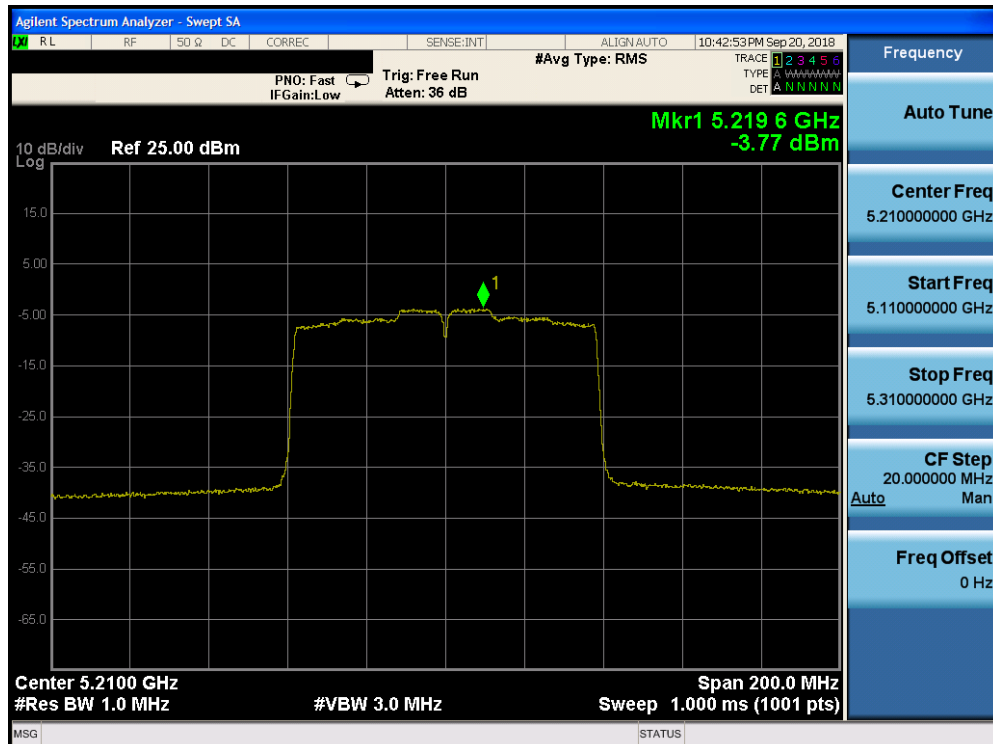
Plot 7-129. Power Spectral Density Plot CDD CORE 1 (80MHz BW 802.11ac (UNII Band 1) – Ch. 42)
