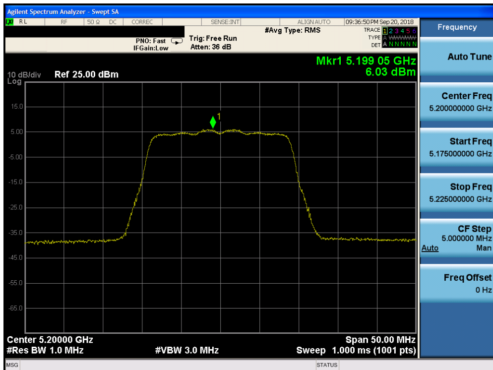
Plot 7-121. Power Spectral Density Plot CDD CORE 1 (20MHz BW 802.11n (UNII Band 1) – Ch. 40)
