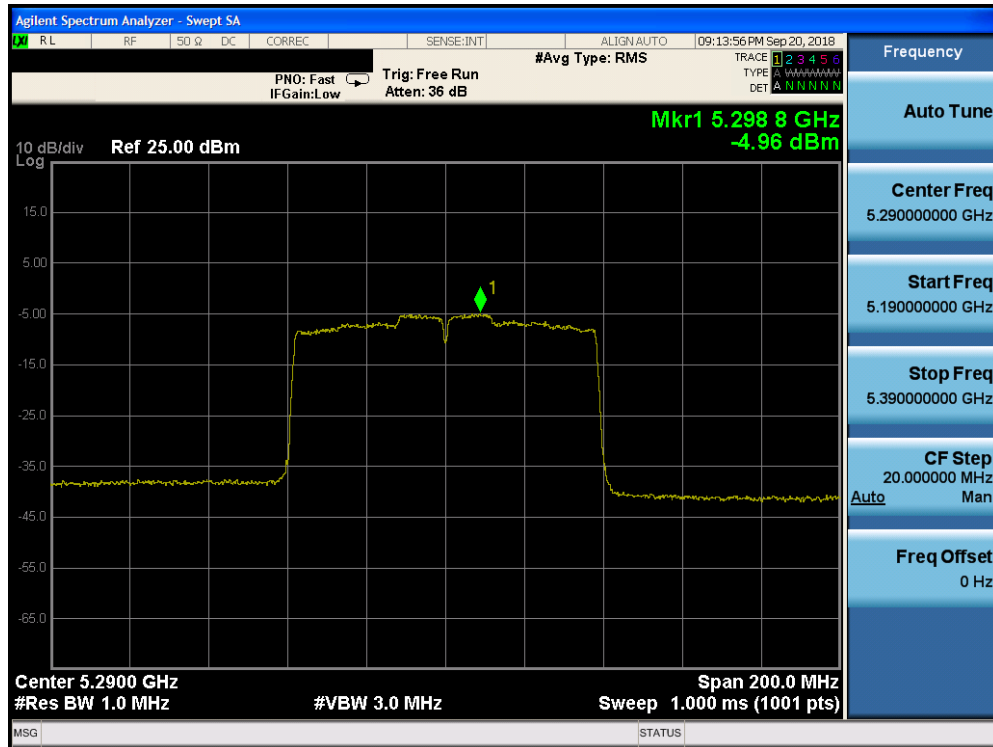
Plot 7-140. Power Spectral Density Plot CDD CORE 0 (80MHz BW 802.11ac (UNII Band 2A) – Ch. 58)
