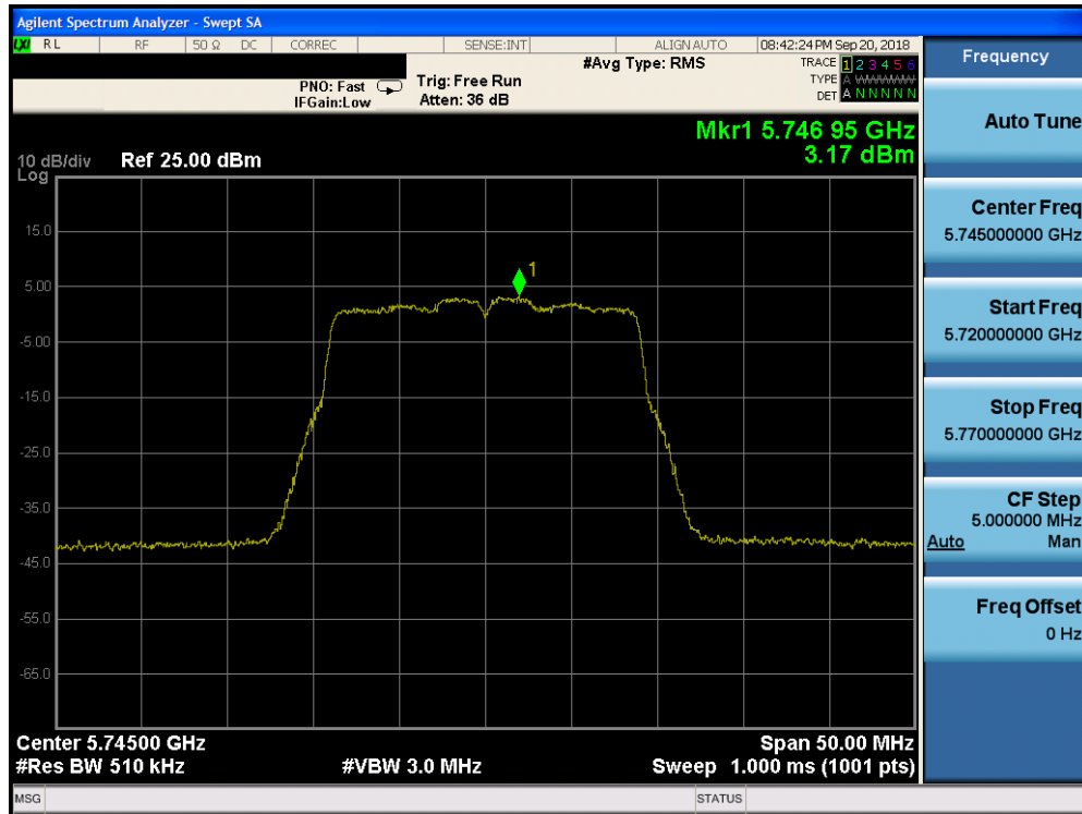
Plot 7-158. Power Spectral Density Plot CDD CORE 0 (20MHz BW 802.11n (UNII Band 3) – Ch. 149)
