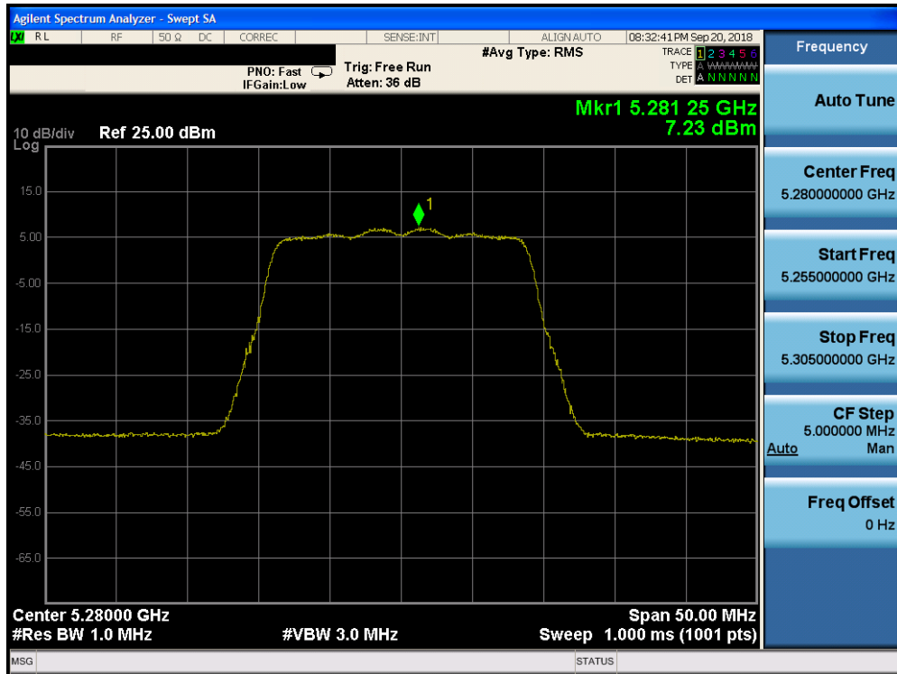
Plot 7-132. Power Spectral Density Plot CDD CORE 0 (20MHz BW 802.11n (UNII Band 2A) – Ch. 56)
