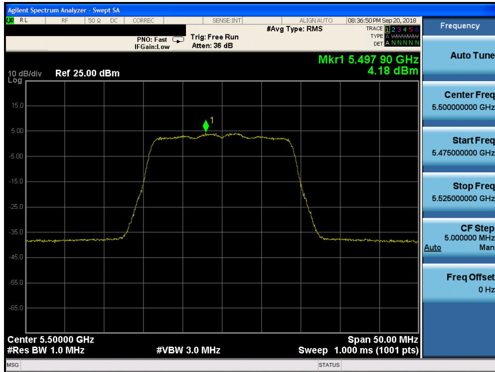
Plot 7-142. Power Spectral Density Plot CDD CORE 0 (20MHz BW 802.11n (UNII Band 2C) – Ch. 100)
