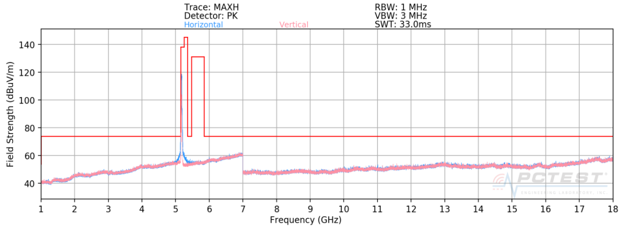
Plot 7-194. Radiated Spurious Plot above 1GHz CDD (802.11n – U1 Ch. 36)
