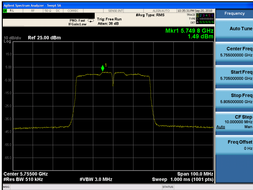
Plot 7-165. Power Spectral Density Plot CDD CORE 1 (40MHz BW 802.11n (UNII Band 3) – Ch. 151)
