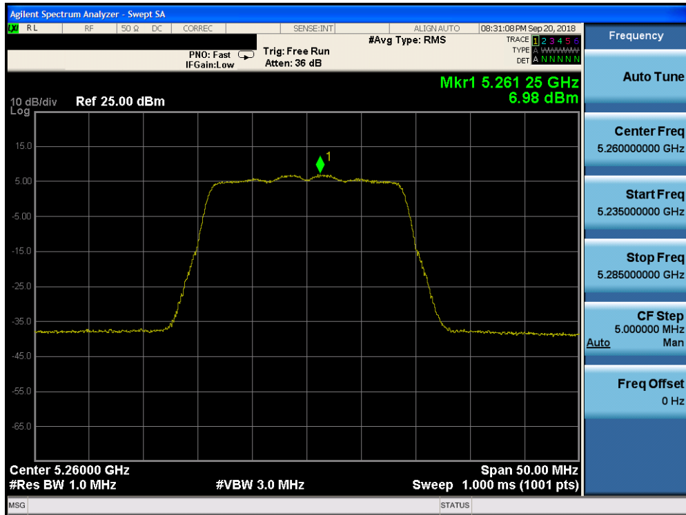
Plot 7-130. Power Spectral Density Plot CDD CORE 0 (20MHz BW 802.11n (UNII Band 2A) – Ch. 52)
