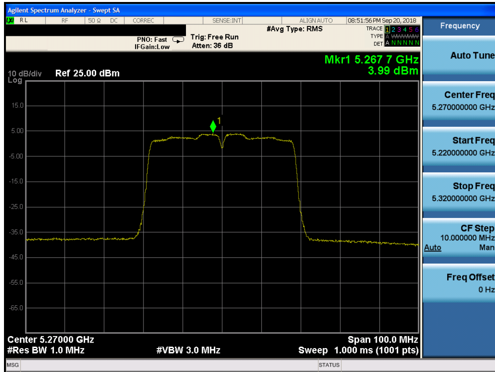
Plot 7-136. Power Spectral Density Plot CDD CORE 0 (40MHz BW 802.11n (UNII Band 2A) – Ch. 54)
