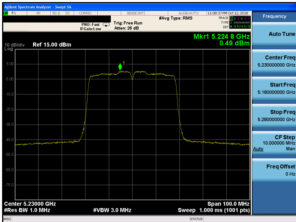
Plot 7-117. Power Spectral Density Plot CDD CORE 1 (40MHz BW 802.11n (UNII Band 1) – Ch. 46) - ISED
