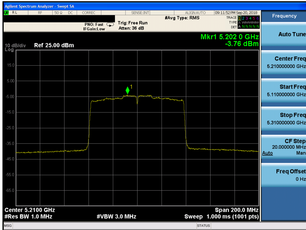
Plot 7-128. Power Spectral Density Plot CDD CORE 0 (80MHz BW 802.11ac (UNII Band 1) – Ch. 42)
