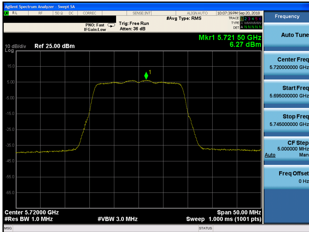
Plot 7-147. Power Spectral Density Plot CDD CORE 1 (20MHz BW 802.11n (UNII Band 2C) – Ch. 144)
