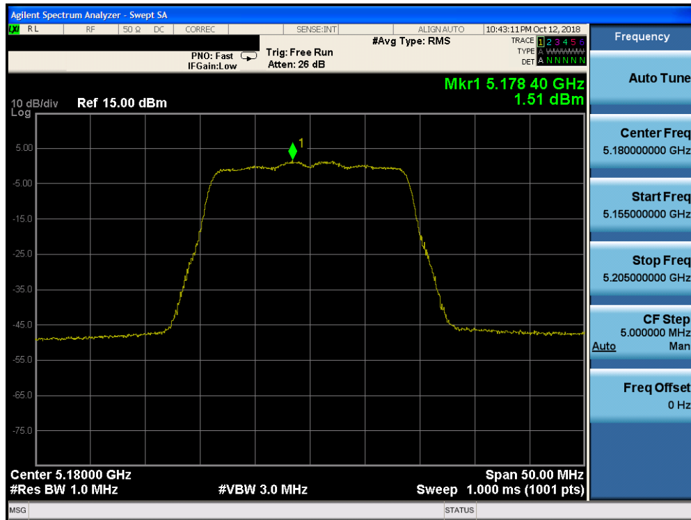
Plot 7-108. Power Spectral Density Plot CDD CORE 0 (20MHz BW 802.11n (UNII Band 1) – Ch. 36) - ISED
