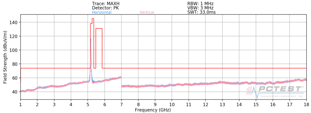
Plot 7-170. Radiated Spurious Plot above 1GHz SISO CORE0 (802.11n – U1 Ch. 36)
