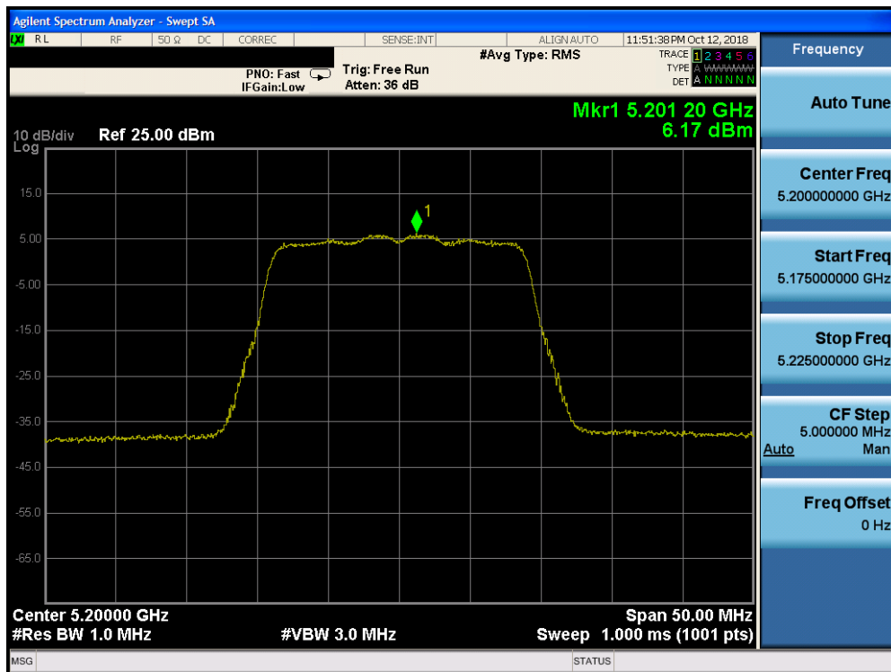
Plot 7-54. Power Spectral Density Plot SISO CORE0 (20MHz BW 802.11n (UNII Band 1) – Ch. 40) - ISD
