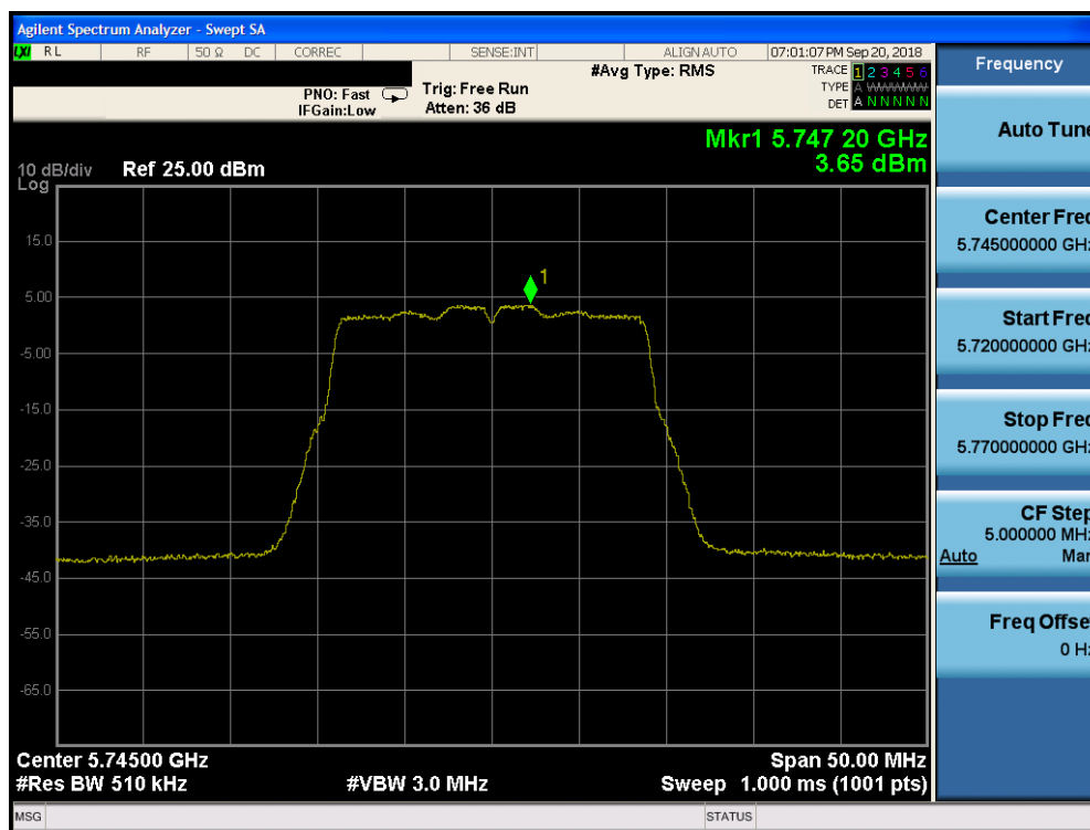
Plot 7-102. Power Spectral Density Plot SISO CORE1 (20MHz BW 802.11n (UNII Band 3) – Ch. 149)
