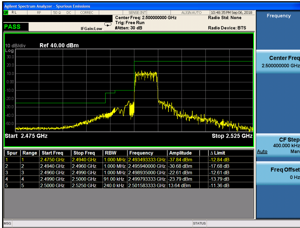
Plot 7-300. Lower ACP Plot (Band 7 – 5.0MHz QPSK – RB Size 25)
