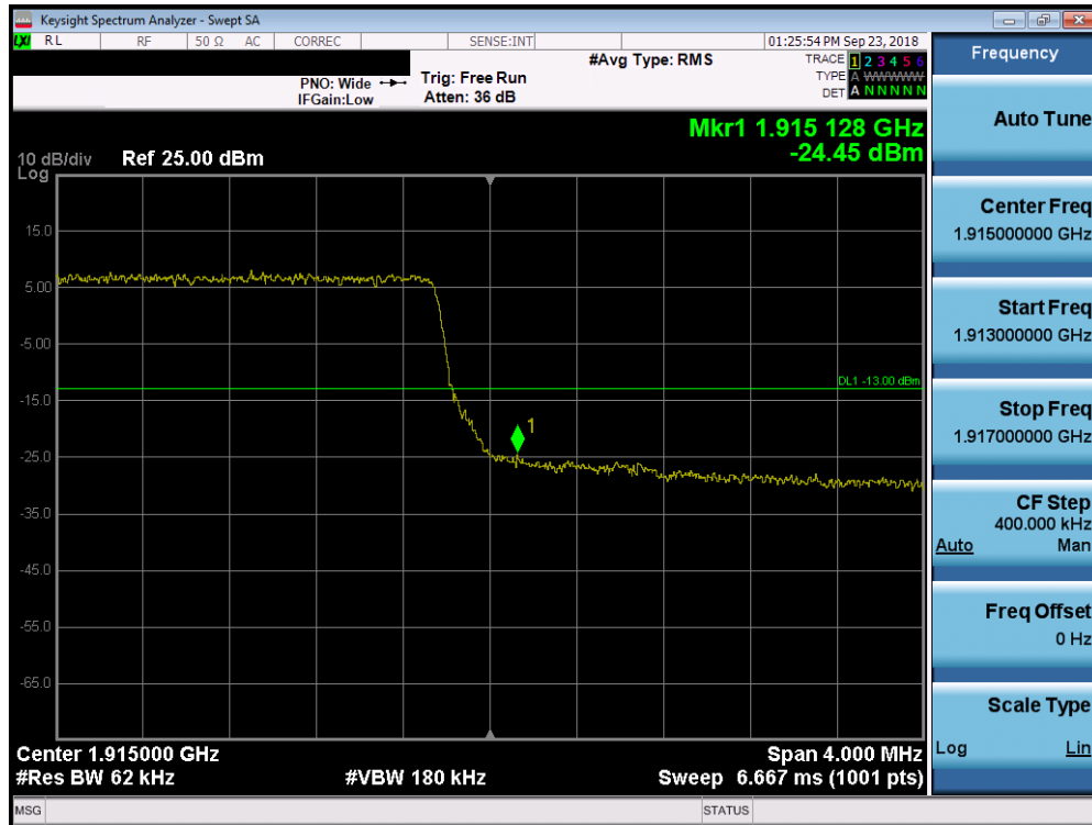
Plot 7-278. Upper Band Edge Plot (Band 25 – 5.0MHz QPSK – RB Size 25)
