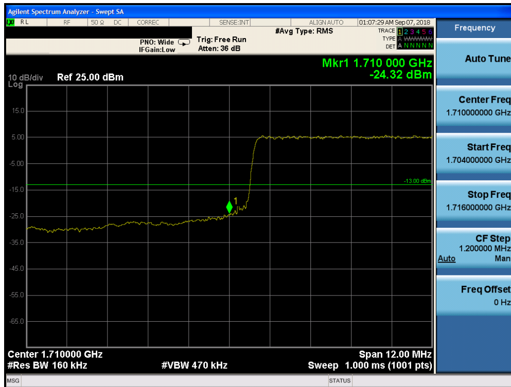
Plot 7-236. Lower Band Edge Plot (Band 66 – 15.0MHz QPSK – RB Size 75)
