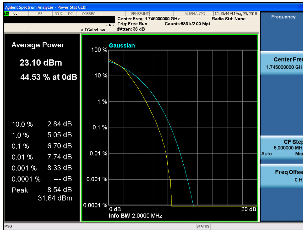
Plot 7-335. PAR Plot (Band 66 – 1.4MHz 16-QAM – RB Size 6)
