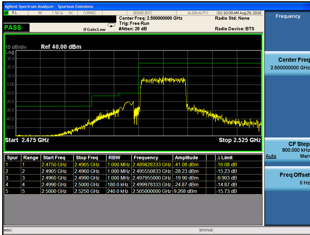
Plot 7-302. Lower ACP Plot (Band 7 – 10.0MHz QPSK – RB Size 50)
