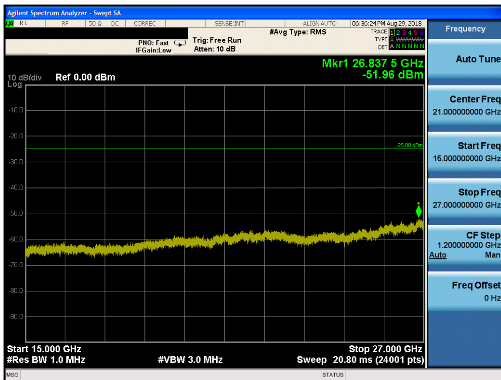
Plot 7-144. Conducted Spurious Plot (Band 7 - 20.0MHz QPSK - RB Size 1, RB Offset 0 - Mid Channel)
