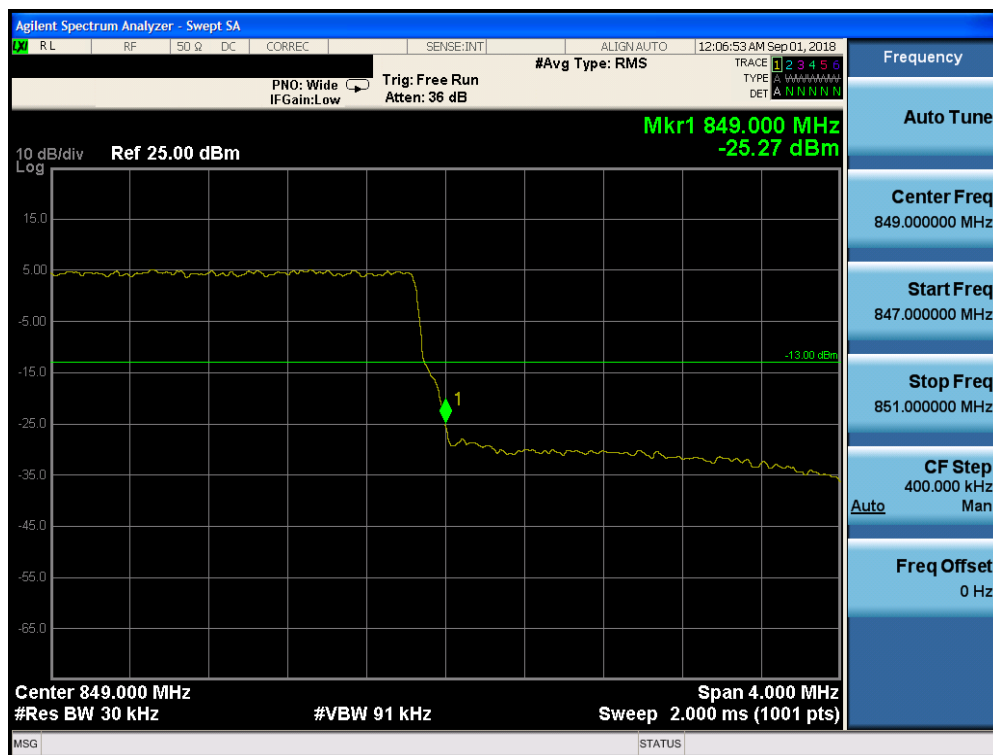
Plot 7-190. Upper Band Edge Plot (Band 26 – 3.0MHz QPSK – RB Size 15)
