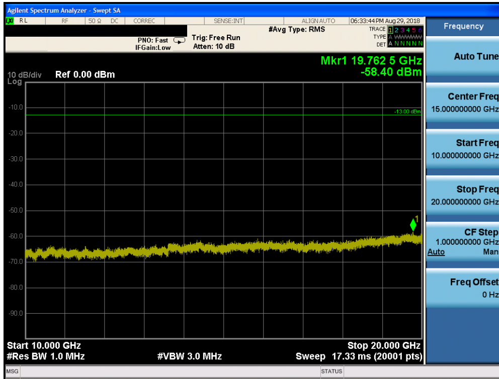
Plot 7-120. Conducted Spurious Plot (Band 66/4 – 20.0MHz QPSK – RB Size 1, RB Offset 0 – Low Channel)
