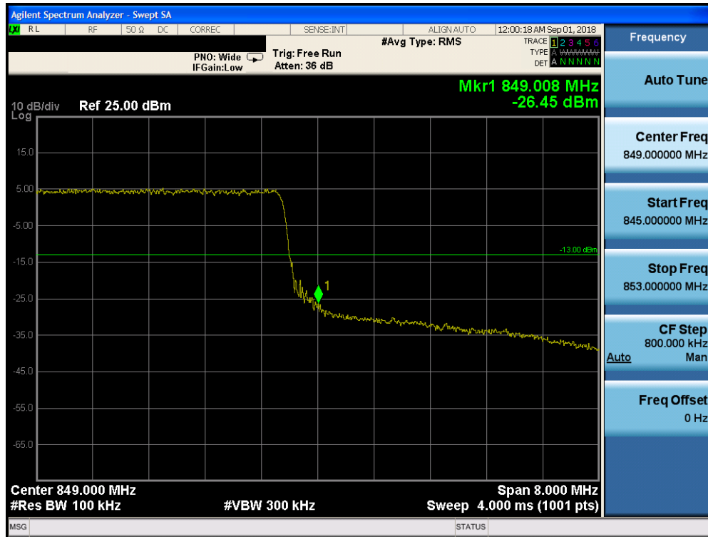
Plot 7-195. Upper Band Edge Plot (Band 26 – 10.0MHz QPSK – RB Size 50)
