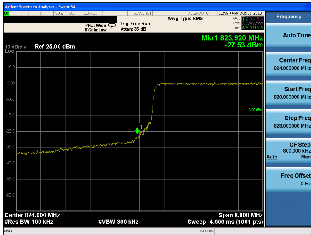
Plot 7-194. Lower Band Edge Plot (Band 26 - 10.0MHz QPSK - RB Size 50)
