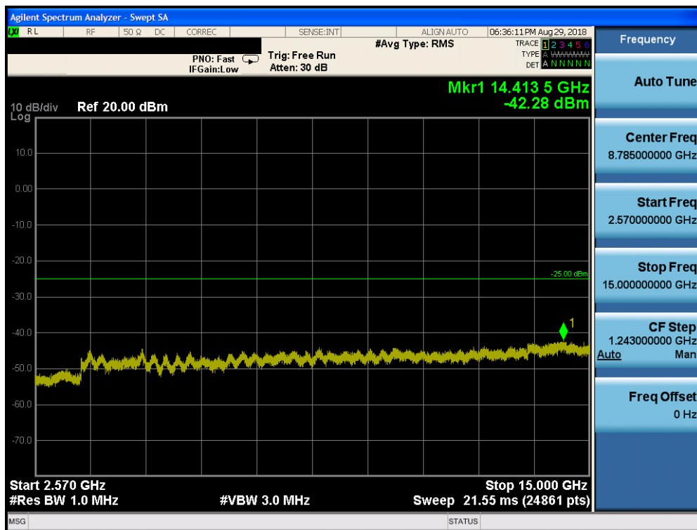
Plot 7-143. Conducted Spurious Plot (Band 7 - 20.0MHz QPSK - RB Size 1, RB Offset 0 - Mid Channel)
