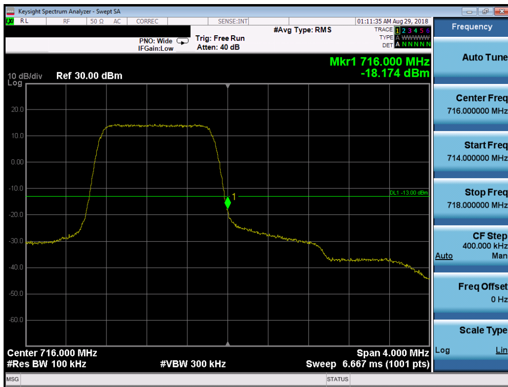
Plot 7-158. Upper Band Edge Plot (Band 12 – 1.4MHz QPSK – RB Size 6)
