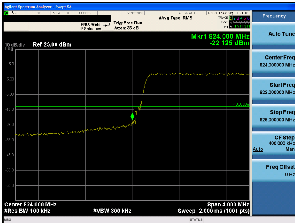
Plot 7-192. Lower Band Edge Plot (Band 26 - 5.0MHz QPSK - RB Size 25)
