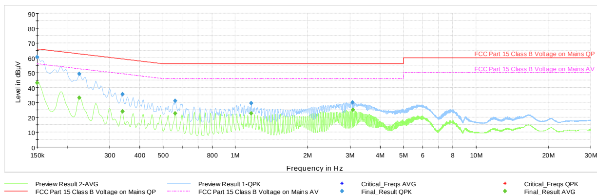
Plot 7-33. AC Line Conducted Plot with Bluetooth LE (L1 – 1Mbps, with Laptop)
