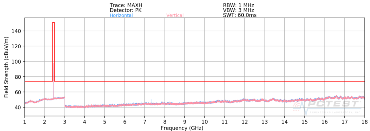
Plot 7-24. Radiated Spurious Plot Above 1GHz (1Mbps – Ch. 19)
