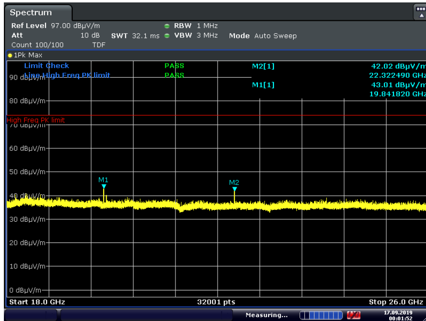
Plot 7-26. Radiated Spurious Plot Above 18GHz (1Mbps – Ch. 39, Ant. Pol. H)
