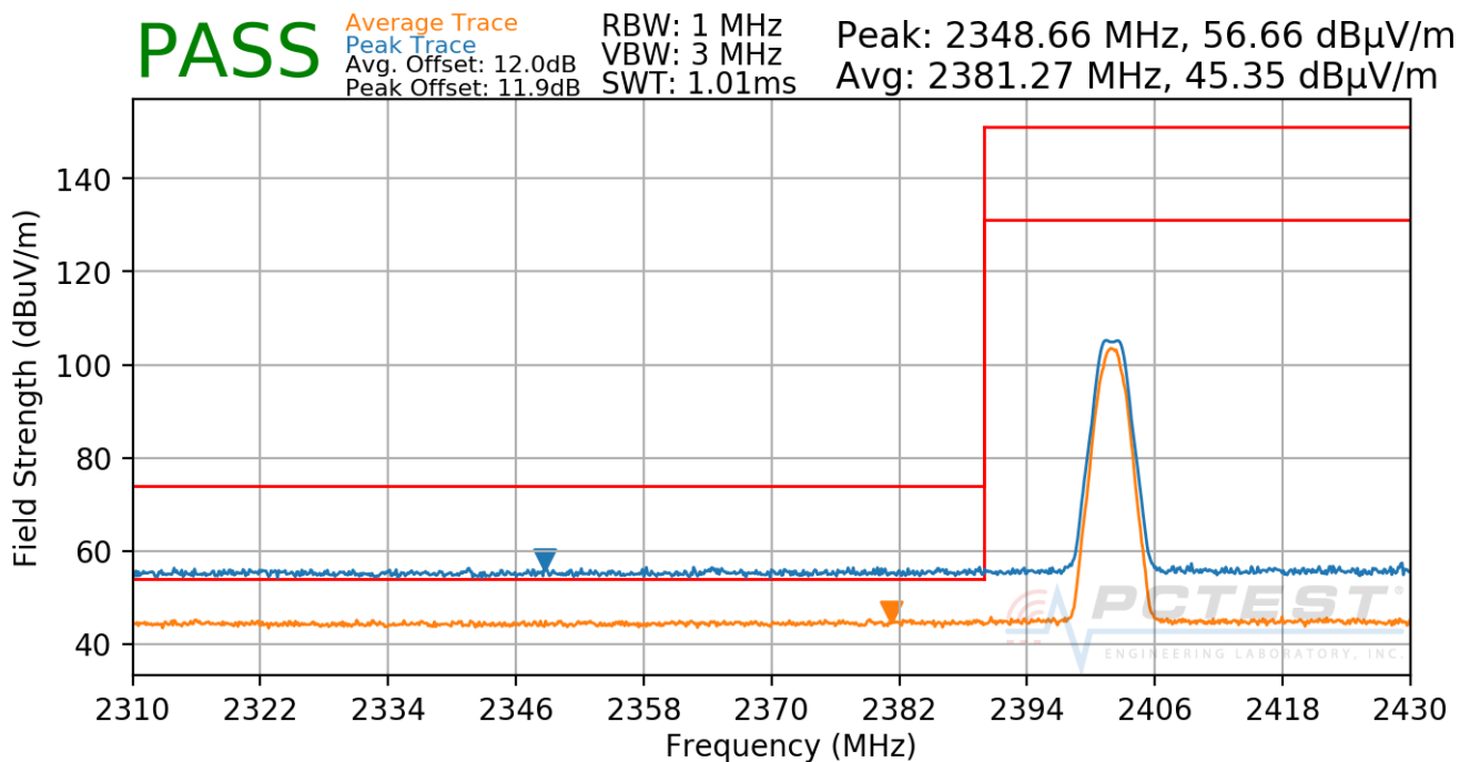
Plot 7-29. Radiated Restricted Lower Band Edge Measurement (Average & Peak)
