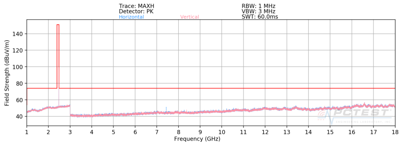
Plot 7-25. Radiated Spurious Plot Above 1GHz (1Mbps – Ch. 39)
