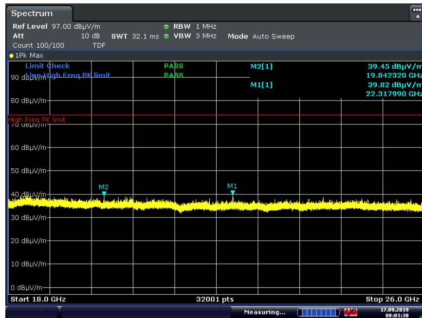
Plot 7-27. Radiated Spurious Plot Above 18GHz (1Mbps – Ch. 39, Ant. Pol. V)
