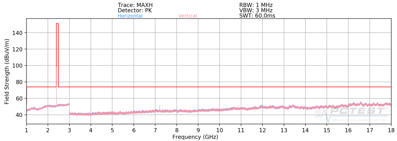
Plot 7-23. Radiated Spurious Plot Above 1GHz (1Mbps – Ch. 0)
