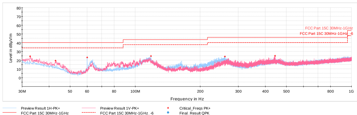
Plot 7-32. Radiated Spurious Plot below 1GHz (1Mbps – Ch.0, Pol. H & V, with Laptop)
