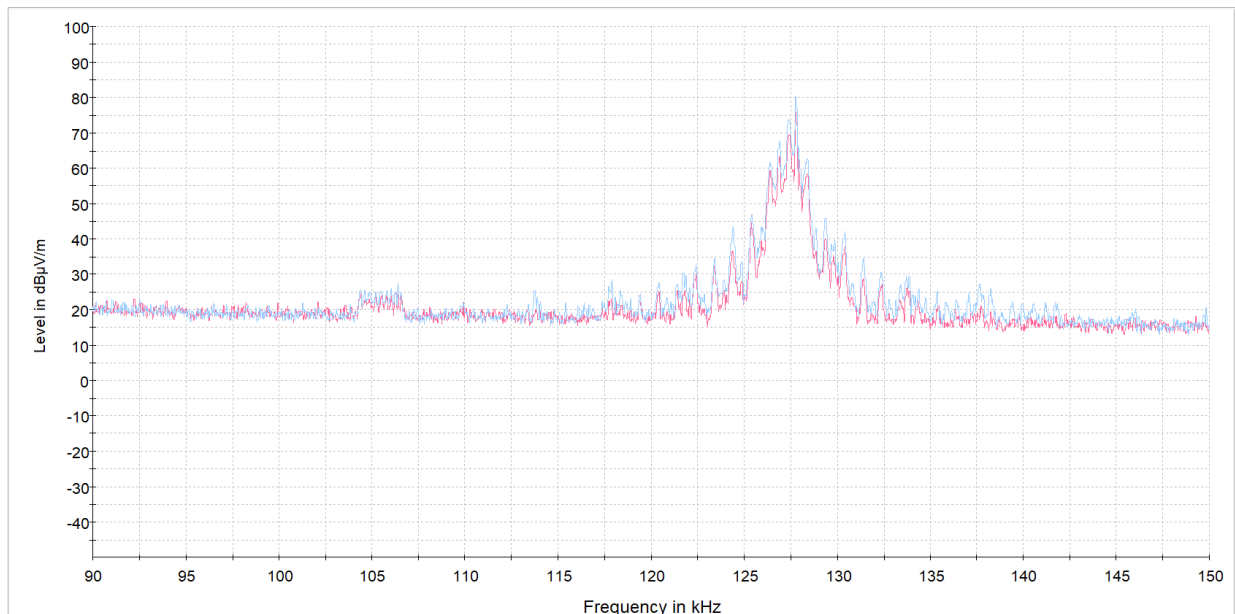
Plot 7-2. Radiated Restricted Lower Band Edge Measurement (Peak)
