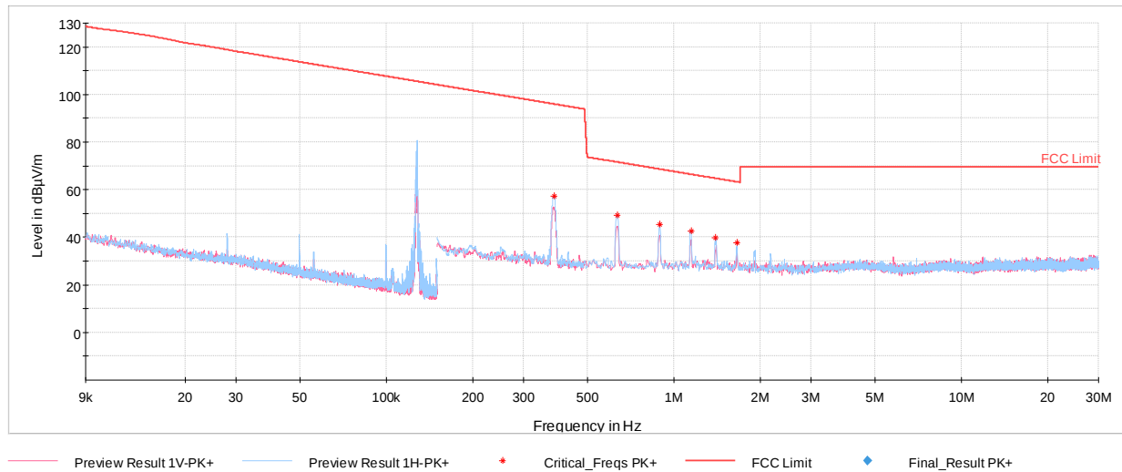
Plot 7-3. Radiated Spurious Plot from 9kHz – 30MHz (Loop Antenna X & Y)
