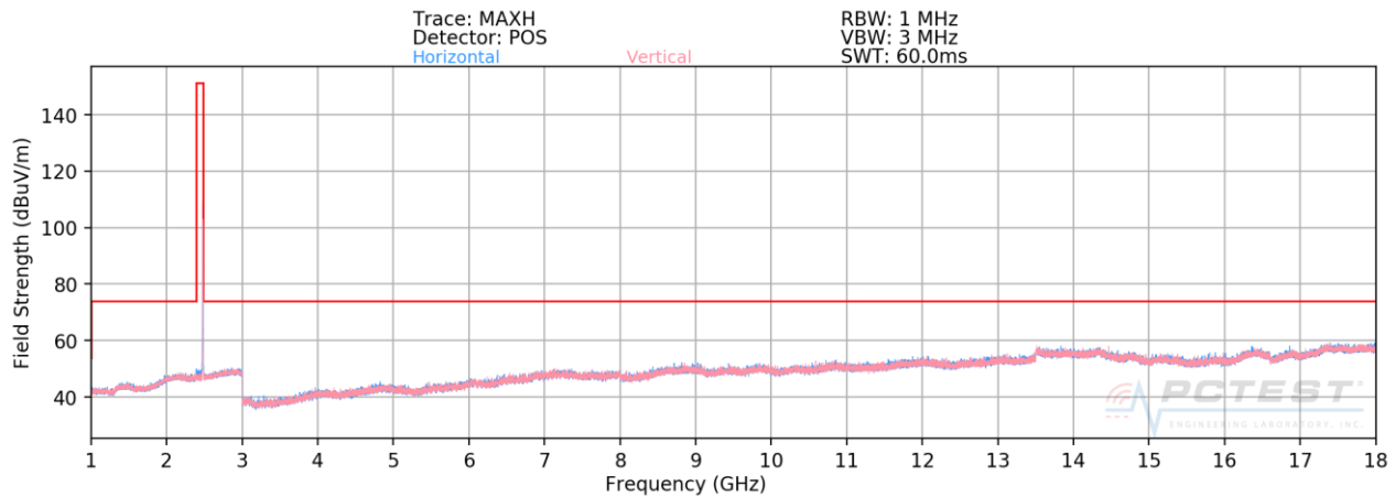
Plot 7-90. Radiated Spurious Plot Above 1GHz ANT0 (8Mbps, HDR8 ePA – Ch. 75, Ant. Pol. H & V)
