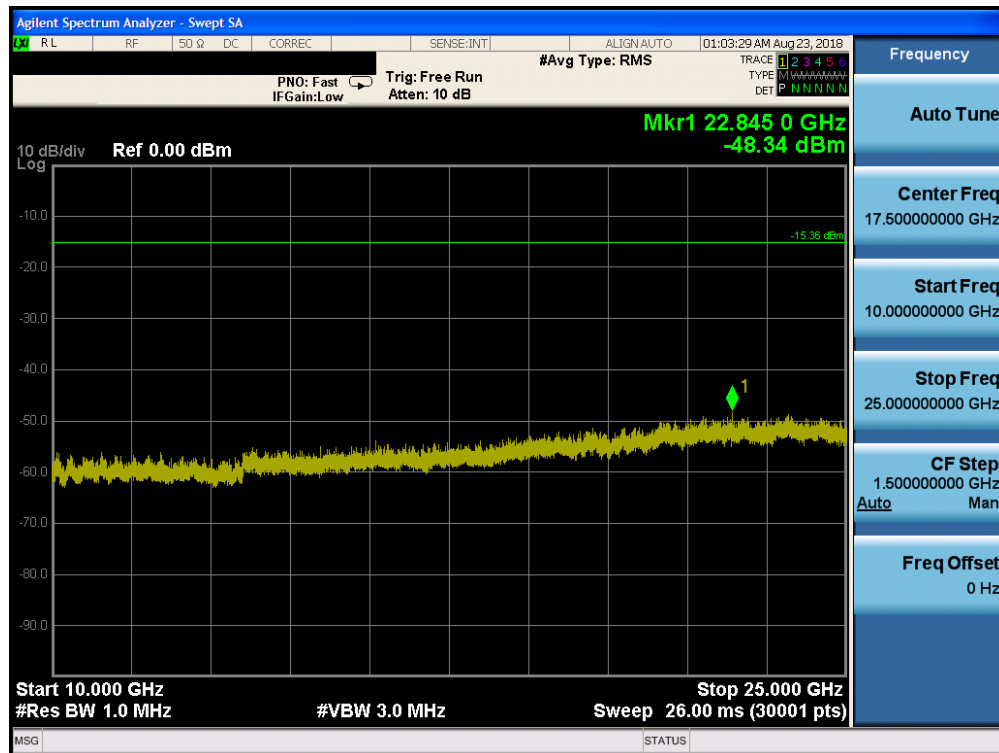
Plot 7-84. Conducted Spurious Plot ANT2 (Bluetooth (HDR4), 4Mbps, ePA – Ch. 75)
