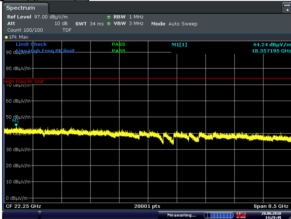
Plot 7-103. Radiated Spurious Plot Above 18GHz ANT0 (8Mbps, HDR8 ePA Ch. 38, Ant. Pol. H)
