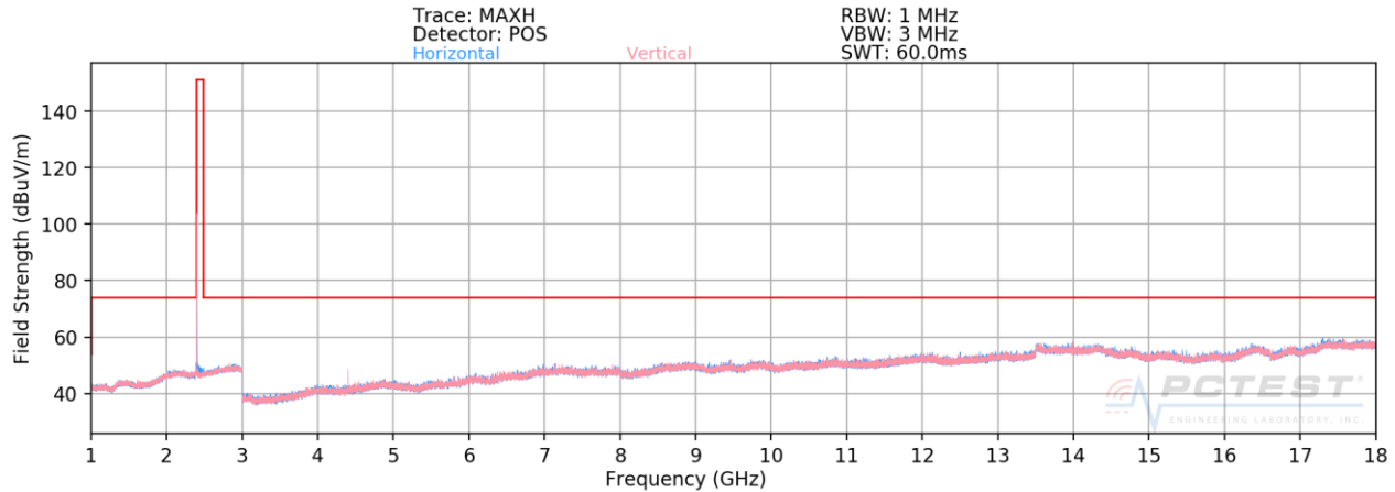
Plot 7-85. Radiated Spurious Plot Above 1GHz ANT0 (4Mbps, HDR4 ePA – Ch. 1, Ant. Pol. H & V)
