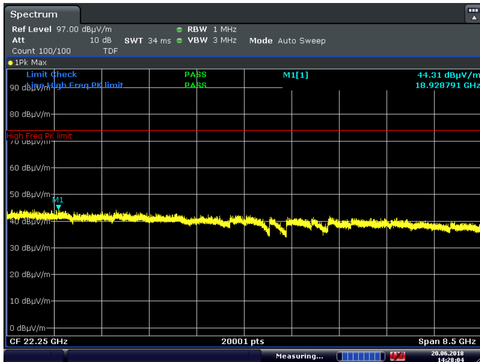
Plot 7-104. Radiated Spurious Plot Above 18GHz ANT0 (8Mbps, HDR8 ePA Ch.38, Ant. Pol. V)
