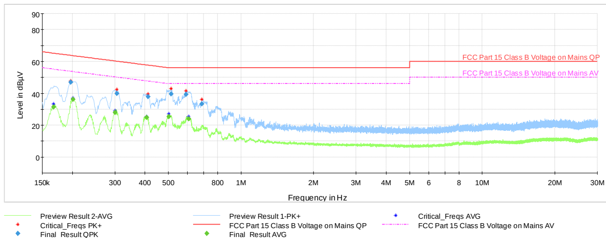
Plot 7-118. Line Conducted Plot with Bluetooth HDR ePA Ch. 38 (L1, with AC/DC Adapter)
