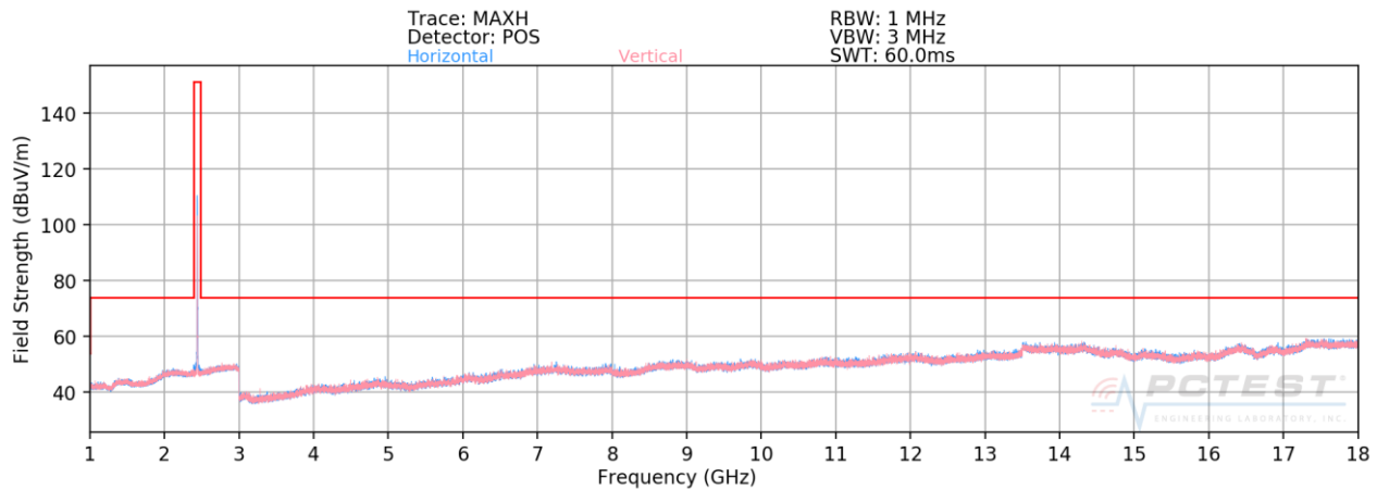
Plot 7-89. Radiated Spurious Plot Above 1GHz ANT0 (8Mbps, HDR8 ePA – Ch. 38, Ant. Pol. H & V)
