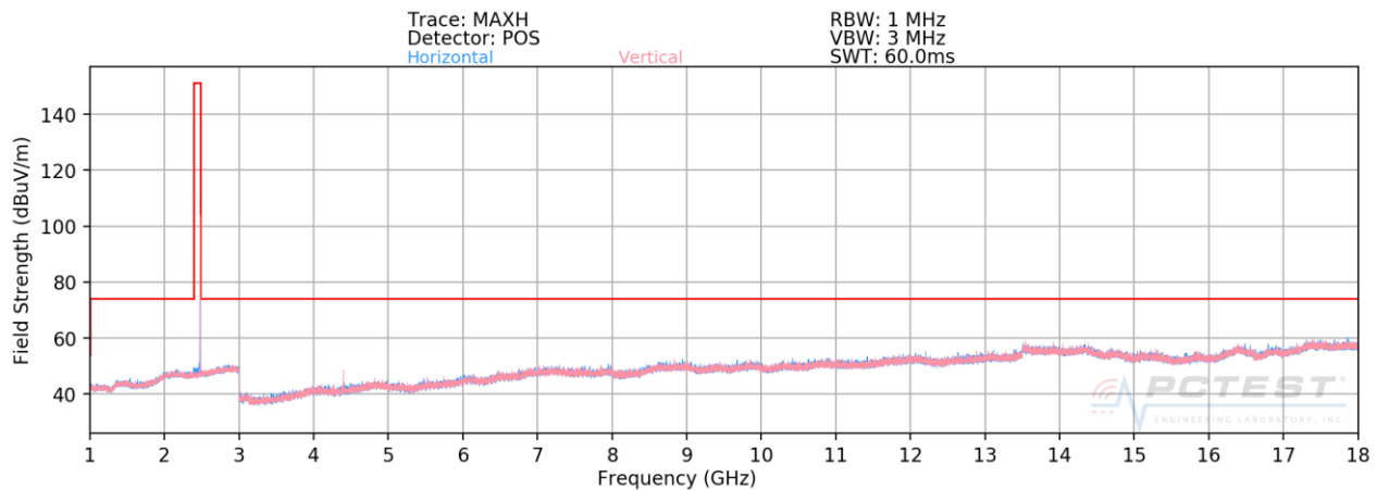
Plot 7-87. Radiated Spurious Plot Above 1GHz ANT0 (4Mbps, HDR4 ePA – Ch. 75, Ant. Pol. H & V)
