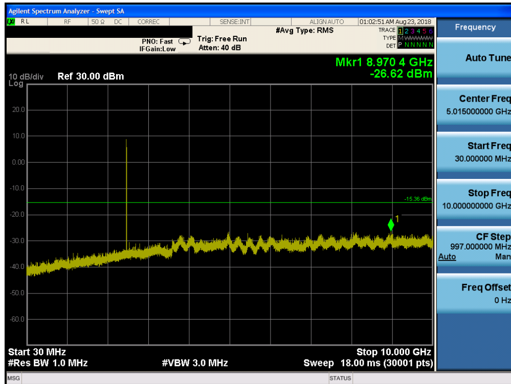
Plot 7-83. Conducted Spurious Plot ANT2 (Bluetooth (HDR4), 4Mbps, ePA – Ch. 75)
