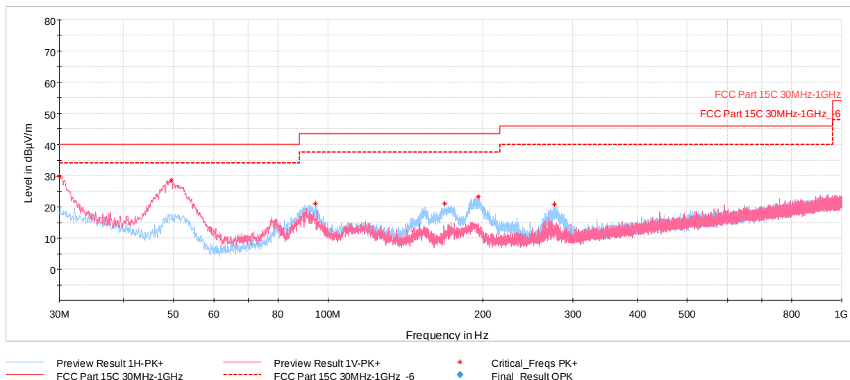
Plot 7-117. Radiated Spurious Plot below 1GHz (4Mbps, HDR4 ePA, Pol. H & V, with AC/DC Adapter)
