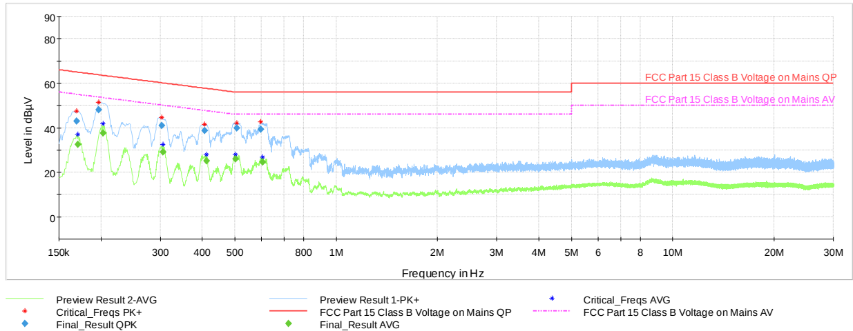
Plot 7-119. Line Conducted Plot with Bluetooth HDR ePA Ch. 38 (N, with AC/DC Adapter)
