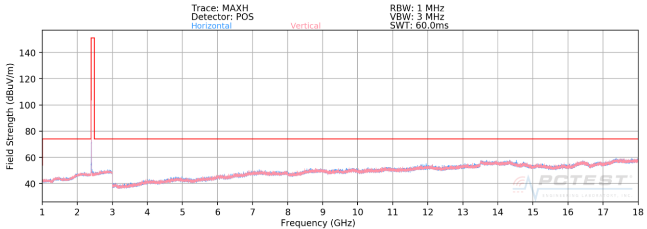
Plot 7-88. Radiated Spurious Plot Above 1GHz ANT0 (8Mbps, HDR8 ePA – Ch. 1, Ant. Pol. H & V)
