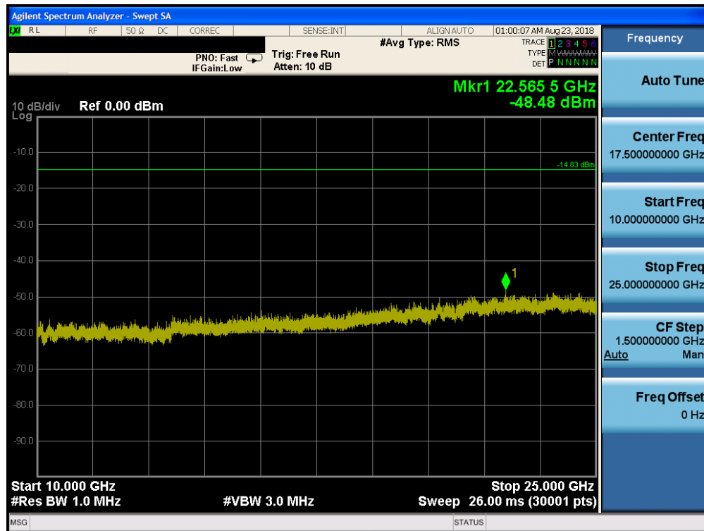
Plot 7-82. Conducted Spurious Plot ANT2 (Bluetooth (HDR4), 4Mbps, ePA – Ch. 38)
