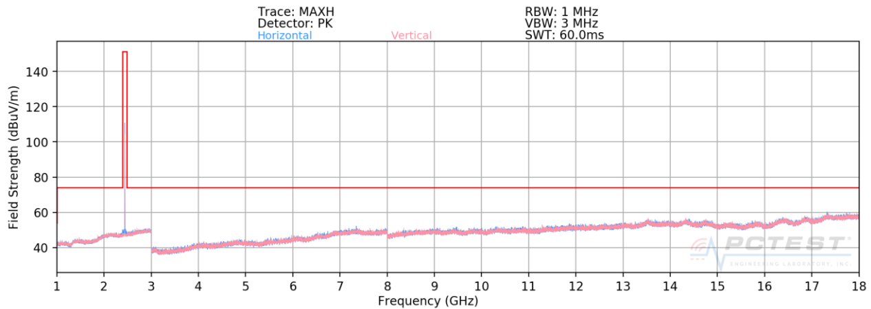
Plot 7-86. Radiated Spurious Plot Above 1GHz ANT0 (4Mbps, HDR4 ePA – Ch. 38, Ant. Pol. H & V)
