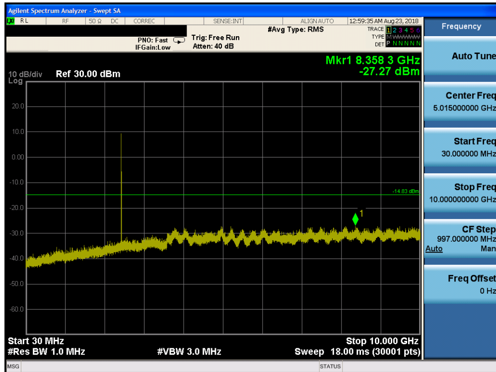
Plot 7-81. Conducted Spurious Plot ANT2 (Bluetooth (HDR4), 4Mbps, ePA – Ch. 38)
