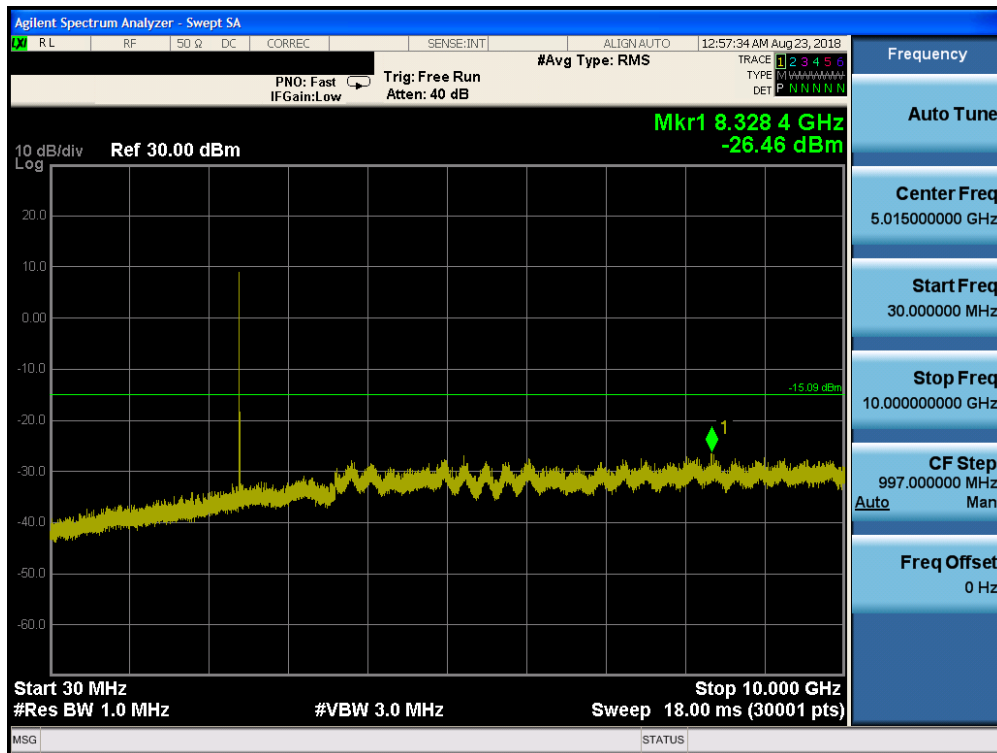
Plot 7-79. Conducted Spurious Plot ANT2 (Bluetooth (HDR4), 4Mbps, ePA – Ch. 1)
