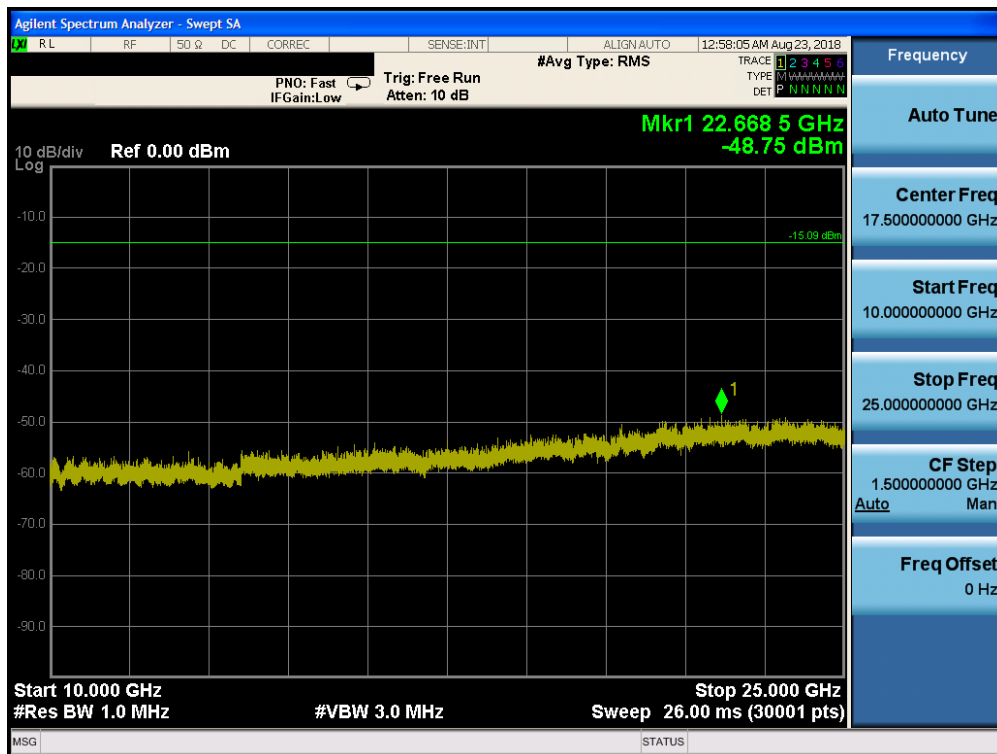
Plot 7-80. Conducted Spurious Plot ANT2 (Bluetooth (HDR4), 4Mbps, ePA – Ch. 1)
