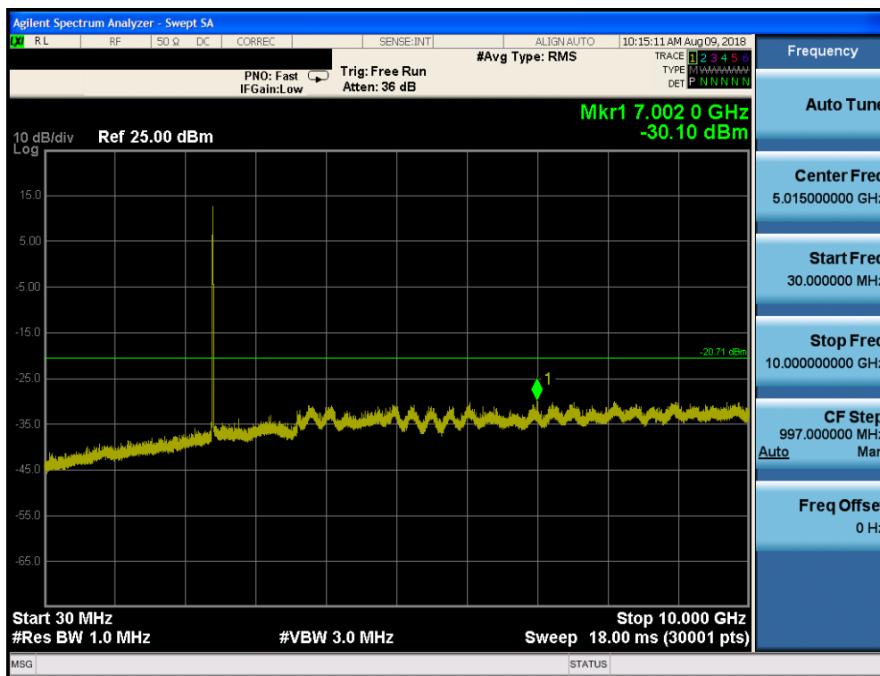
Plot 7-121. Conducted Spurious Plot SISO Core 1 Primary (802.11b – Ch. 1)
