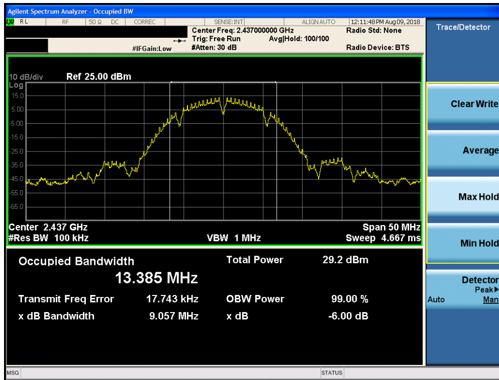
Plot 7-20. 6dB Bandwidth Plot SISO Core 1 Diversity (802.11b – Ch. 6)
