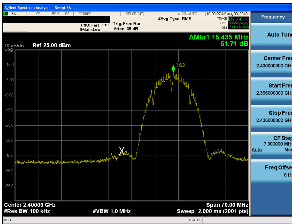
Plot 7-91. Band Edge Plot SISO Core 1 Primary (802.11b – Ch. 1)
