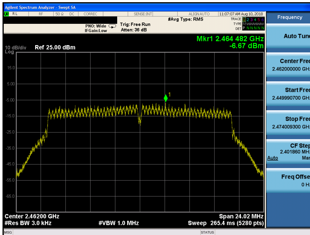
Plot 7-45. Power Spectral Density Plot SISO Core 1 Primary (802.11n (2.4GHz) – Ch. 11)
