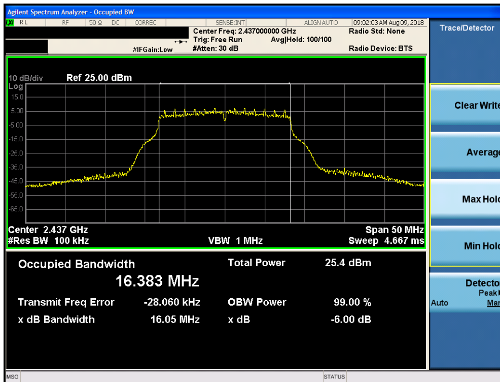
Plot 7-5. 6dB Bandwidth Plot SISO Core 0 (802.11g – Ch. 6)
