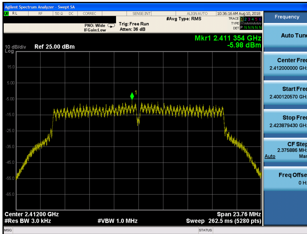
Plot 7-31. Power Spectral Density Plot SISO Core 0 (802.11g – Ch. 1)
