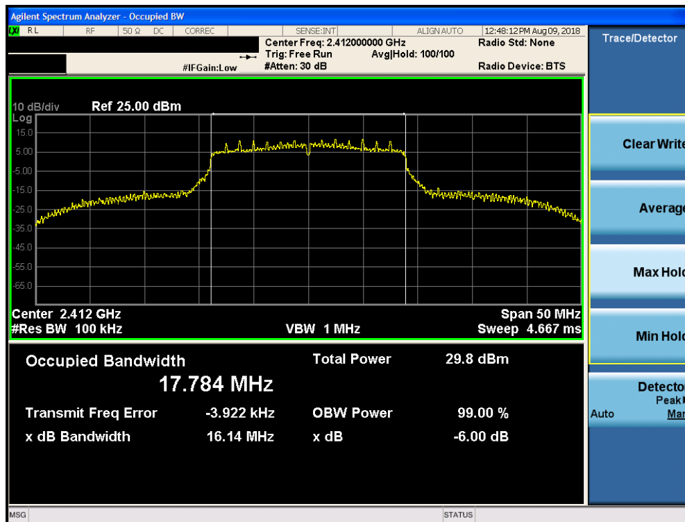
Plot 7-25. 6dB Bandwidth Plot SISO Core 1 Diversity (802.11n (2.4GHz) – Ch. 1)
