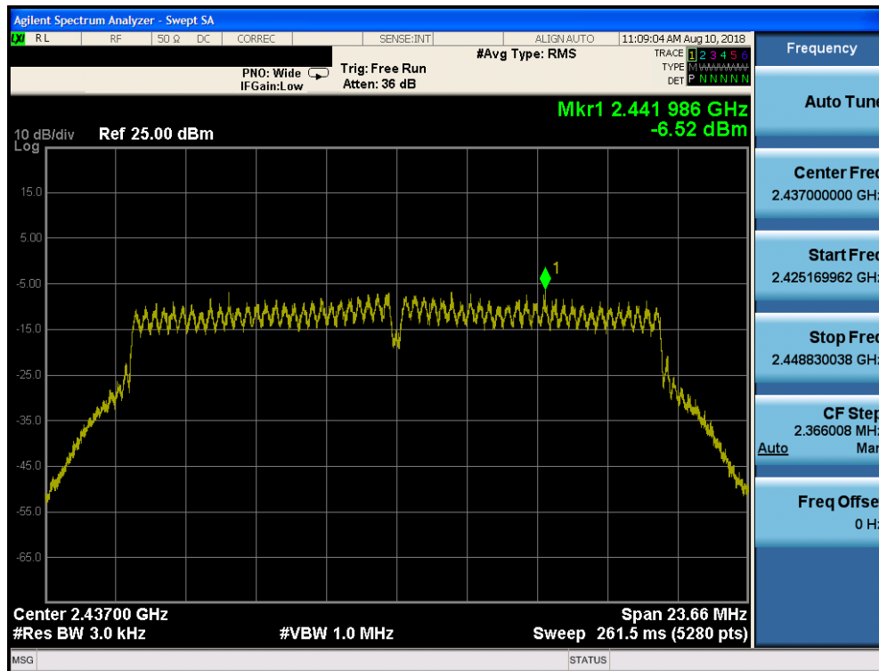
Plot 7-44. Power Spectral Density Plot SISO Core 1 Primary (802.11n (2.4GHz) – Ch. 6)
