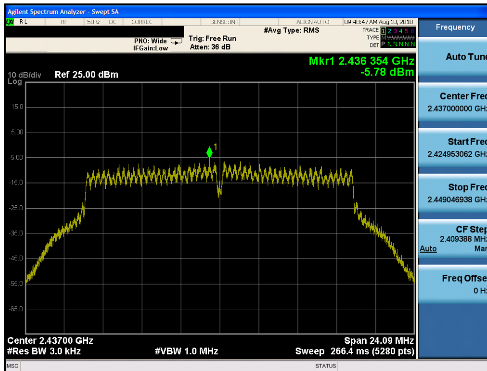
Plot 7-32. Power Spectral Density Plot SISO Core 0 (802.11g – Ch. 6)
