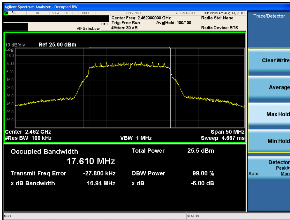
Plot 7-9. 6dB Bandwidth Plot SISO Core 0 (802.11n (2.4GHz) – Ch. 11)
