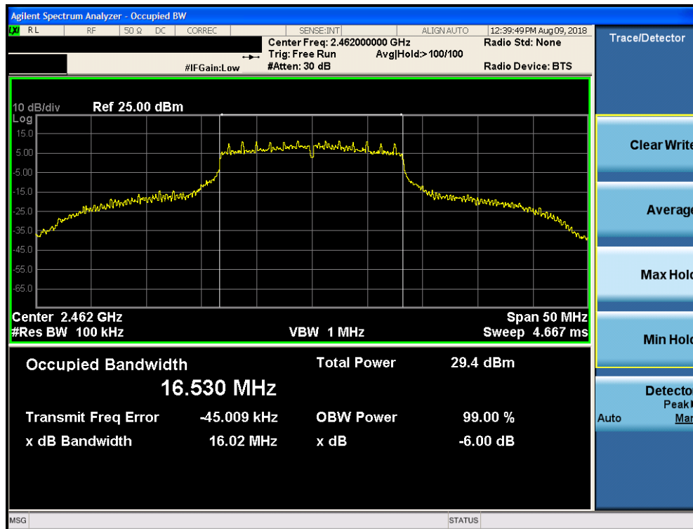
Plot 7-24. 6dB Bandwidth Plot SISO Core 1 Diversity (802.11g – Ch. 11)
