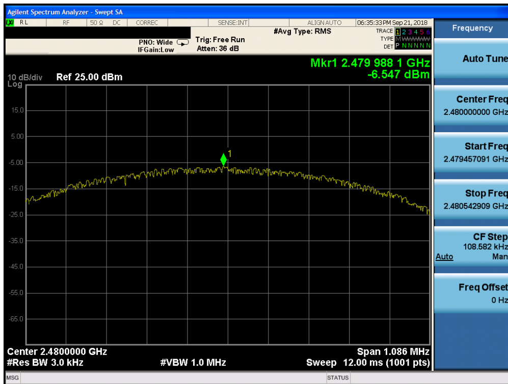
Plot 7-36. Power Spectral Density Plot (Bluetooth (LE), 1Mbps, iPA – Ch. 39, Antenna 1)
