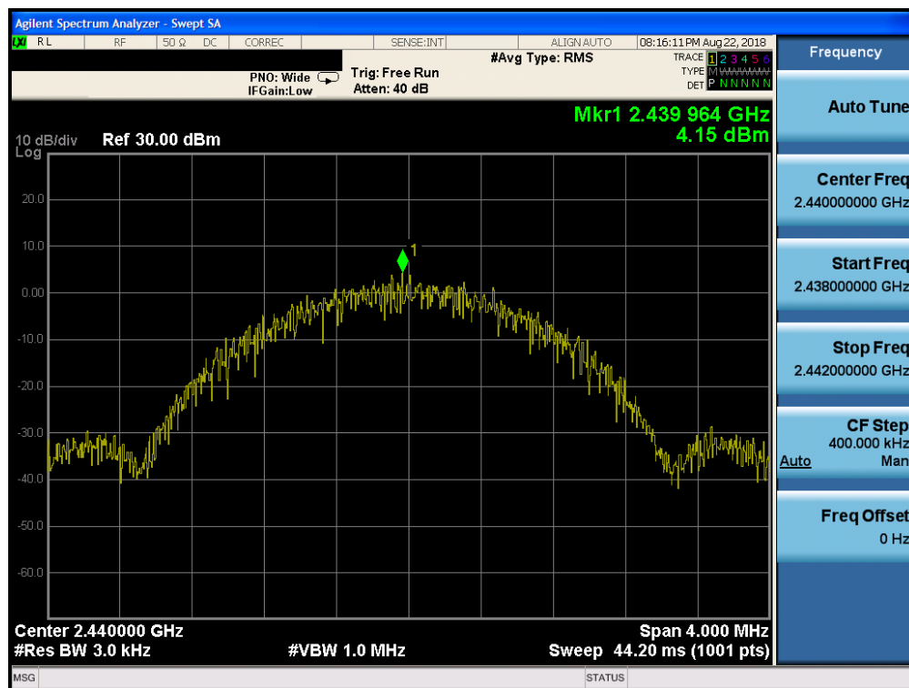
Plot 7-26. Power Spectral Density Plot (Bluetooth (LE), 2Mbps, ePA – Ch. 19, Antenna 0)
