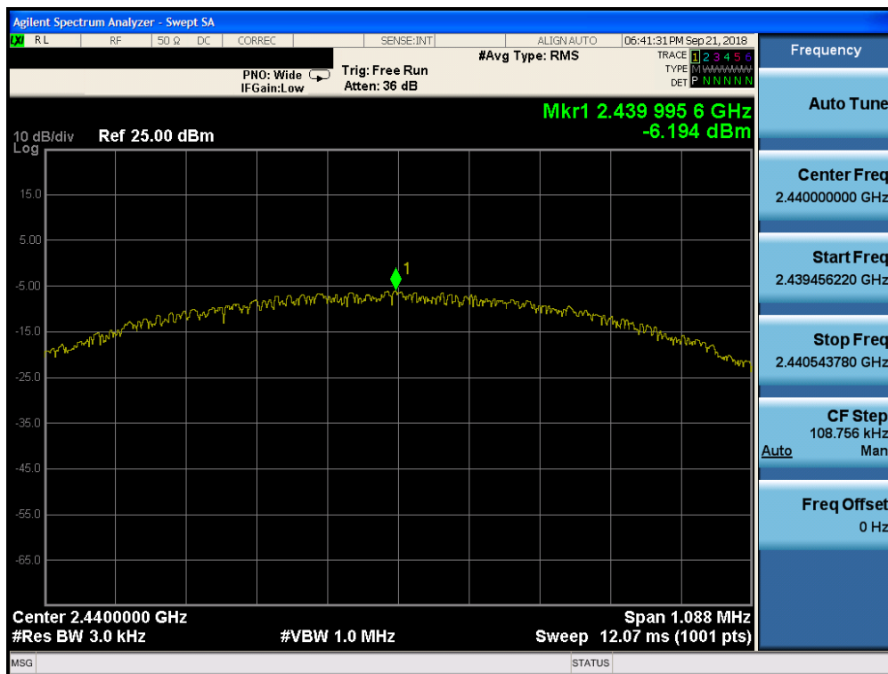
Plot 7-47. Power Spectral Density Plot (Bluetooth (LE), 1Mbps, iPA – Ch. 19, Antenna 2)
