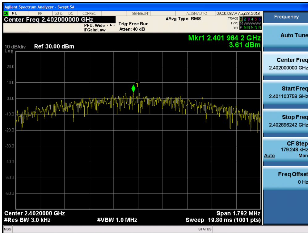
Plot 7-49. Power Spectral Density Plot (Bluetooth (LE), 2Mbps, ePA – Ch. 0, Antenna 2)
