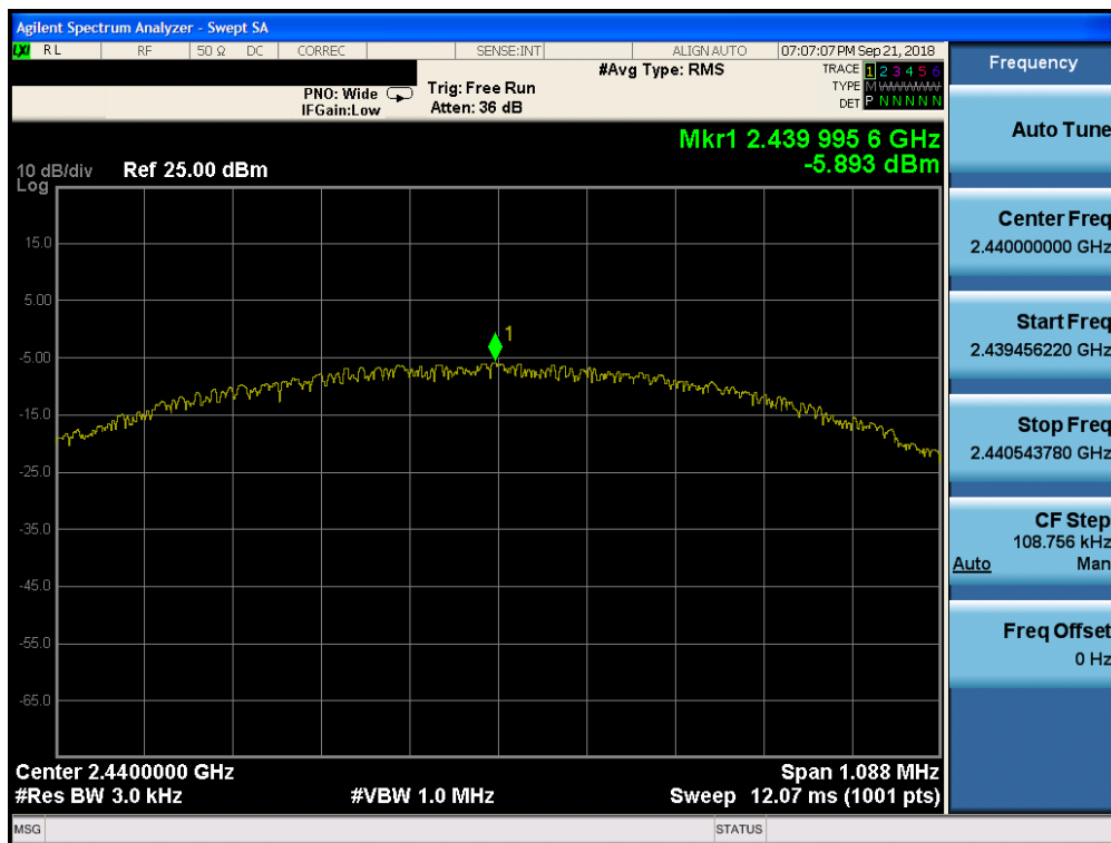
Plot 7-23. Power Spectral Density Plot (Bluetooth (LE), 1Mbps, iPA – Ch. 19, Antenna 0)
