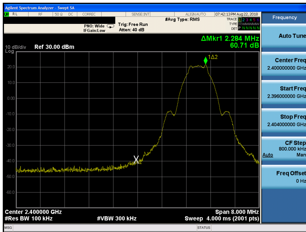
Plot 7-55. Band Edge Plot (Bluetooth (LE), ePA – Ch. 0, Antenna 0)
