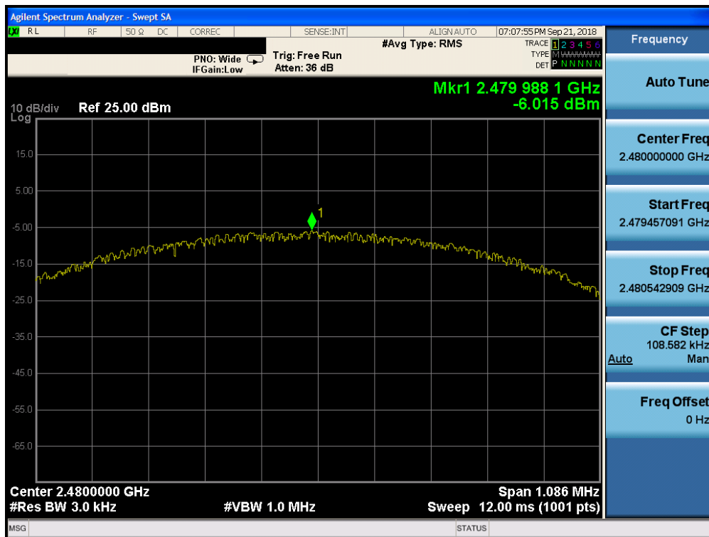
Plot 7-24. Power Spectral Density Plot (Bluetooth (LE), 1Mbps, iPA – Ch. 39, Antenna 0)
