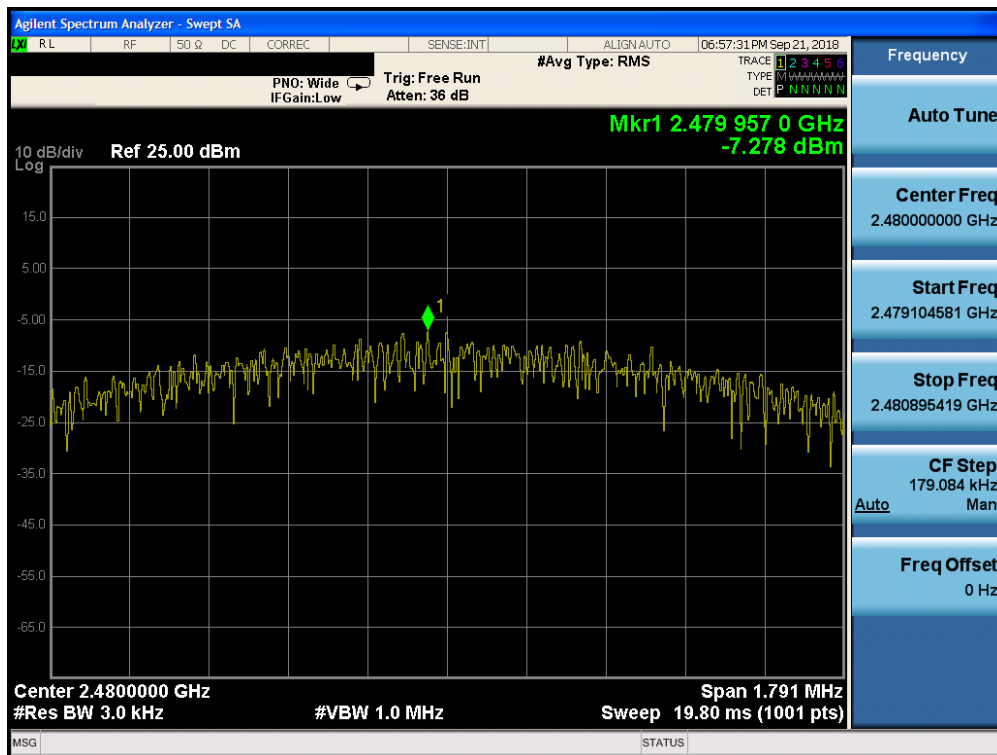
Plot 7-42. Power Spectral Density Plot (Bluetooth (LE), 2Mbps, iPA – Ch. 39, Antenna 1)
