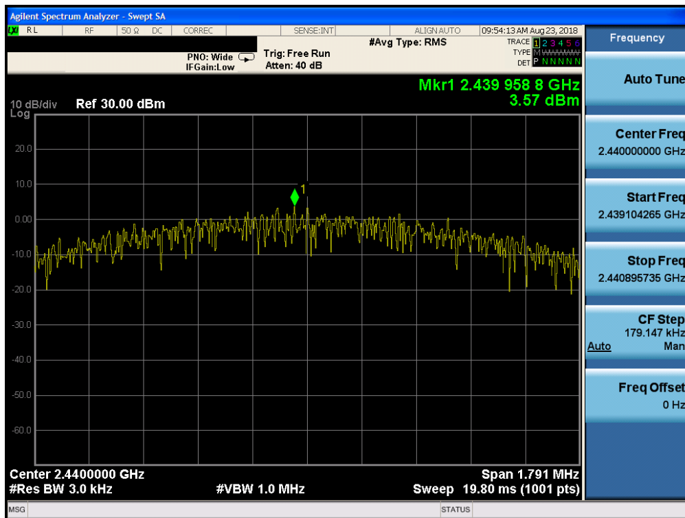
Plot 7-50. Power Spectral Density Plot (Bluetooth (LE), 2Mbps, ePA – Ch. 19, Antenna 2)
