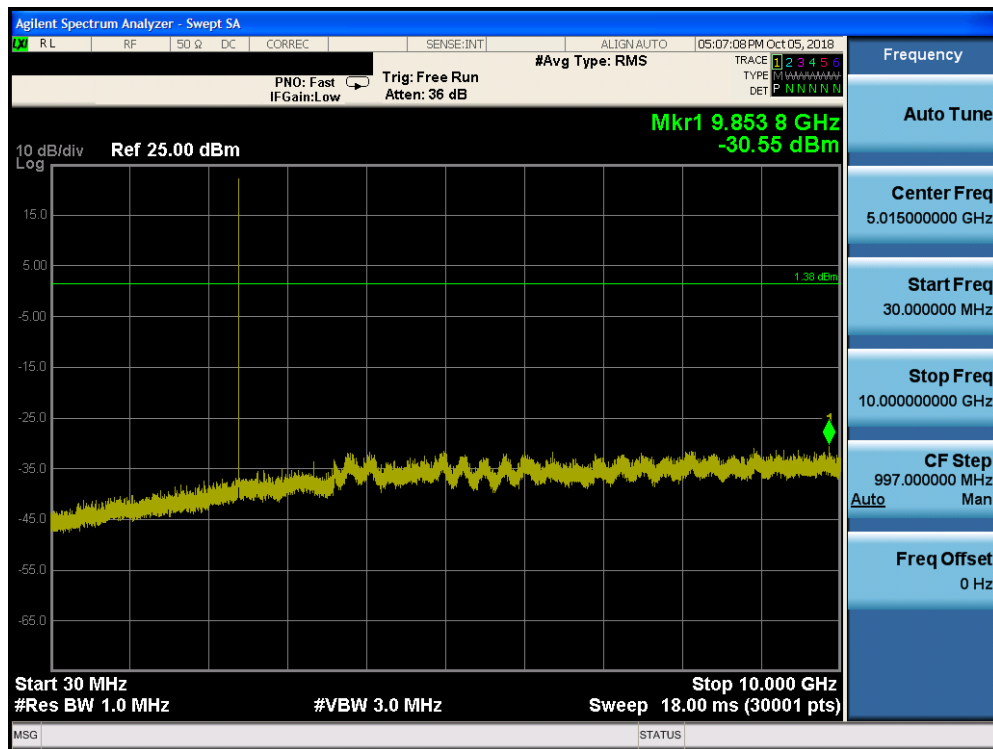
Plot 7-61. Conducted Spurious Plot (Bluetooth (LE), 1Mbps, ePA – Ch. 0, Antenna 0)
