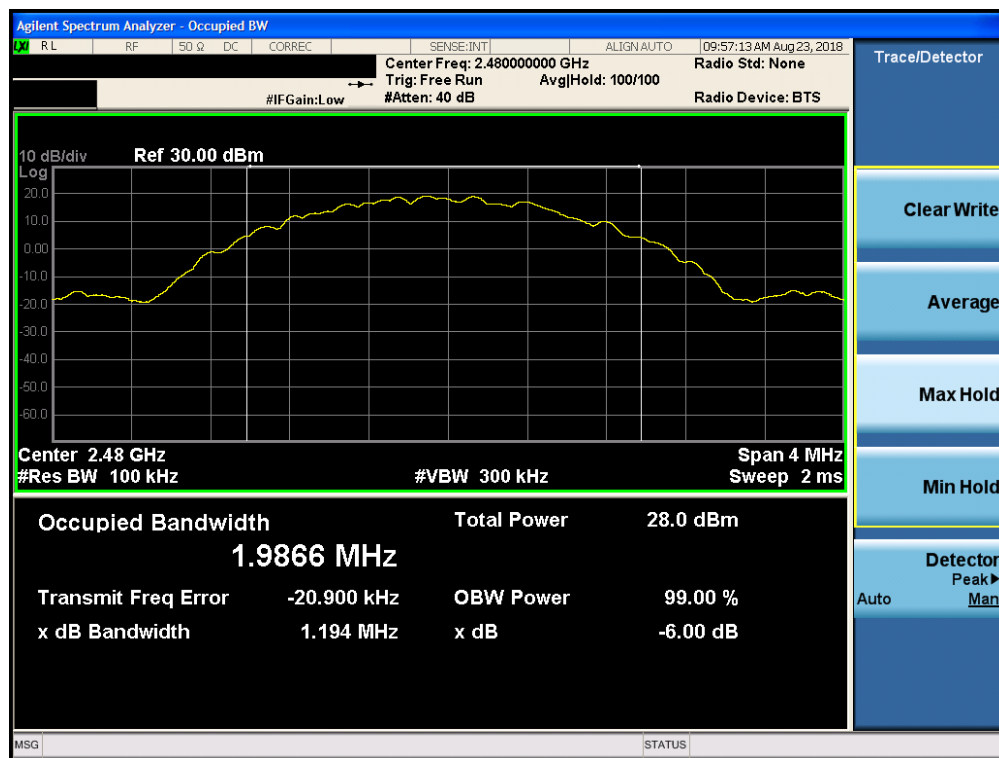
Plot 7-18. 6dB Bandwidth Plot (Bluetooth (LE), 2Mbps, ePA – Ch. 39, Antenna 2)
