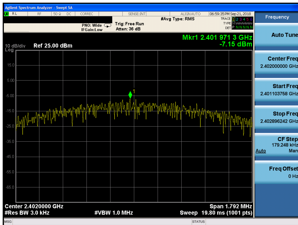
Plot 7-52. Power Spectral Density Plot (Bluetooth (LE), 2Mbps, iPA – Ch. 0, Antenna 2)
