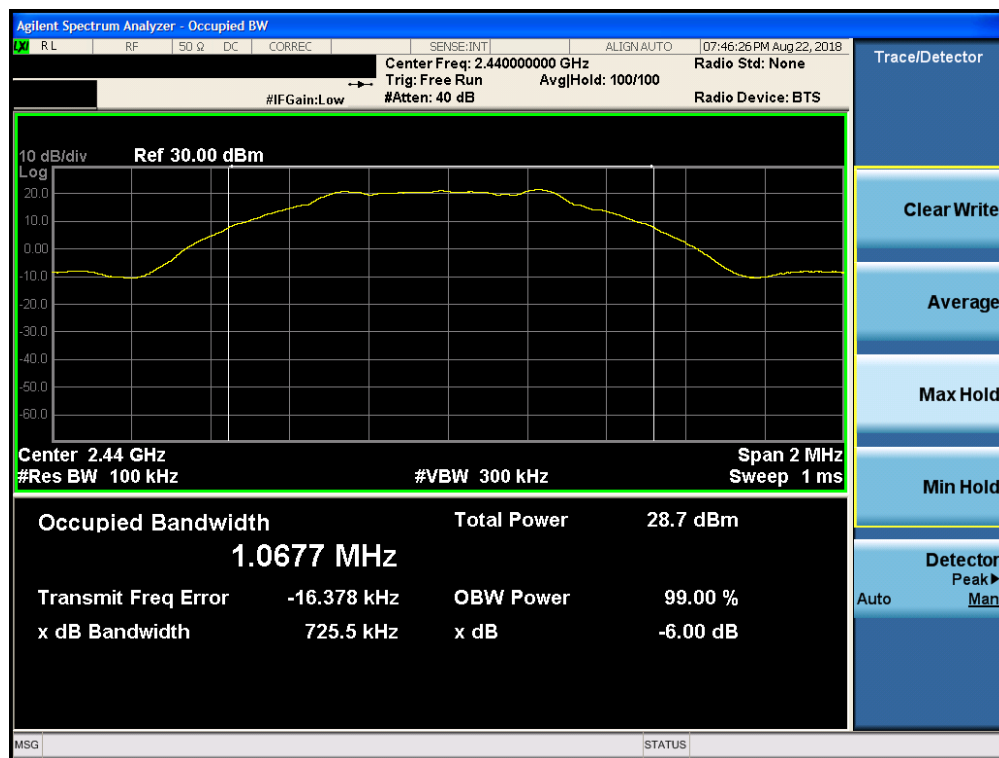
Plot 7-2. 6dB Bandwidth Plot (Bluetooth (LE), 1Mbps, ePA – Ch. 19, Antenna 0)
