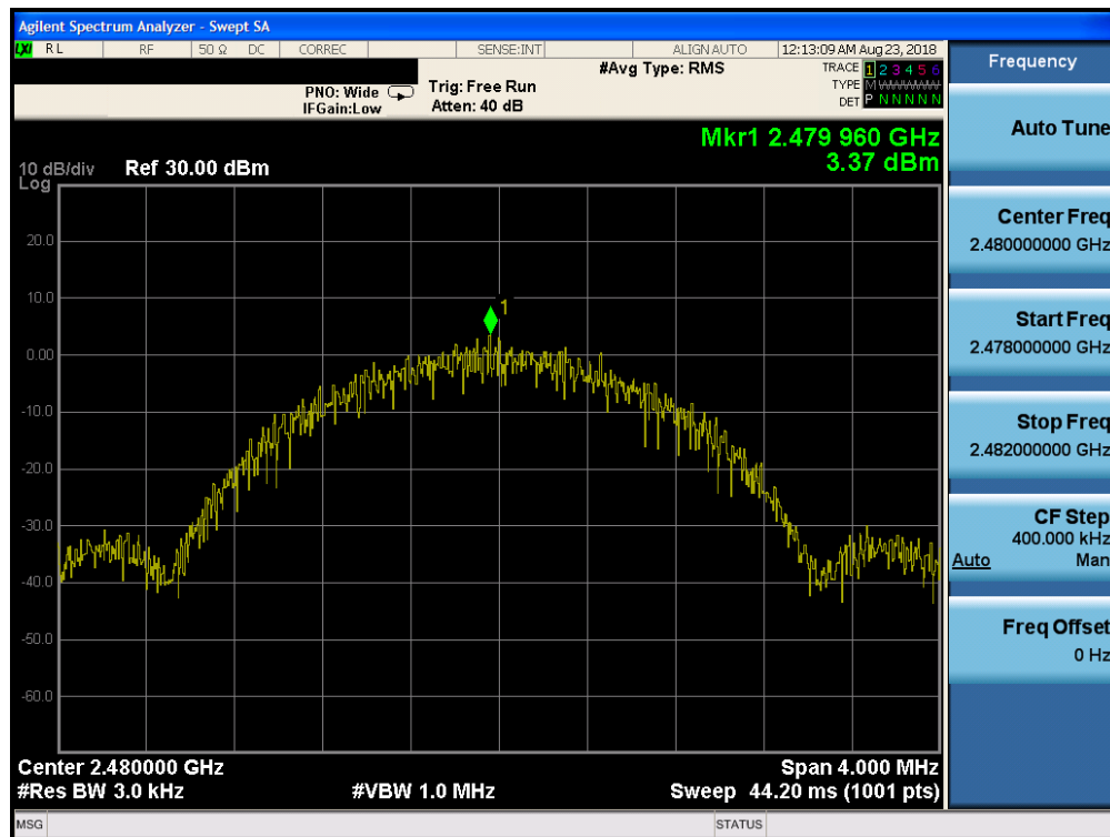
Plot 7-39. Power Spectral Density Plot (Bluetooth (LE), 2Mbps, ePA – Ch. 39, Antenna 1)
