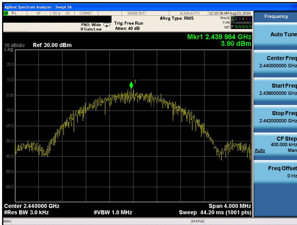
Plot 7-38. Power Spectral Density Plot (Bluetooth (LE), 2Mbps, ePA – Ch. 19, Antenna 1)
