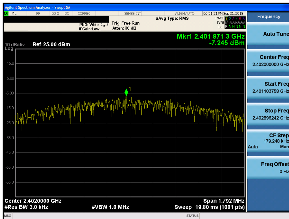
Plot 7-28. Power Spectral Density Plot (Bluetooth (LE), 2Mbps, iPA – Ch. 0, Antenna 0)
