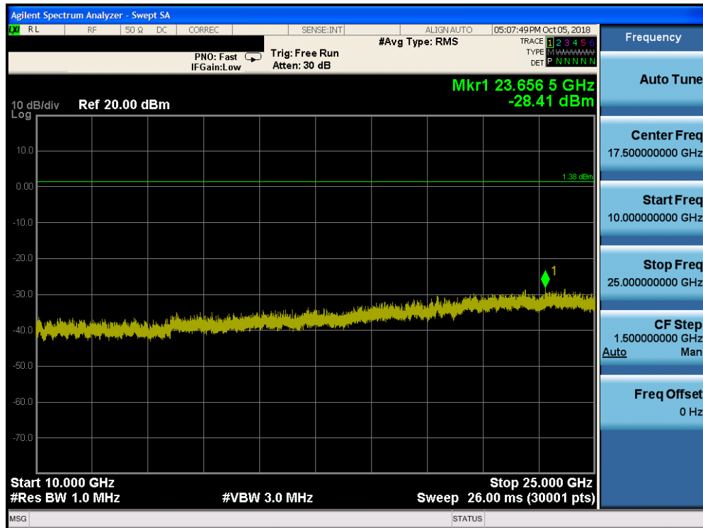
Plot 7-62. Conducted Spurious Plot (Bluetooth (LE), 1Mbps, ePA – Ch. 0, Antenna 0)
