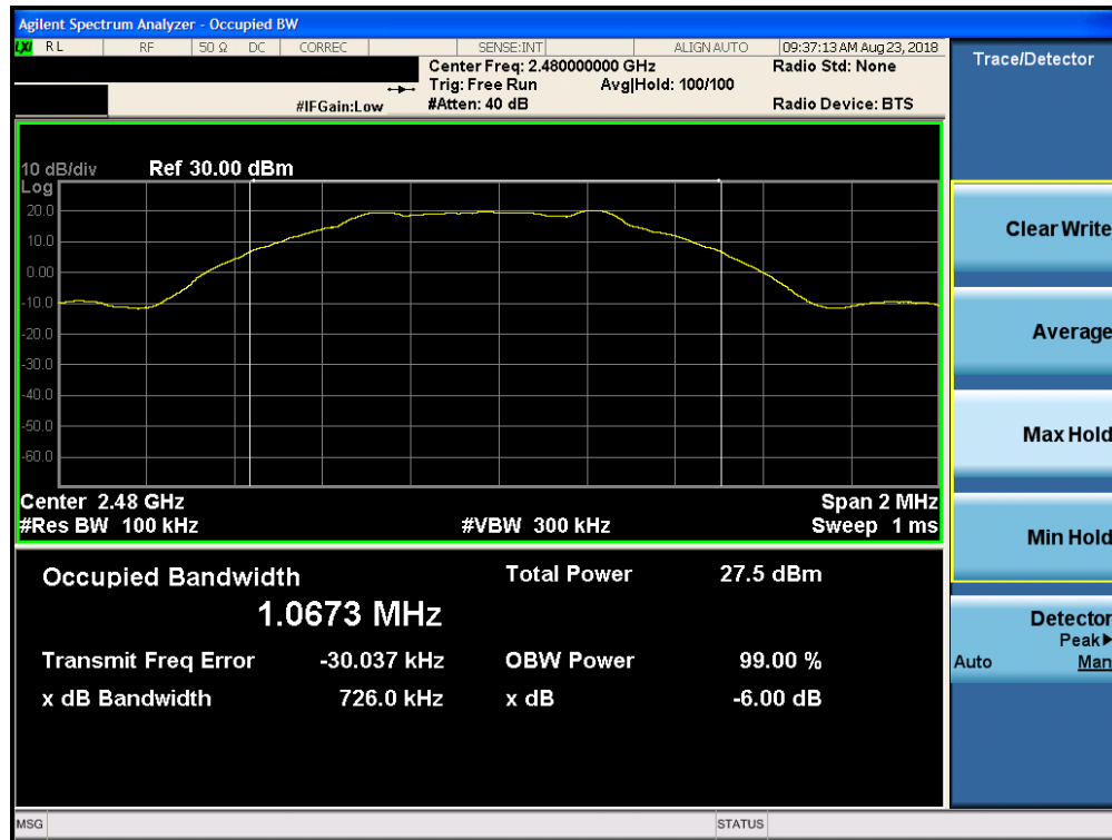
Plot 7-15. 6dB Bandwidth Plot (Bluetooth (LE), 1Mbps, ePA – Ch. 39, Antenna 2)
