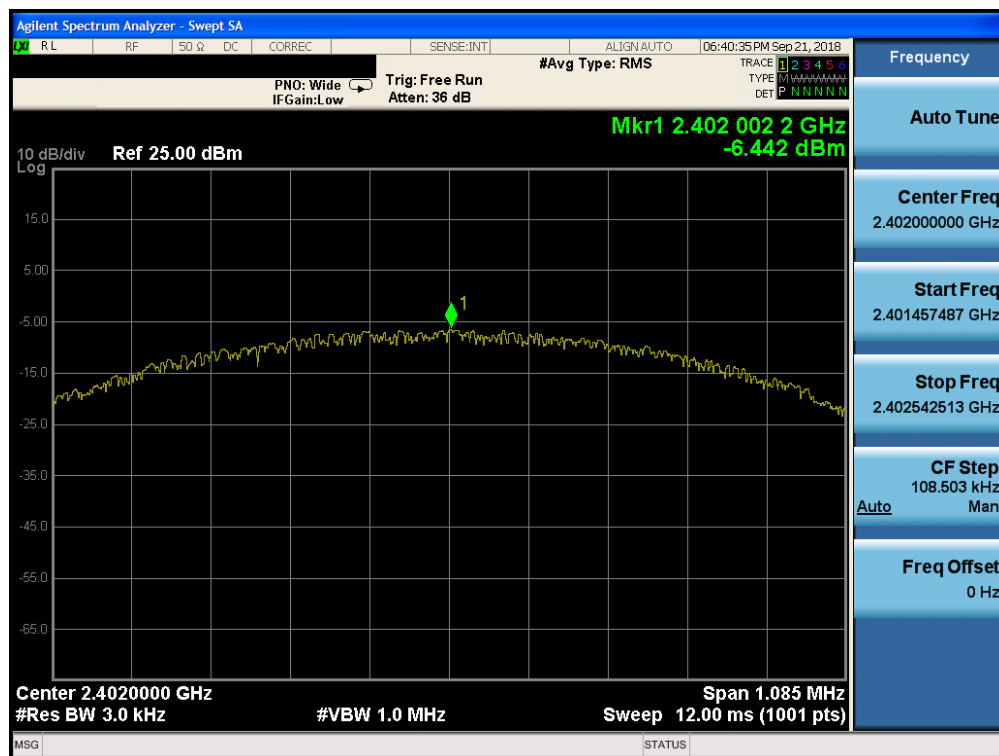
Plot 7-46. Power Spectral Density Plot (Bluetooth (LE), 1Mbps, iPA – Ch. 0, Antenna 2)
