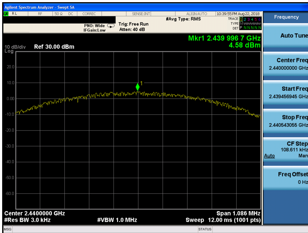
Plot 7-32. Power Spectral Density Plot (Bluetooth (LE), 1Mbps, ePA – Ch. 19, Antenna 1)
