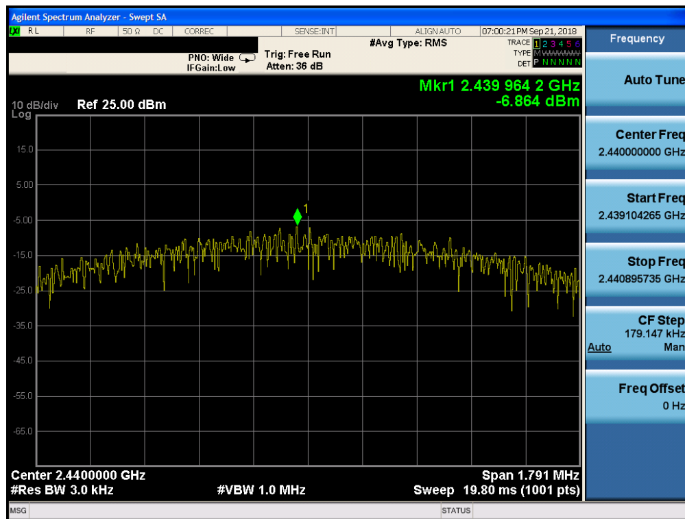
Plot 7-53. Power Spectral Density Plot (Bluetooth (LE), 2Mbps, iPA – Ch. 19, Antenna 2)
