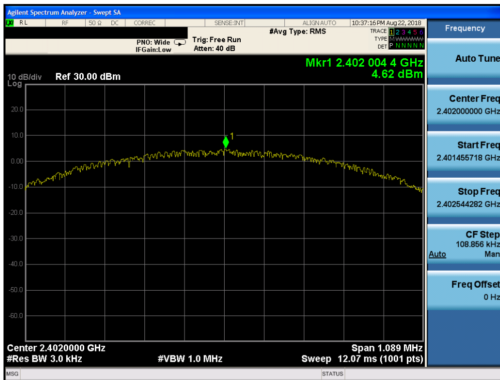
Plot 7-31. Power Spectral Density Plot (Bluetooth (LE), 1Mbps, ePA – Ch. 0, Antenna 1)
