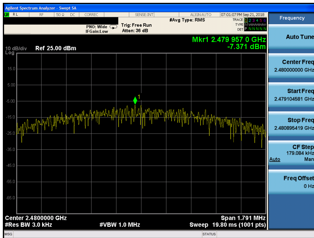
Plot 7-54. Power Spectral Density Plot (Bluetooth (LE), 2Mbps, iPA – Ch. 39, Antenna 2)
