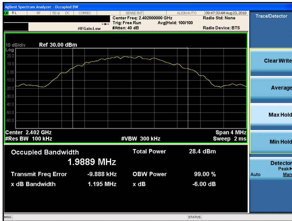
Plot 7-16. 6dB Bandwidth Plot (Bluetooth (LE), 2Mbps, ePA – Ch. 0, Antenna 2)
