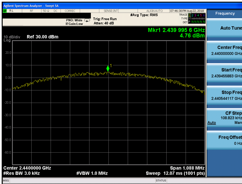
Plot 7-20. Power Spectral Density Plot (Bluetooth (LE), 1Mbps, ePA – Ch. 19, Antenna 0)
