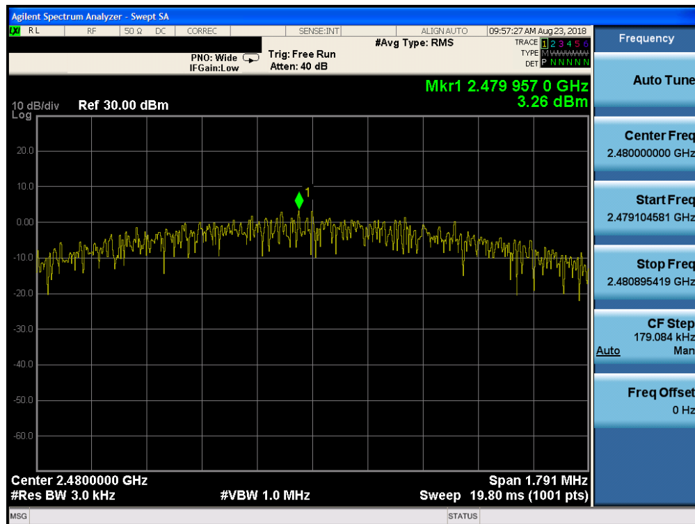
Plot 7-51. Power Spectral Density Plot (Bluetooth (LE), 2Mbps, ePA – Ch. 39, Antenna 2)
