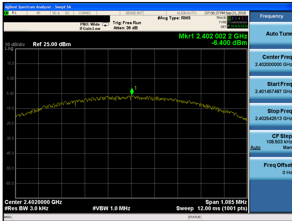
Plot 7-22. Power Spectral Density Plot (Bluetooth (LE), 1Mbps, iPA – Ch. 0, Antenna 0)
