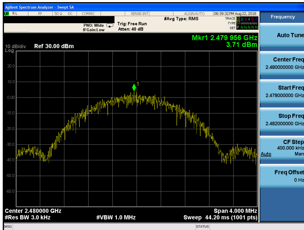
Plot 7-27. Power Spectral Density Plot (Bluetooth (LE), 2Mbps, ePA – Ch. 39, Antenna 0)
