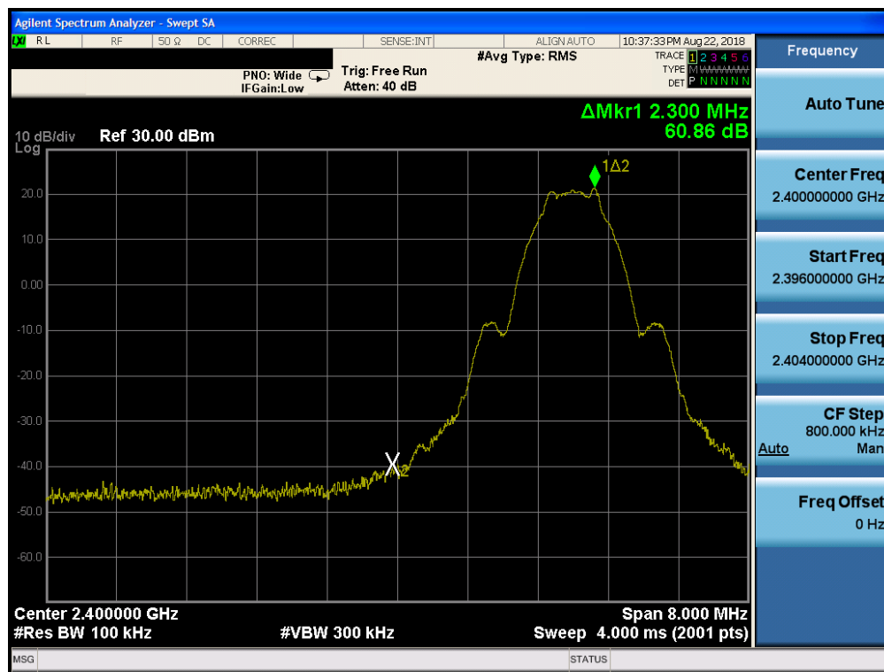
Plot 7-57. Band Edge Plot (Bluetooth (LE), ePA – Ch. 0, Antenna 1)
