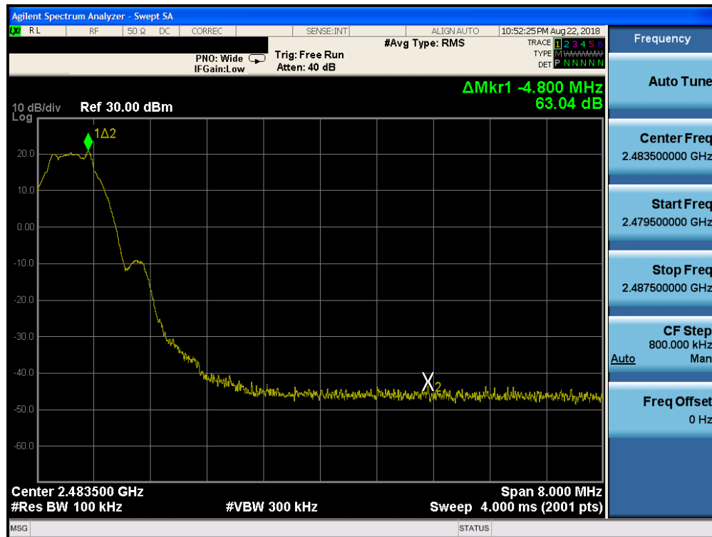
Plot 7-58. Band Edge Plot (Bluetooth (LE), ePA – Ch. 39, Antenna 1)
