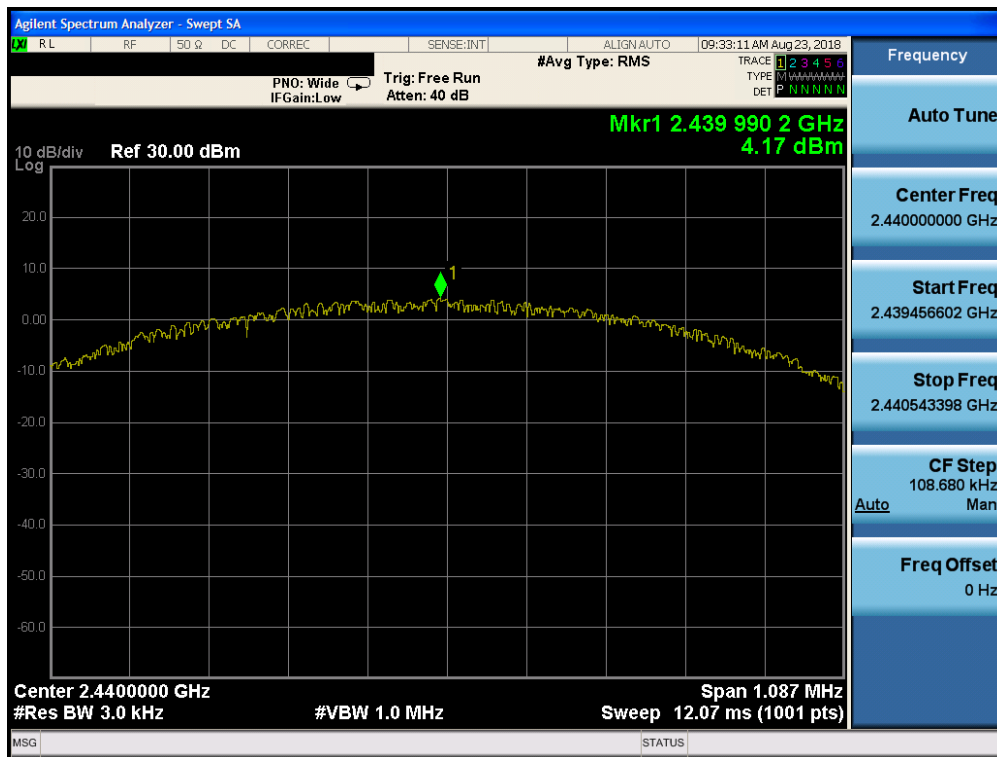
Plot 7-44. Power Spectral Density Plot (Bluetooth (LE), 1Mbps, ePA – Ch. 19, Antenna 2)
