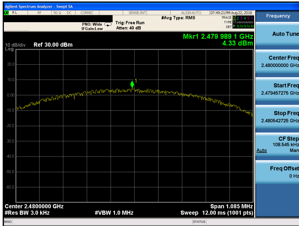
Plot 7-21. Power Spectral Density Plot (Bluetooth (LE), 1Mbps, ePA – Ch. 39, Antenna 0)
