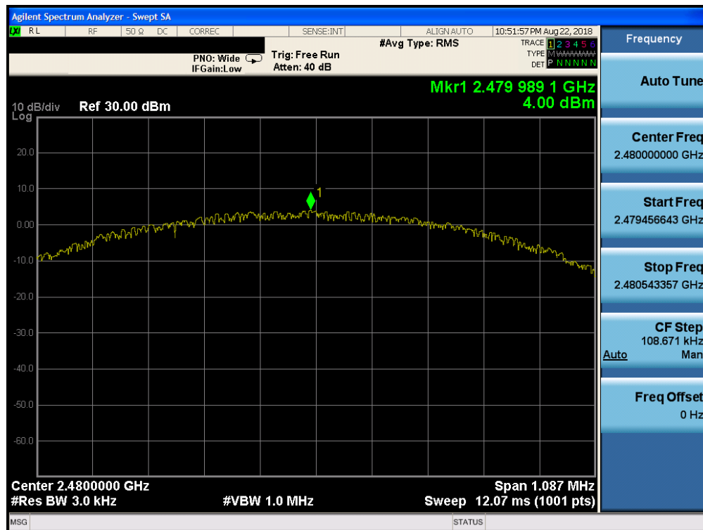
Plot 7-33. Power Spectral Density Plot (Bluetooth (LE), 1Mbps, ePA – Ch. 39, Antenna 1)
