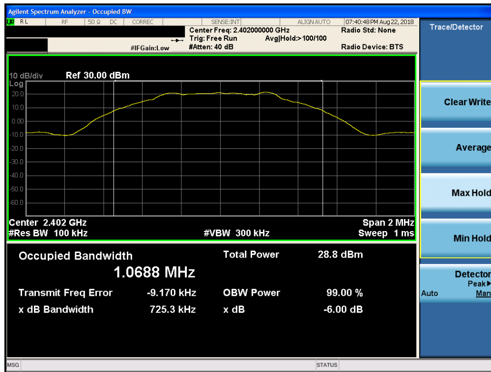
Plot 7-1. 6dB Bandwidth Plot (Bluetooth (LE), 1Mbps, ePA – Ch. 0, Antenna 0)
