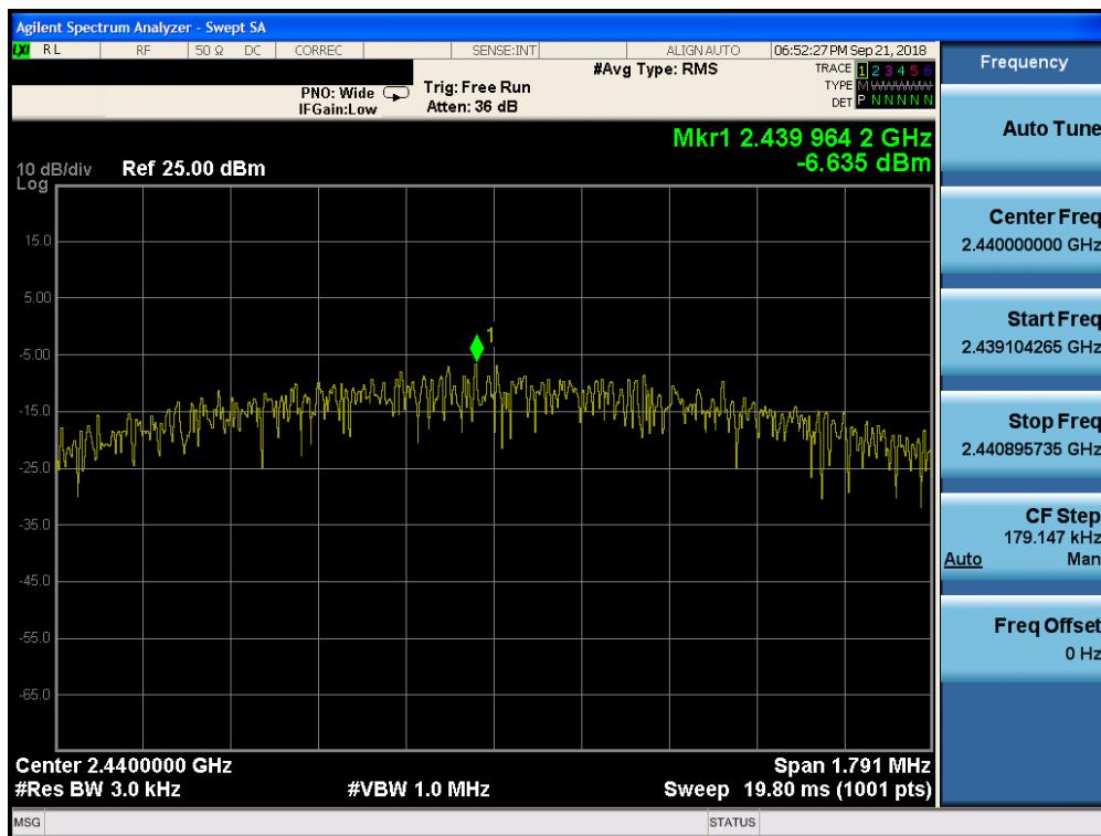
Plot 7-29. Power Spectral Density Plot (Bluetooth (LE), 2Mbps, iPA – Ch. 19, Antenna 0)
