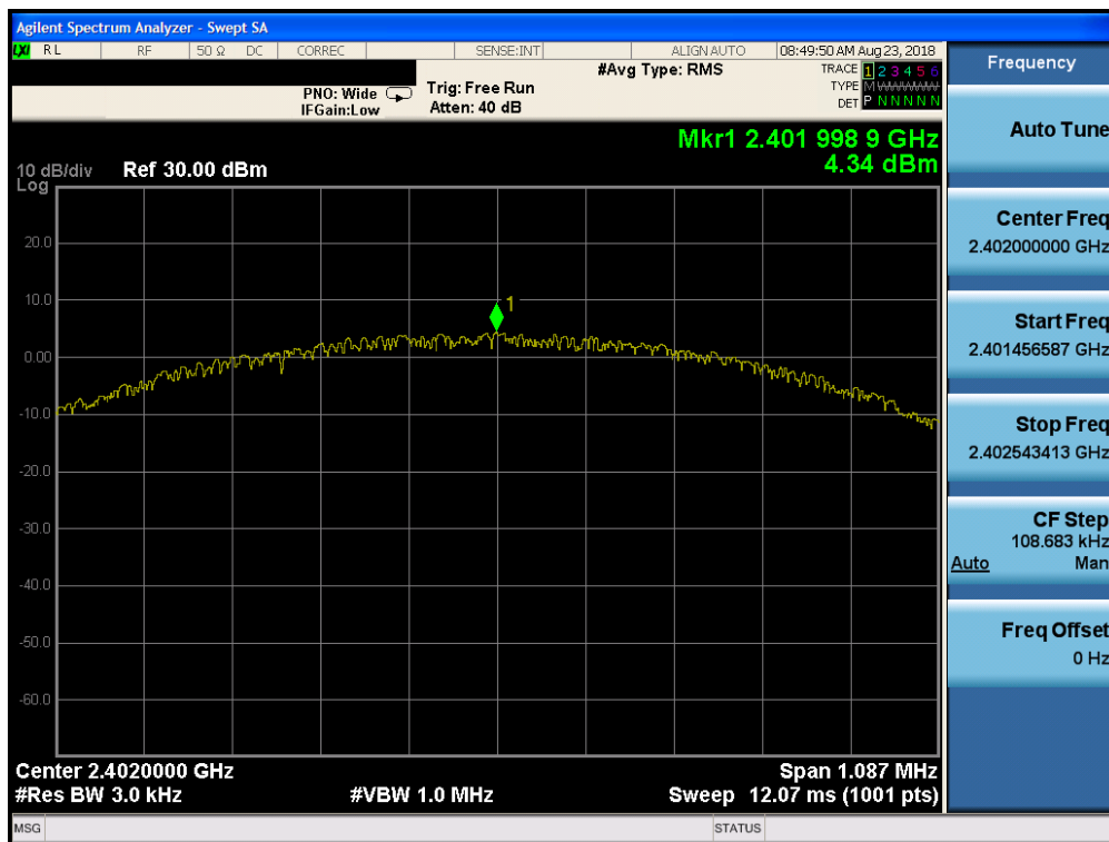
Plot 7-43. Power Spectral Density Plot (Bluetooth (LE), 1Mbps, ePA – Ch. 0, Antenna 2)
