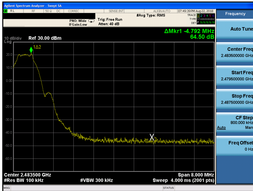
Plot 7-56. Band Edge Plot (Bluetooth (LE), ePA – Ch. 39, Antenna 0)
