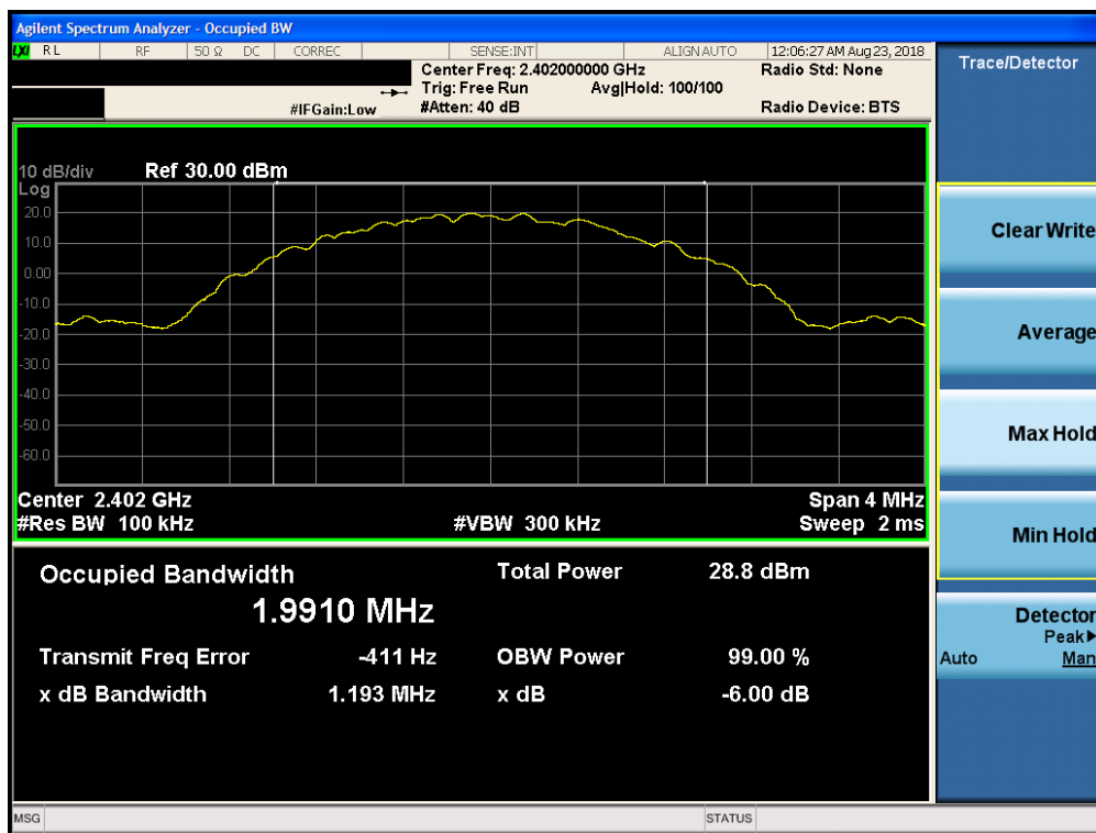
Plot 7-10. 6dB Bandwidth Plot (Bluetooth (LE), 2Mbps, ePA – Ch. 0, Antenna 1)
