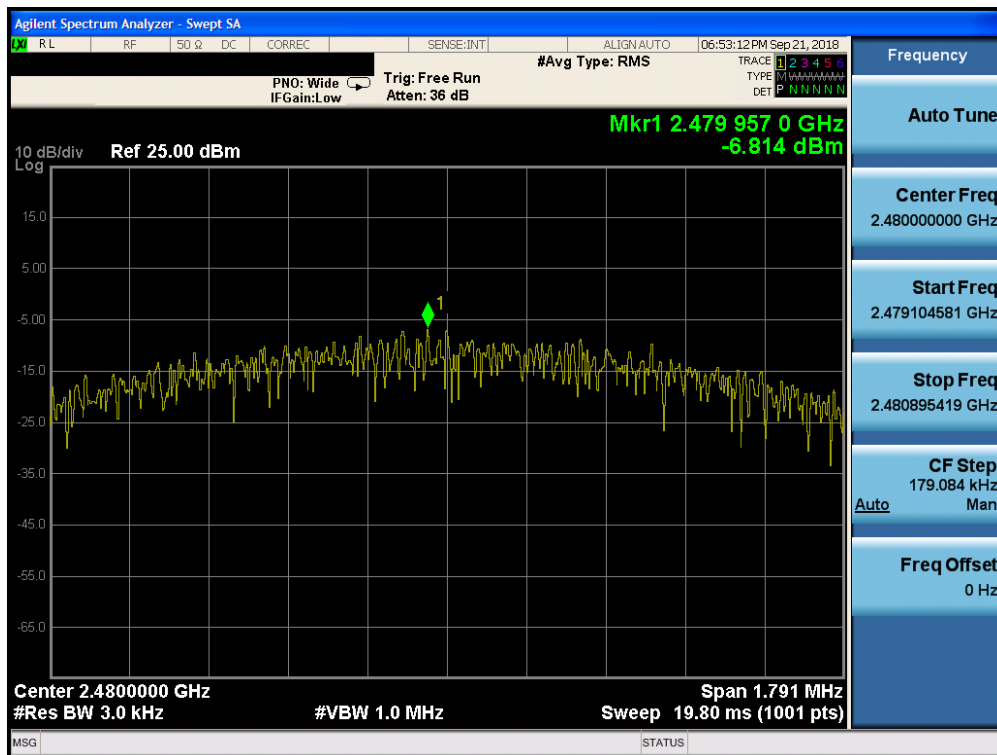
Plot 7-30. Power Spectral Density Plot (Bluetooth (LE), 2Mbps, iPA – Ch. 39, Antenna 0)
