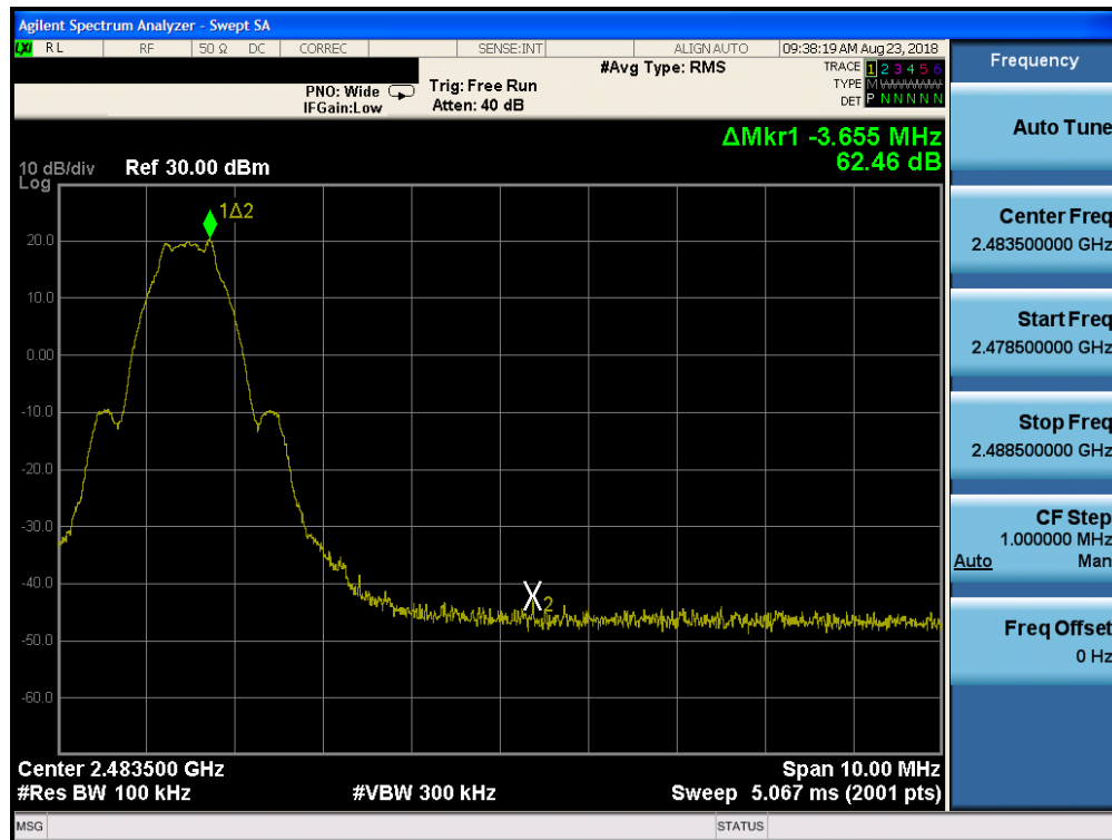
Plot 7-60. Band Edge Plot (Bluetooth (LE), ePA – Ch. 39, Antenna 2)
