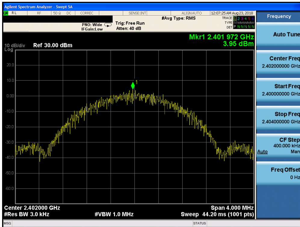
Plot 7-37. Power Spectral Density Plot (Bluetooth (LE), 2Mbps, ePA – Ch. 0, Antenna 1)
