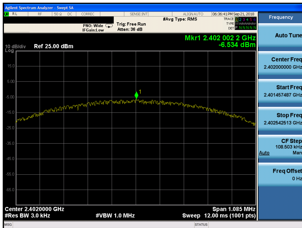
Plot 7-34. Power Spectral Density Plot (Bluetooth (LE), 1Mbps, iPA – Ch. 0, Antenna 1)
