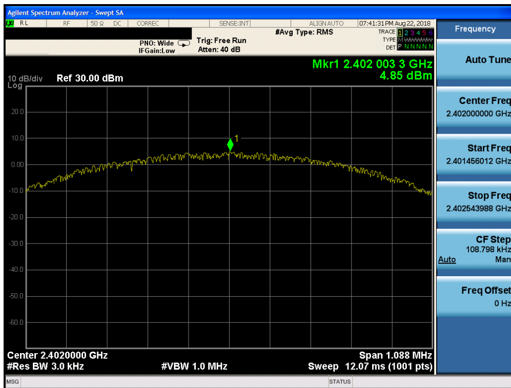
Plot 7-19. Power Spectral Density Plot (Bluetooth (LE), 1Mbps, ePA – Ch. 0, Antenna 0)
