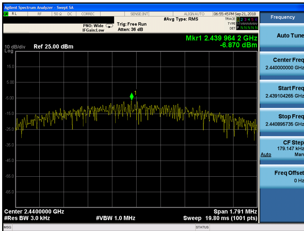
Plot 7-41. Power Spectral Density Plot (Bluetooth (LE), 2Mbps, iPA – Ch. 19, Antenna 1)
