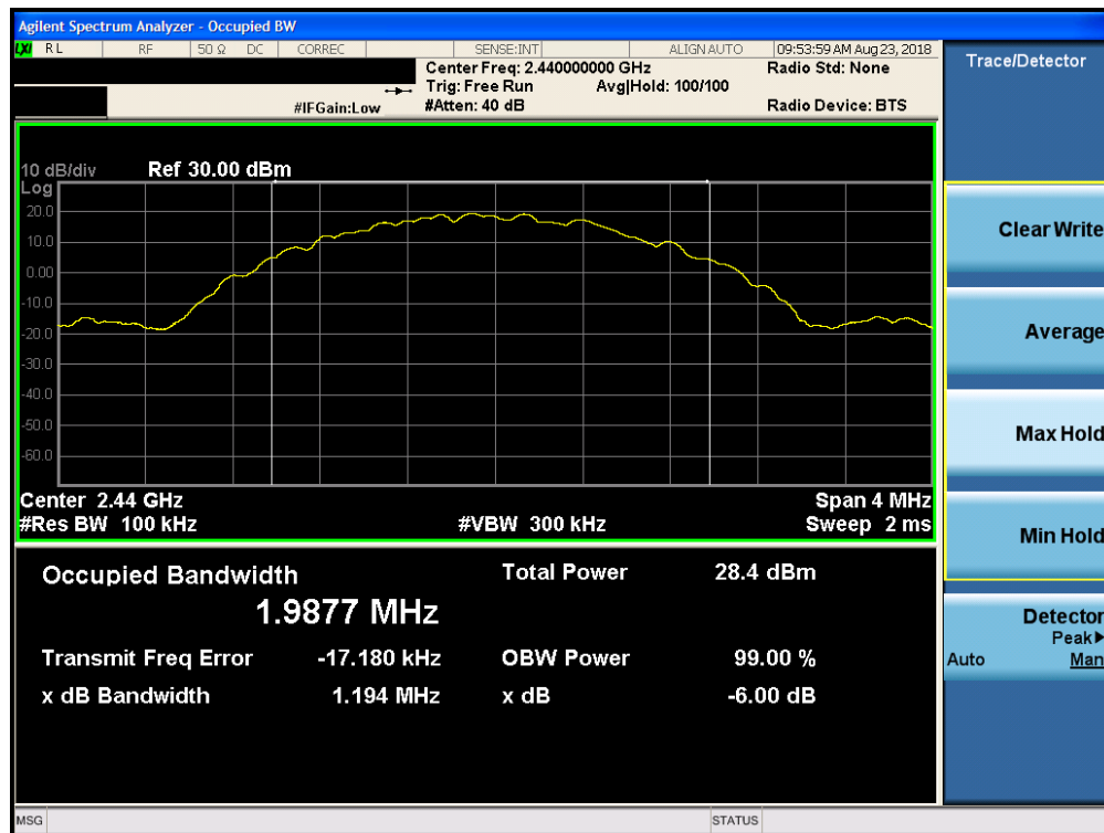
Plot 7-17. 6dB Bandwidth Plot (Bluetooth (LE), 2Mbps, ePA – Ch. 19, Antenna 2)
