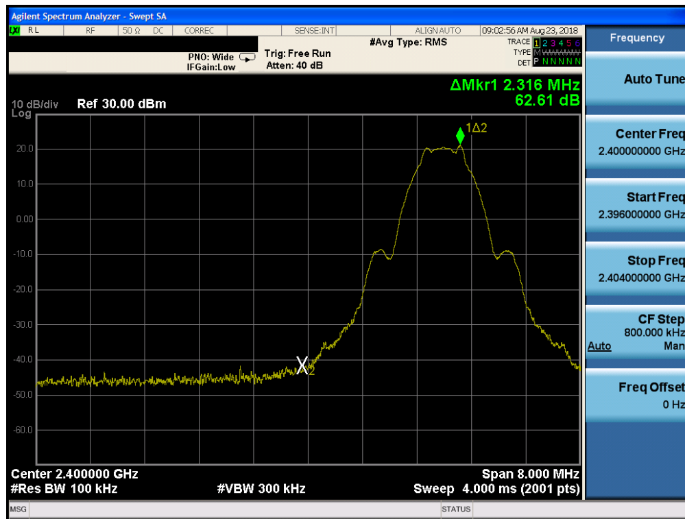
Plot 7-59. Band Edge Plot (Bluetooth (LE), ePA – Ch. 0, Antenna 2)
