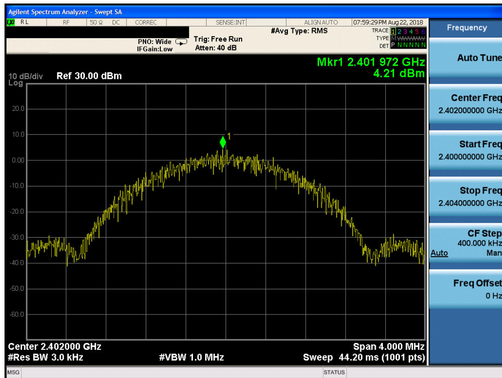
Plot 7-25. Power Spectral Density Plot (Bluetooth (LE), 2Mbps, ePA – Ch. 0, Antenna 0)
