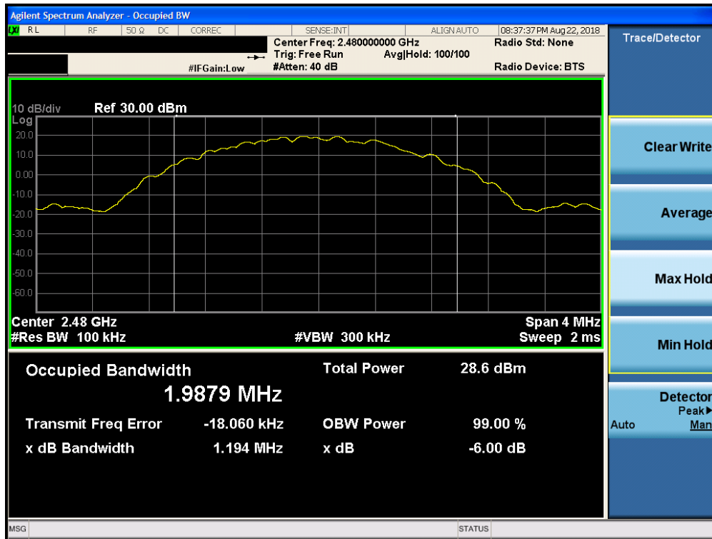
Plot 7-6. 6dB Bandwidth Plot (Bluetooth (LE), 2Mbps, ePA – Ch. 39, Antenna 0)
