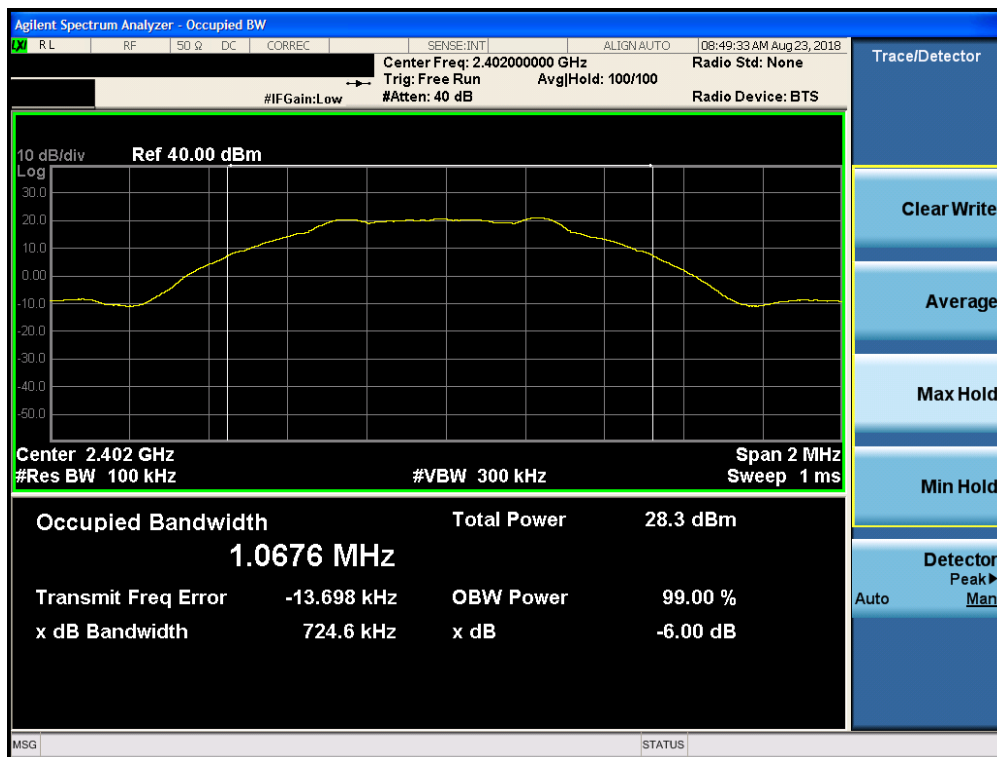
Plot 7-13. 6dB Bandwidth Plot (Bluetooth (LE), 1Mbps, ePA – Ch. 0, Antenna 2)
