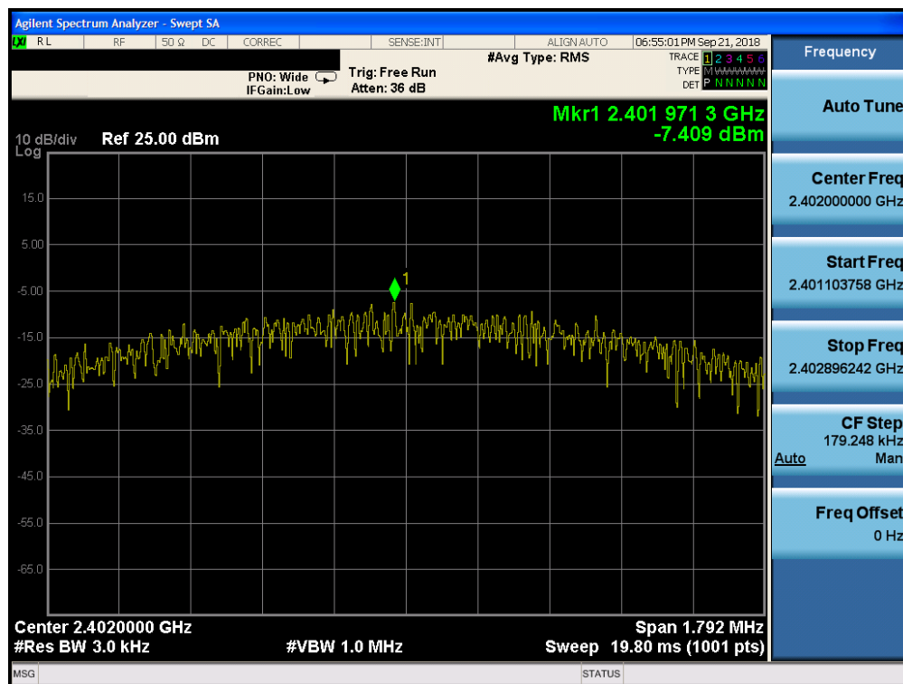
Plot 7-40. Power Spectral Density Plot (Bluetooth (LE), 2Mbps, iPA – Ch. 0, Antenna 1)
