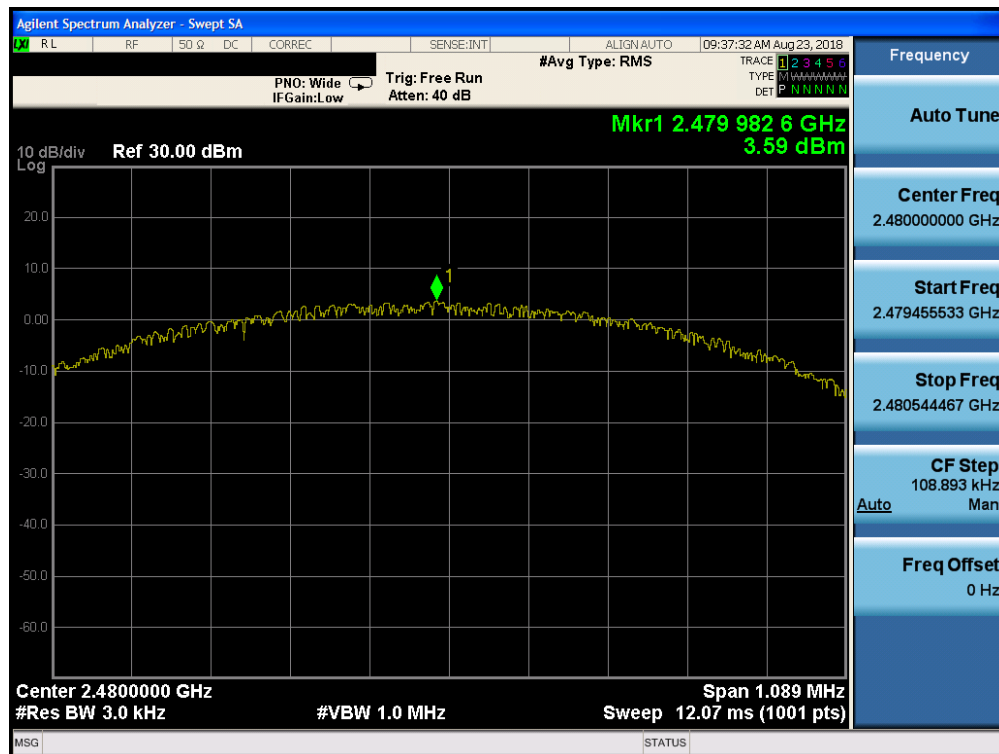
Plot 7-45. Power Spectral Density Plot (Bluetooth (LE), 1Mbps, ePA – Ch. 39, Antenna 2)
