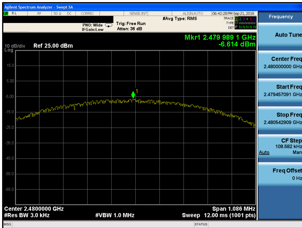
Plot 7-48. Power Spectral Density Plot (Bluetooth (LE), 1Mbps, iPA – Ch. 39, Antenna 2)
