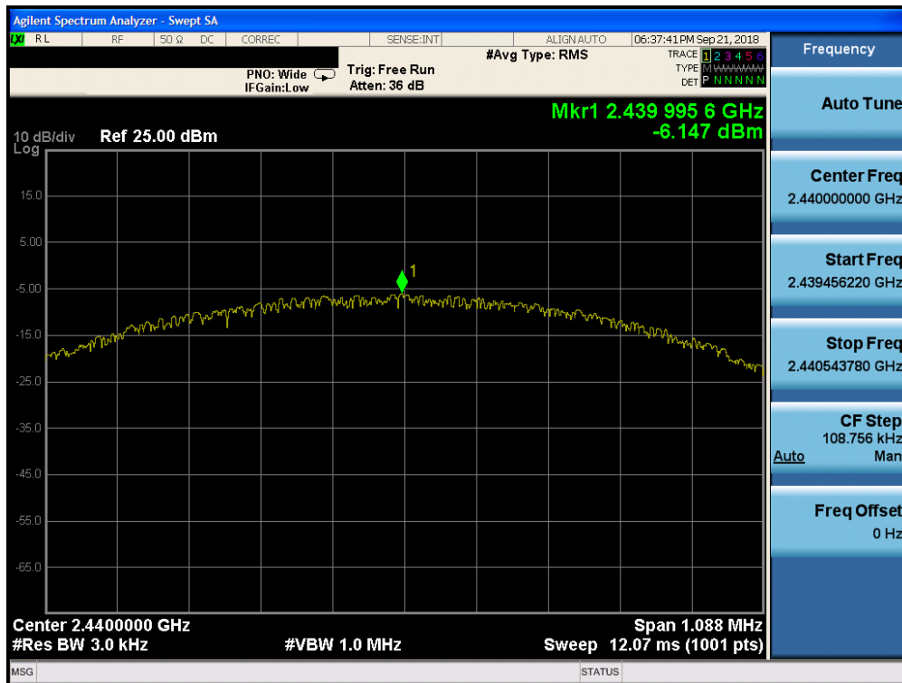
Plot 7-35. Power Spectral Density Plot (Bluetooth (LE), 1Mbps, iPA – Ch. 19, Antenna 1)
